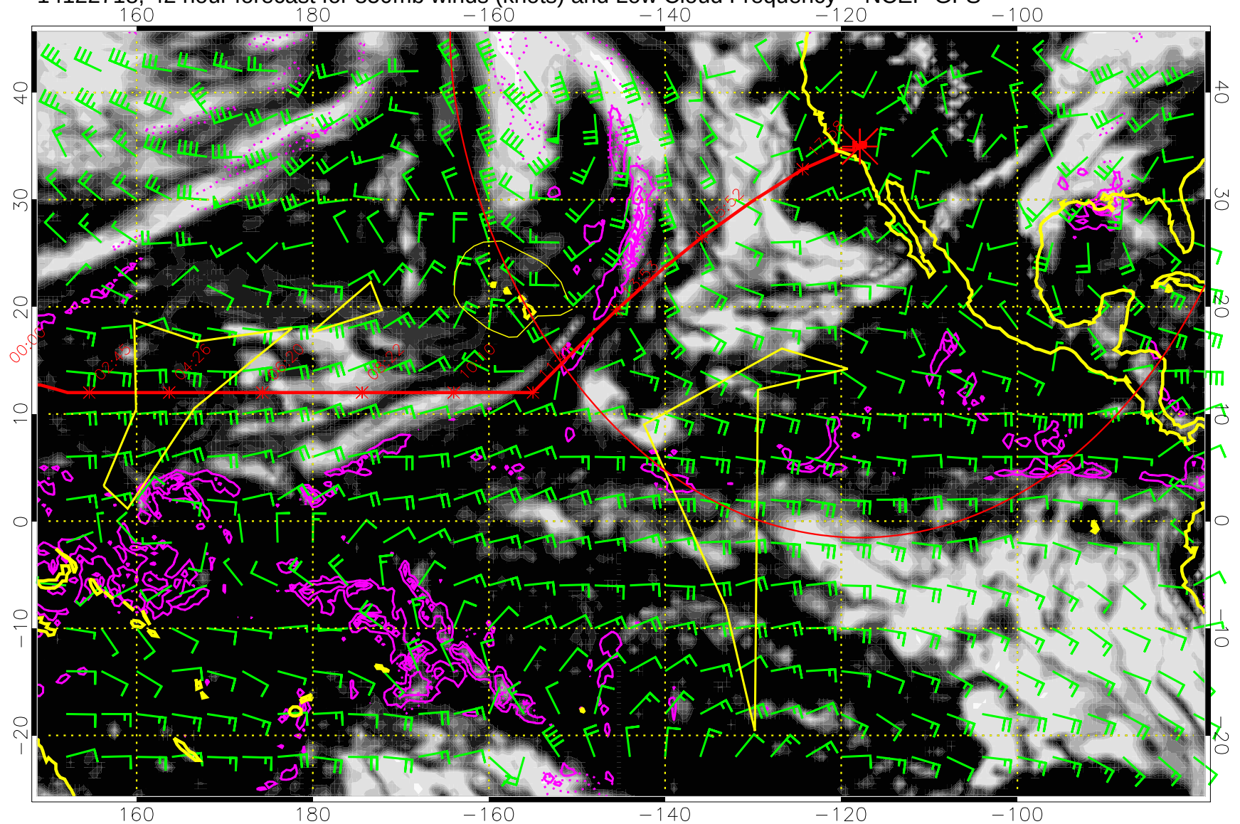
14122718, 42 hour forecast for 850mb winds (knots) and Low Cloud Frequency -- NCEP GFS
