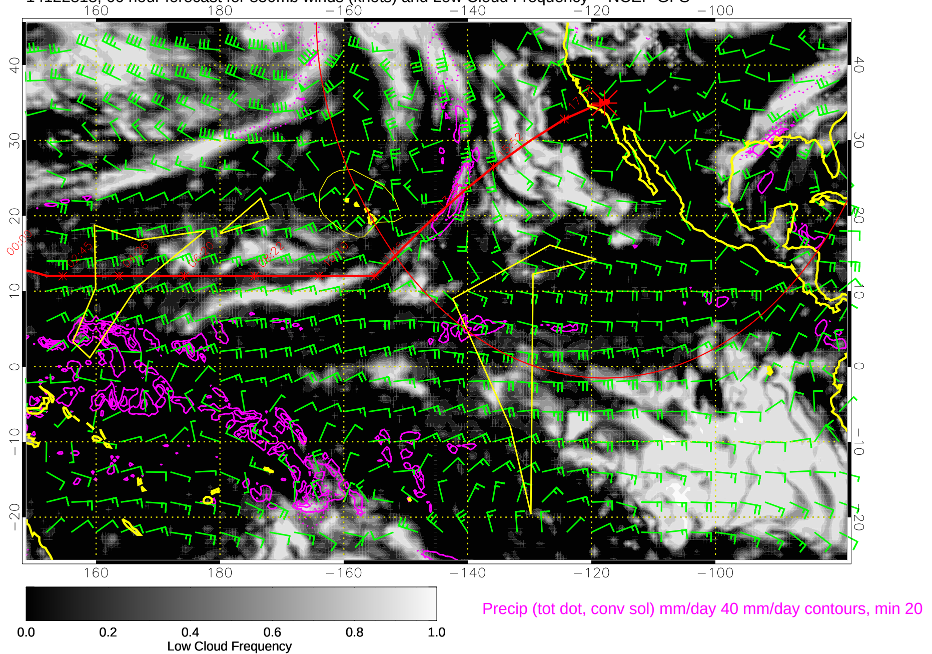
14122818, 66 hour forecast for 850mb winds (knots) and Low Cloud Frequency -- NCEP GFS
