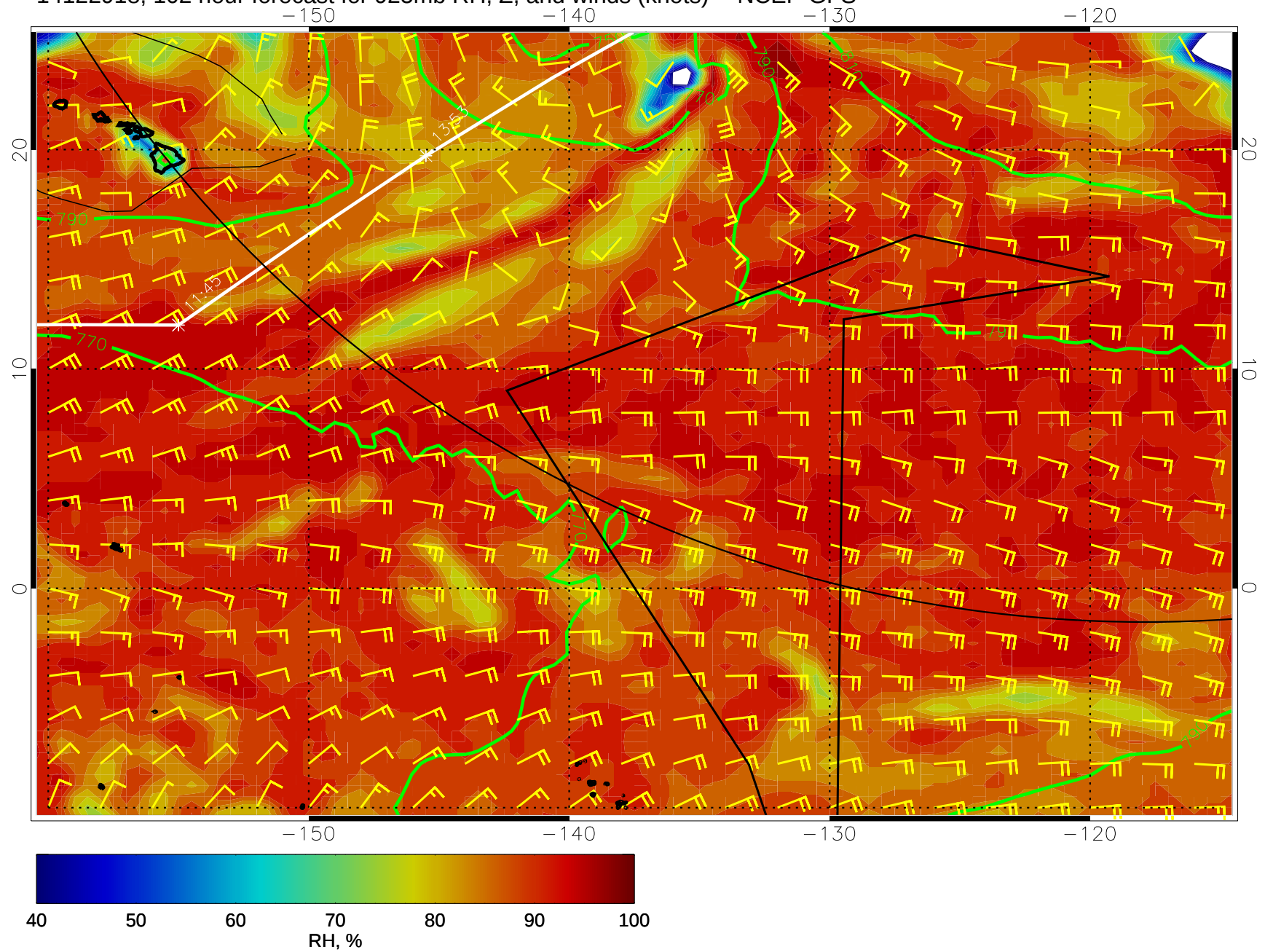
14122918, 102 hour forecast for 925mb RH, Z, and winds (knots) -- NCEP GFS
