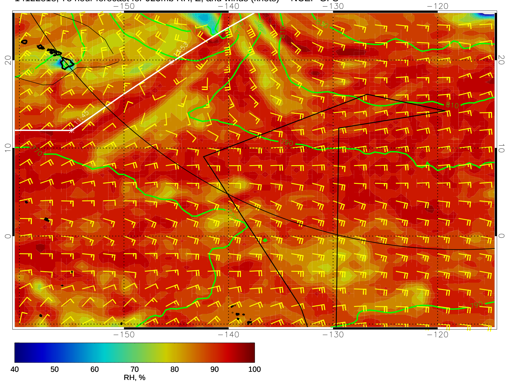
14122818, 78 hour forecast for 925mb RH, Z, and winds (knots) -- NCEP GFS
