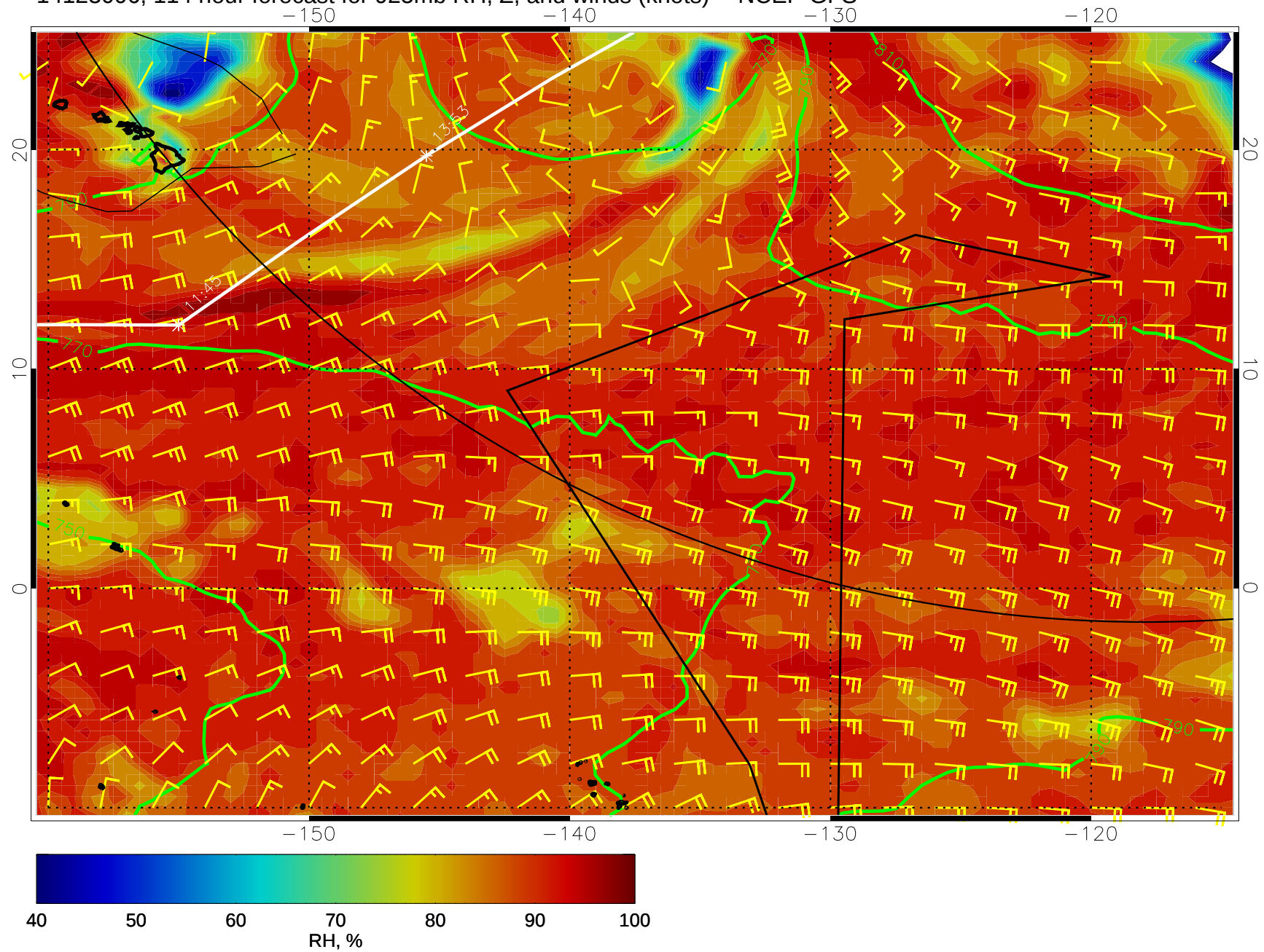
14123006, 114 hour forecast for 925mb RH, Z, and winds (knots) -- NCEP GFS
