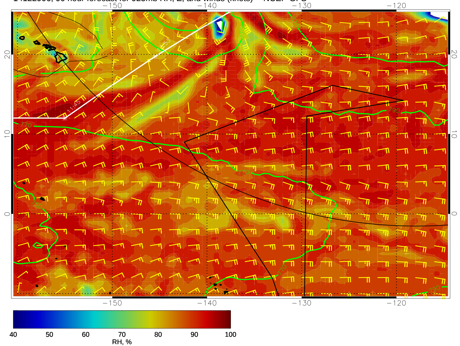
14122906, 90 hour forecast for 925mb RH, Z, and winds (knots) -- NCEP GFS
