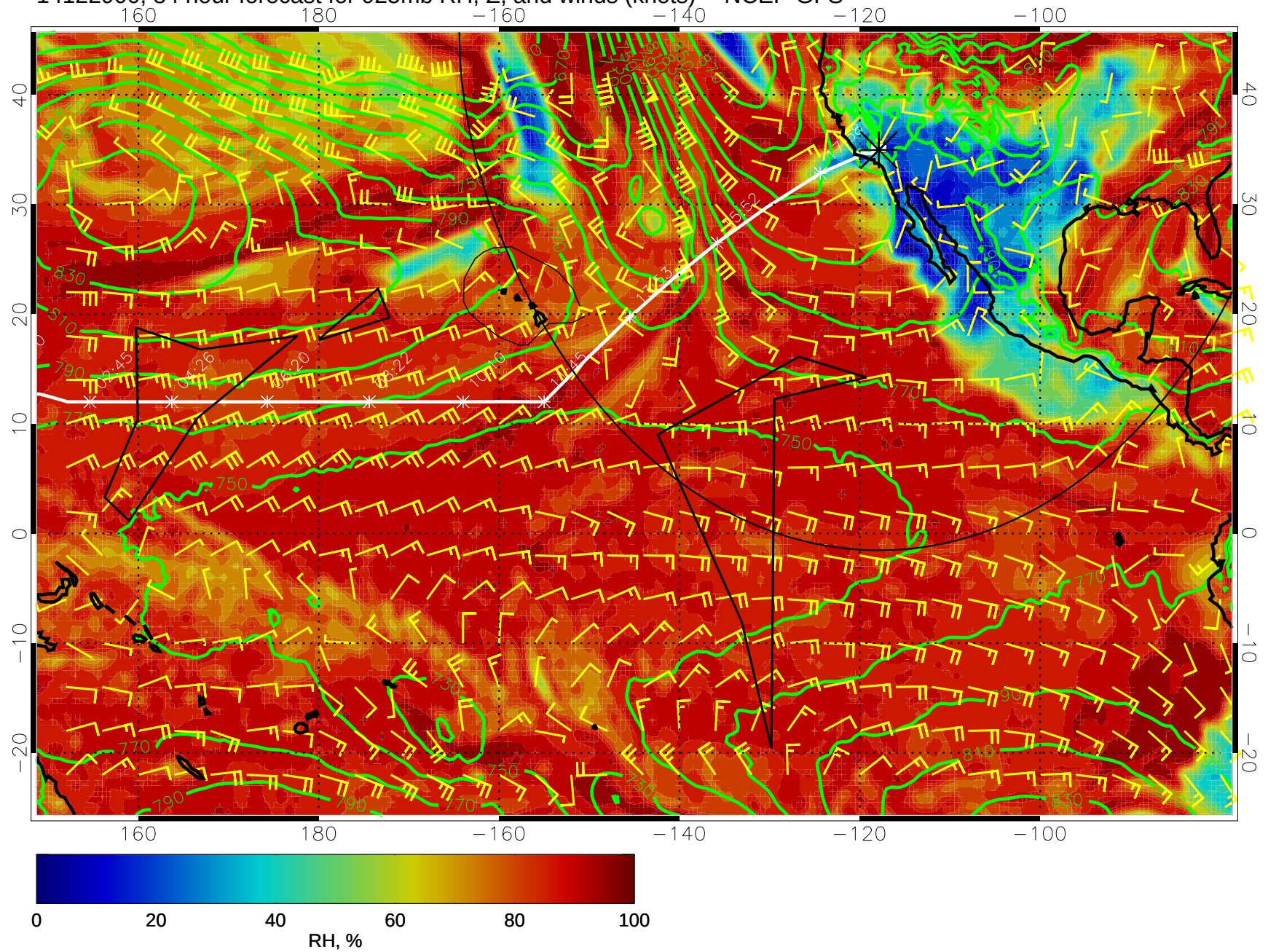
14122900, 84 hour forecast for 925mb RH, Z, and winds (knots) -- NCEP GFS
