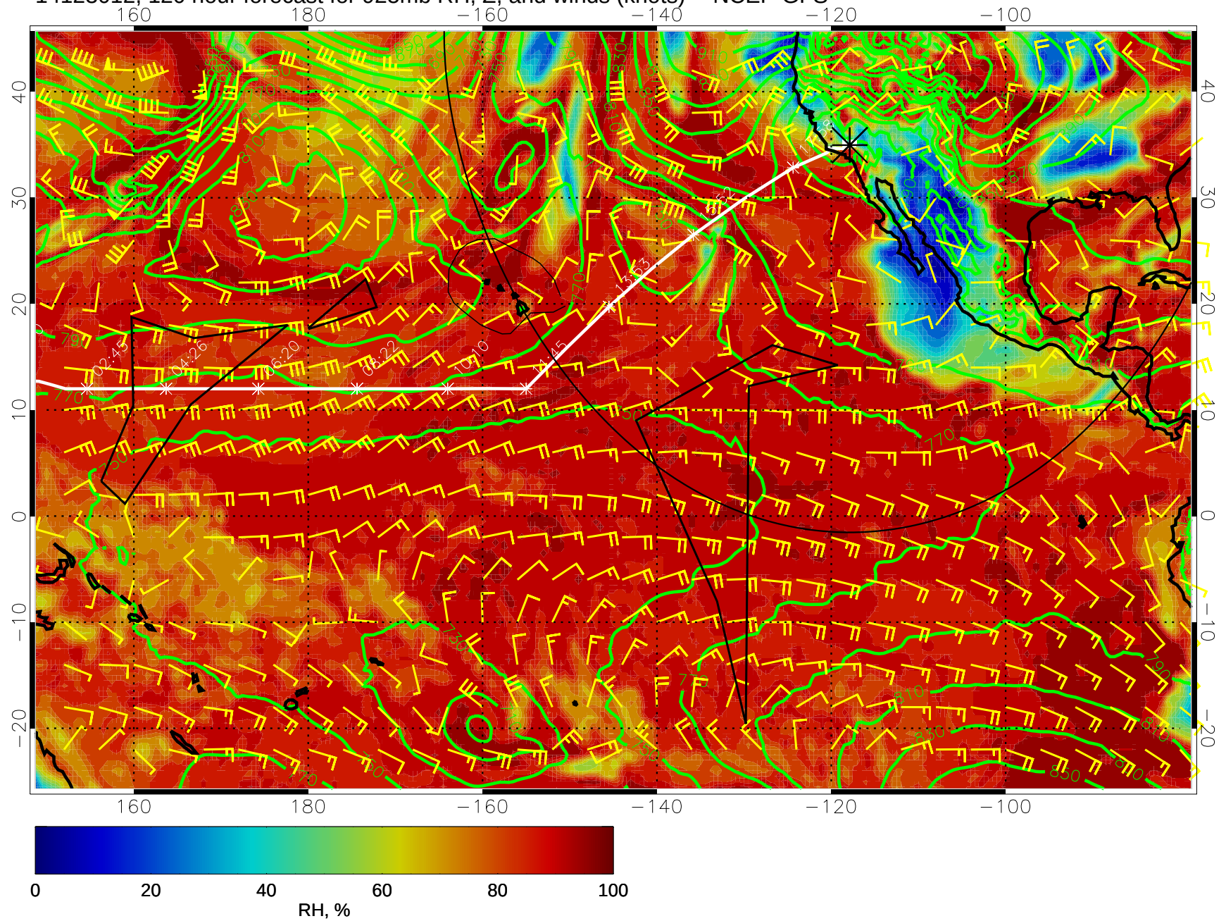
14123012, 120 hour forecast for 925mb RH, Z, and winds (knots) -- NCEP GFS
