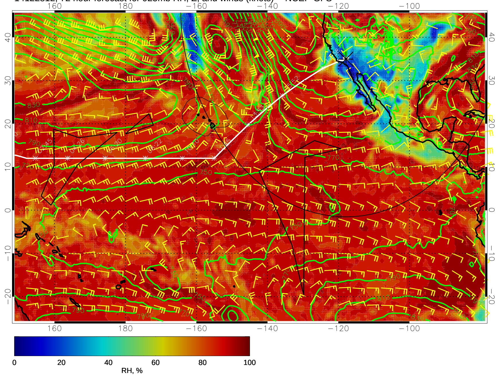
14122812, 72 hour forecast for 925mb RH, Z, and winds (knots) -- NCEP GFS
