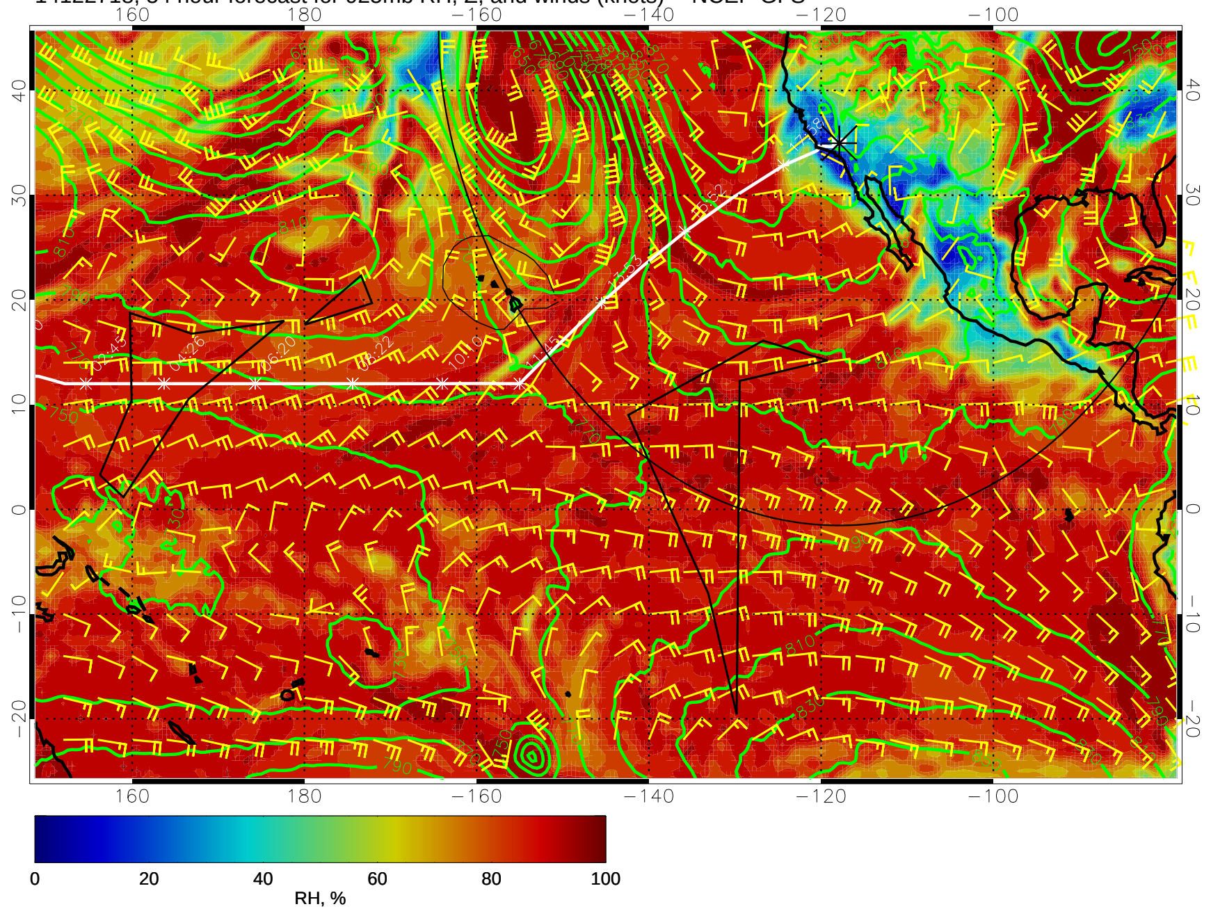
14122718, 54 hour forecast for 925mb RH, Z, and winds (knots) -- NCEP GFS
