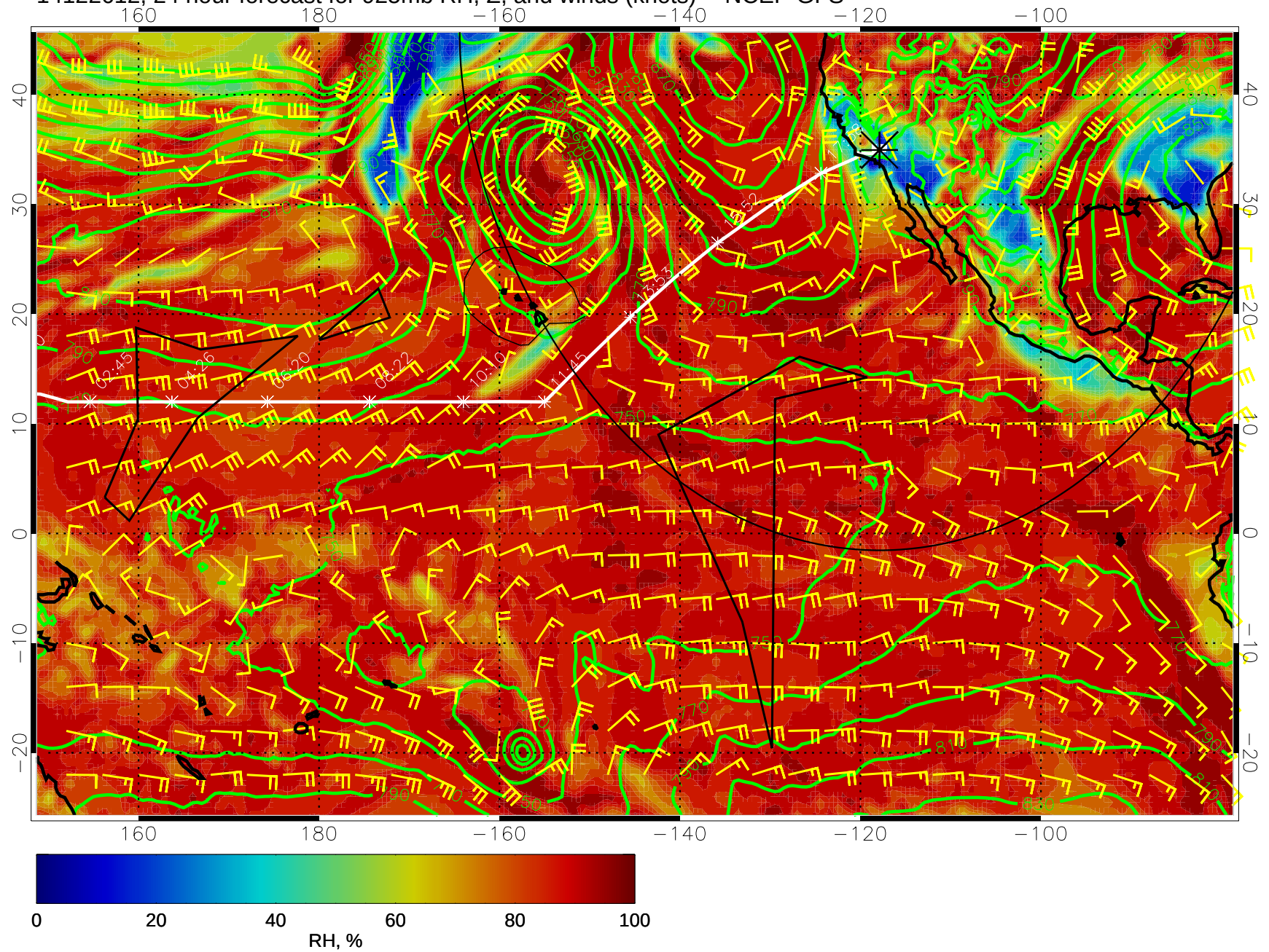
14122612, 24 hour forecast for 925mb RH, Z, and winds (knots) -- NCEP GFS
