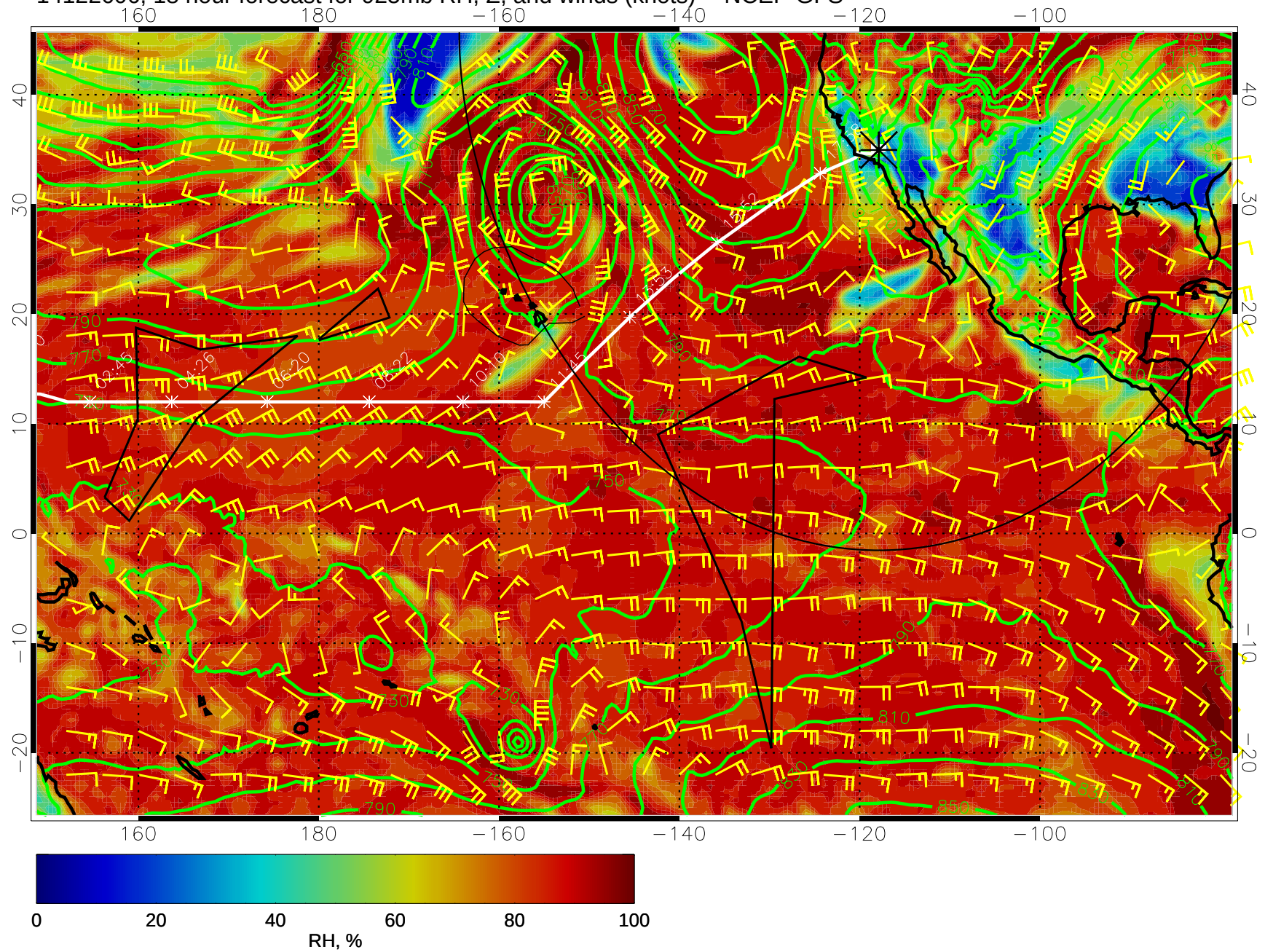
14122606, 18 hour forecast for 925mb RH, Z, and winds (knots) -- NCEP GFS
