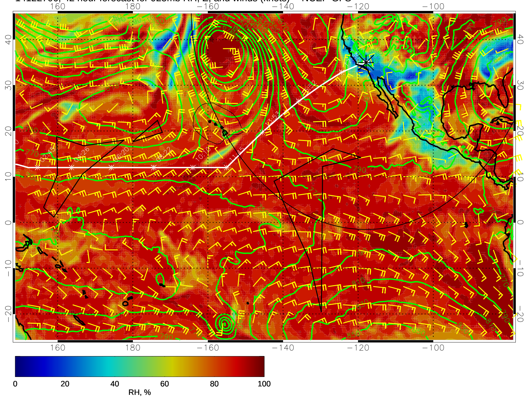
14122706, 42 hour forecast for 925mb RH, Z, and winds (knots) -- NCEP GFS
