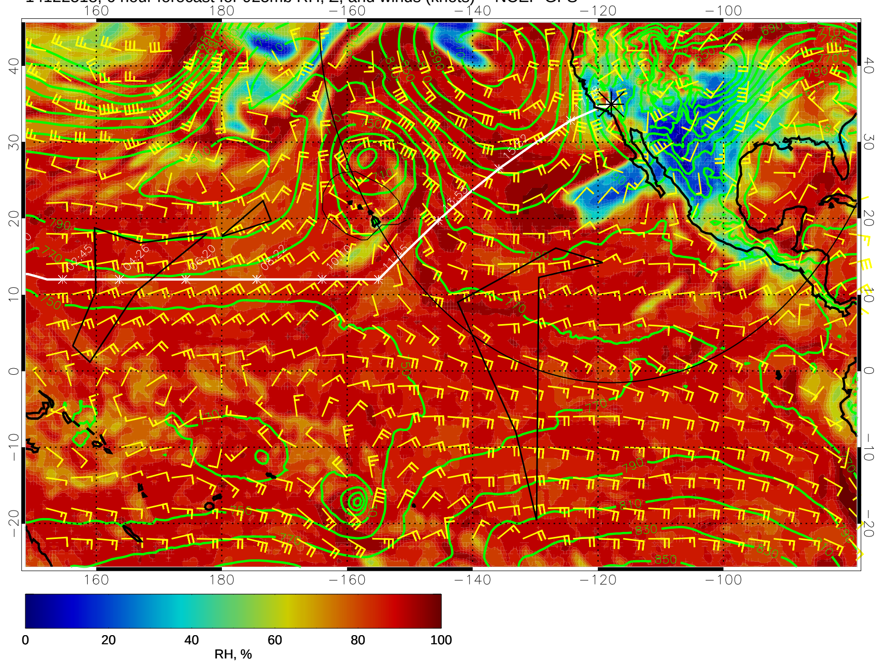
14122518, 6 hour forecast for 925mb RH, Z, and winds (knots) -- NCEP GFS
