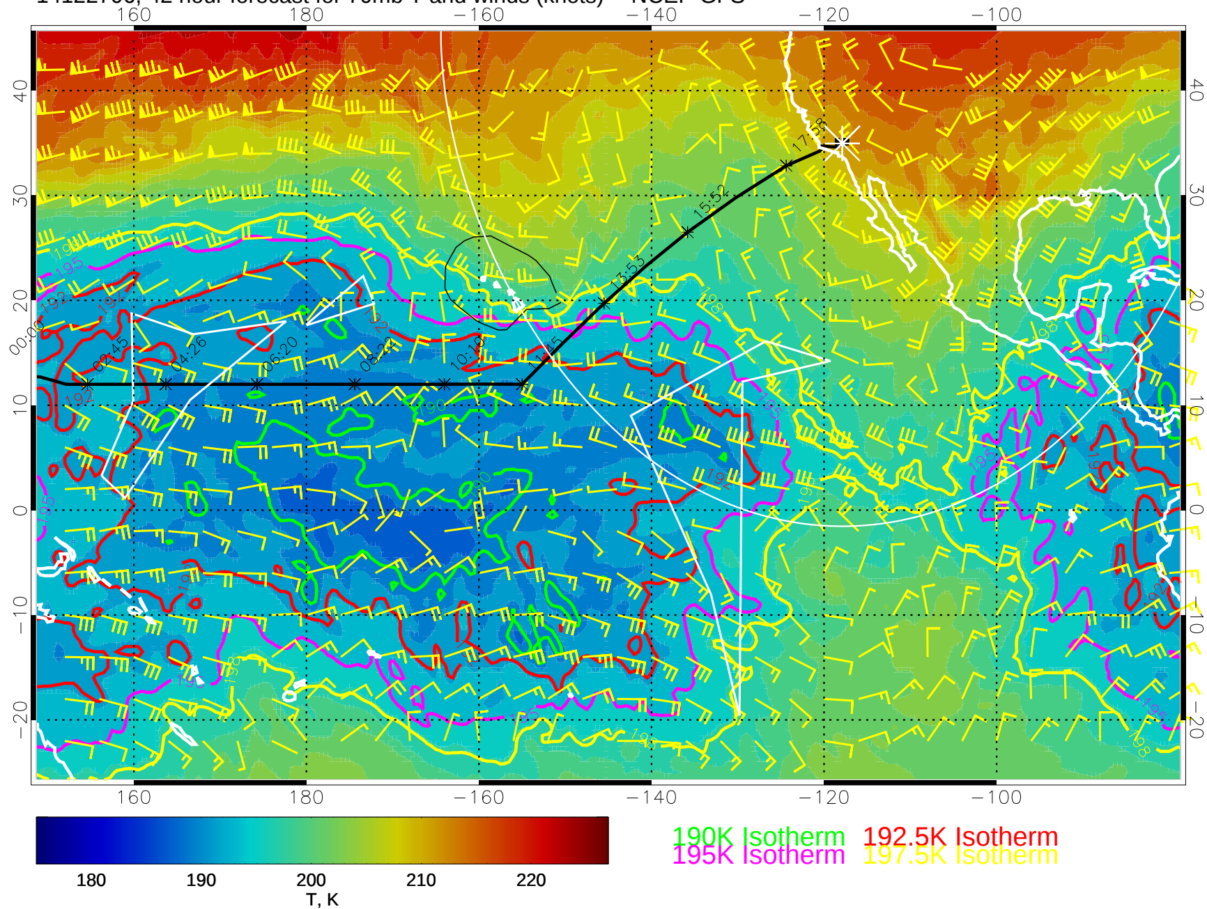
14122706, 42 hour forecast for 70mb T and winds (knots) -- NCEP GFS
