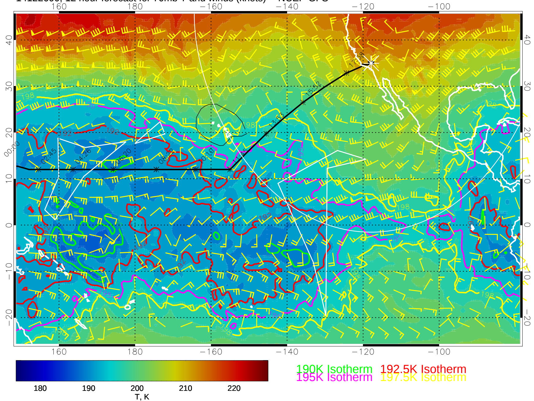
14122600, 12 hour forecast for 70mb T and winds (knots) -- NCEP GFS
