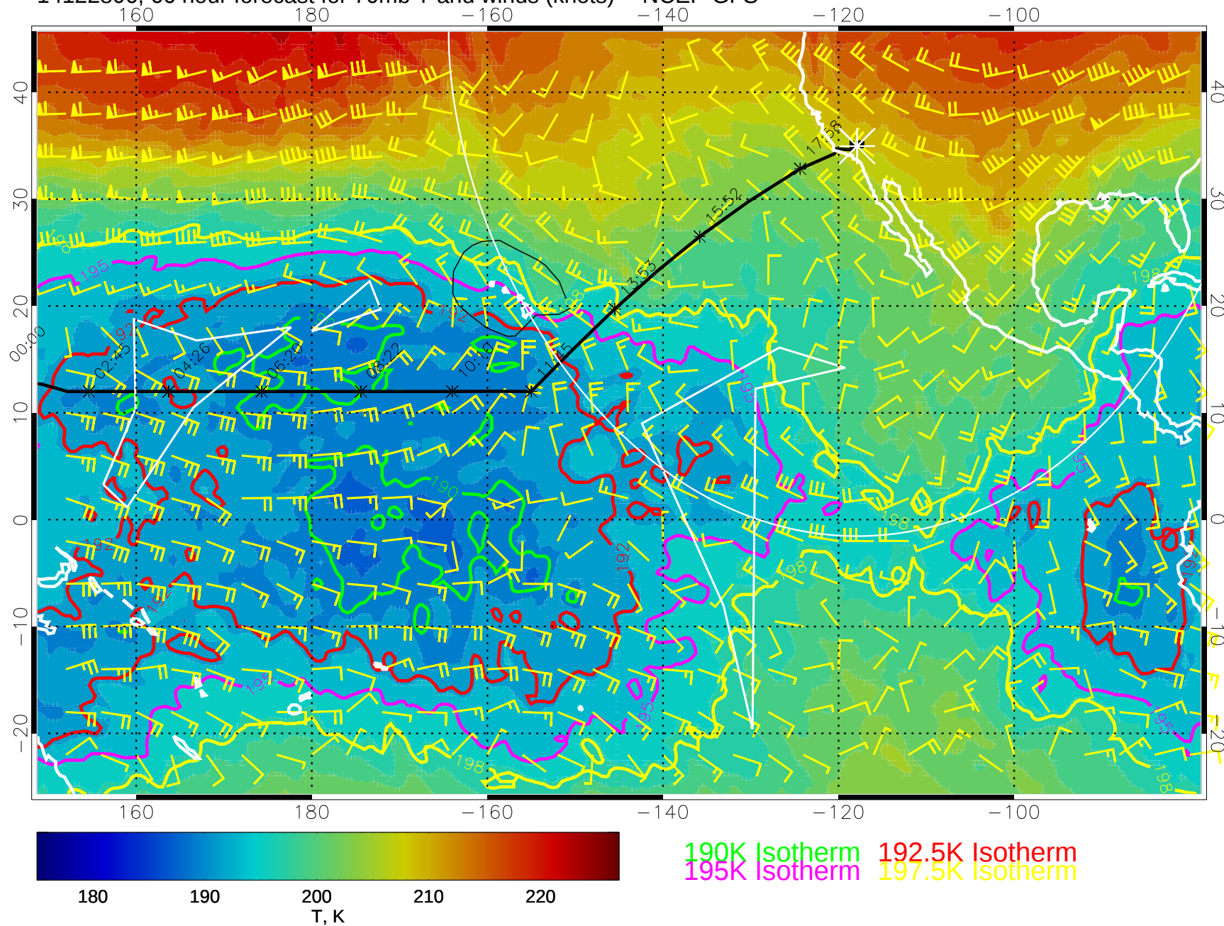
14122806, 66 hour forecast for 70mb T and winds (knots) -- NCEP GFS
