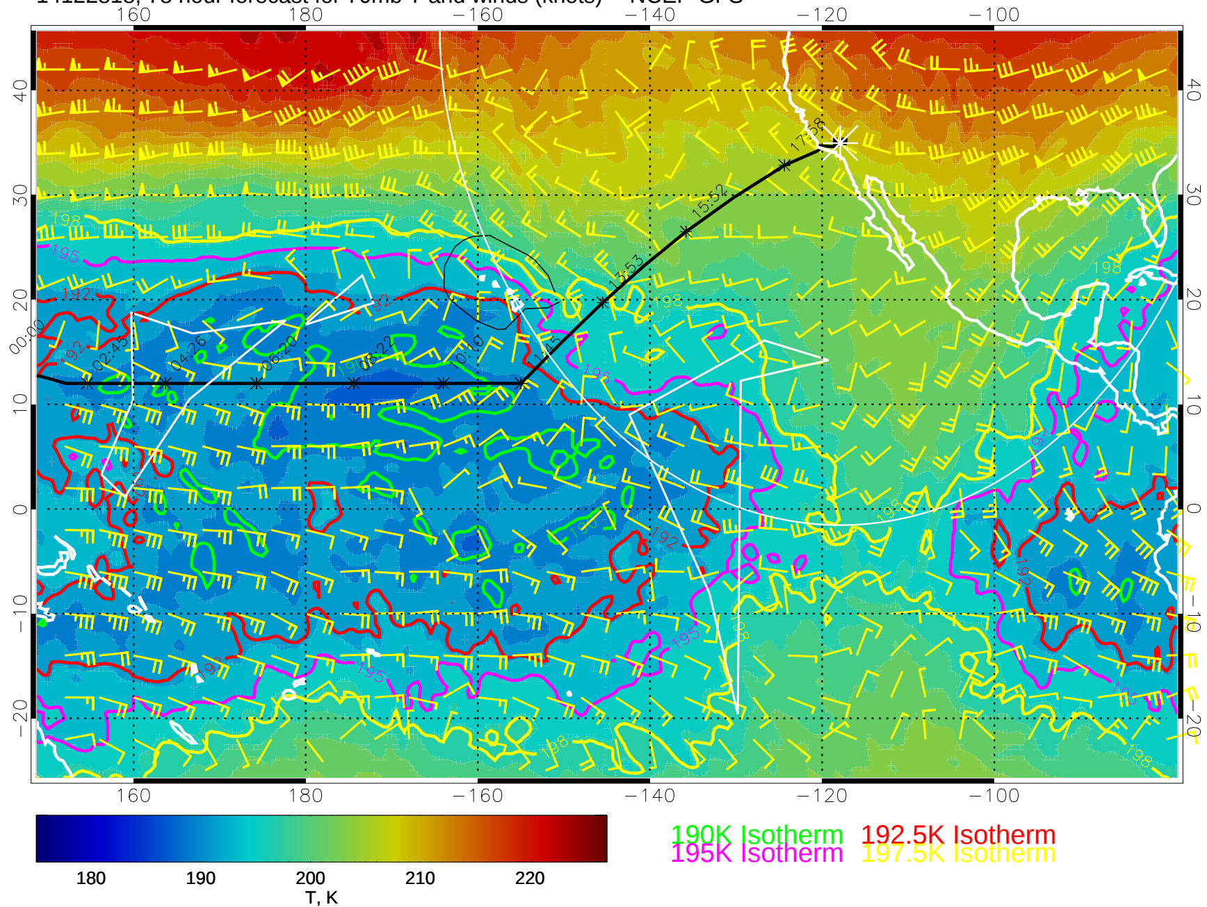
14122818, 78 hour forecast for 70mb T and winds (knots) -- NCEP GFS
