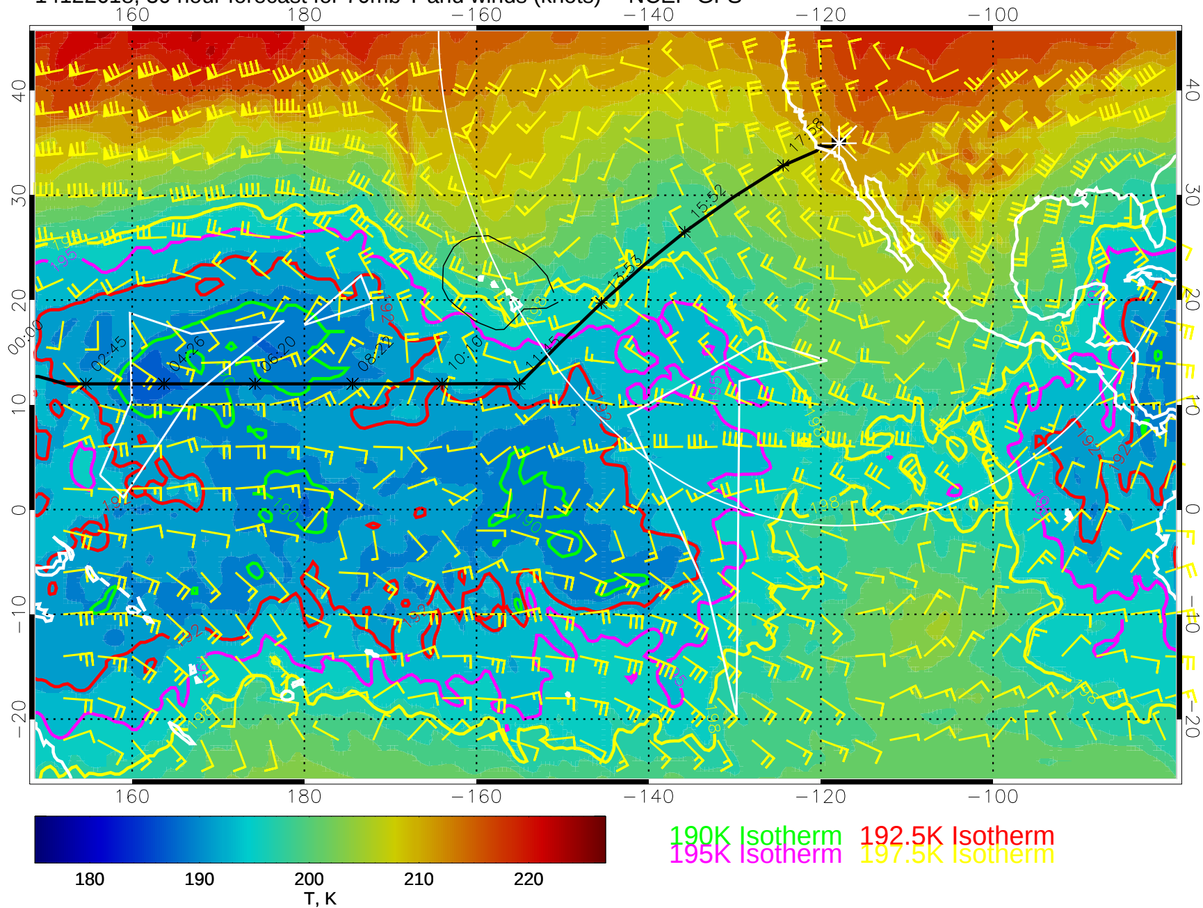
14122618, 30 hour forecast for 70mb T and winds (knots) -- NCEP GFS
