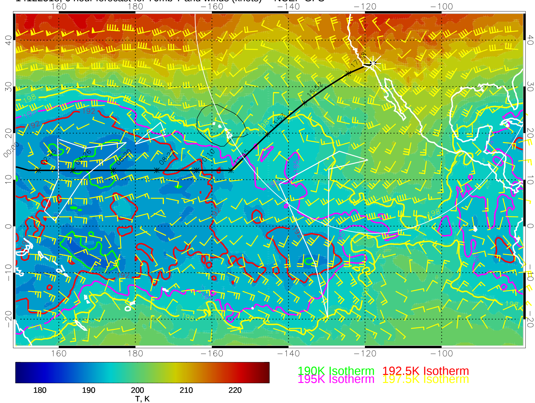
14122518, 6 hour forecast for 70mb T and winds (knots) -- NCEP GFS
