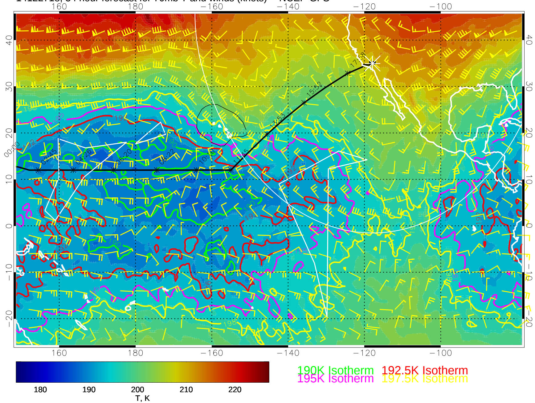
14122718, 54 hour forecast for 70mb T and winds (knots) -- NCEP GFS
