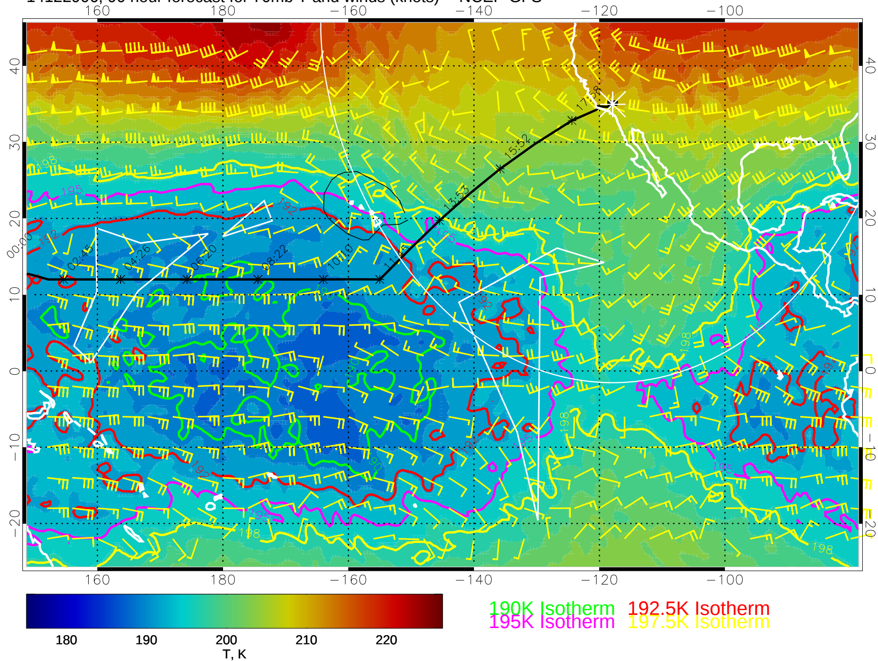
14122906, 90 hour forecast for 70mb T and winds (knots) -- NCEP GFS
