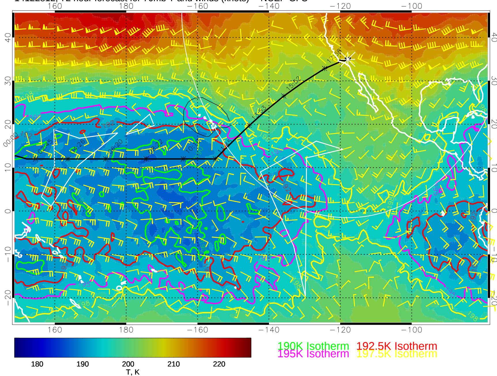
14122812, 72 hour forecast for 70mb T and winds (knots) -- NCEP GFS
