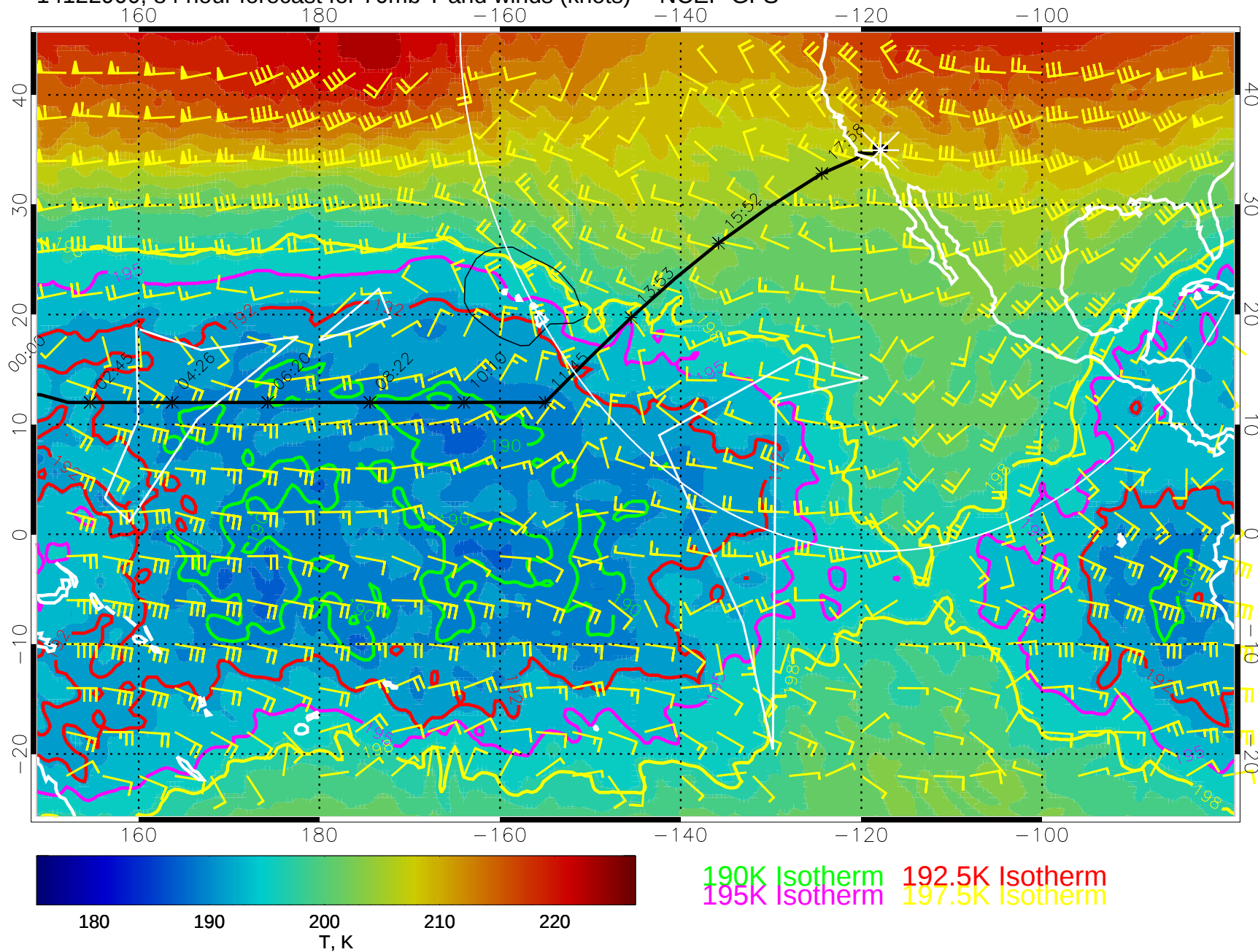
14122900, 84 hour forecast for 70mb T and winds (knots) -- NCEP GFS
