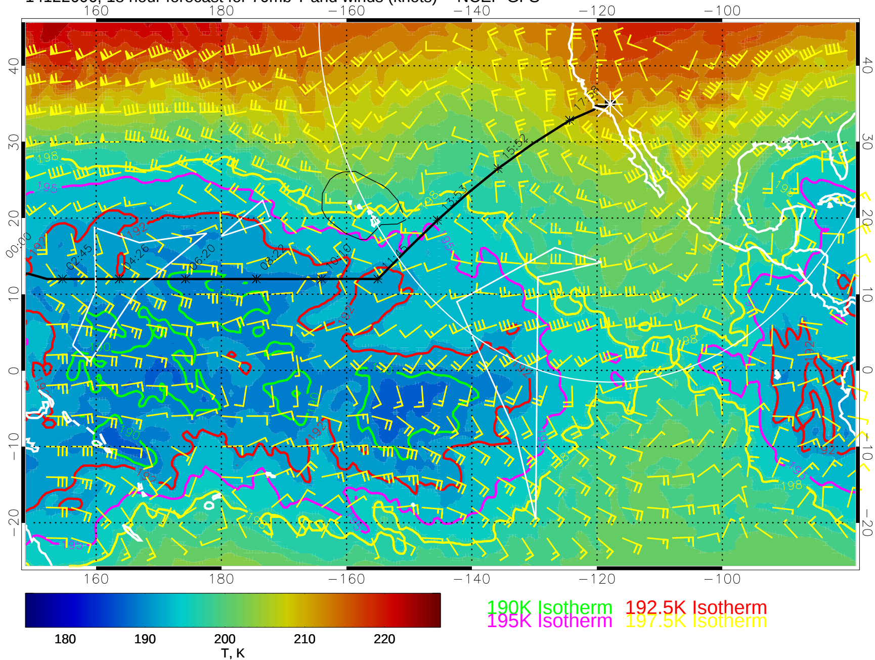
14122606, 18 hour forecast for 70mb T and winds (knots) -- NCEP GFS
