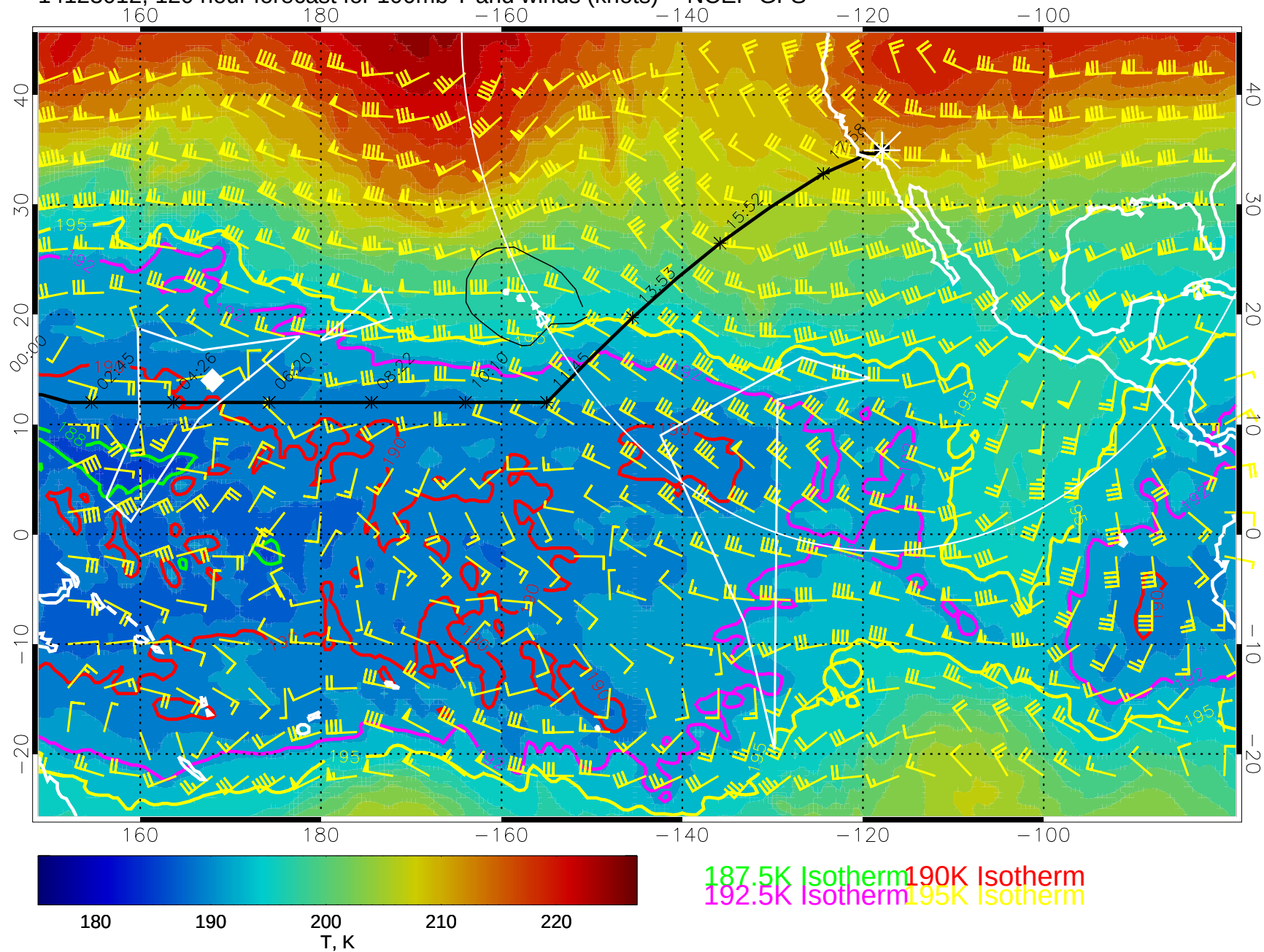
14123012, 120 hour forecast for 100mb T and winds (knots) -- NCEP GFS
