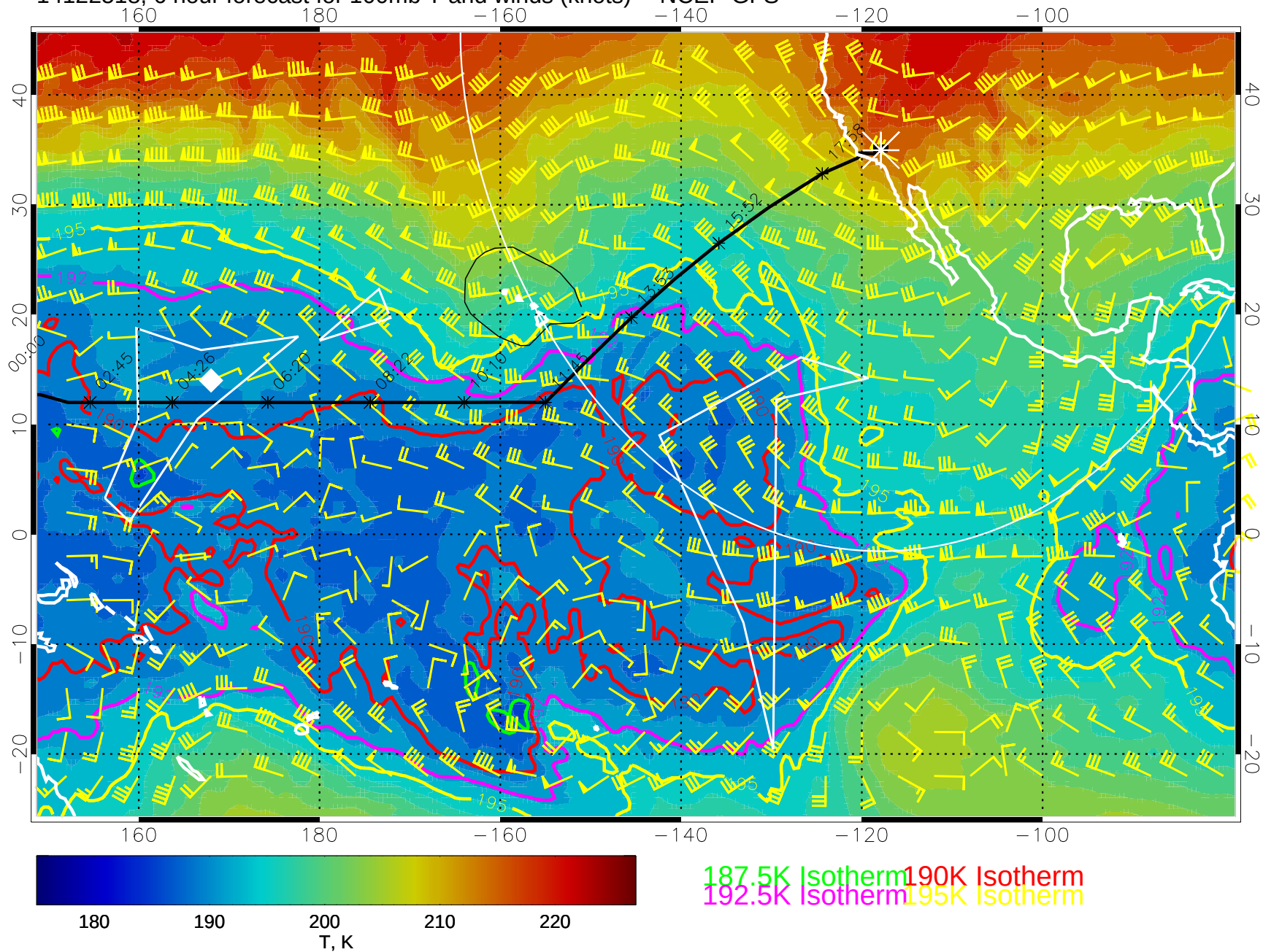
14122518, 6 hour forecast for 100mb T and winds (knots) -- NCEP GFS
