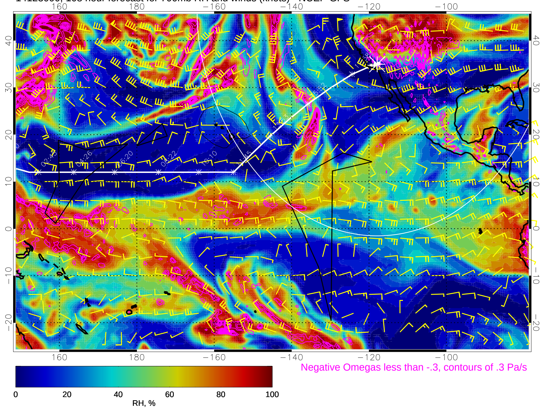
14123000, 108 hour forecast for 700mb RH and winds (knots) - NCEP GFS
