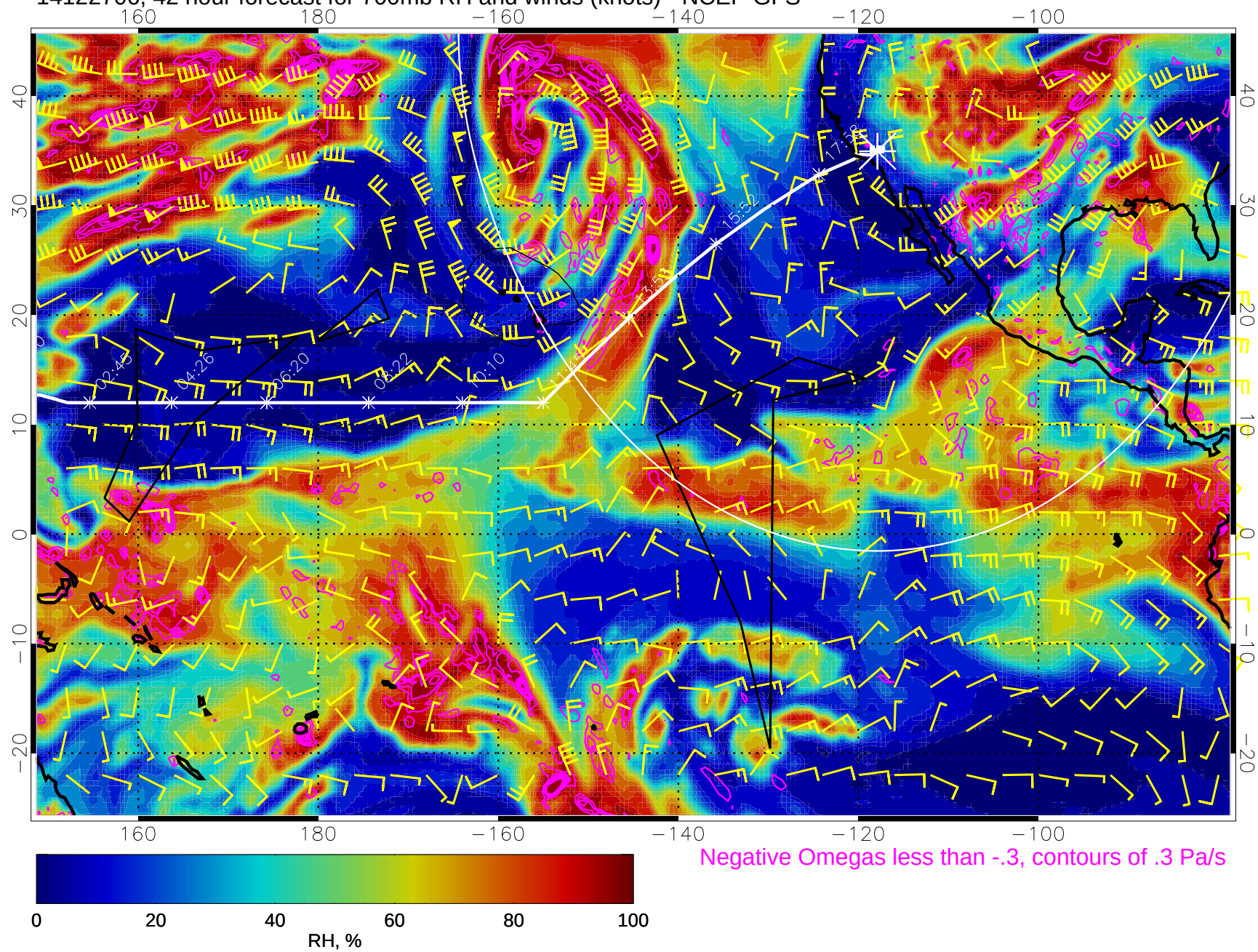
14122706, 42 hour forecast for 700mb RH and winds (knots) - NCEP GFS
