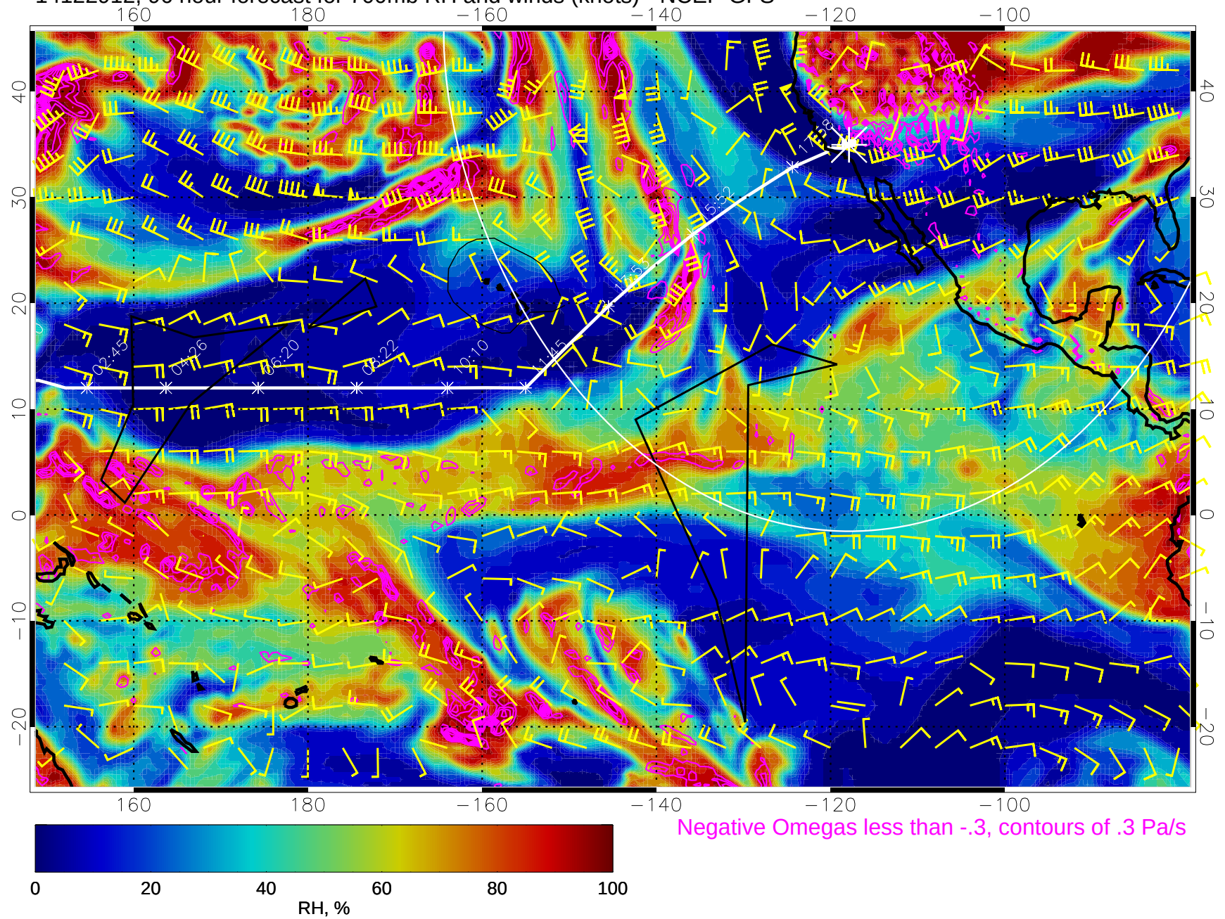
14122912, 96 hour forecast for 700mb RH and winds (knots) - NCEP GFS
