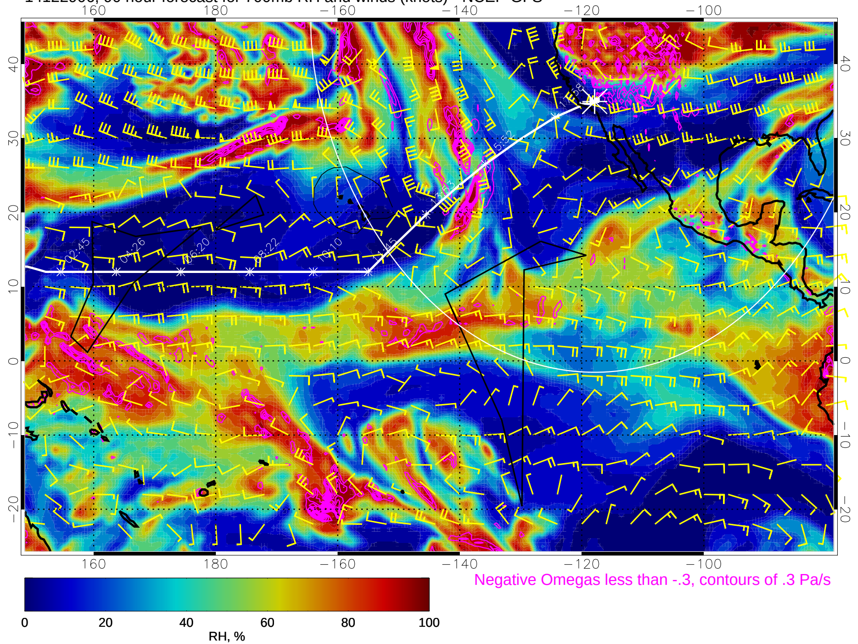
14122906, 90 hour forecast for 700mb RH and winds (knots) - NCEP GFS
