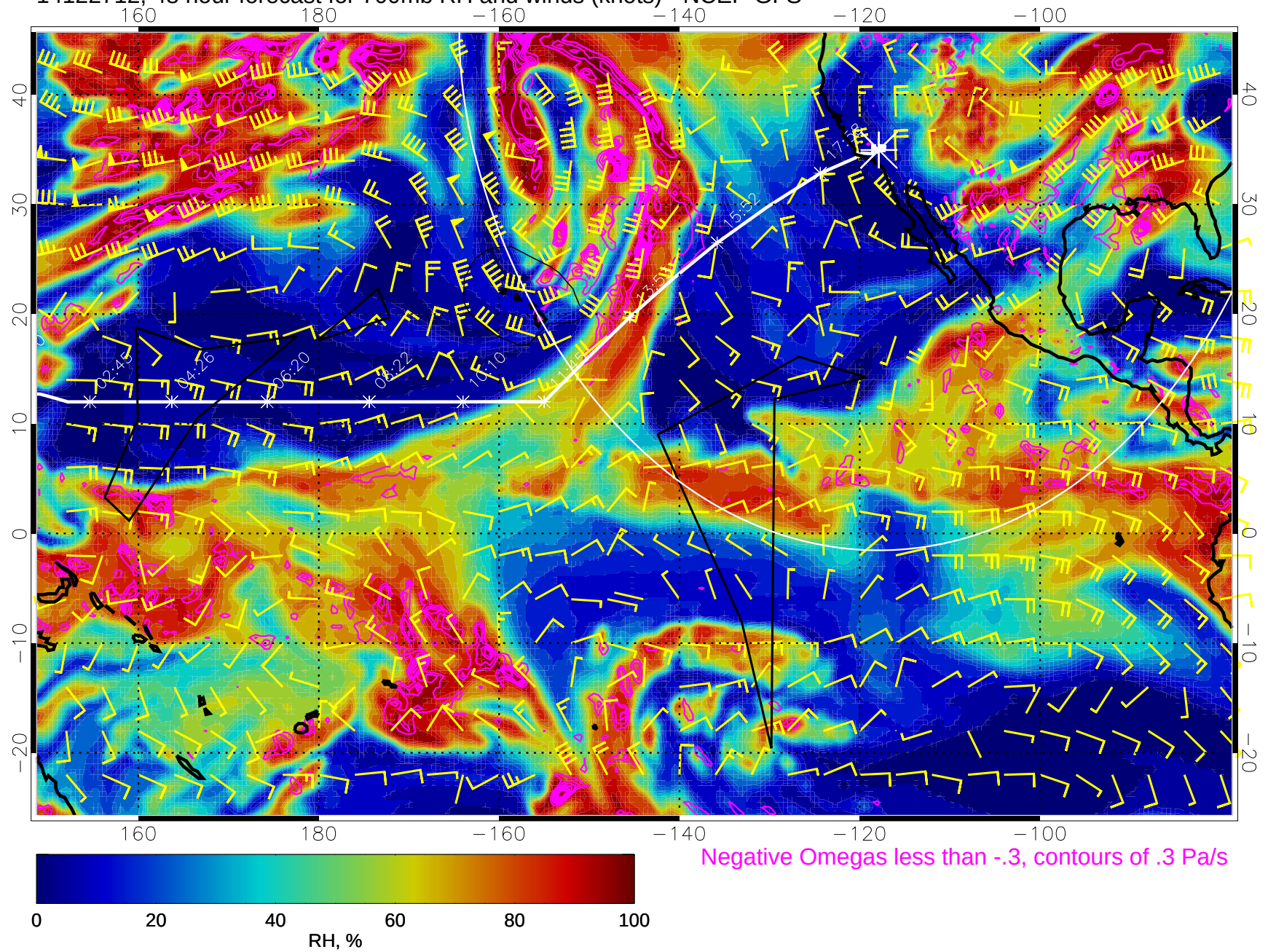
14122712, 48 hour forecast for 700mb RH and winds (knots) - NCEP GFS
