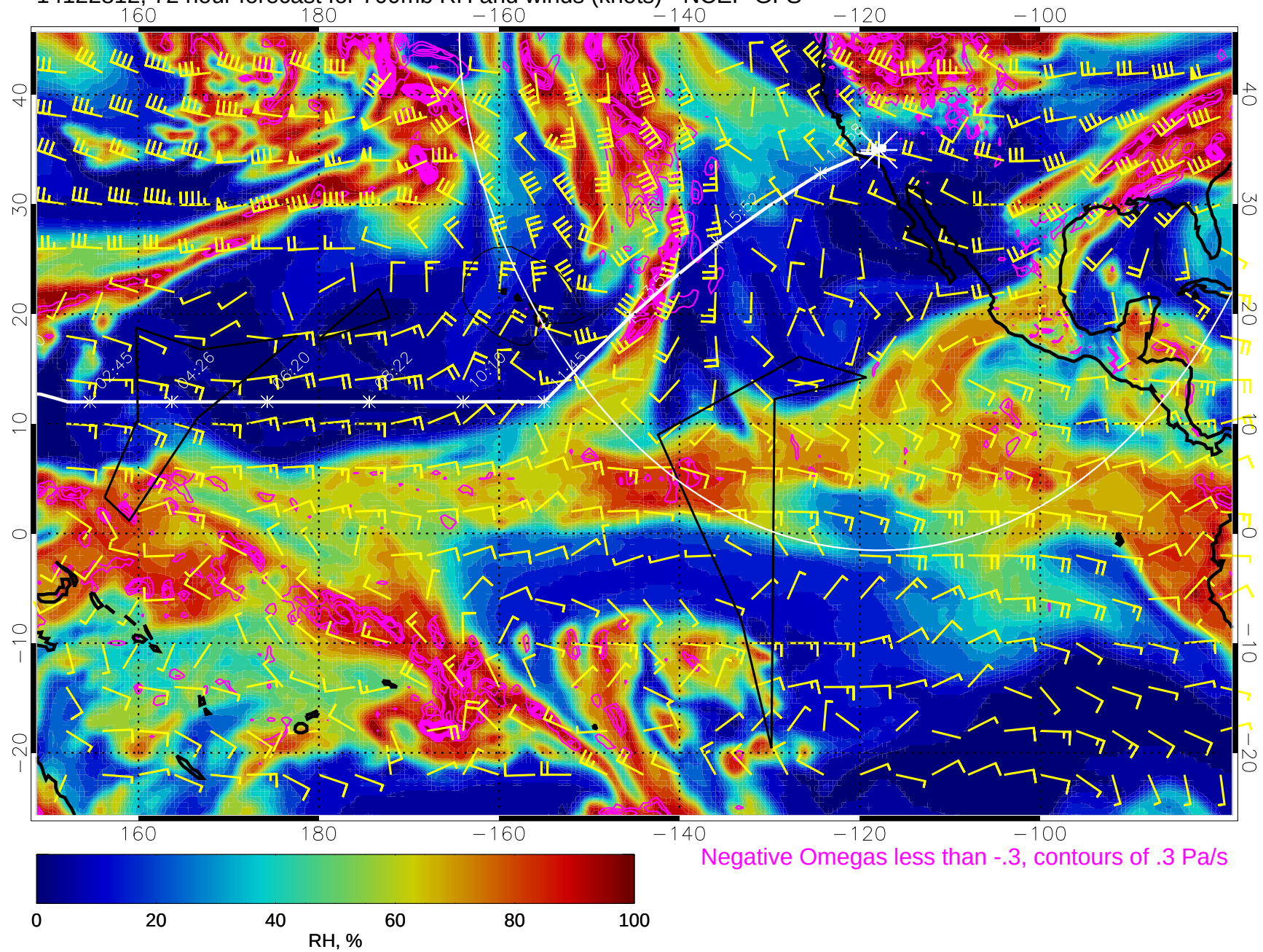
14122812, 72 hour forecast for 700mb RH and winds (knots) - NCEP GFS
