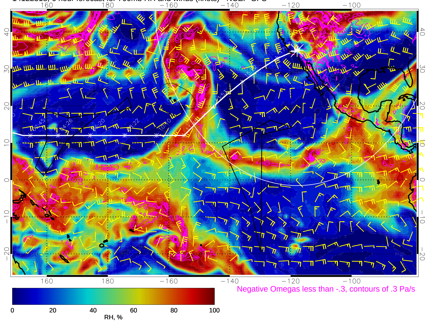
14122518, 6 hour forecast for 700mb RH and winds (knots) - NCEP GFS
