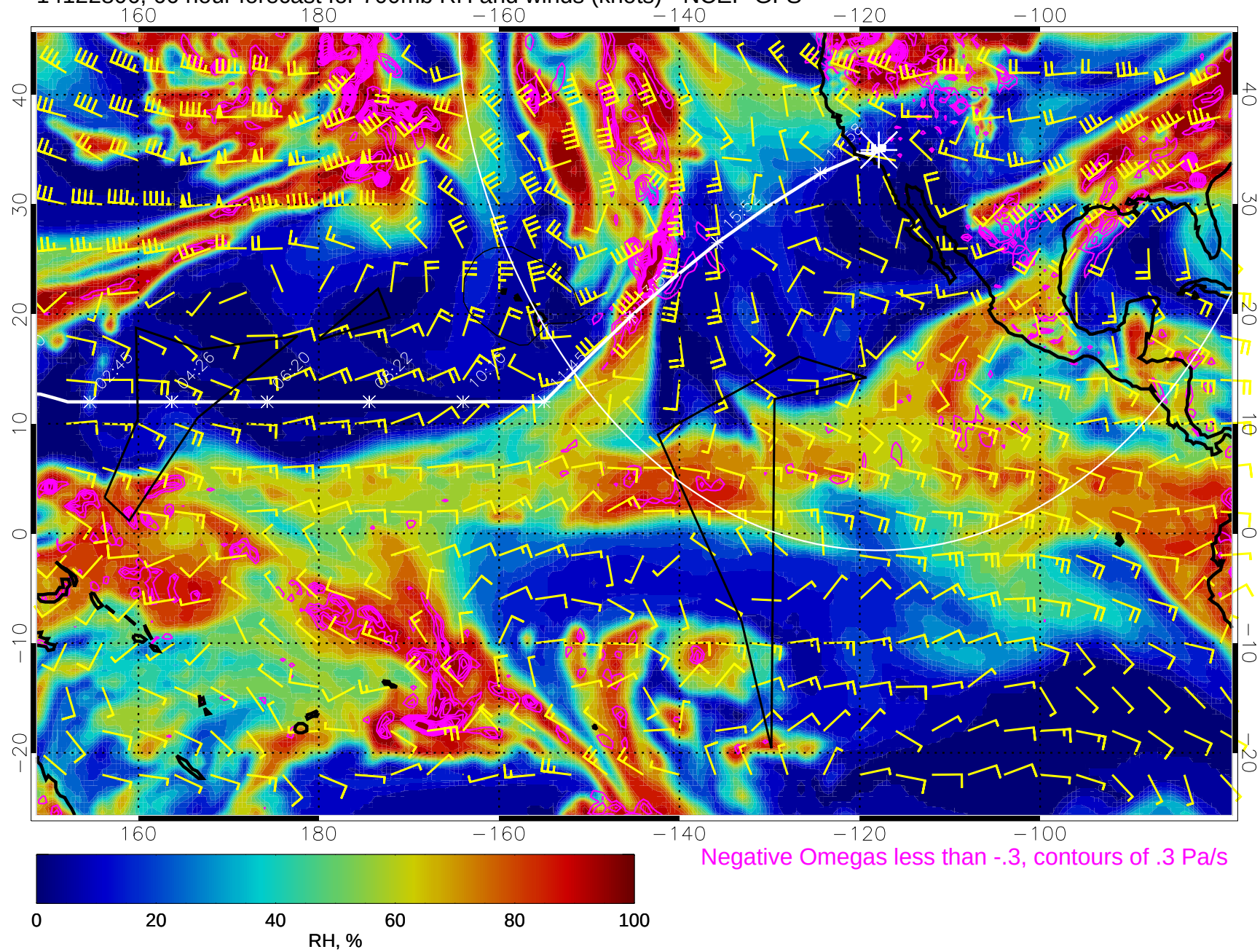
14122806, 66 hour forecast for 700mb RH and winds (knots) - NCEP GFS
