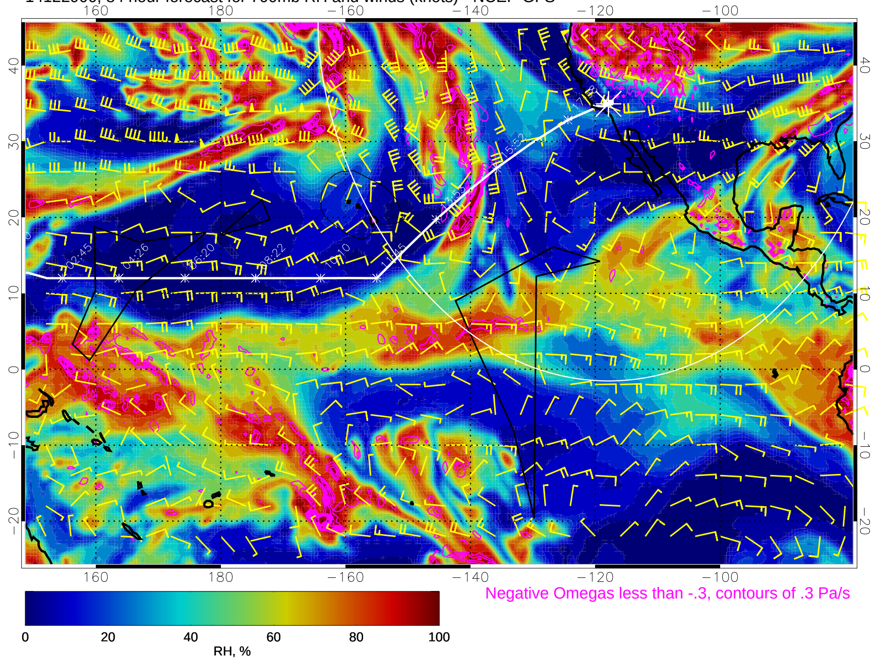
14122900, 84 hour forecast for 700mb RH and winds (knots) - NCEP GFS
