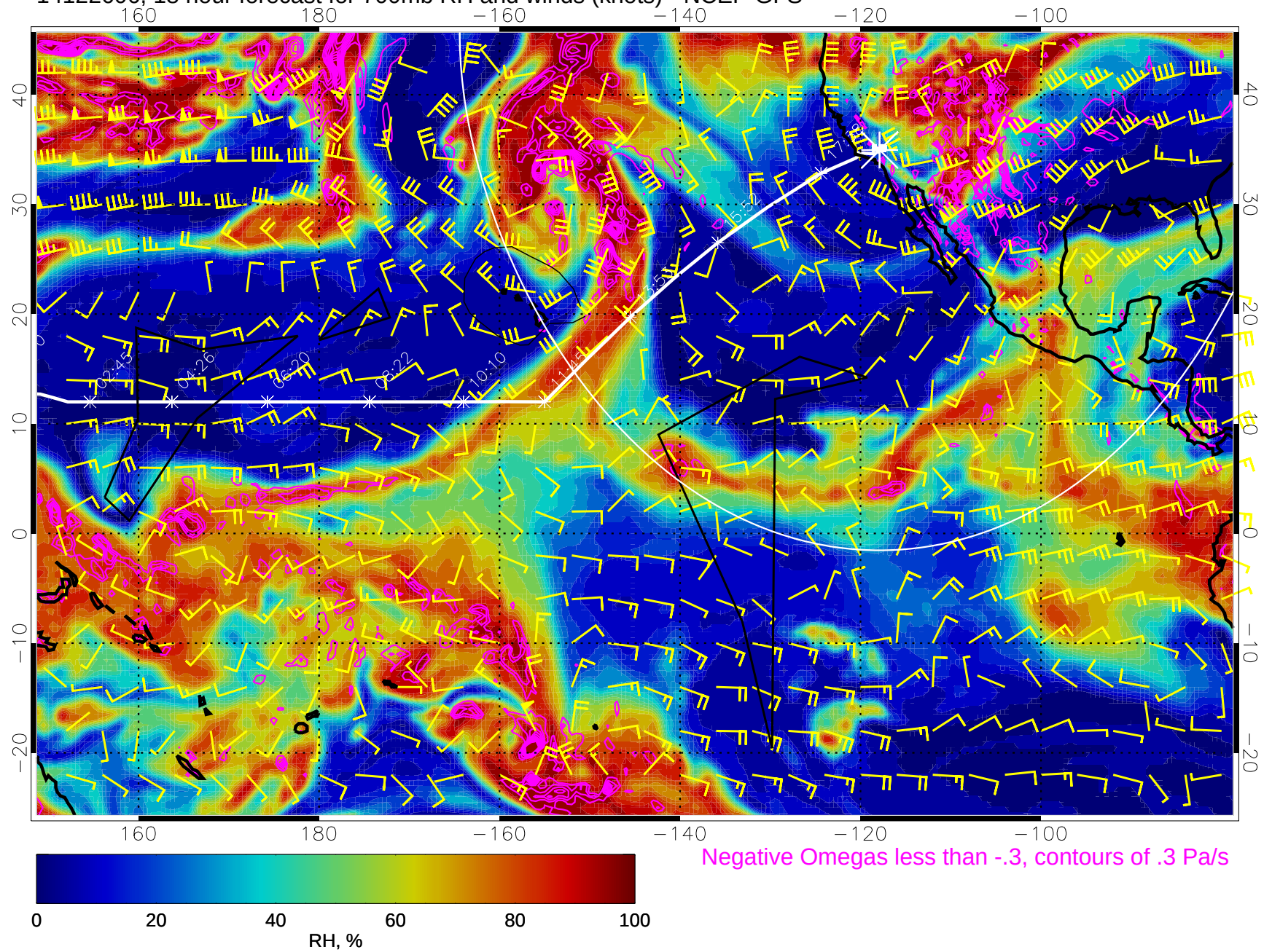
14122606, 18 hour forecast for 700mb RH and winds (knots) - NCEP GFS
