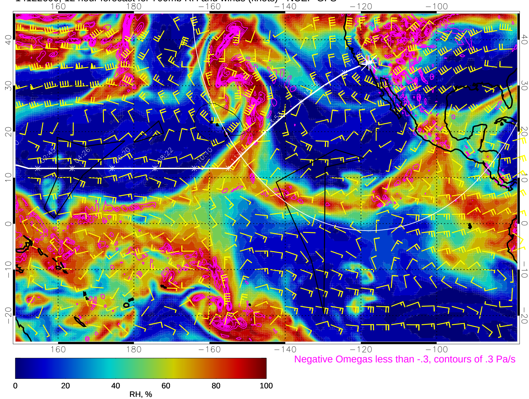
14122600, 12 hour forecast for 700mb RH and winds (knots) - NCEP GFS
