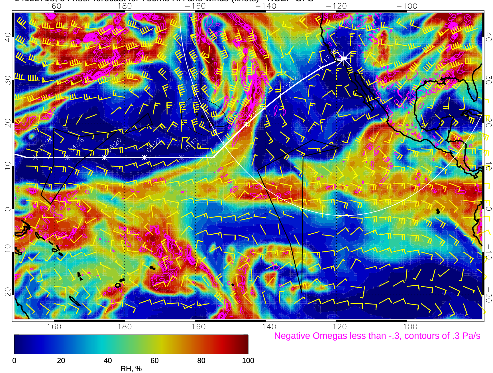
14122718, 54 hour forecast for 700mb RH and winds (knots) - NCEP GFS
