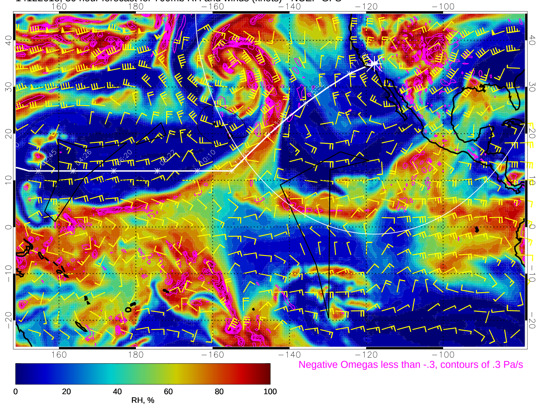
14122618, 30 hour forecast for 700mb RH and winds (knots) - NCEP GFS
