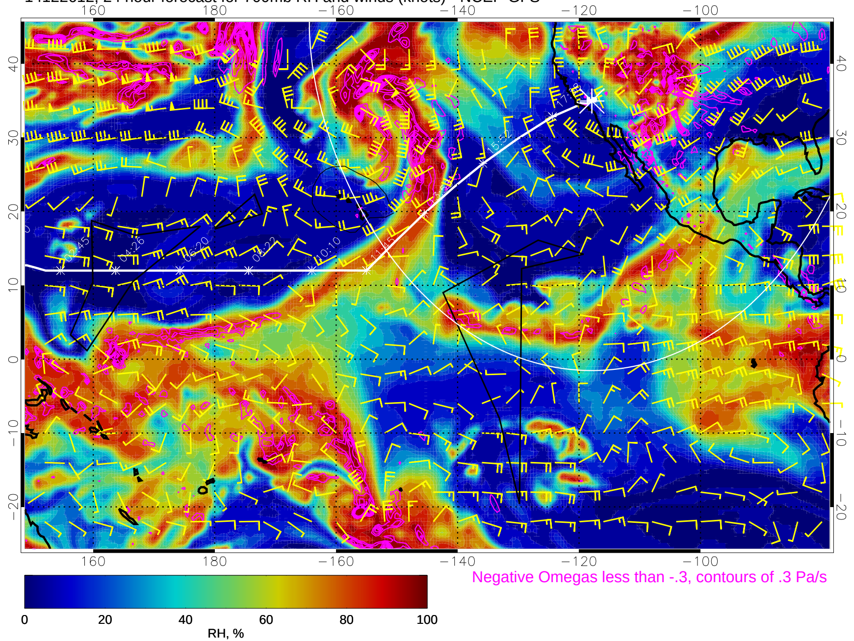
14122612, 24 hour forecast for 700mb RH and winds (knots) - NCEP GFS
