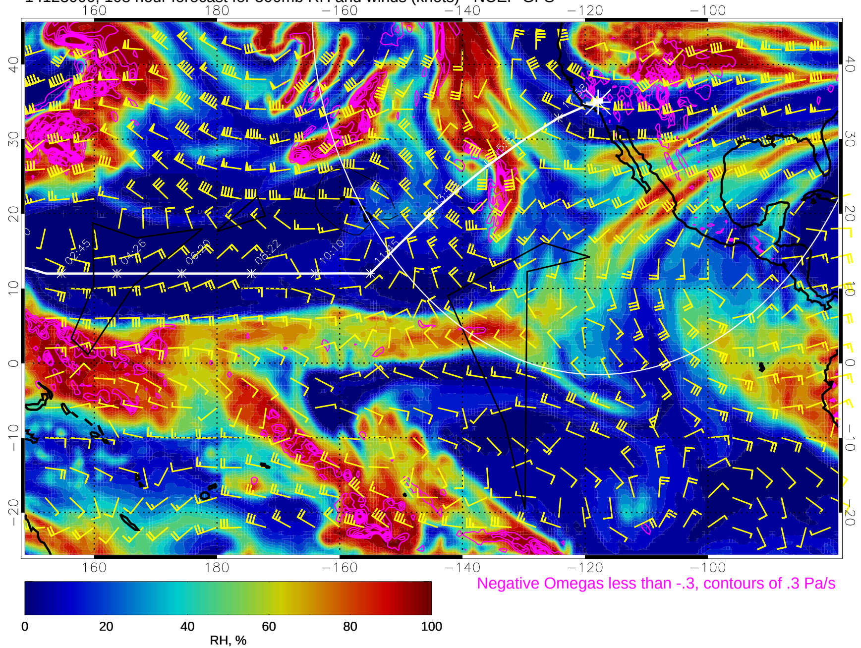
14123000, 108 hour forecast for 500mb RH and winds (knots) - NCEP GFS
