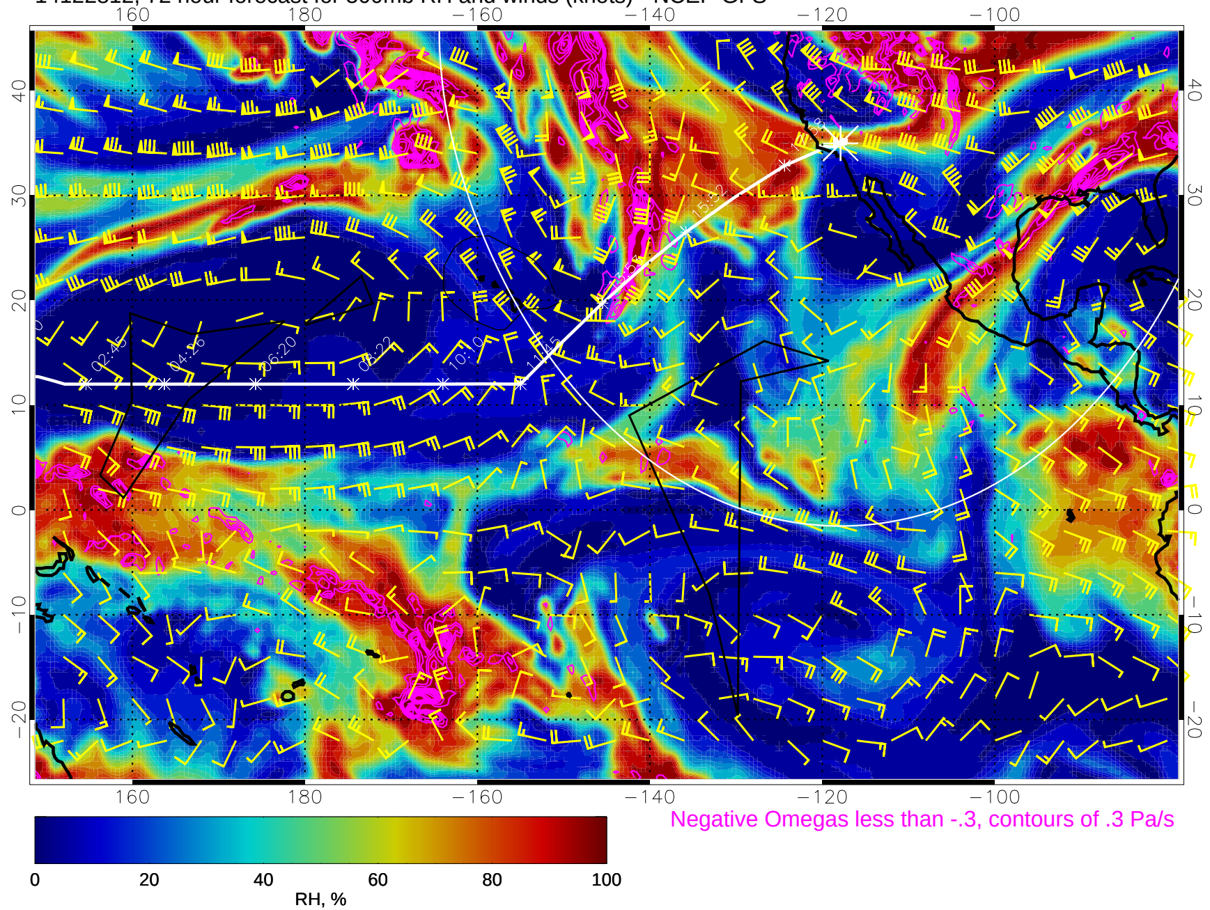
14122812, 72 hour forecast for 500mb RH and winds (knots) - NCEP GFS
