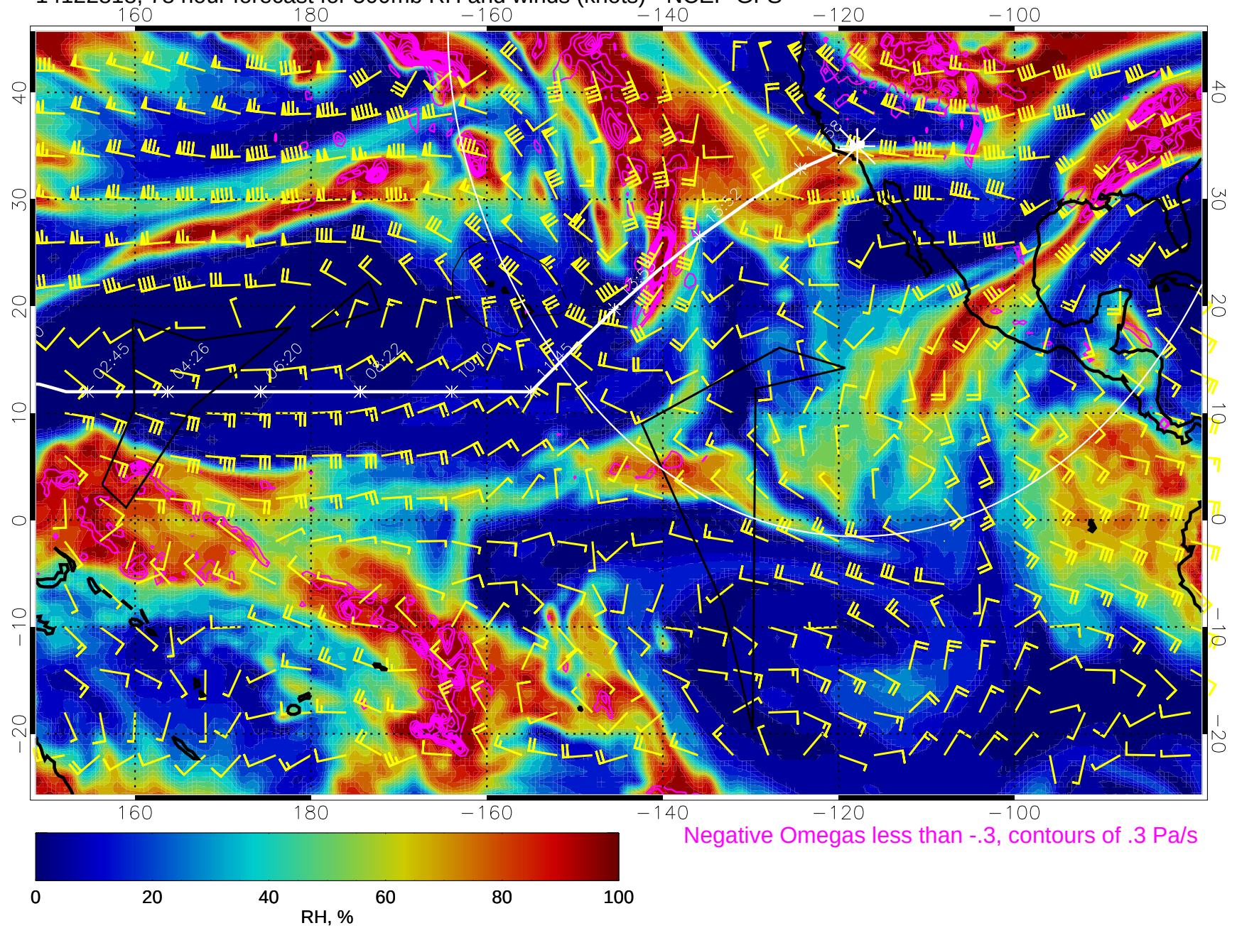
14122818, 78 hour forecast for 500mb RH and winds (knots) - NCEP GFS
