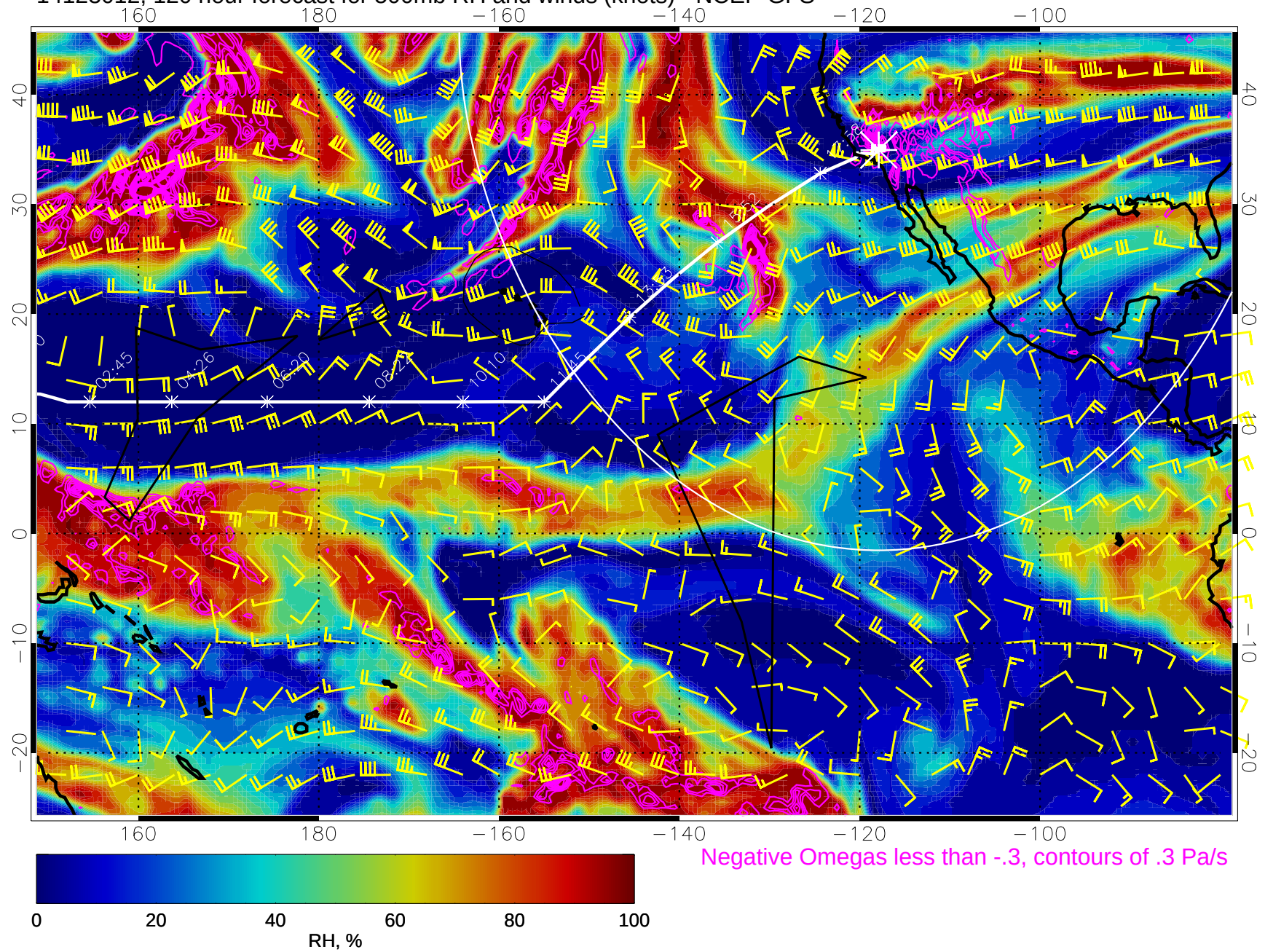
14123012, 120 hour forecast for 500mb RH and winds (knots) - NCEP GFS
