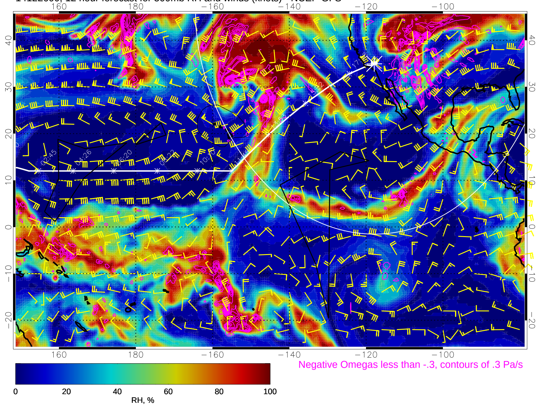
14122600, 12 hour forecast for 500mb RH and winds (knots) - NCEP GFS
