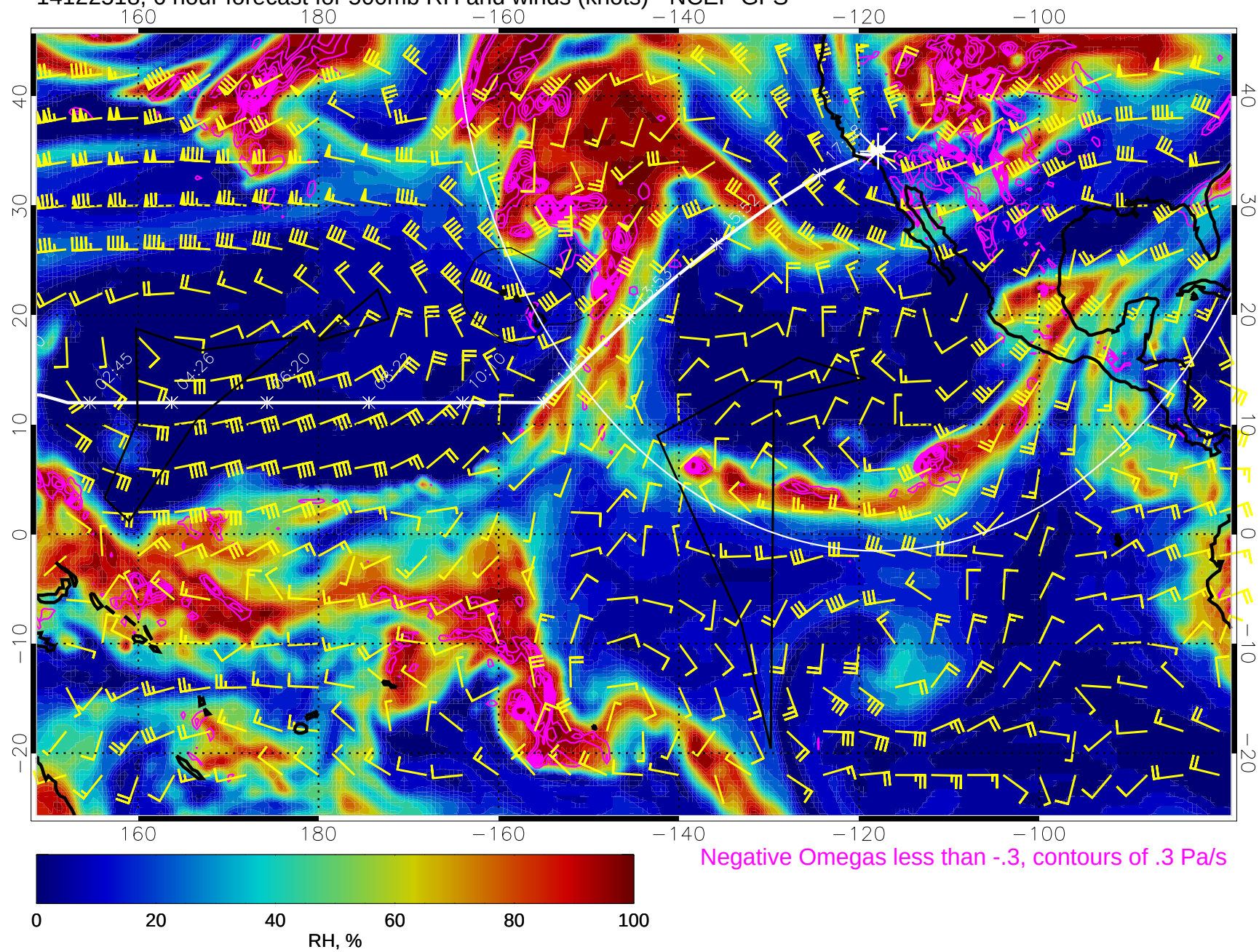
14122518, 6 hour forecast for 500mb RH and winds (knots) - NCEP GFS
