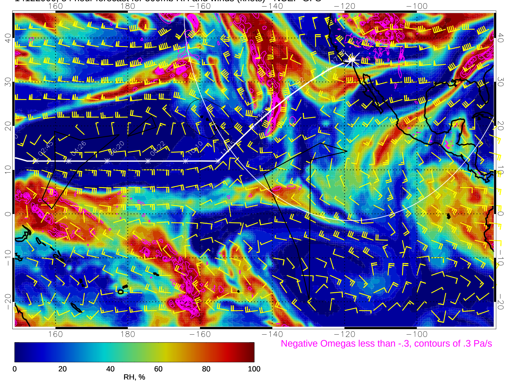
14122900, 84 hour forecast for 500mb RH and winds (knots) - NCEP GFS
