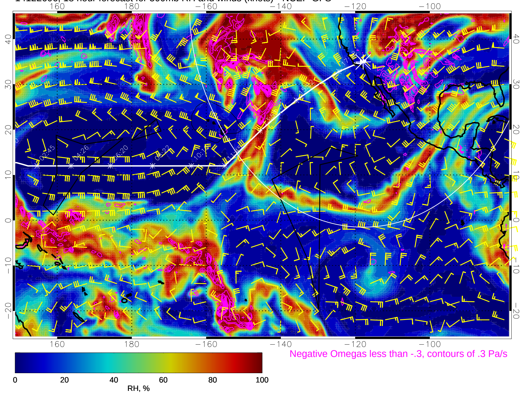
14122606, 18 hour forecast for 500mb RH and winds (knots) - NCEP GFS
