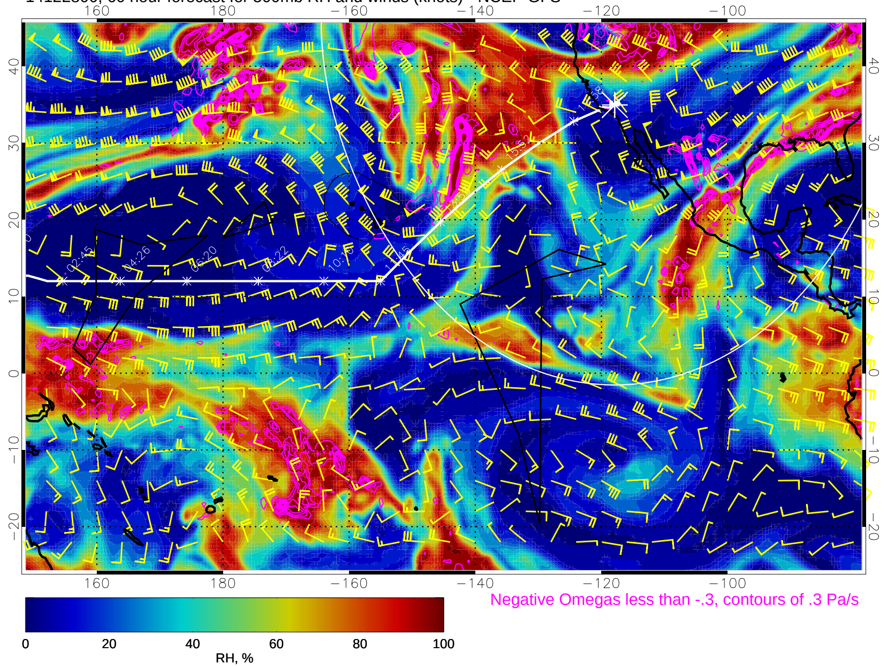
14122800, 60 hour forecast for 500mb RH and winds (knots) - NCEP GFS
