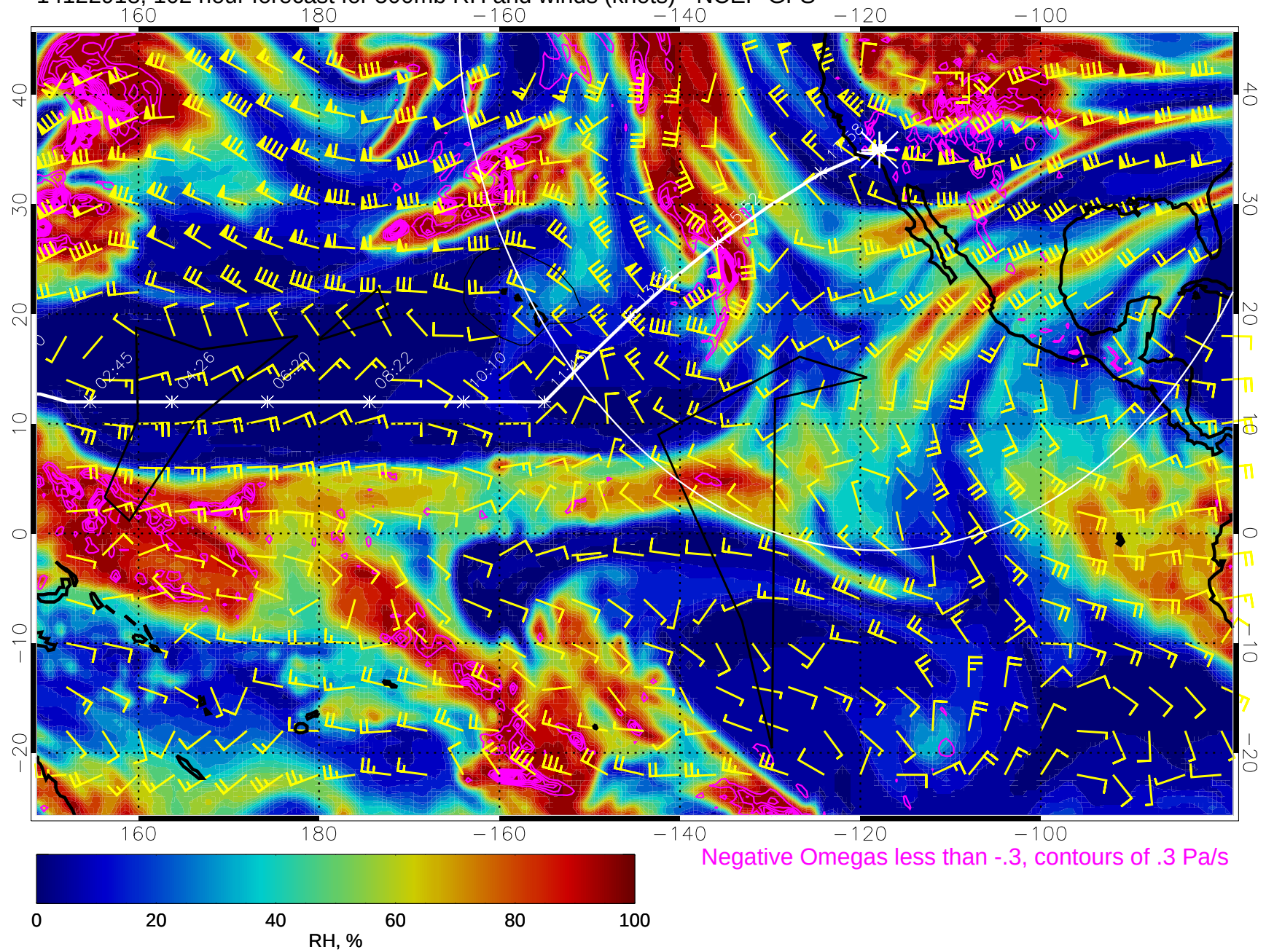
14122918, 102 hour forecast for 500mb RH and winds (knots) - NCEP GFS
