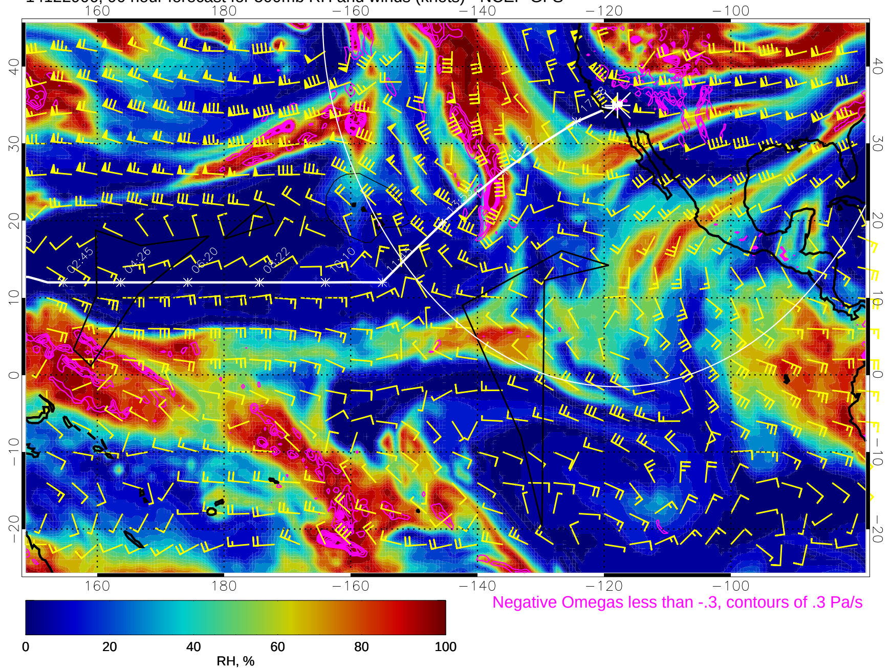
14122906, 90 hour forecast for 500mb RH and winds (knots) - NCEP GFS
