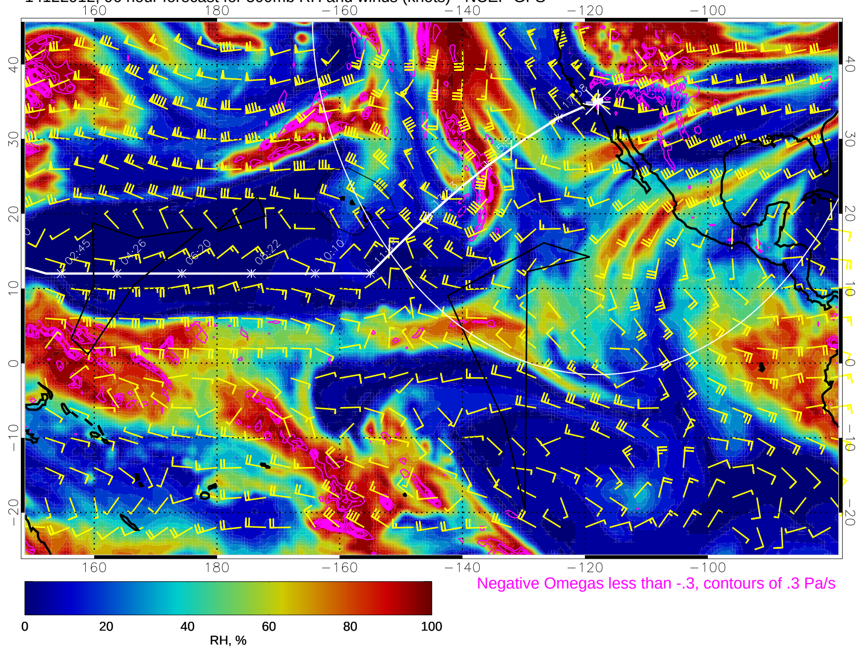
14122912, 96 hour forecast for 500mb RH and winds (knots) - NCEP GFS
