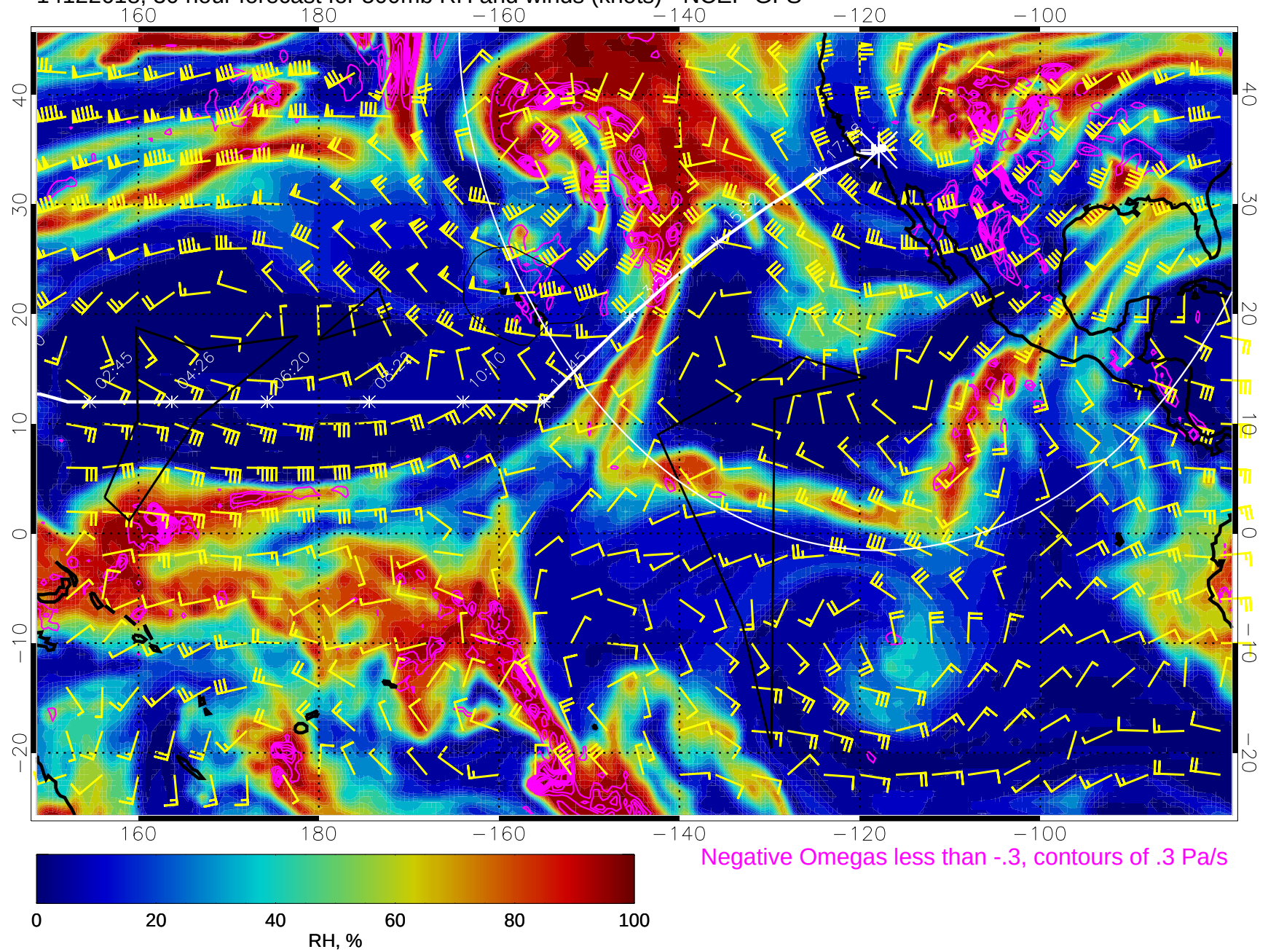
14122618, 30 hour forecast for 500mb RH and winds (knots) - NCEP GFS
