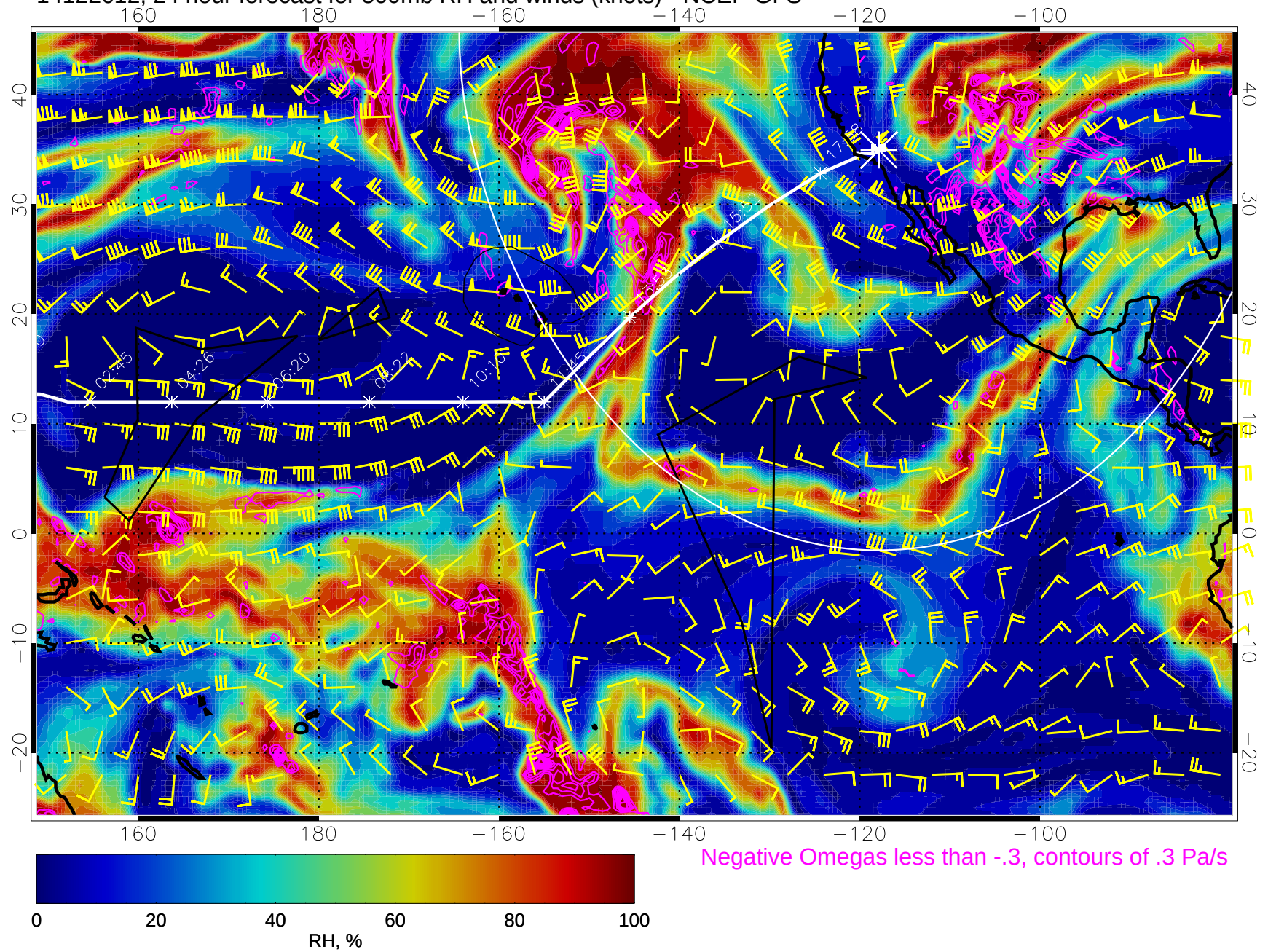
14122612, 24 hour forecast for 500mb RH and winds (knots) - NCEP GFS
