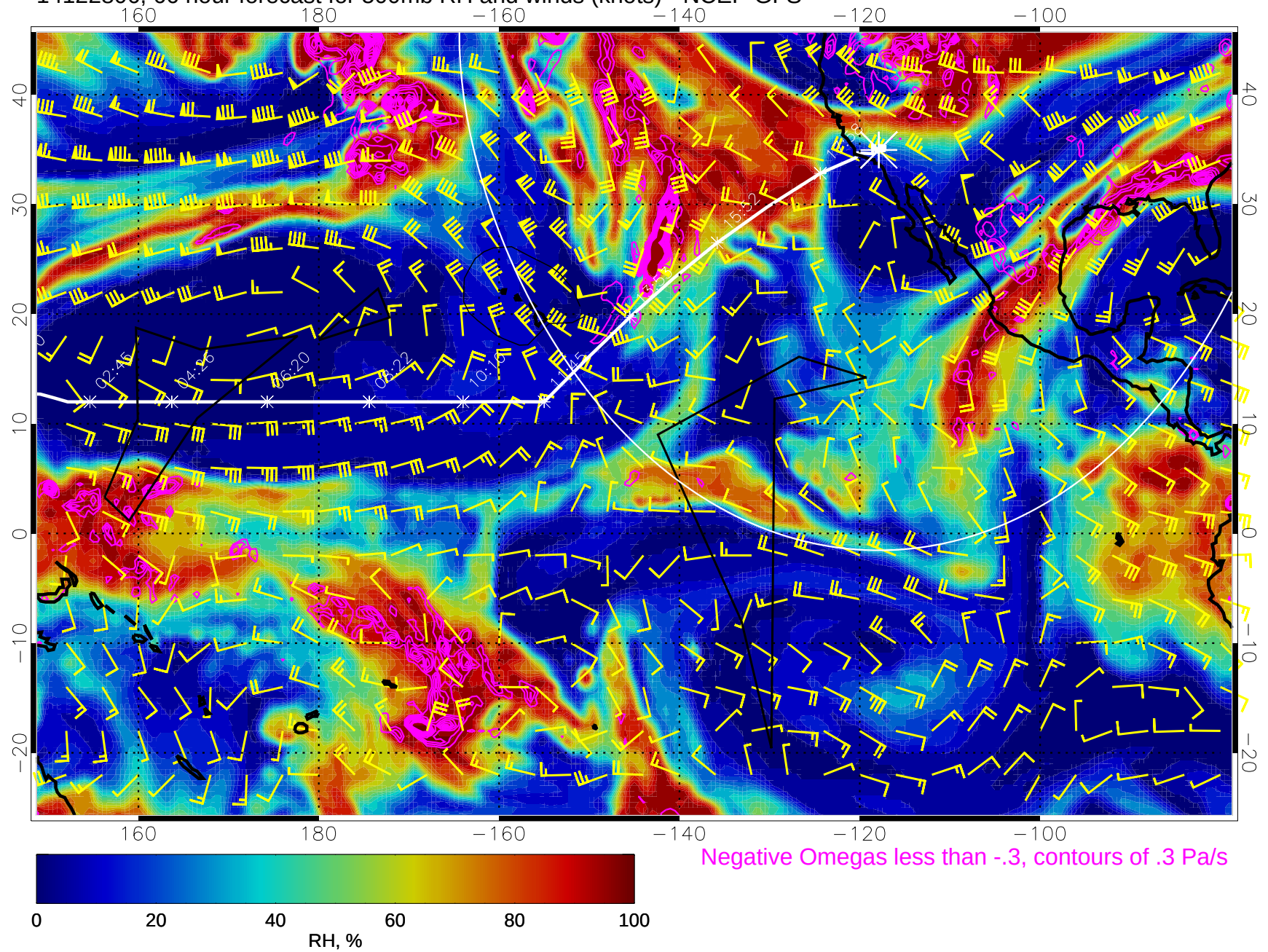
14122806, 66 hour forecast for 500mb RH and winds (knots) - NCEP GFS
