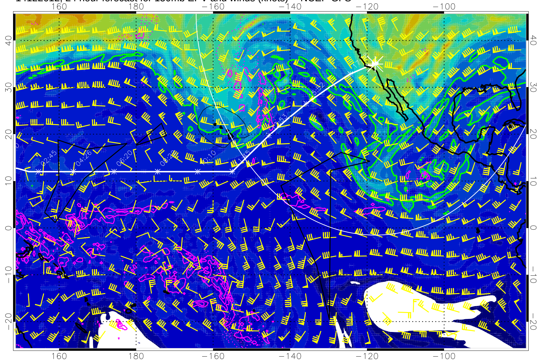
14122612, 24 hour forecast for 150mb EPV and winds (knots) -- NCEP GFS
