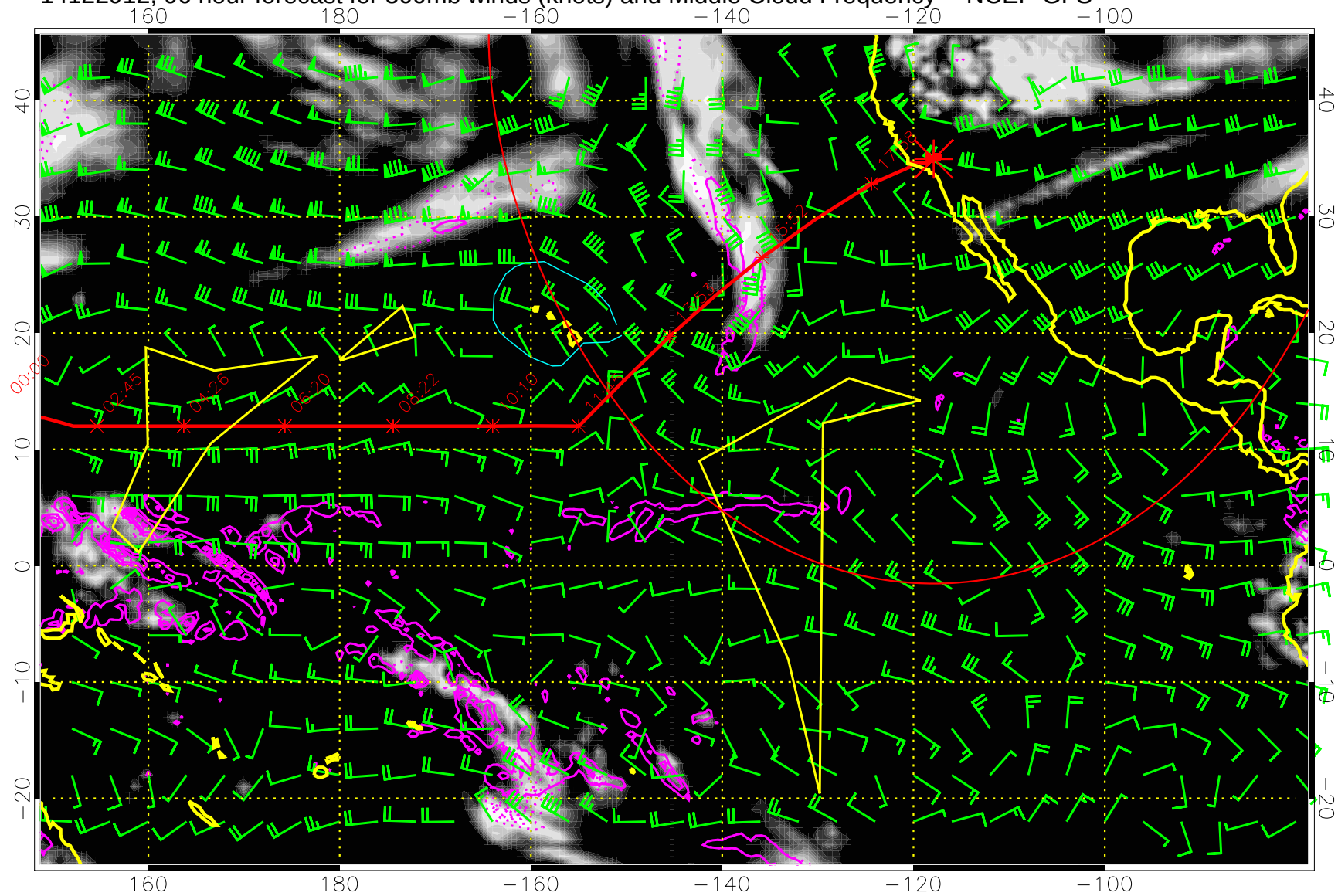
14122912, 96 hour forecast for 500mb winds (knots) and Middle Cloud Frequency -- NCEP GFS
