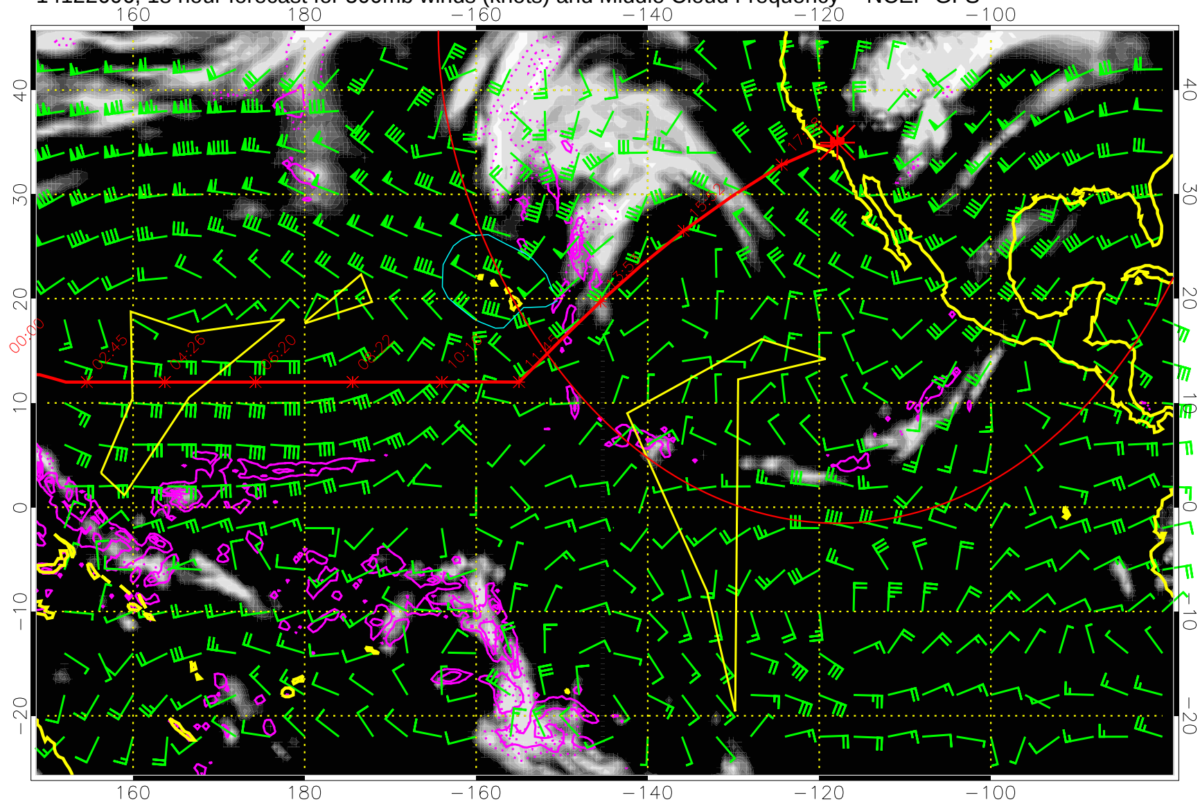
14122606, 18 hour forecast for 500mb winds (knots) and Middle Cloud Frequency -- NCEP GFS
