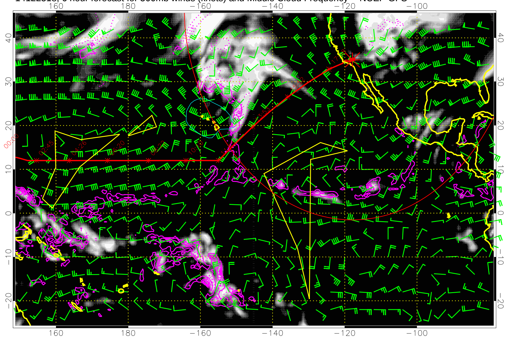
14122518, 6 hour forecast for 500mb winds (knots) and Middle Cloud Frequency -- NCEP GFS
