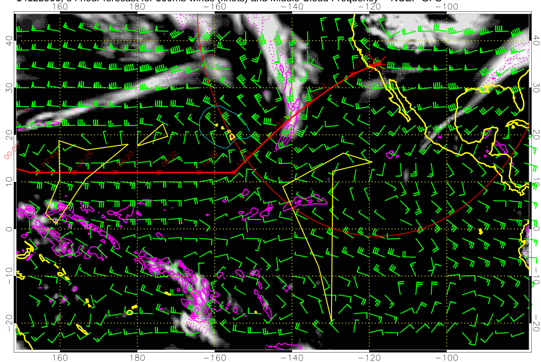
14122900, 84 hour forecast for 500mb winds (knots) and Middle Cloud Frequency -- NCEP GFS
