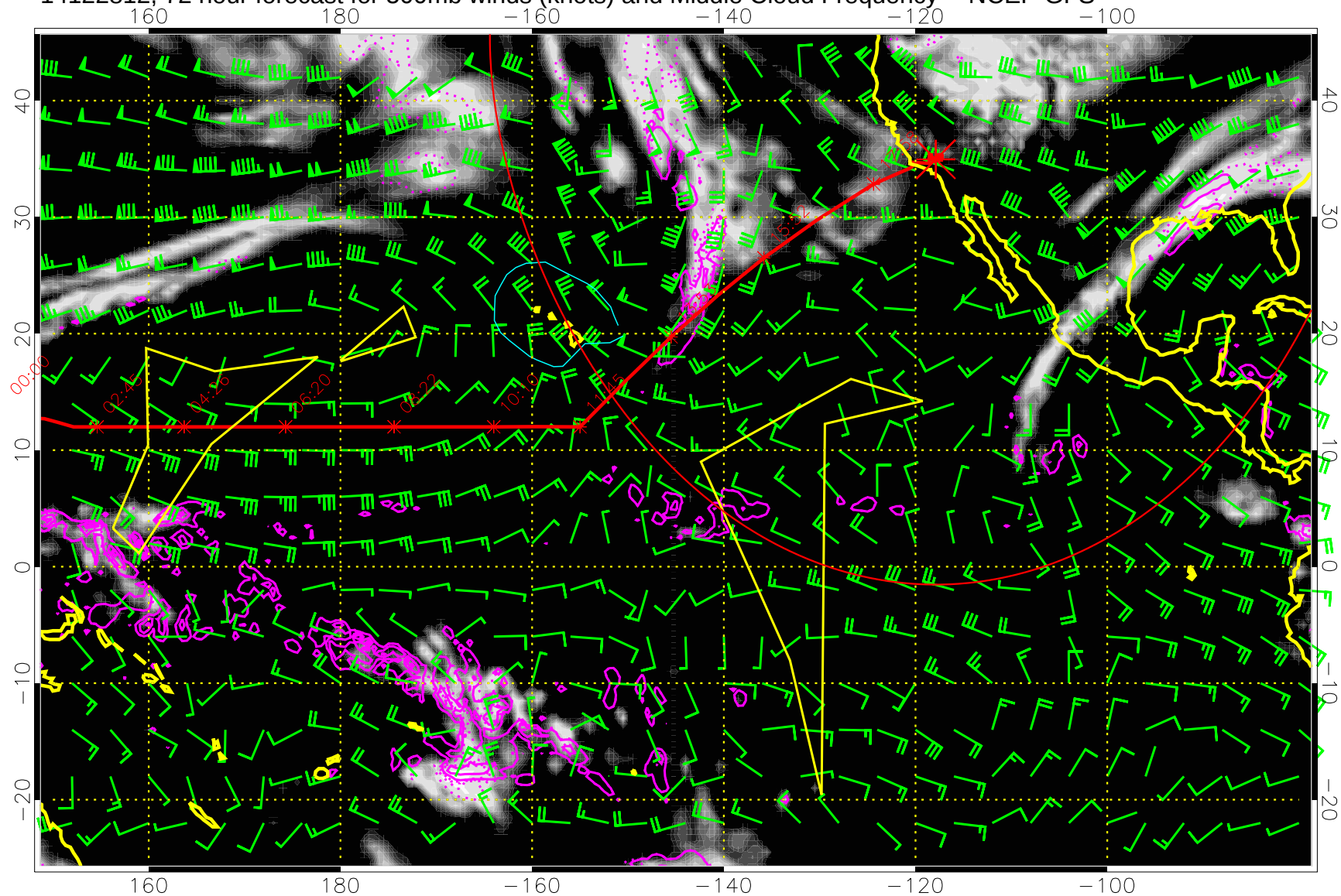
14122812, 72 hour forecast for 500mb winds (knots) and Middle Cloud Frequency -- NCEP GFS
