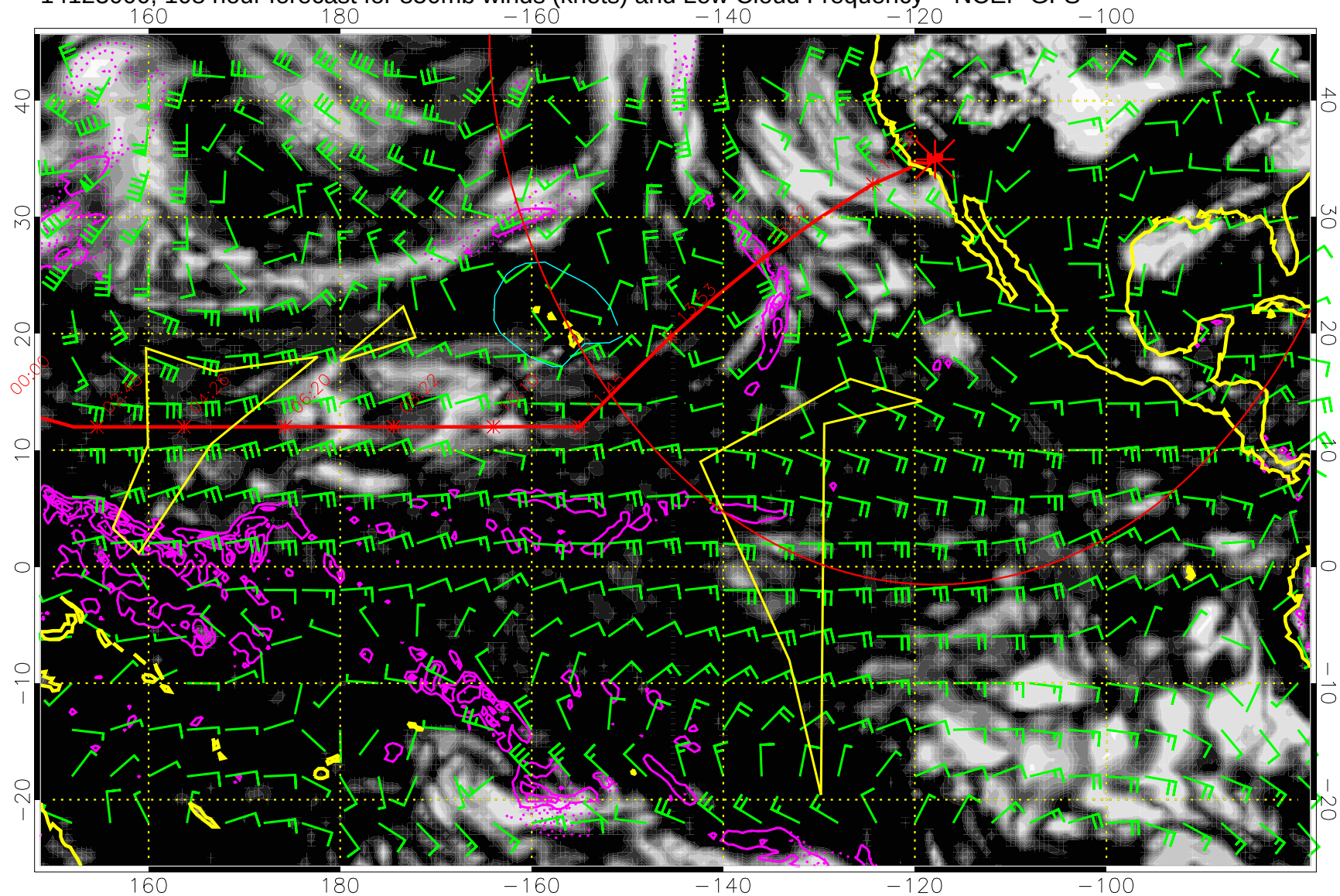
14123000, 108 hour forecast for 850mb winds (knots) and Low Cloud Frequency -- NCEP GFS
