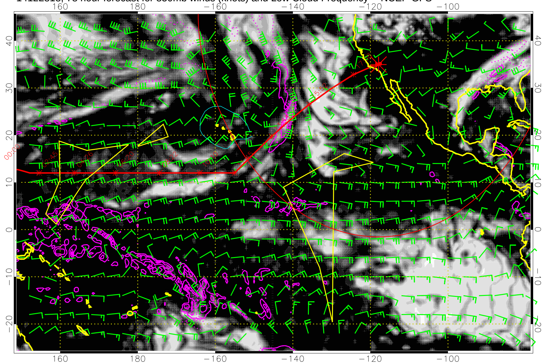
14122818, 78 hour forecast for 850mb winds (knots) and Low Cloud Frequency -- NCEP GFS
