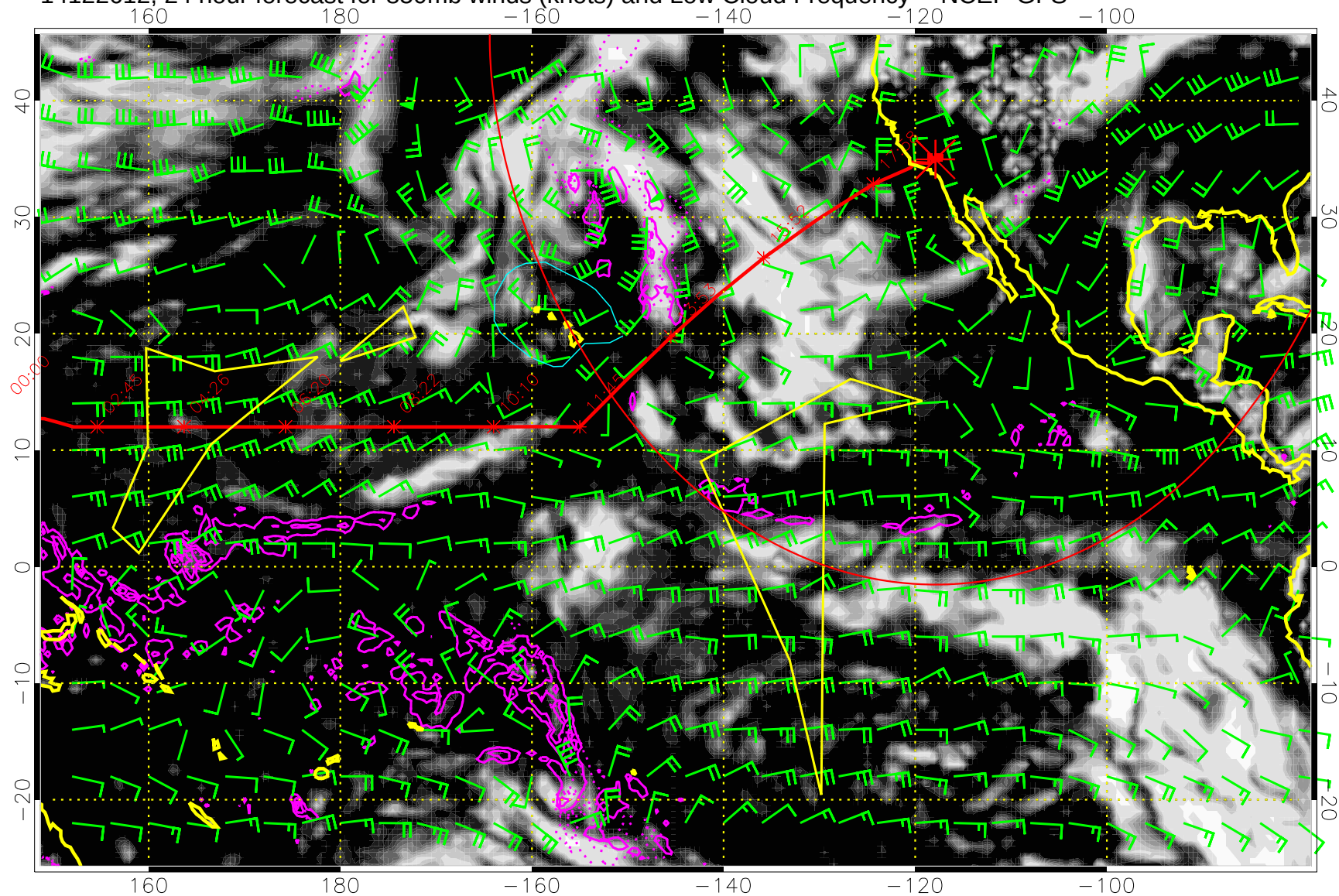
14122612, 24 hour forecast for 850mb winds (knots) and Low Cloud Frequency -- NCEP GFS
