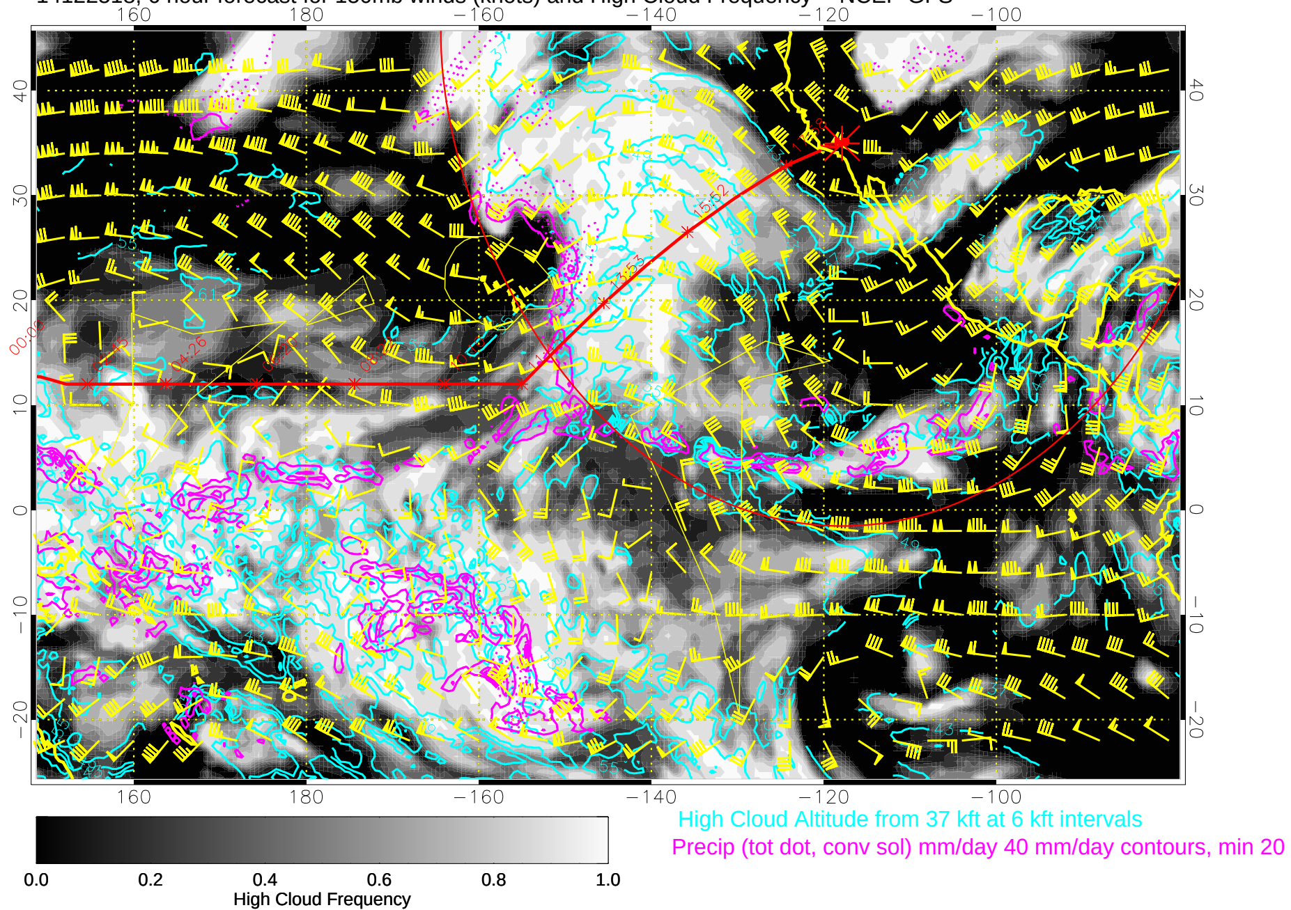
14122518, 6 hour forecast for 150mb winds (knots) and High Cloud Frequency -- NCEP GFS
