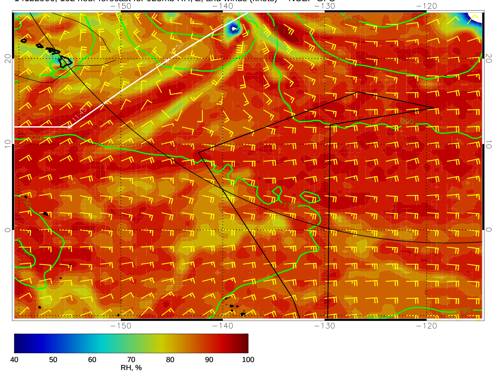
14122906, 102 hour forecast for 925mb RH, Z, and winds (knots) -- NCEP GFS
