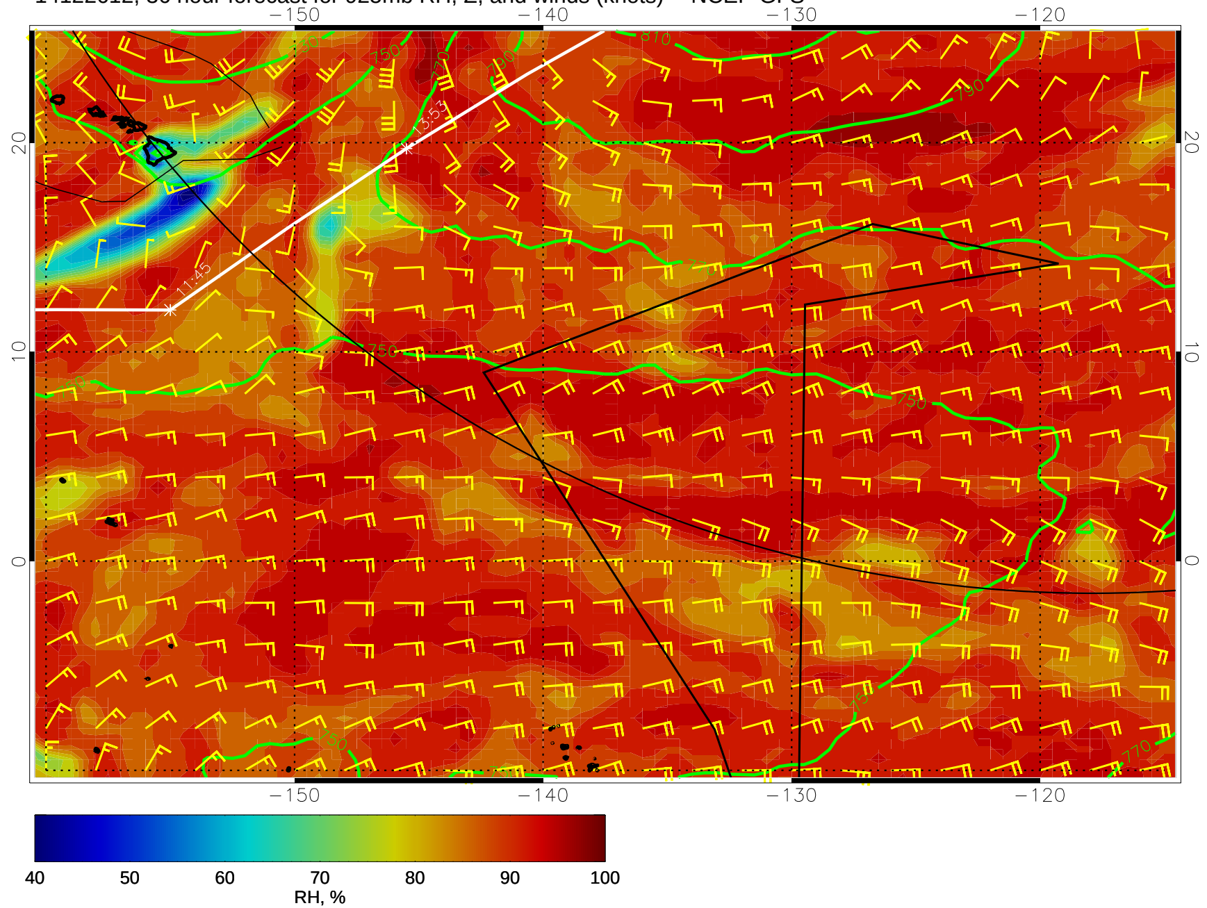
14122612, 36 hour forecast for 925mb RH, Z, and winds (knots) -- NCEP GFS
