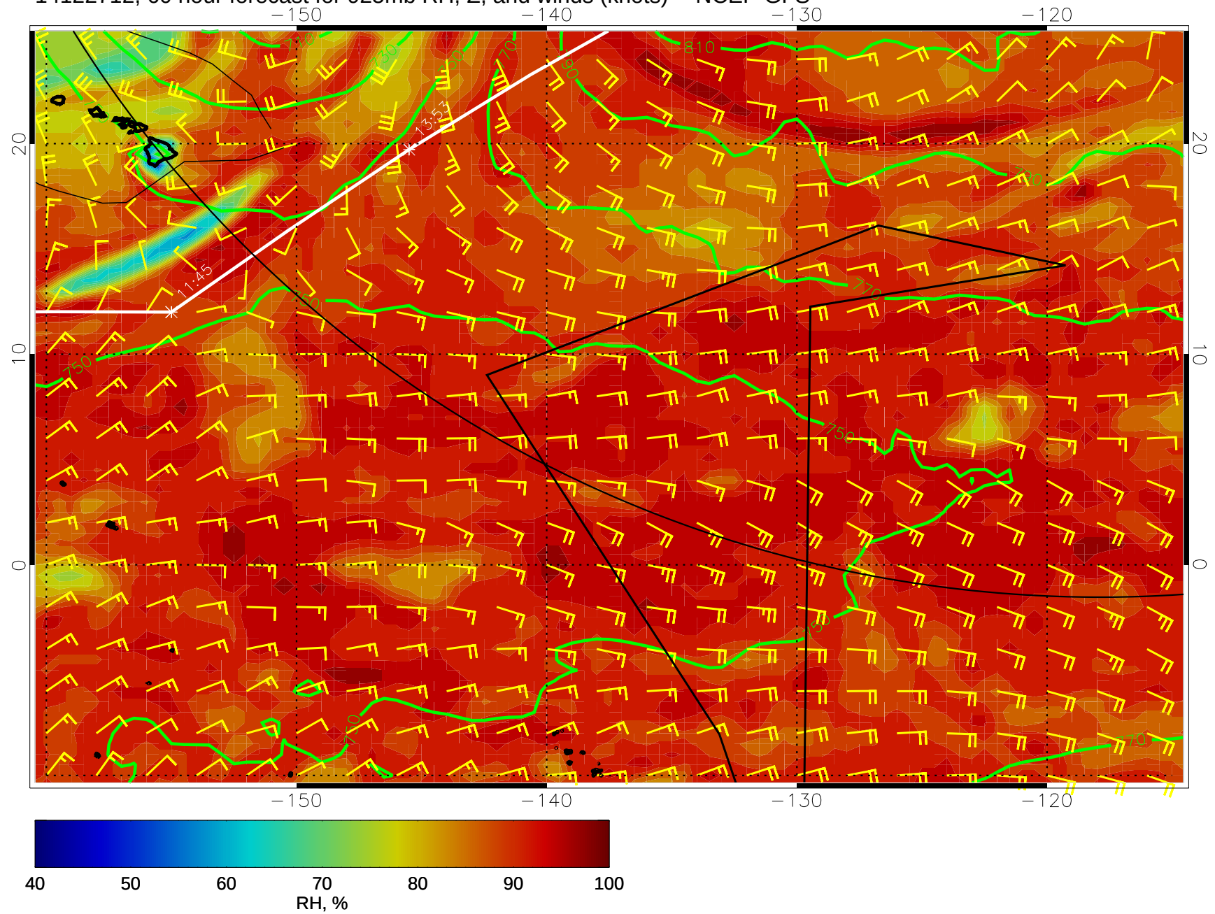
14122712, 60 hour forecast for 925mb RH, Z, and winds (knots) -- NCEP GFS
