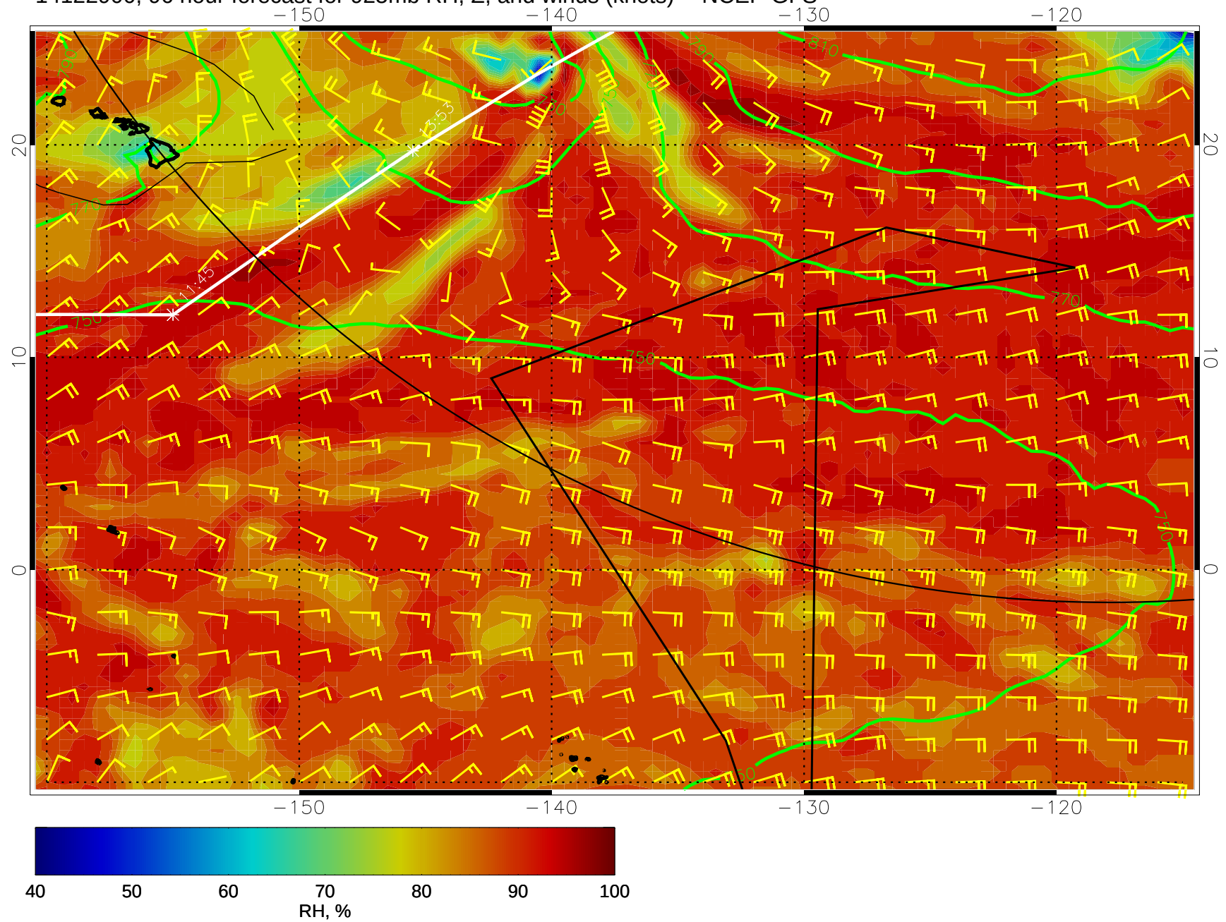
14122900, 96 hour forecast for 925mb RH, Z, and winds (knots) -- NCEP GFS
