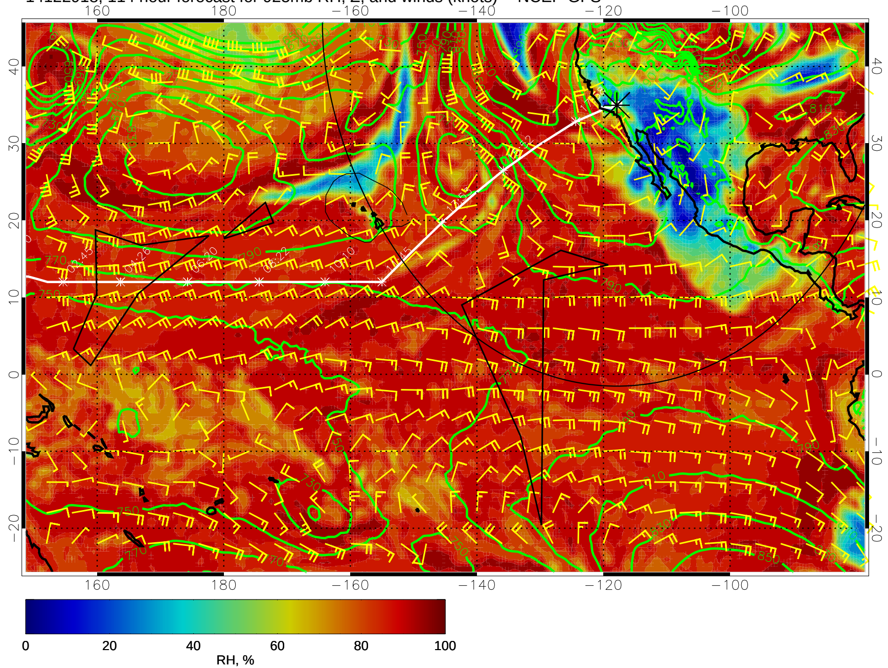
14122918, 114 hour forecast for 925mb RH, Z, and winds (knots) -- NCEP GFS
