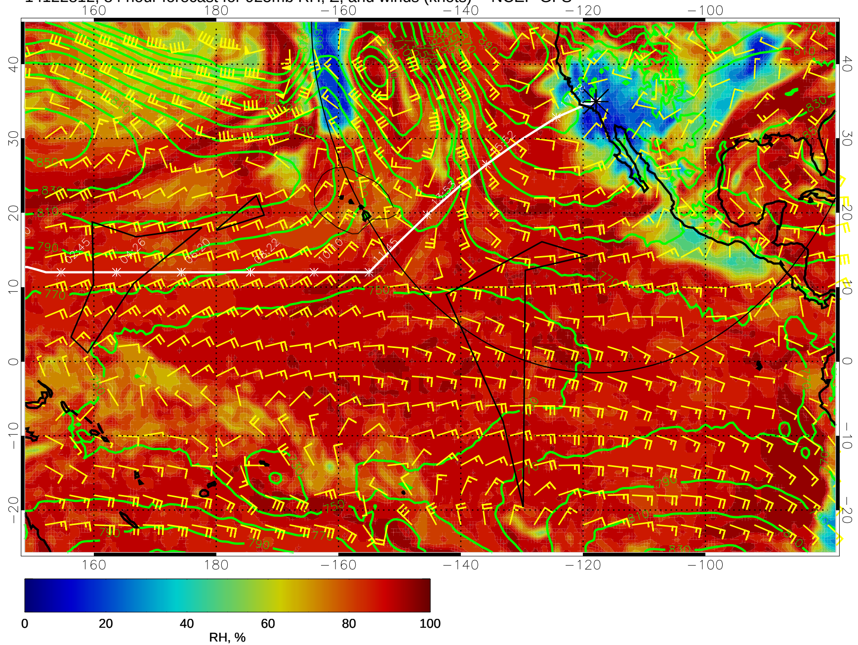
14122812, 84 hour forecast for 925mb RH, Z, and winds (knots) -- NCEP GFS
