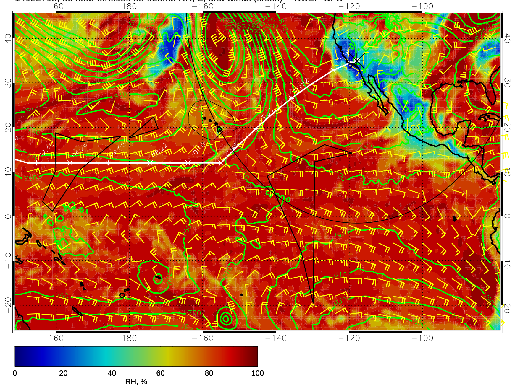
14122718, 66 hour forecast for 925mb RH, Z, and winds (knots) -- NCEP GFS
