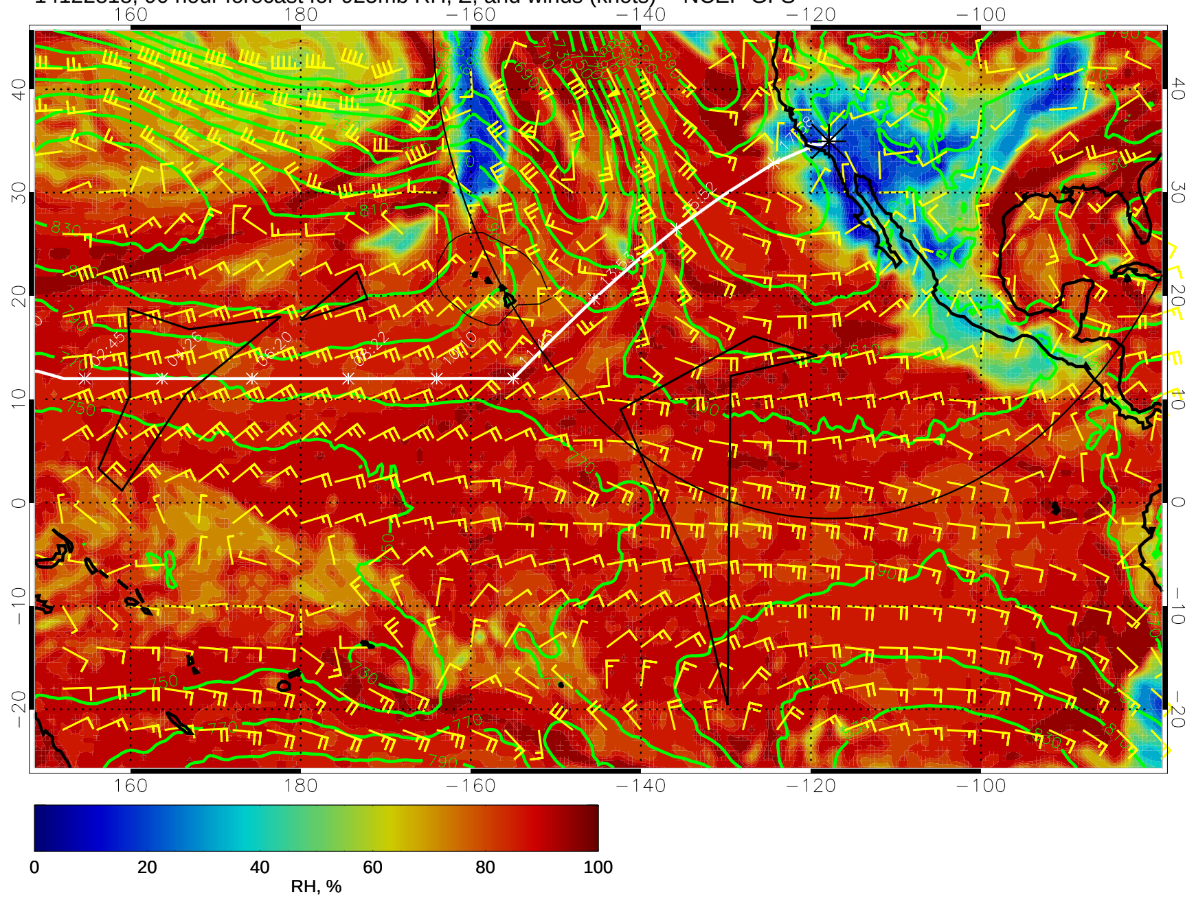
14122818, 90 hour forecast for 925mb RH, Z, and winds (knots) -- NCEP GFS
