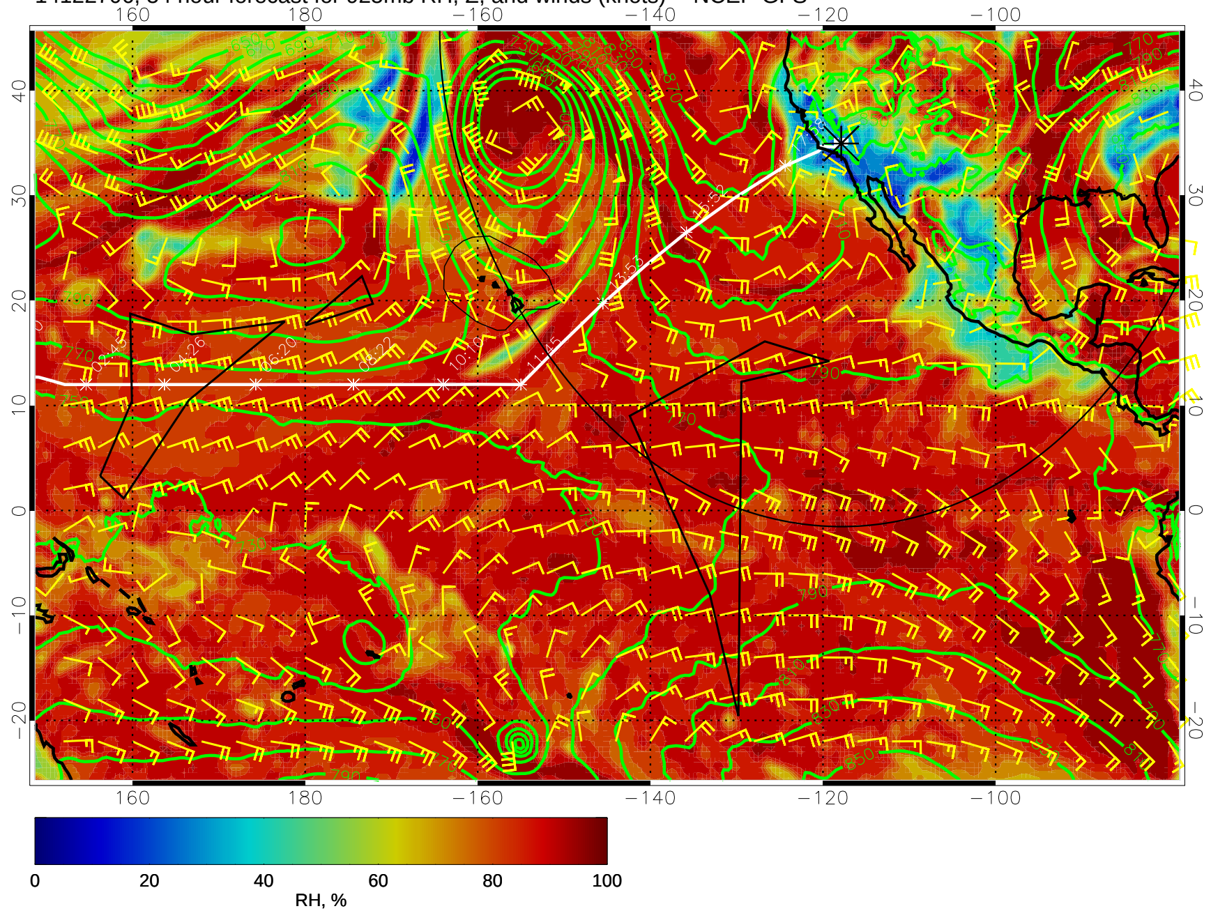
14122706, 54 hour forecast for 925mb RH, Z, and winds (knots) -- NCEP GFS
