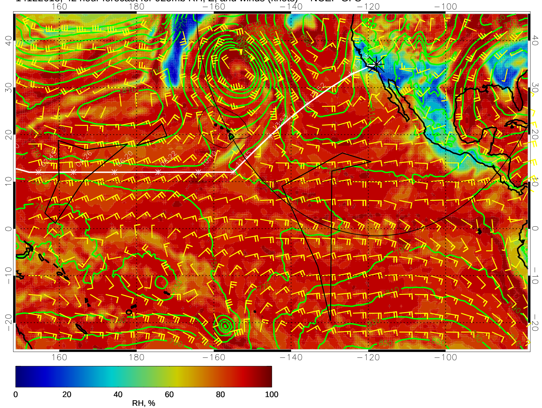
14122618, 42 hour forecast for 925mb RH, Z, and winds (knots) -- NCEP GFS
