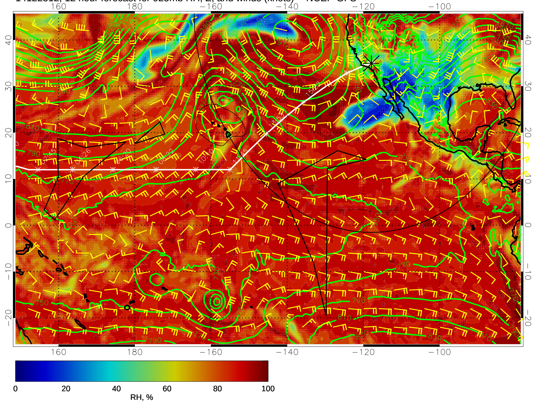
14122512, 12 hour forecast for 925mb RH, Z, and winds (knots) -- NCEP GFS
