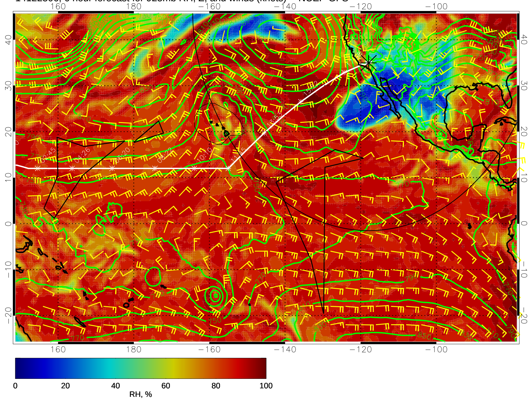
14122506, 6 hour forecast for 925mb RH, Z, and winds (knots) -- NCEP GFS
