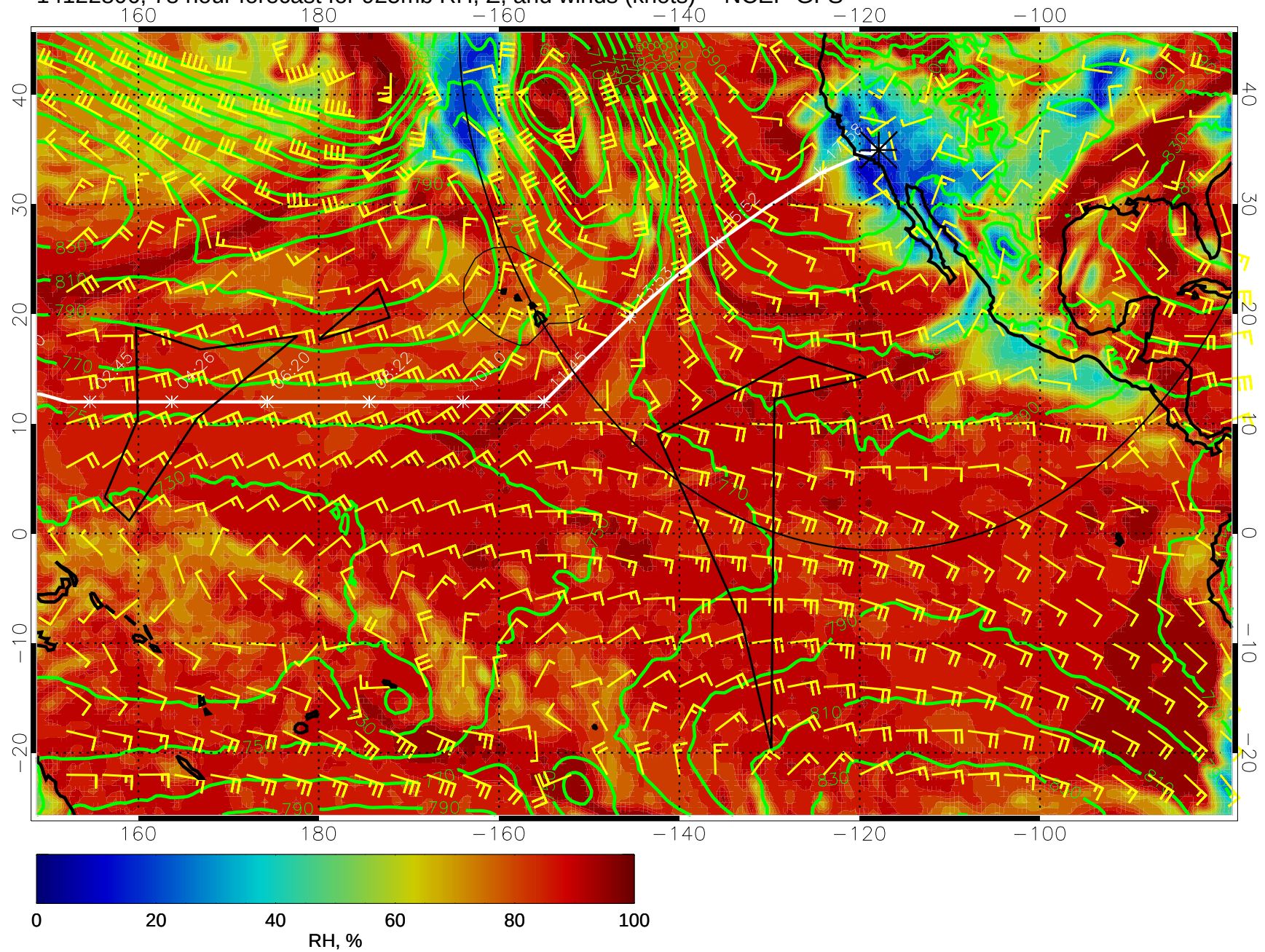
14122806, 78 hour forecast for 925mb RH, Z, and winds (knots) -- NCEP GFS
