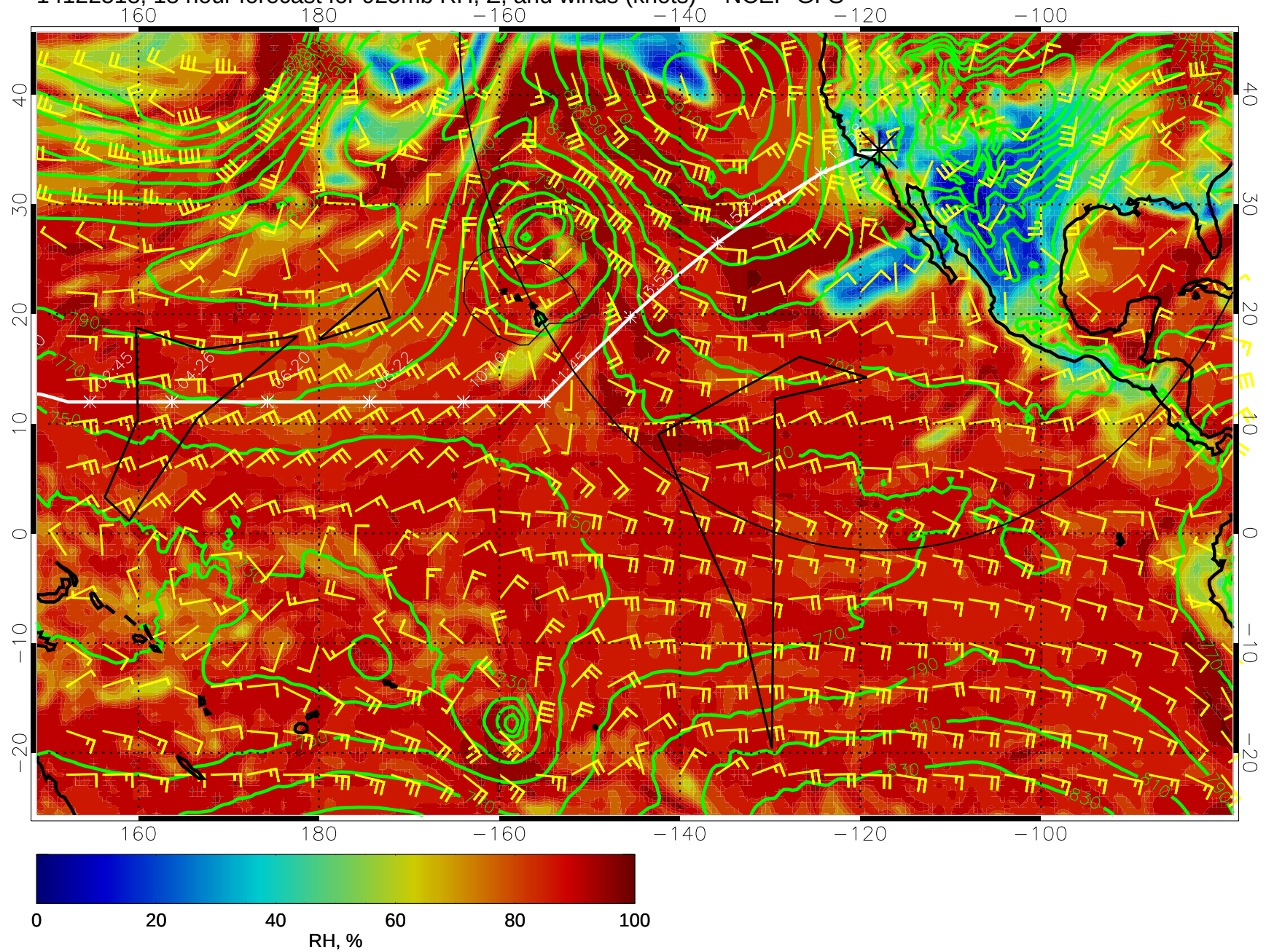
14122518, 18 hour forecast for 925mb RH, Z, and winds (knots) -- NCEP GFS
