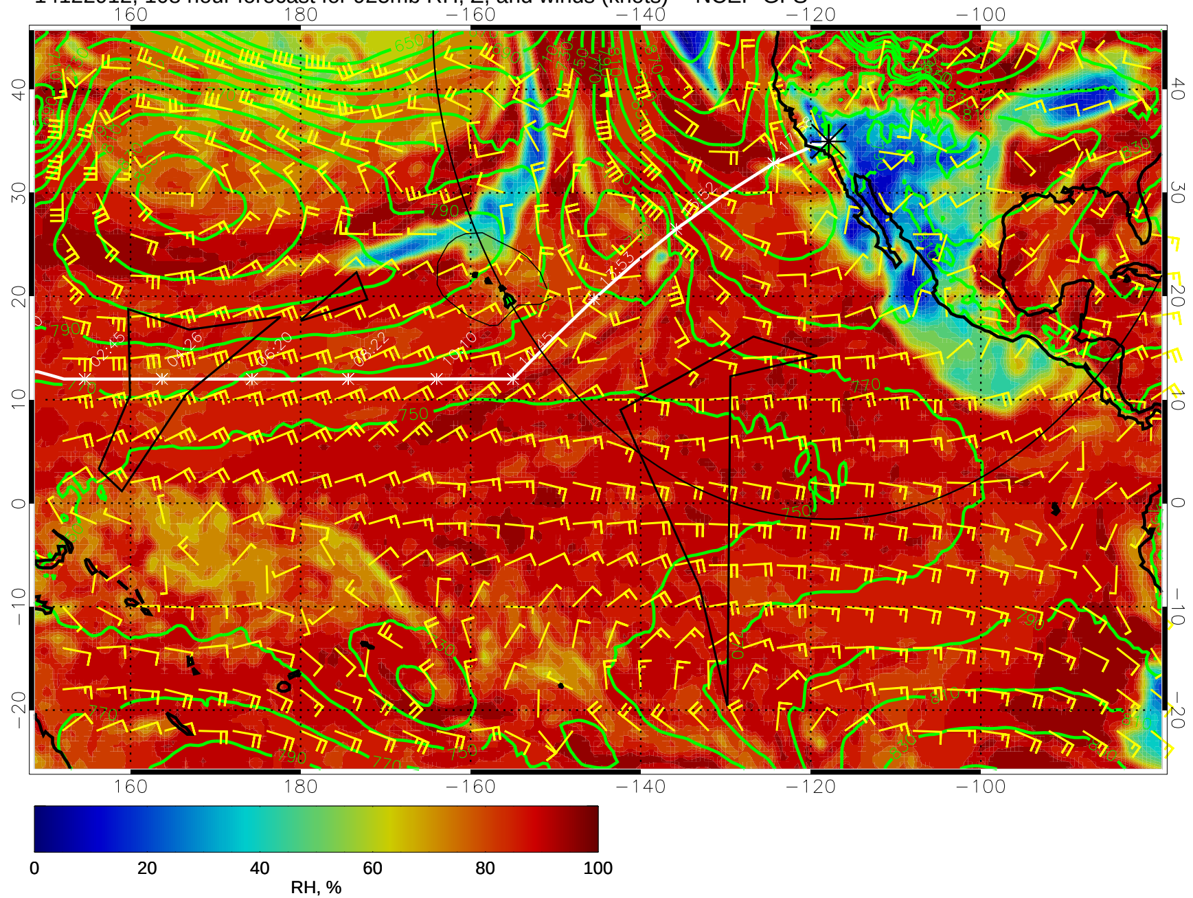
14122912, 108 hour forecast for 925mb RH, Z, and winds (knots) -- NCEP GFS
