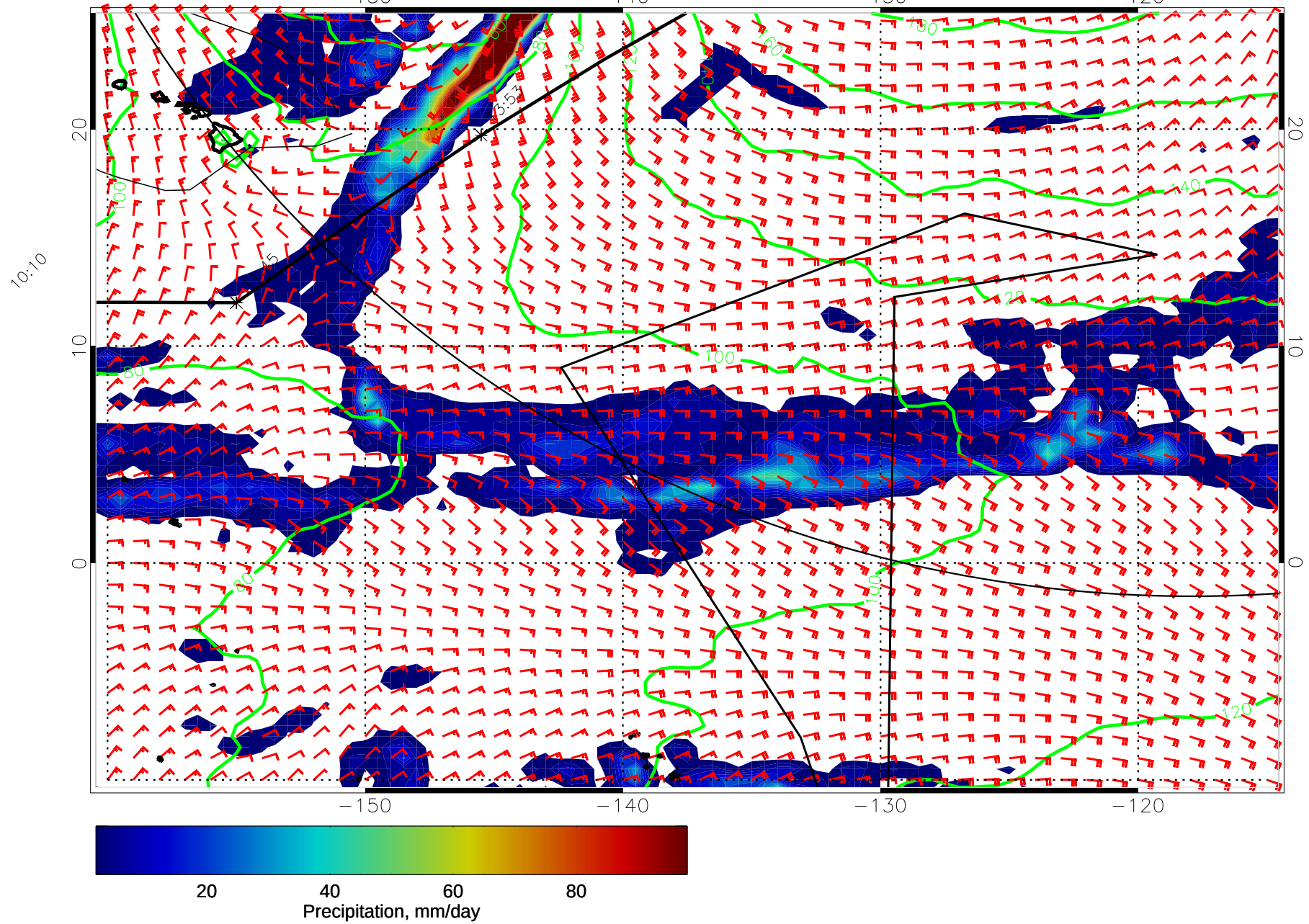
14122718, 66 hour forecast for precip, 1000mb Z, and winds (knots) -- NCEP GFS
