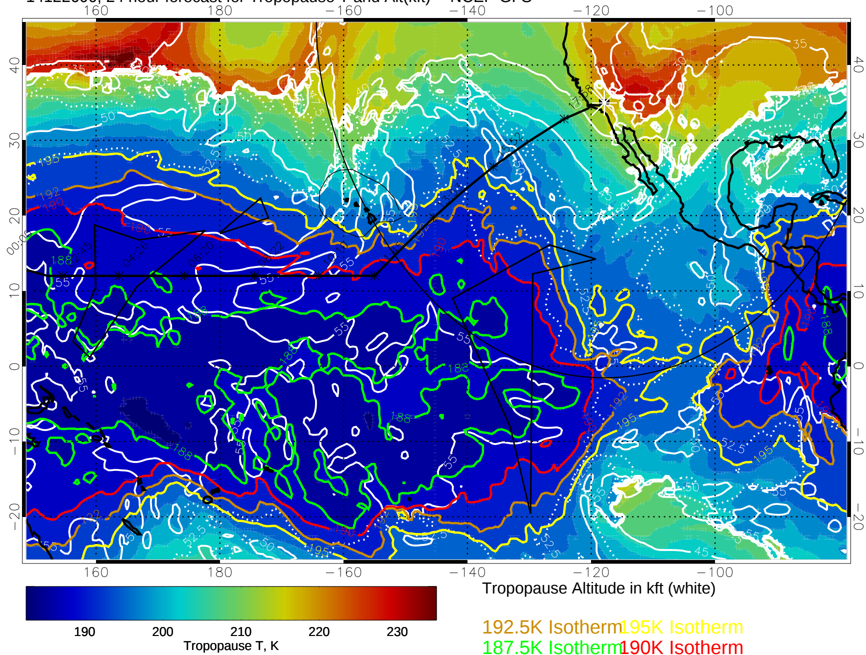
14122600, 24 hour forecast for Tropopause T and Alt(kft) -- NCEP GFS
