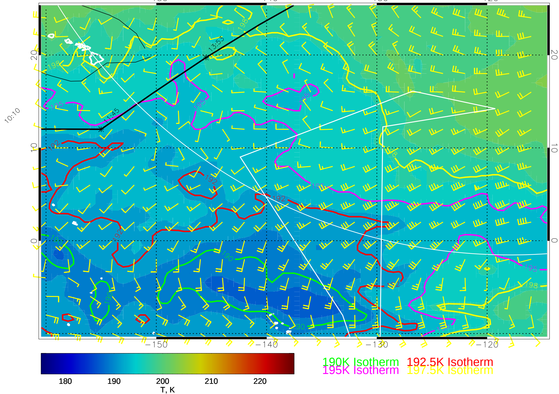
14122600, 24 hour forecast for 70mb T and winds (knots) -- NCEP GFS
