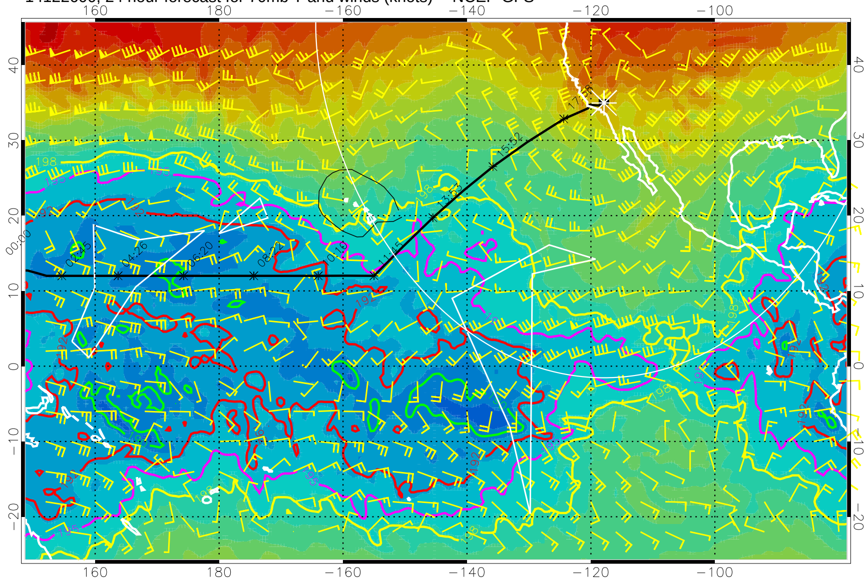
14122600, 24 hour forecast for 70mb T and winds (knots) -- NCEP GFS
