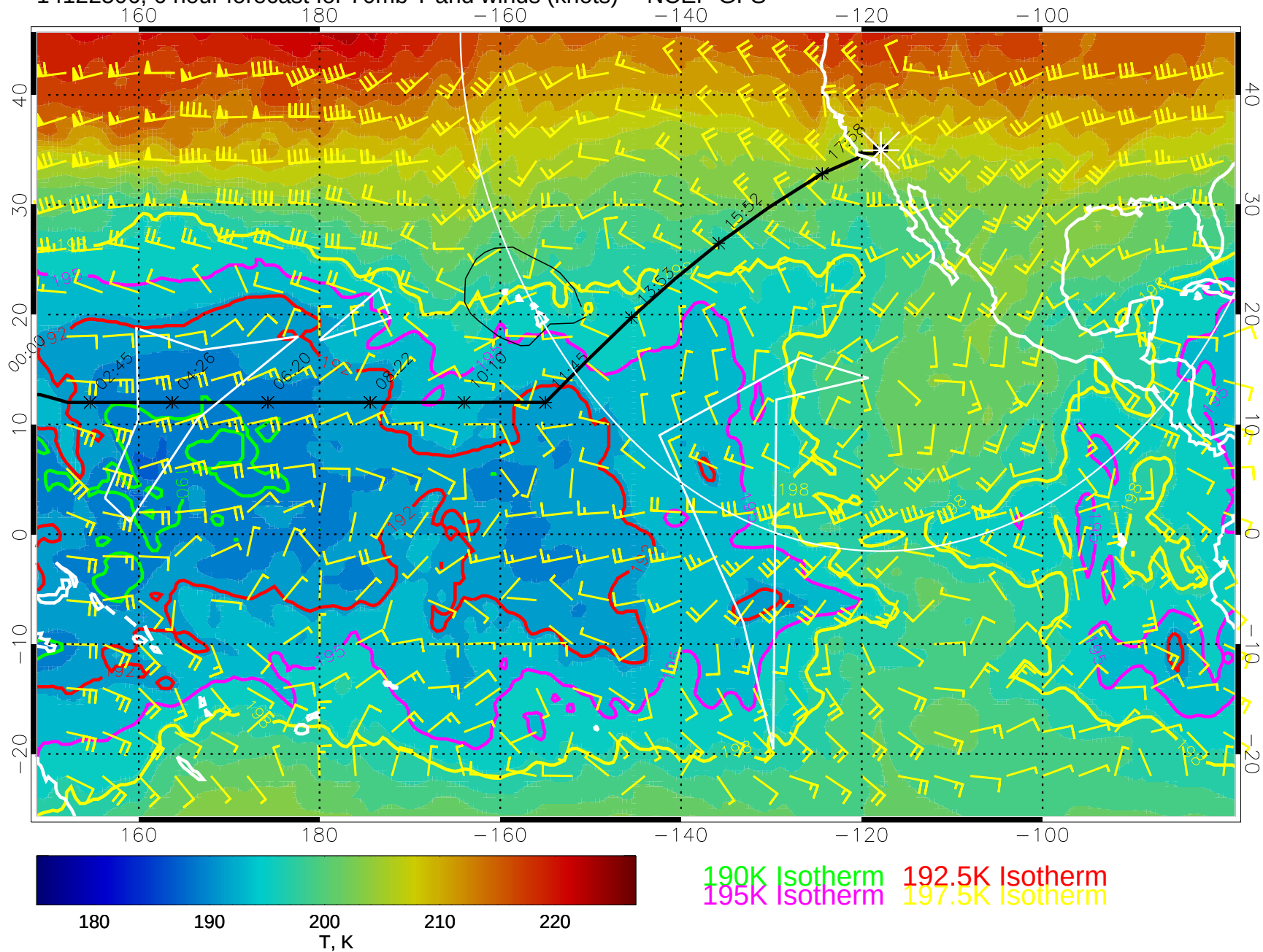
14122506, 6 hour forecast for 70mb T and winds (knots) -- NCEP GFS
