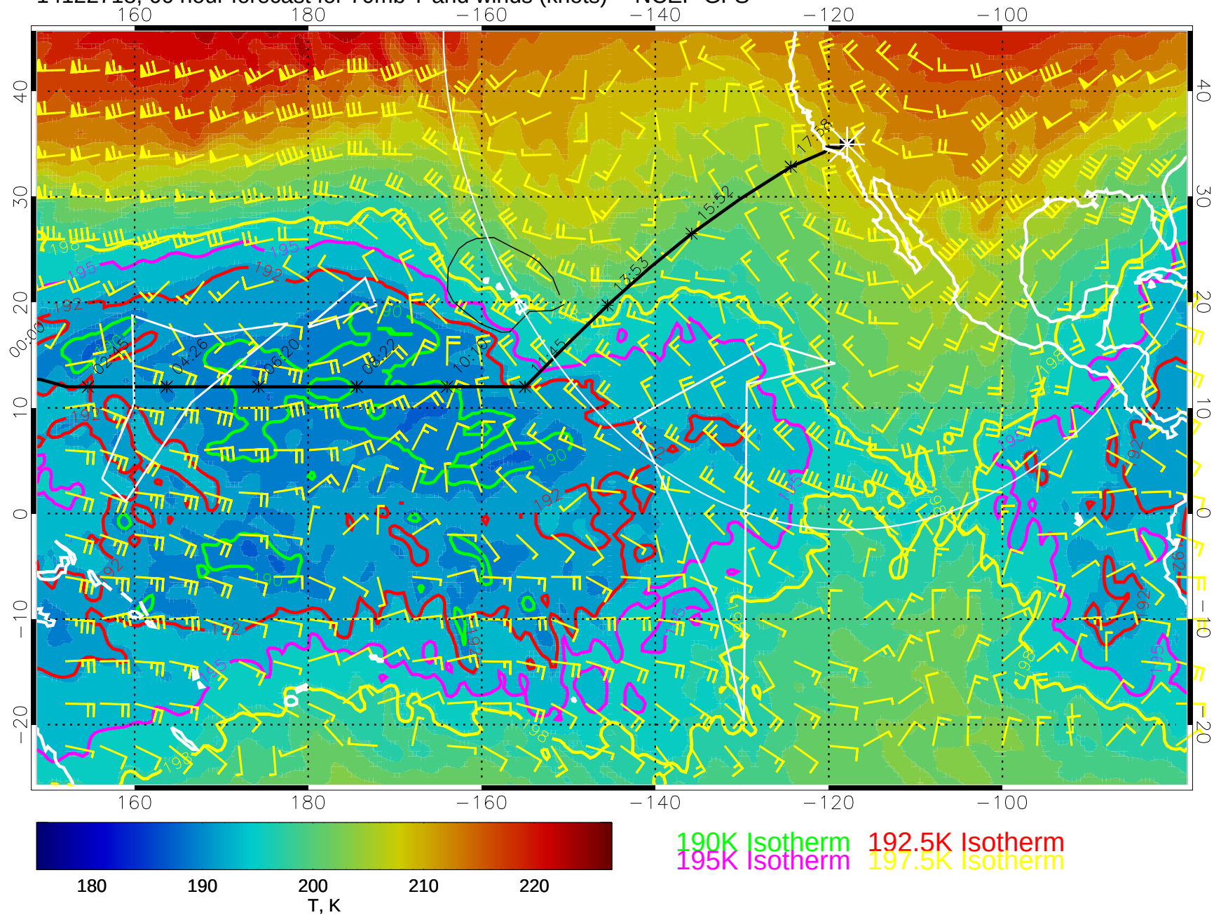
14122718, 66 hour forecast for 70mb T and winds (knots) -- NCEP GFS
