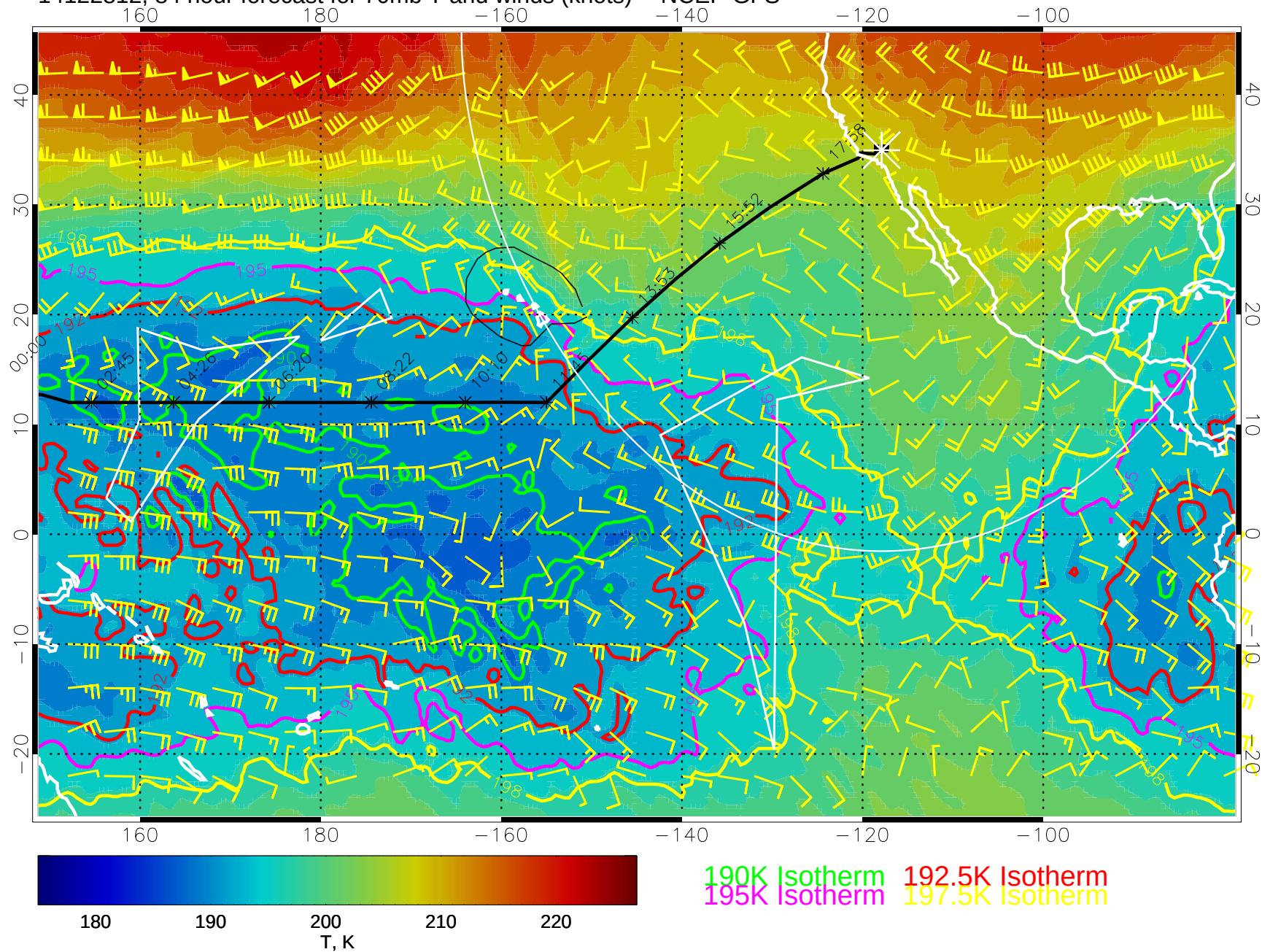
14122812, 84 hour forecast for 70mb T and winds (knots) -- NCEP GFS
