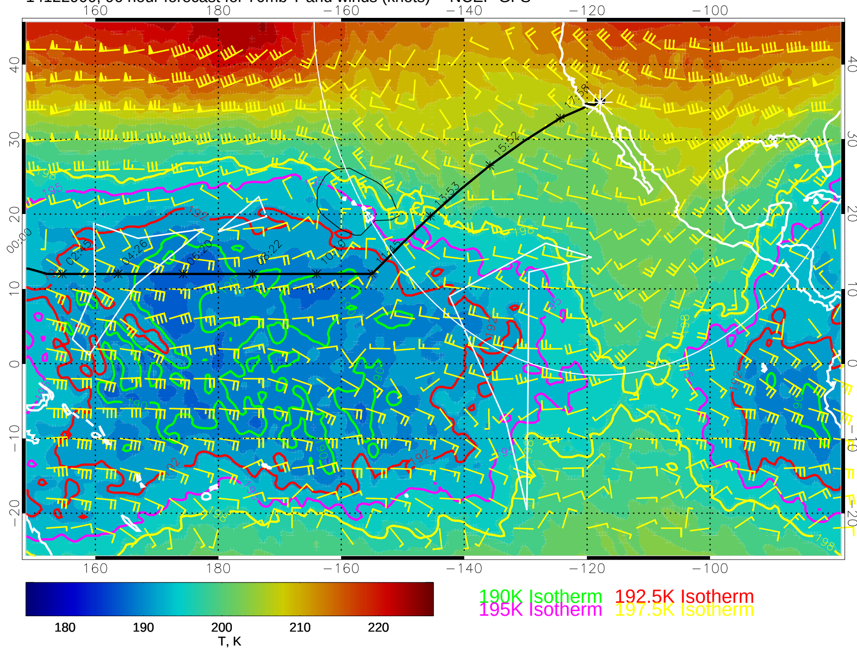
14122900, 96 hour forecast for 70mb T and winds (knots) -- NCEP GFS
