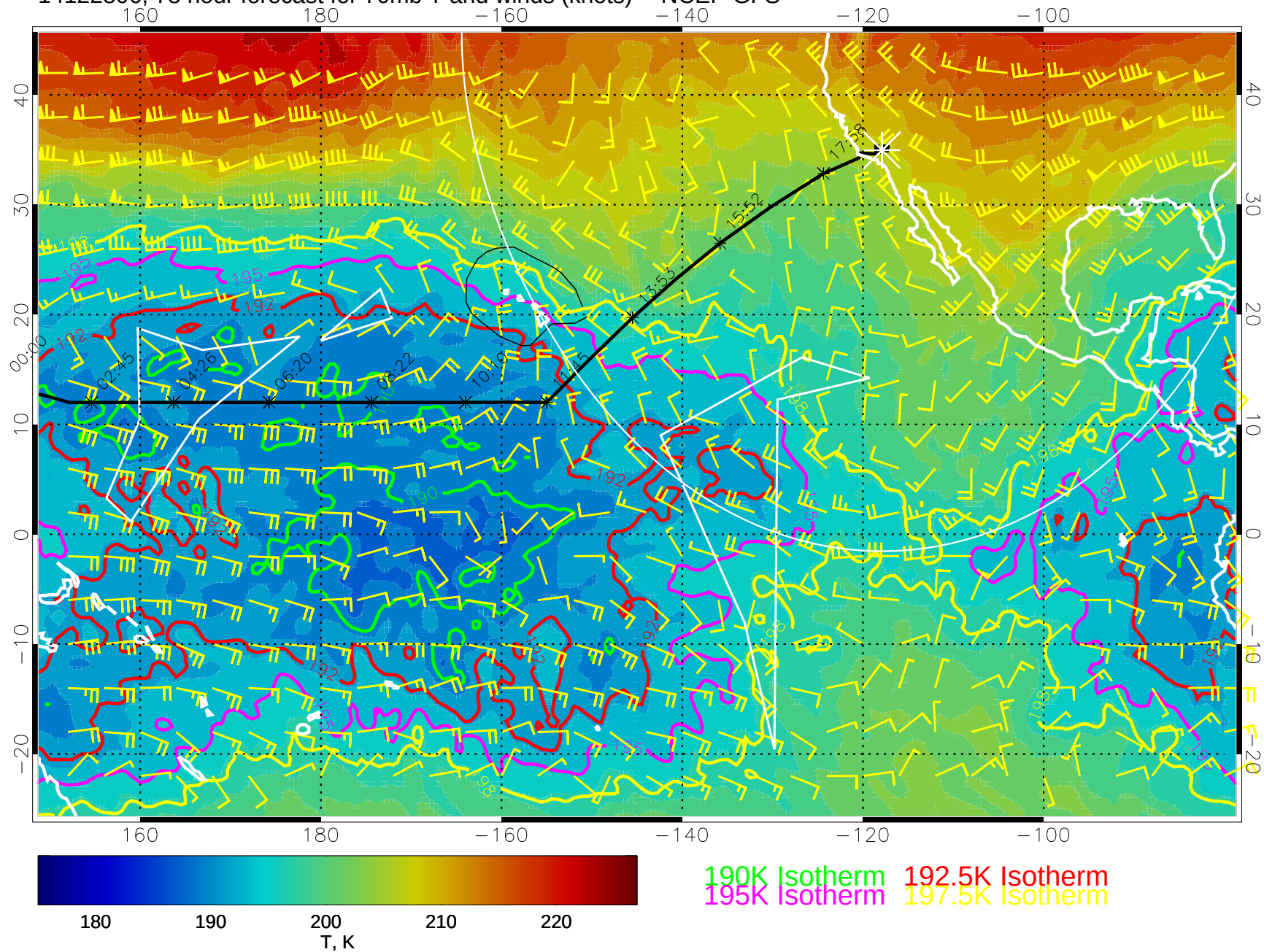
14122806, 78 hour forecast for 70mb T and winds (knots) -- NCEP GFS
