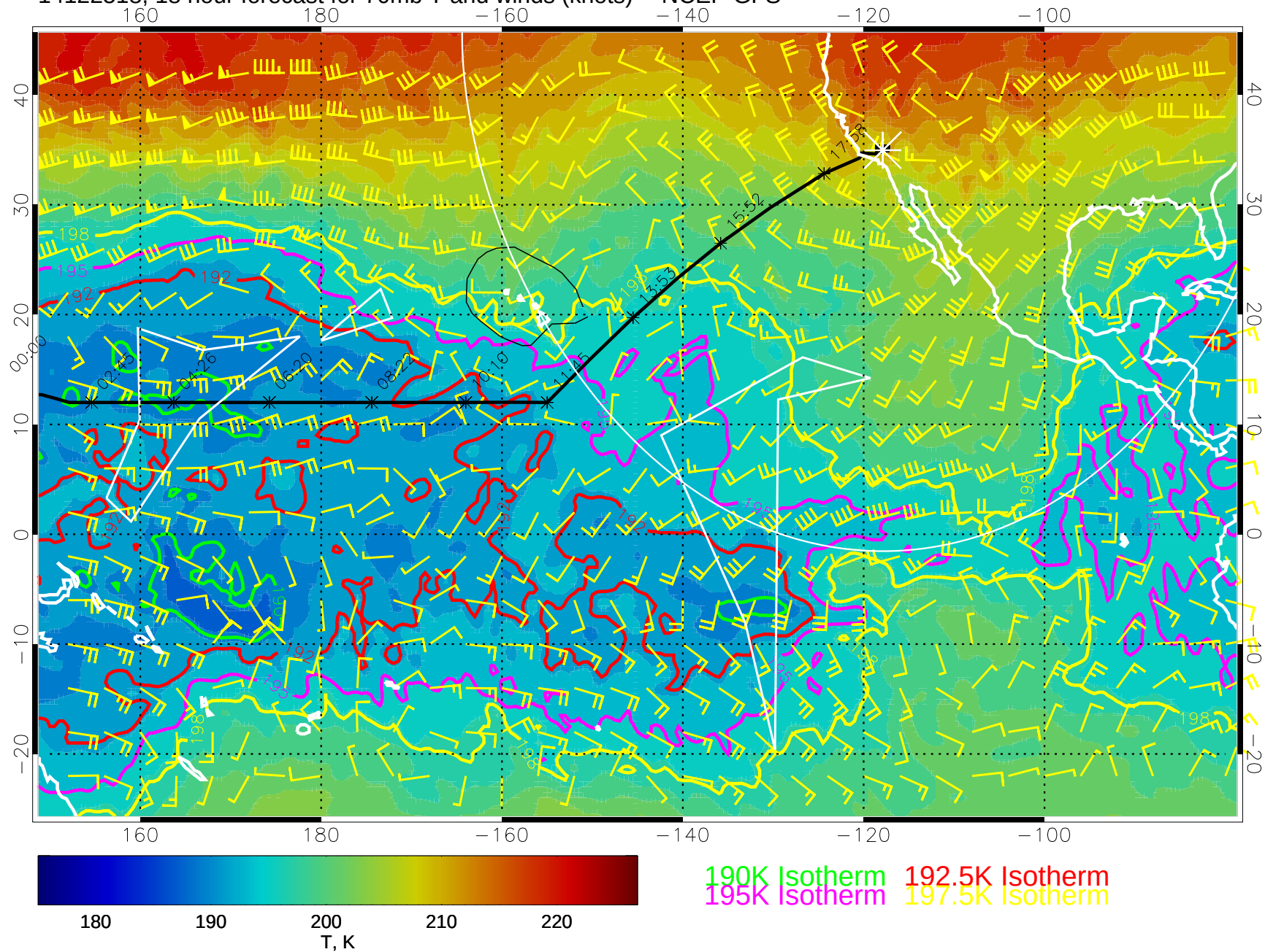
14122518, 18 hour forecast for 70mb T and winds (knots) -- NCEP GFS
