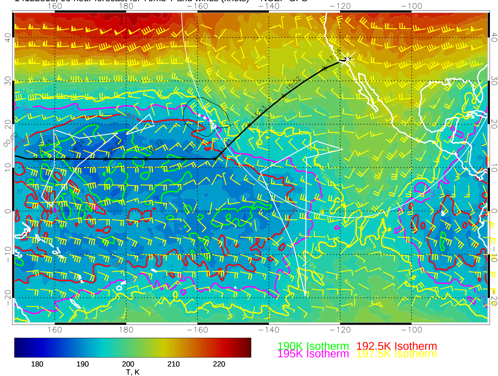
14122818, 90 hour forecast for 70mb T and winds (knots) -- NCEP GFS
