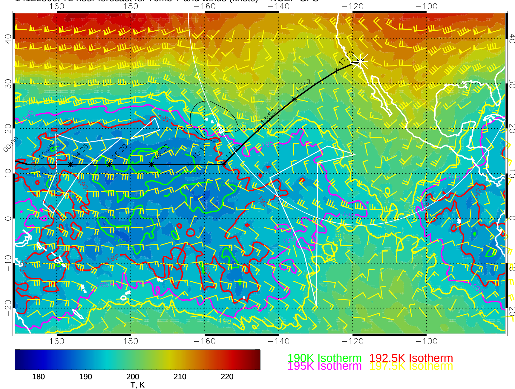
14122800, 72 hour forecast for 70mb T and winds (knots) -- NCEP GFS
