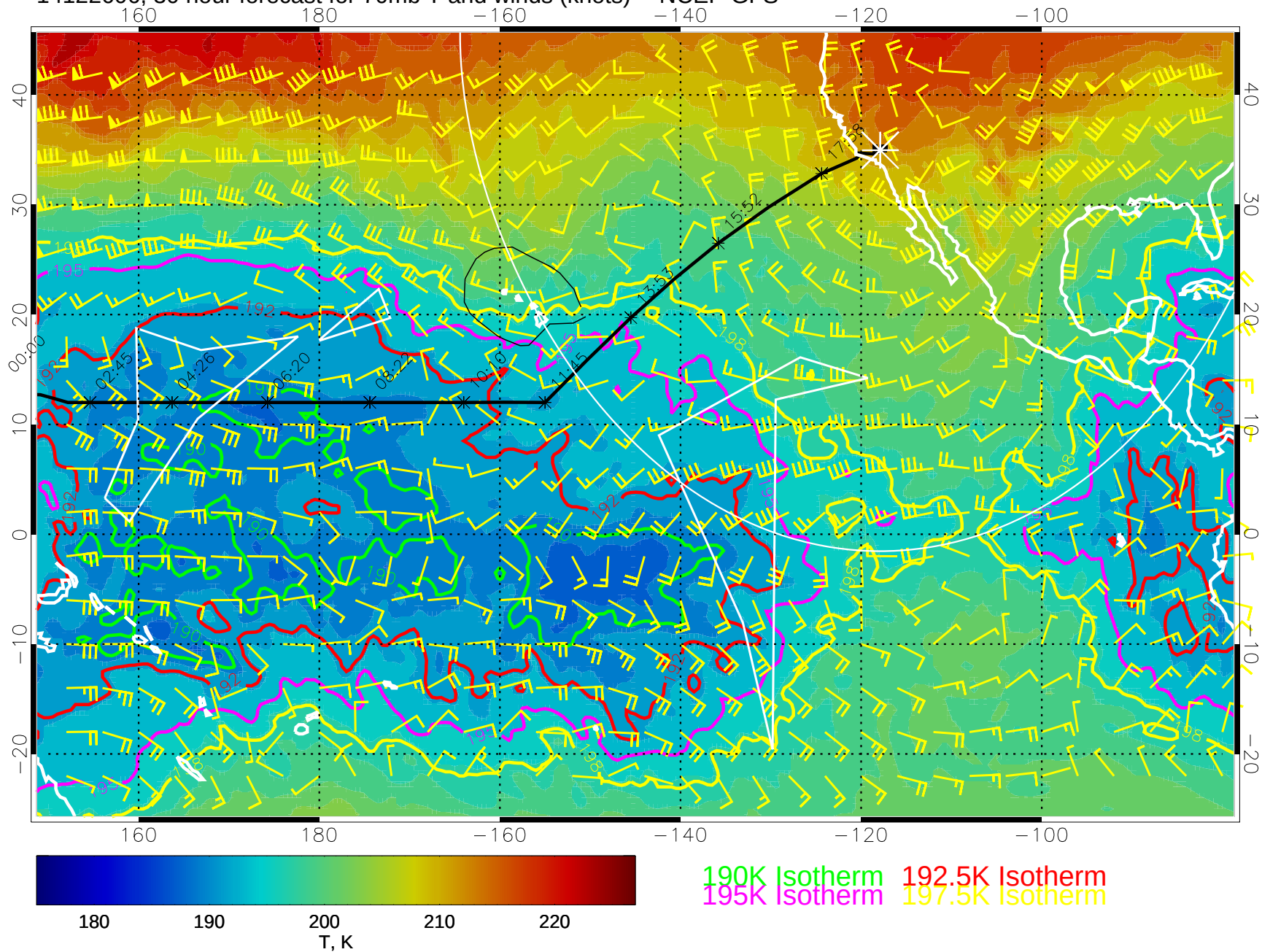
14122606, 30 hour forecast for 70mb T and winds (knots) -- NCEP GFS
