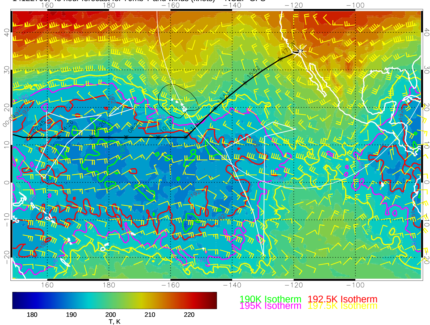
14122700, 48 hour forecast for 70mb T and winds (knots) -- NCEP GFS
