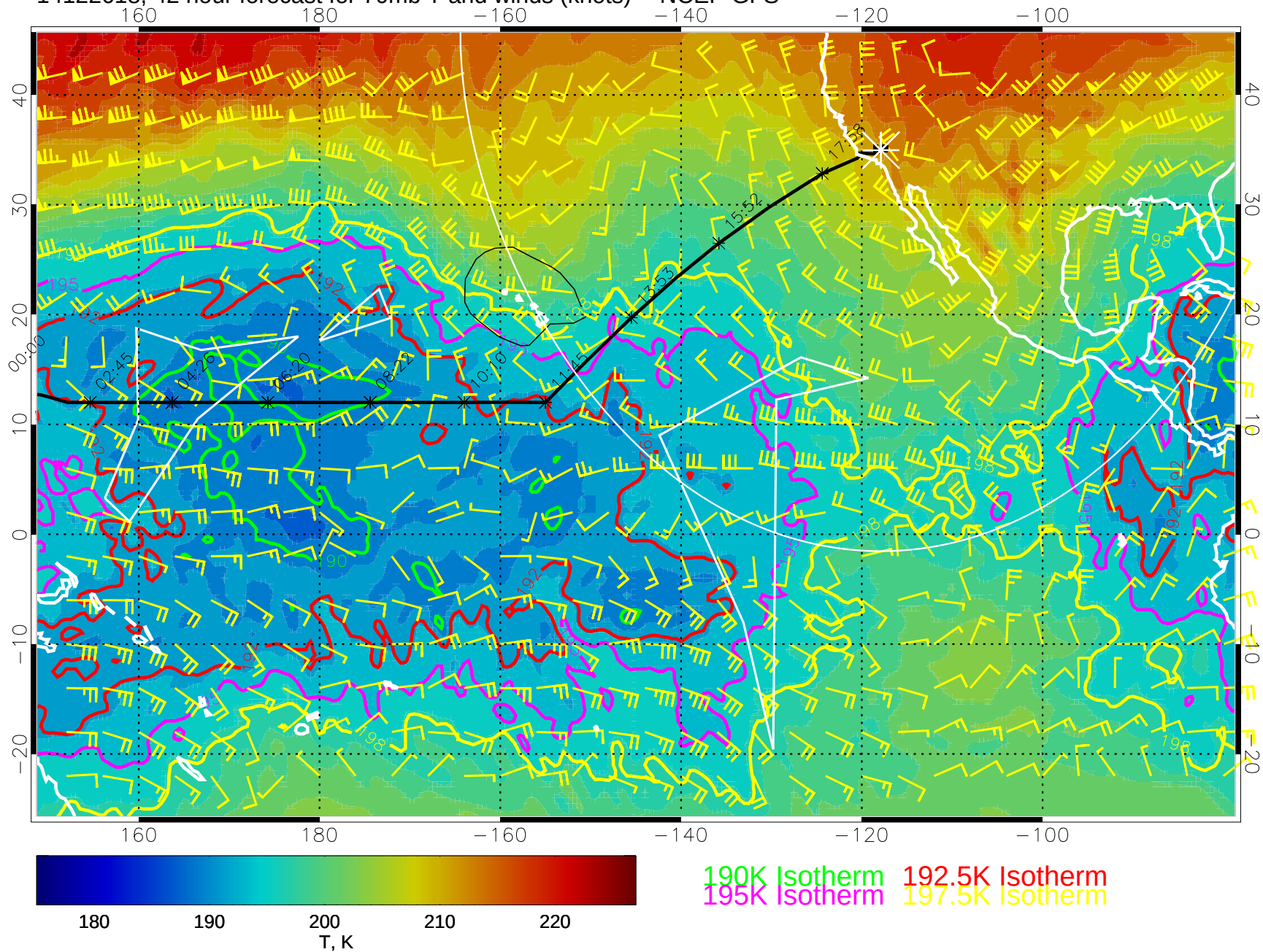
14122618, 42 hour forecast for 70mb T and winds (knots) -- NCEP GFS
