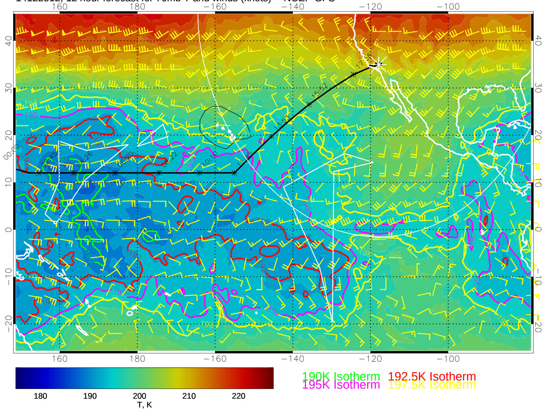
14122512, 12 hour forecast for 70mb T and winds (knots) -- NCEP GFS
