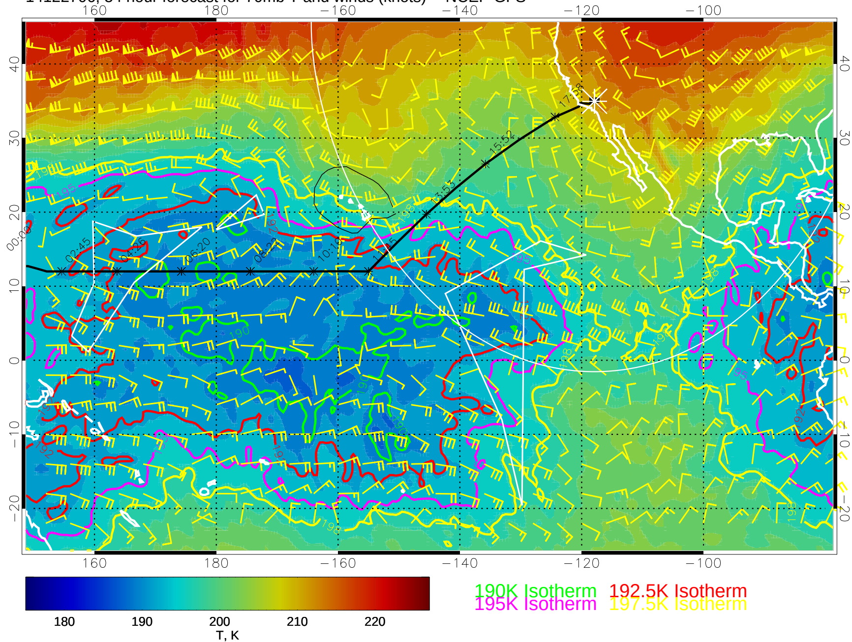
14122706, 54 hour forecast for 70mb T and winds (knots) -- NCEP GFS
