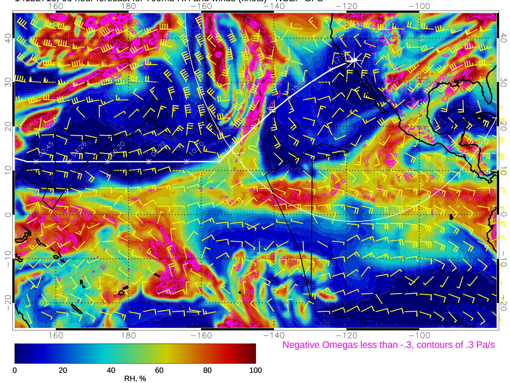
14122718, 66 hour forecast for 700mb RH and winds (knots) - NCEP GFS
