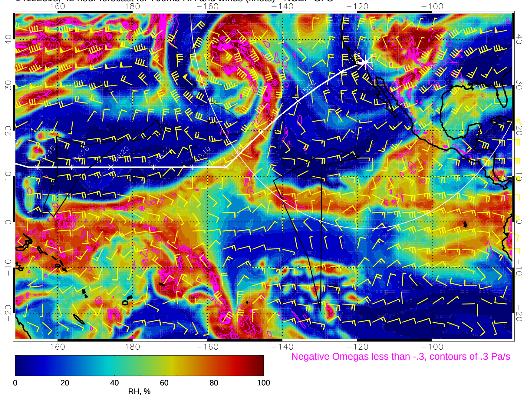
14122618, 42 hour forecast for 700mb RH and winds (knots) - NCEP GFS
