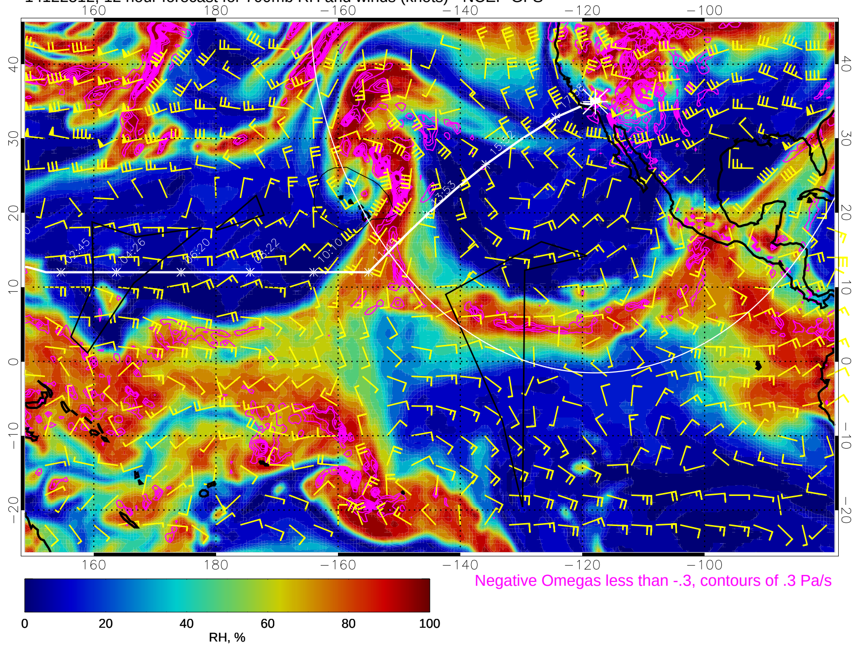
14122512, 12 hour forecast for 700mb RH and winds (knots) - NCEP GFS
