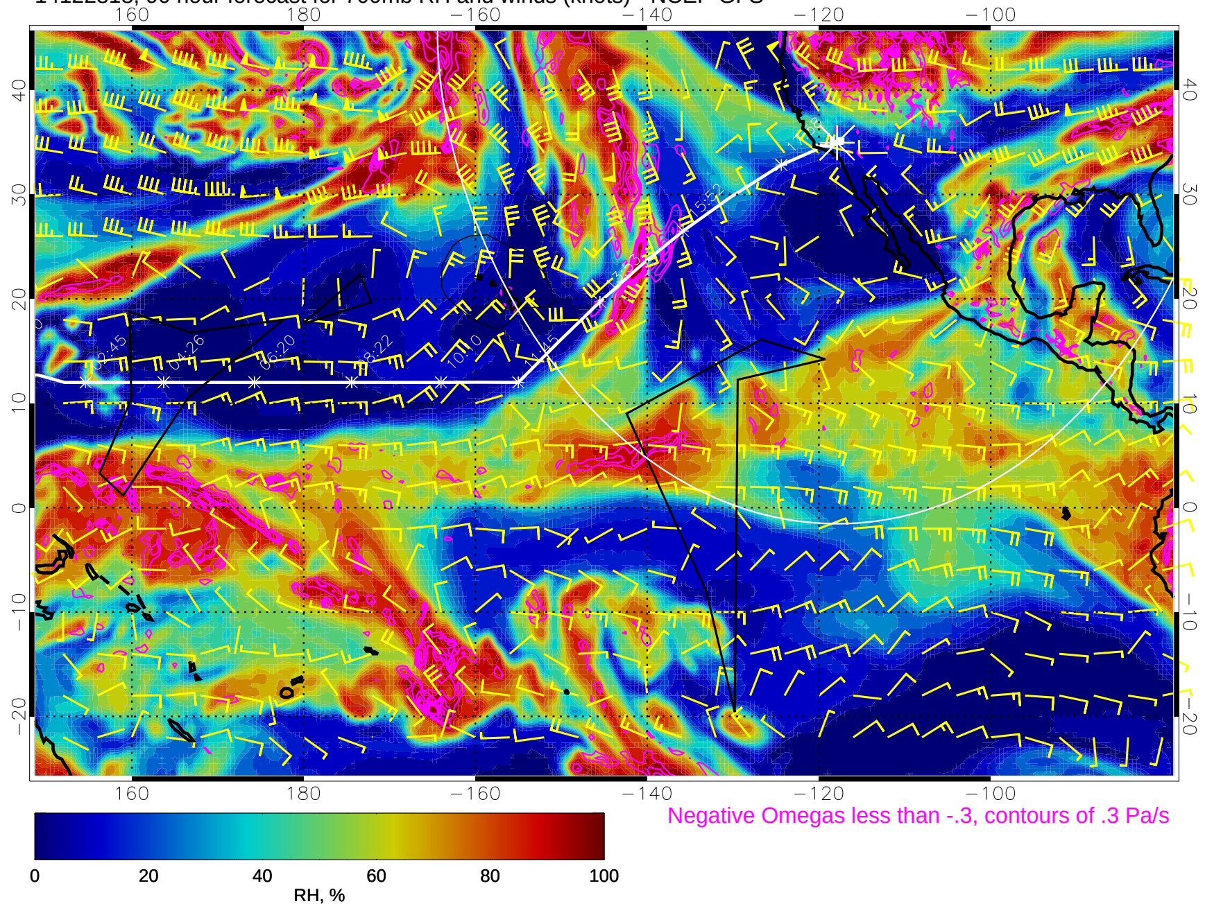
14122818, 90 hour forecast for 700mb RH and winds (knots) - NCEP GFS
