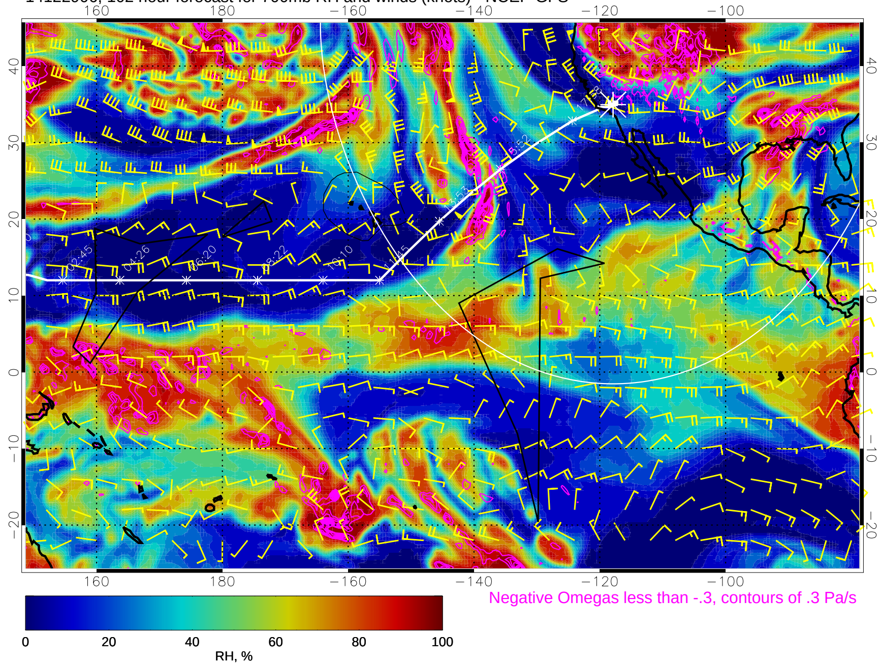
14122906, 102 hour forecast for 700mb RH and winds (knots) - NCEP GFS
