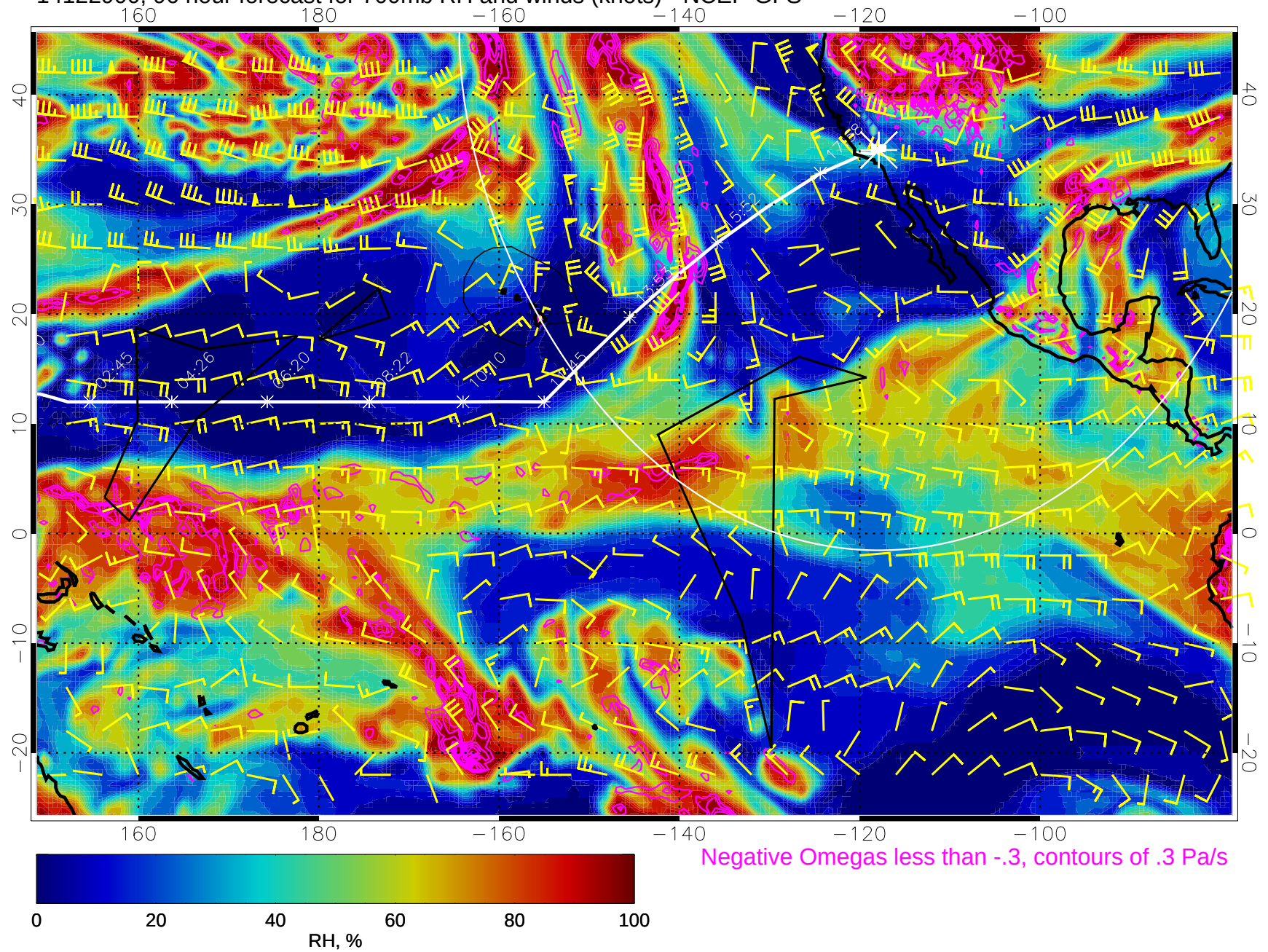
14122900, 96 hour forecast for 700mb RH and winds (knots) - NCEP GFS
