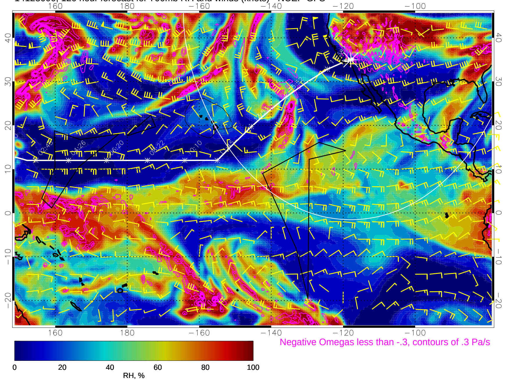
14123000, 120 hour forecast for 700mb RH and winds (knots) - NCEP GFS
