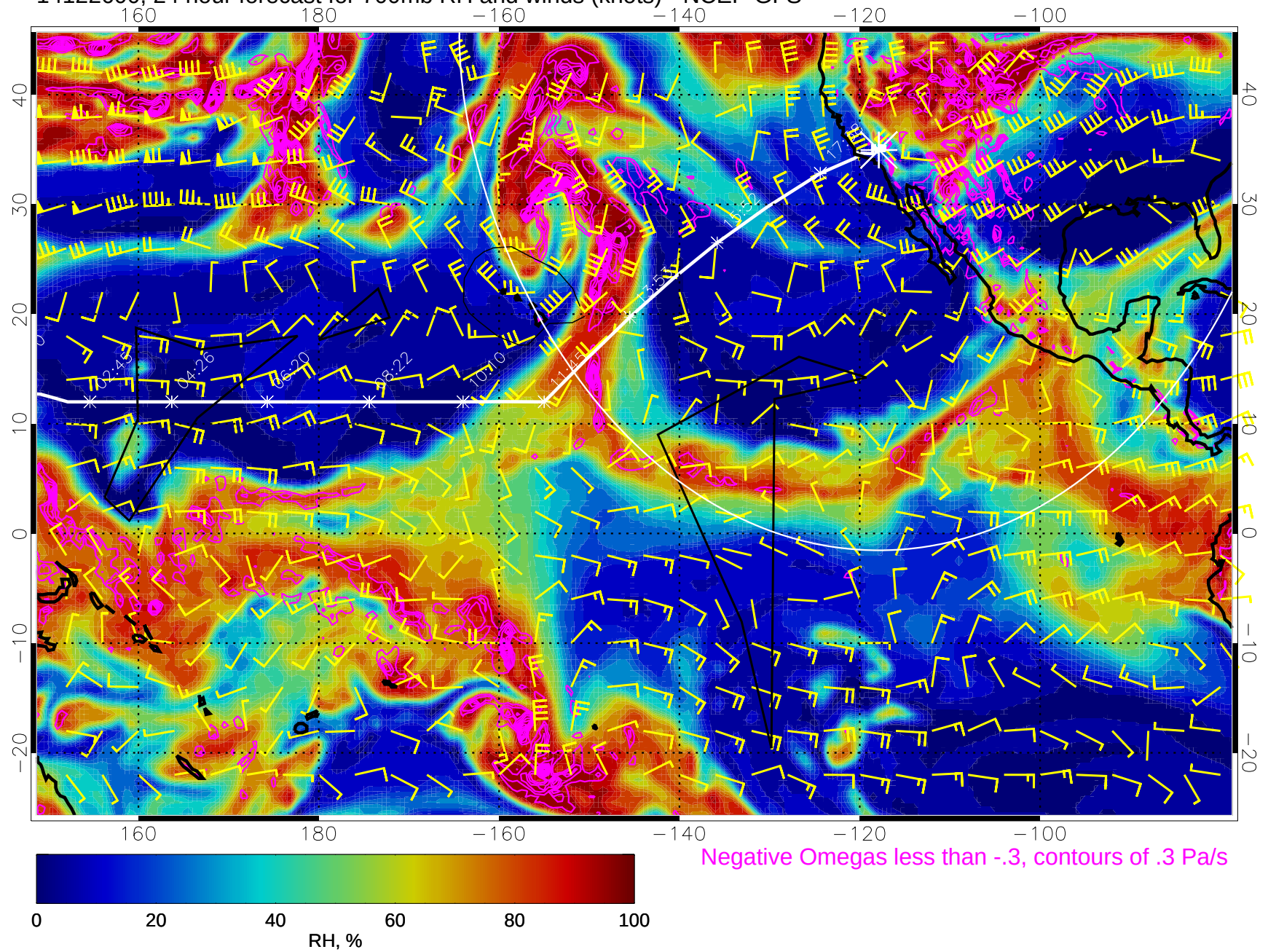
14122600, 24 hour forecast for 700mb RH and winds (knots) - NCEP GFS
