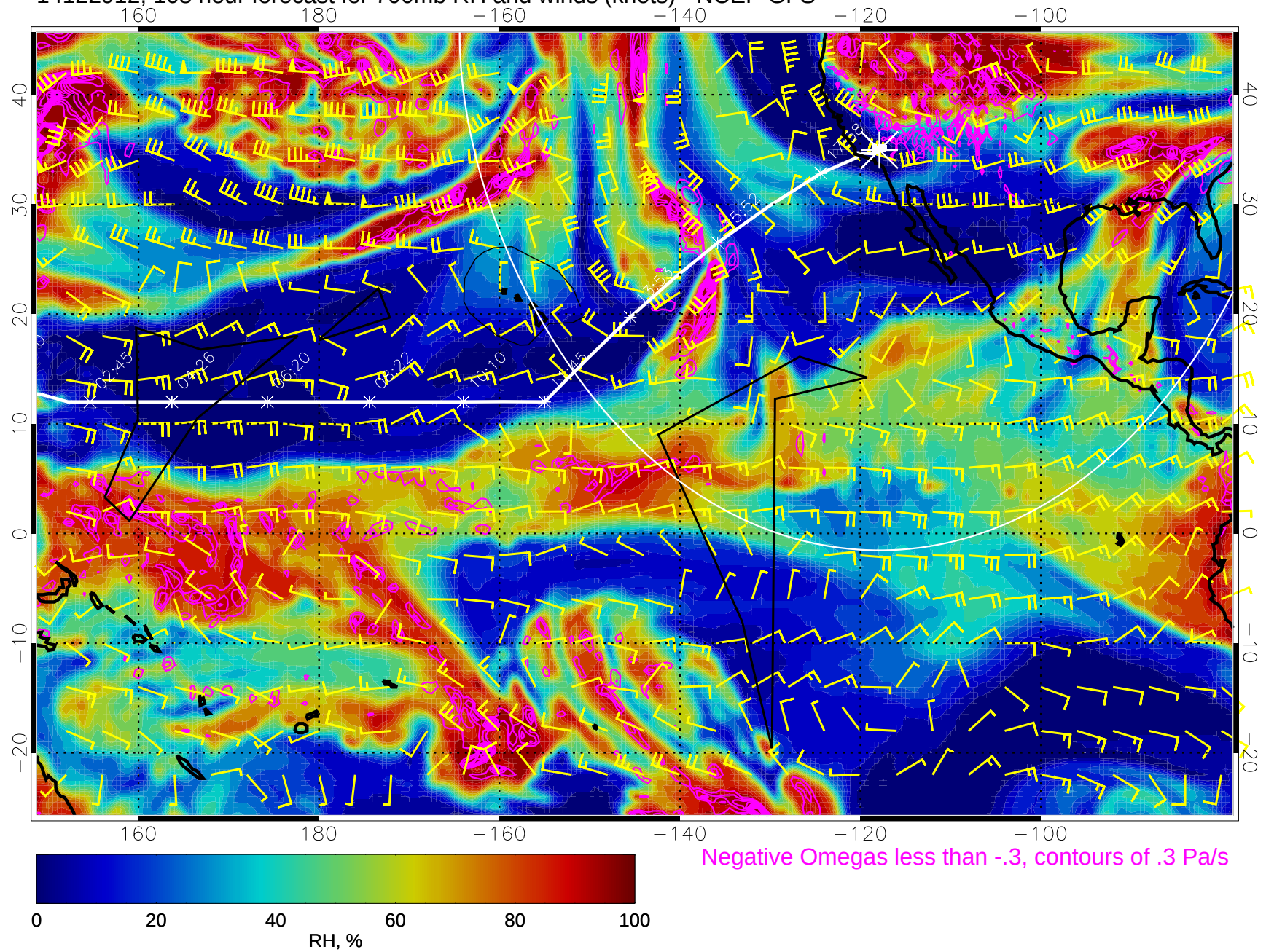
14122912, 108 hour forecast for 700mb RH and winds (knots) - NCEP GFS
