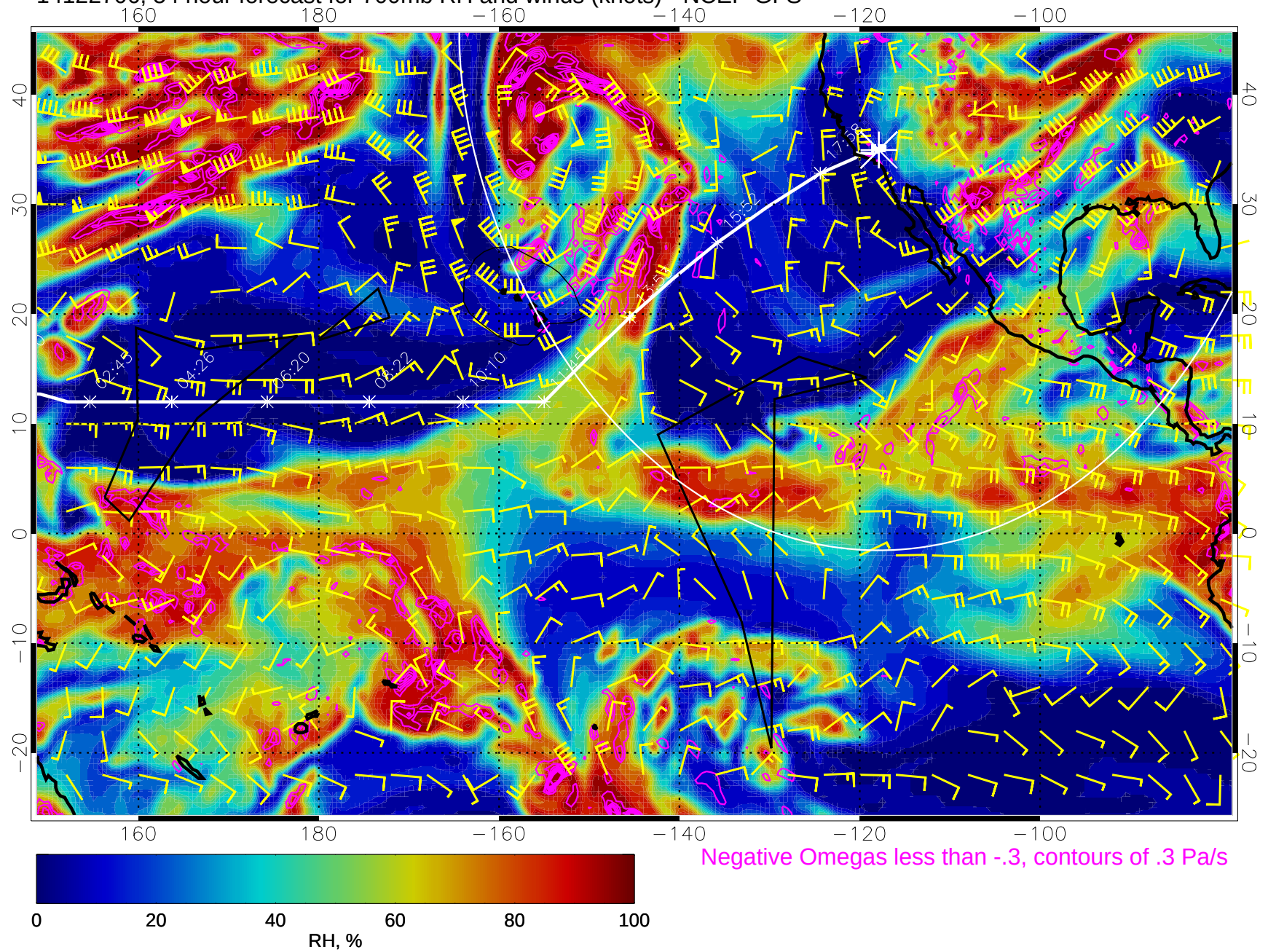
14122706, 54 hour forecast for 700mb RH and winds (knots) - NCEP GFS
