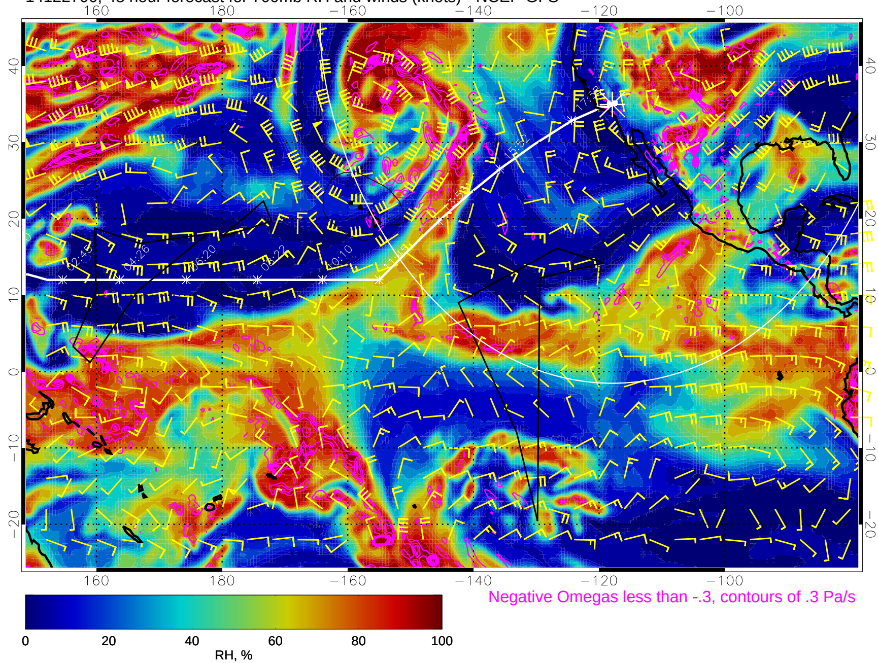
14122700, 48 hour forecast for 700mb RH and winds (knots) - NCEP GFS
