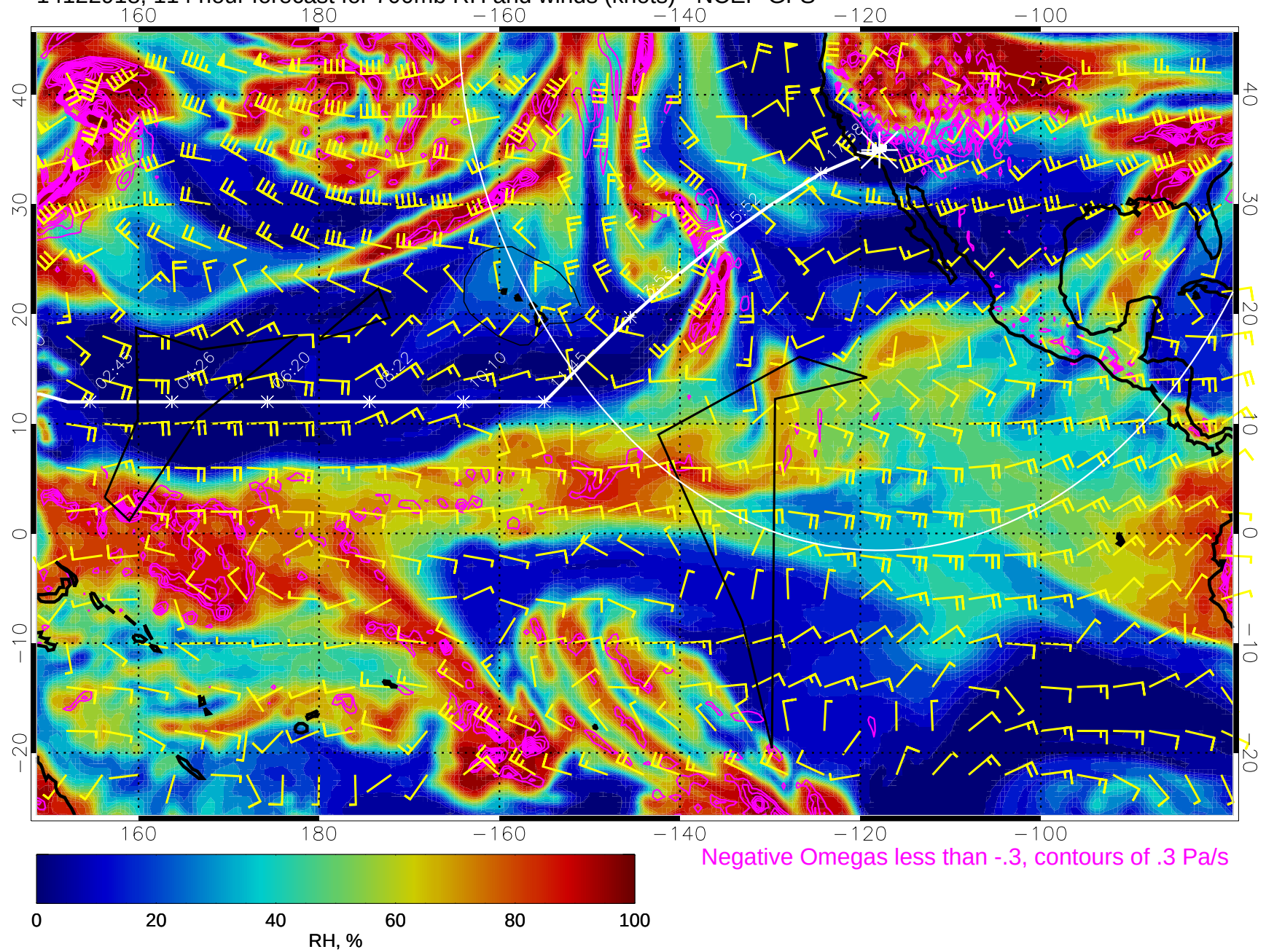
14122918, 114 hour forecast for 700mb RH and winds (knots) - NCEP GFS
