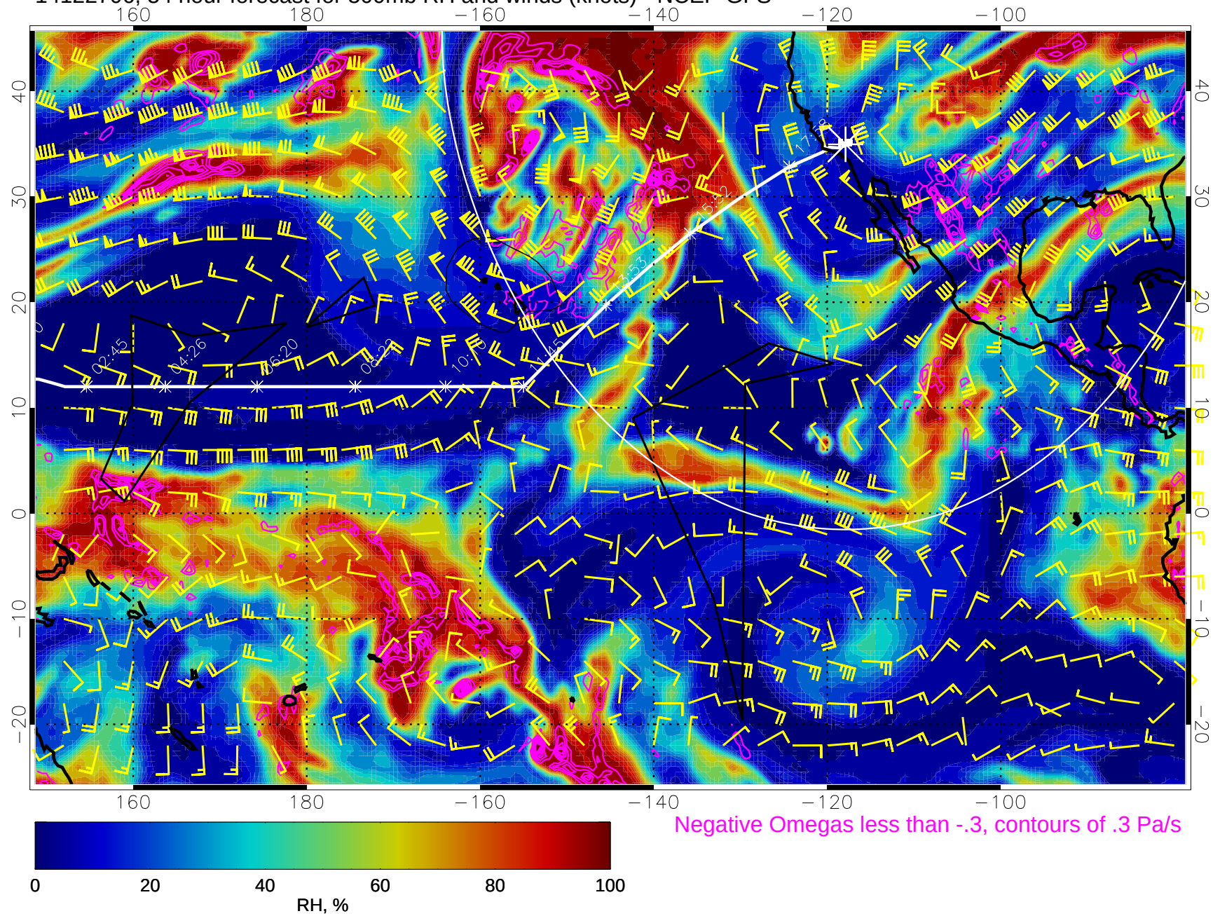
14122706, 54 hour forecast for 500mb RH and winds (knots) - NCEP GFS
