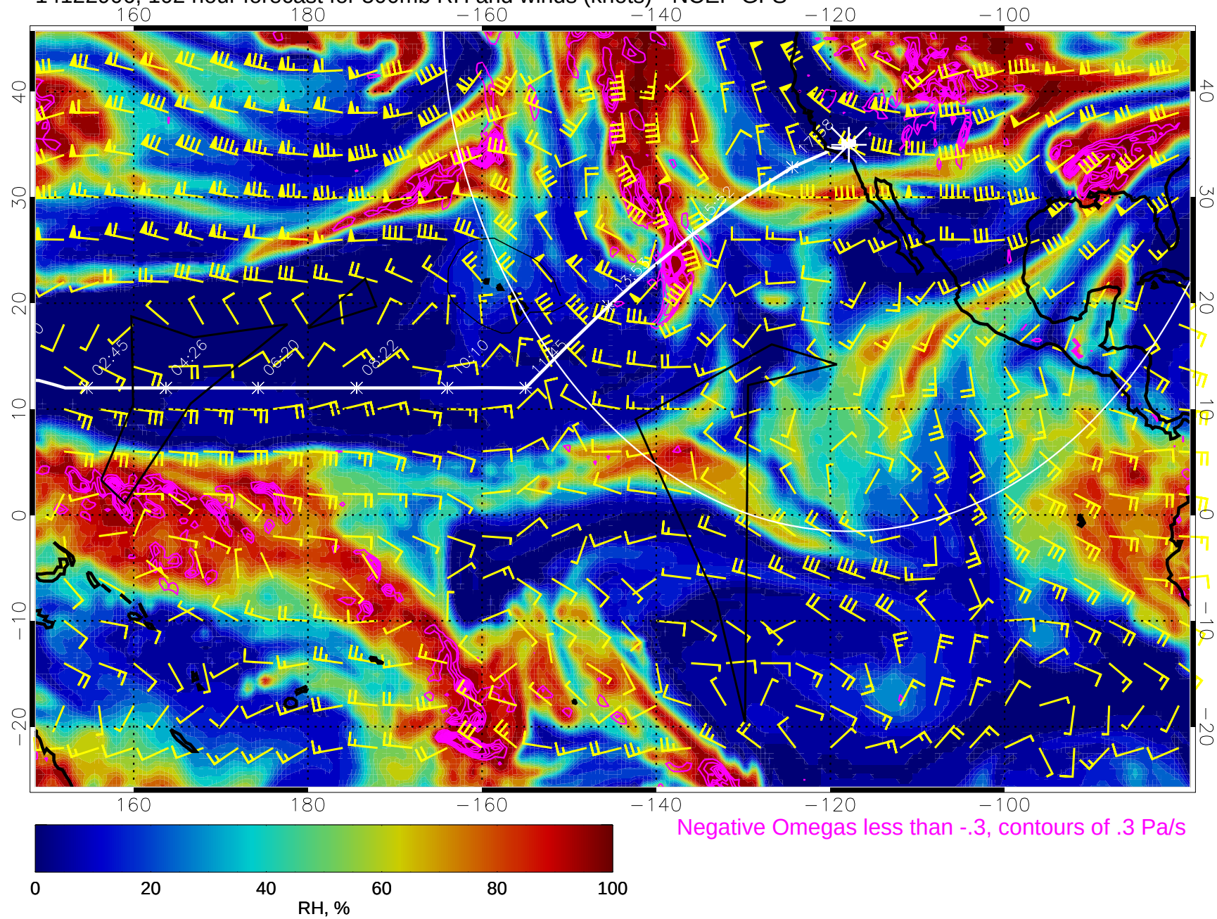
14122906, 102 hour forecast for 500mb RH and winds (knots) - NCEP GFS
