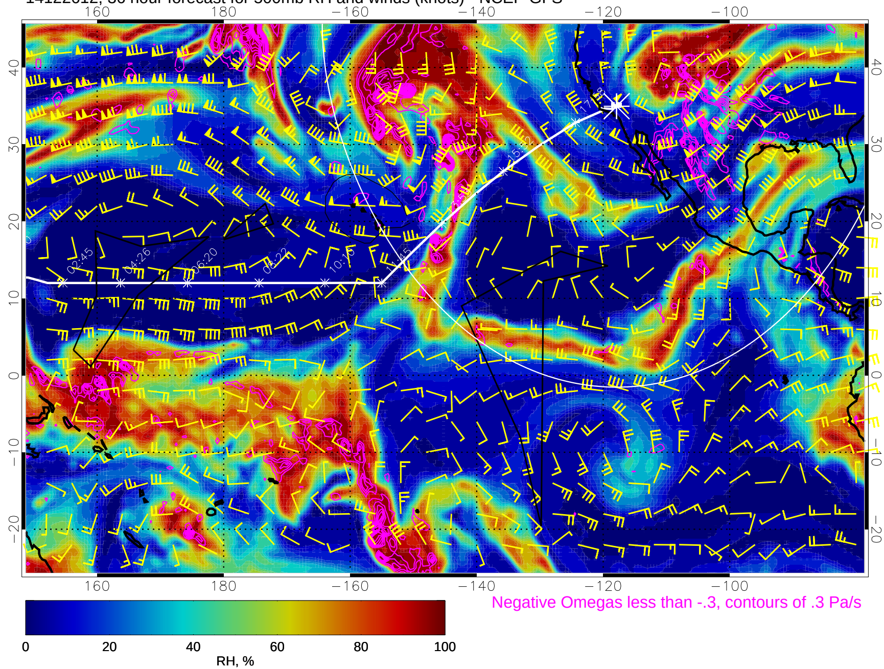
14122612, 36 hour forecast for 500mb RH and winds (knots) - NCEP GFS
