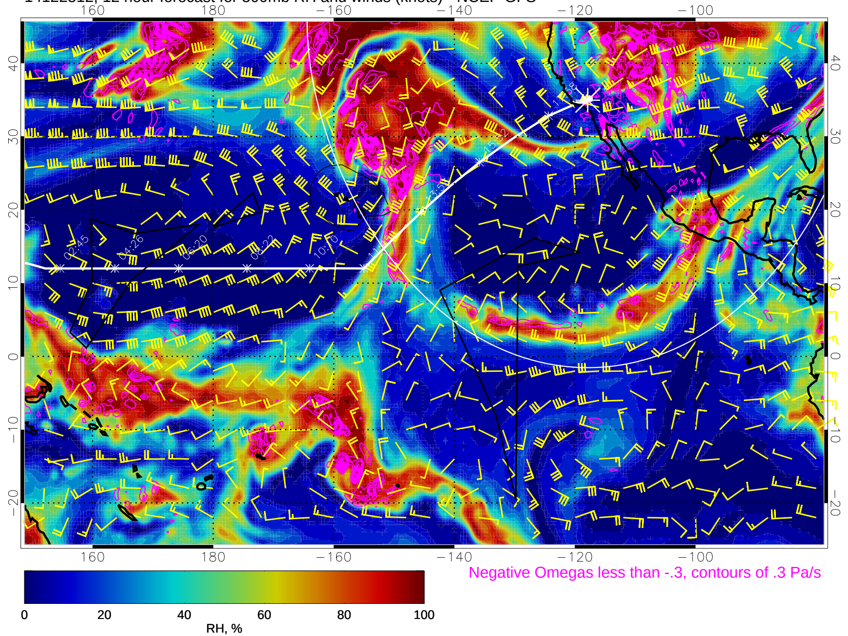
14122512, 12 hour forecast for 500mb RH and winds (knots) - NCEP GFS
