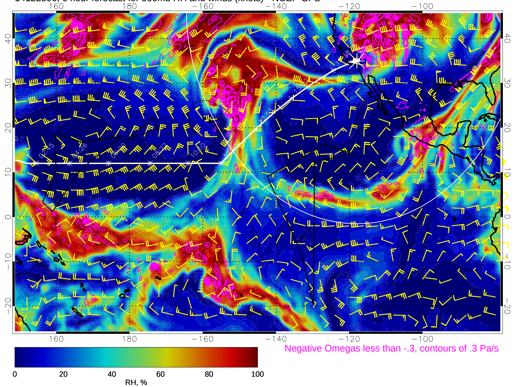
14122506, 6 hour forecast for 500mb RH and winds (knots) - NCEP GFS
