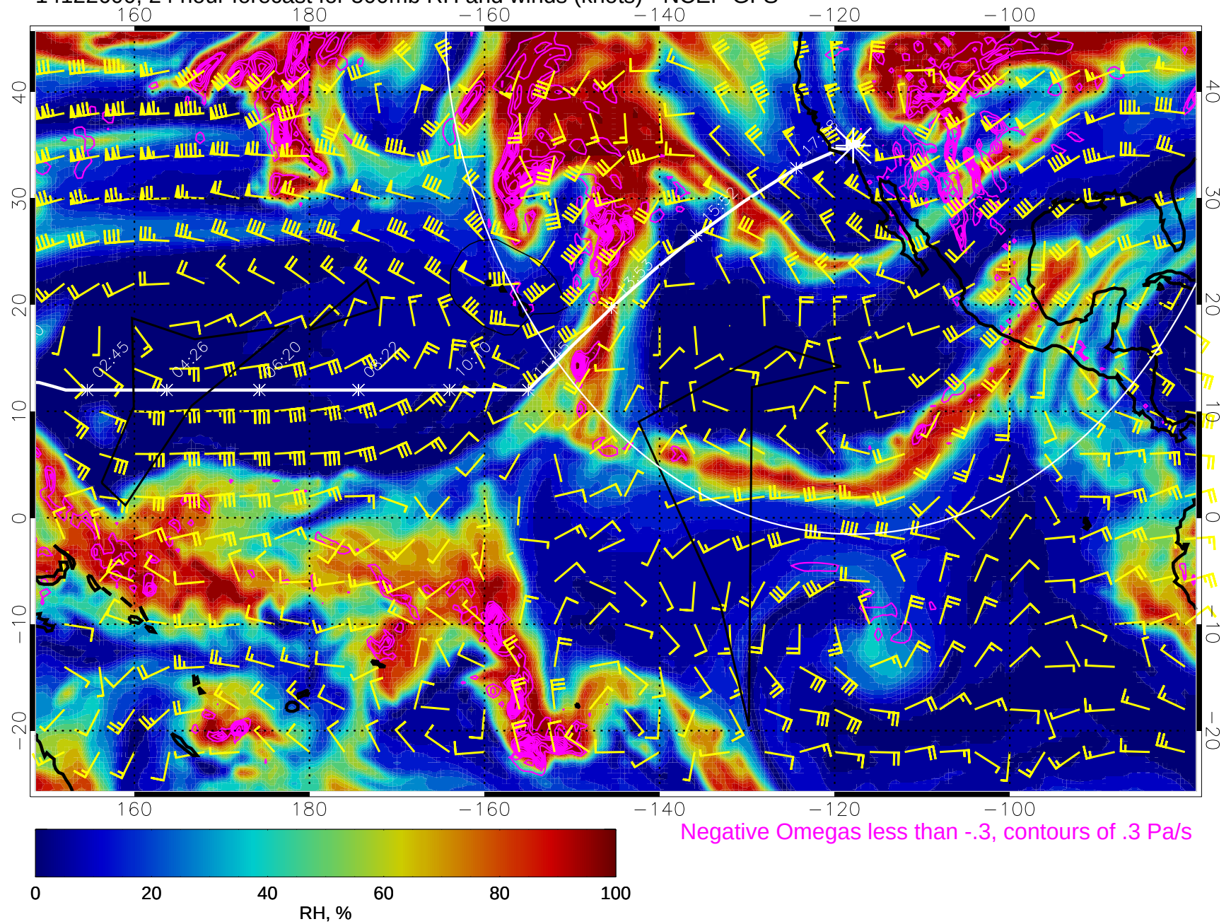
14122600, 24 hour forecast for 500mb RH and winds (knots) - NCEP GFS
