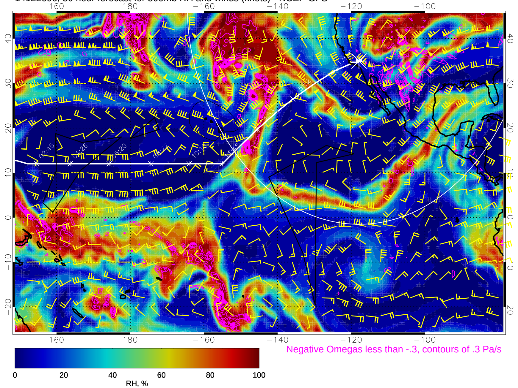
14122606, 30 hour forecast for 500mb RH and winds (knots) - NCEP GFS
