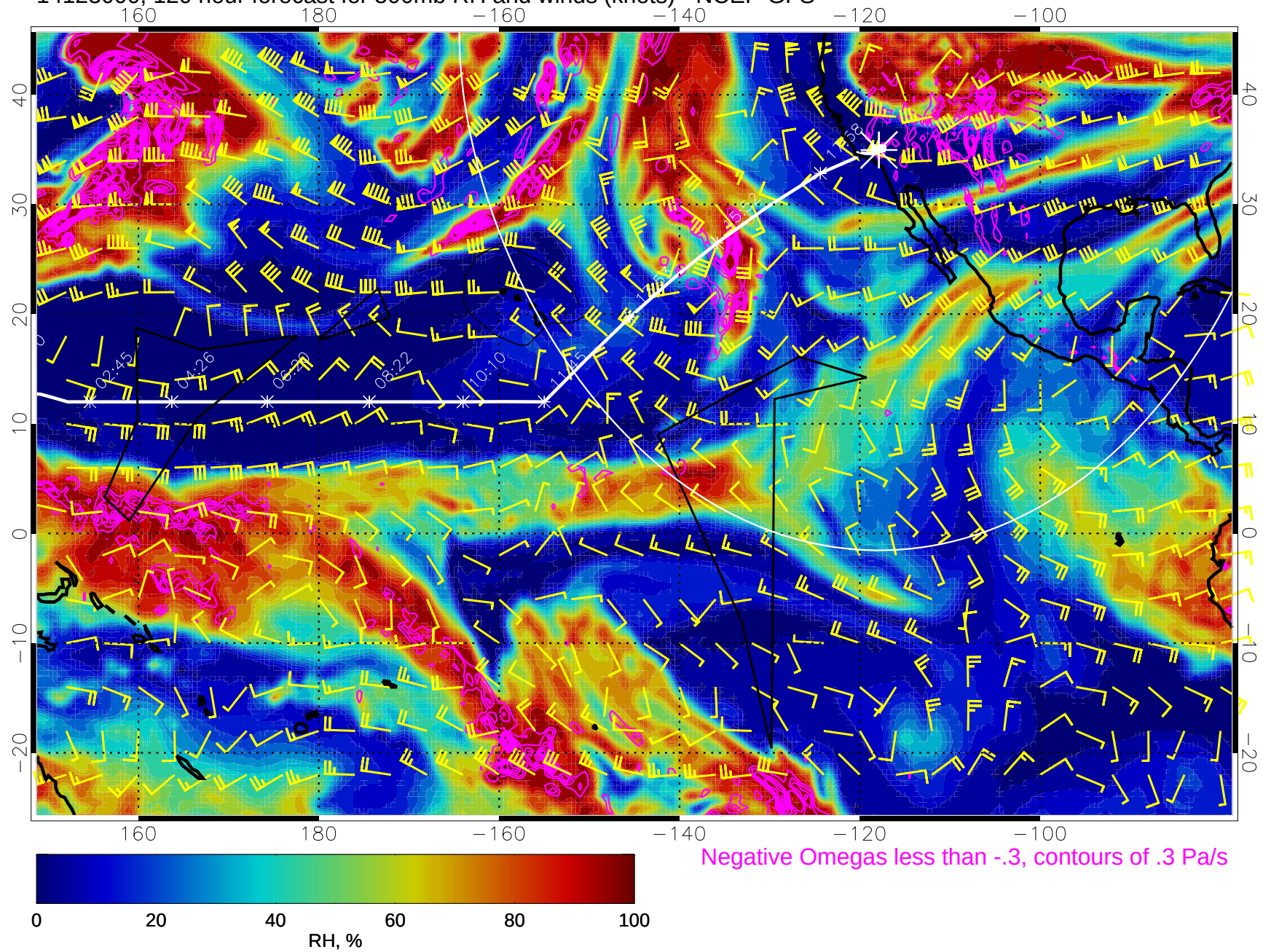
14123000, 120 hour forecast for 500mb RH and winds (knots) - NCEP GFS
