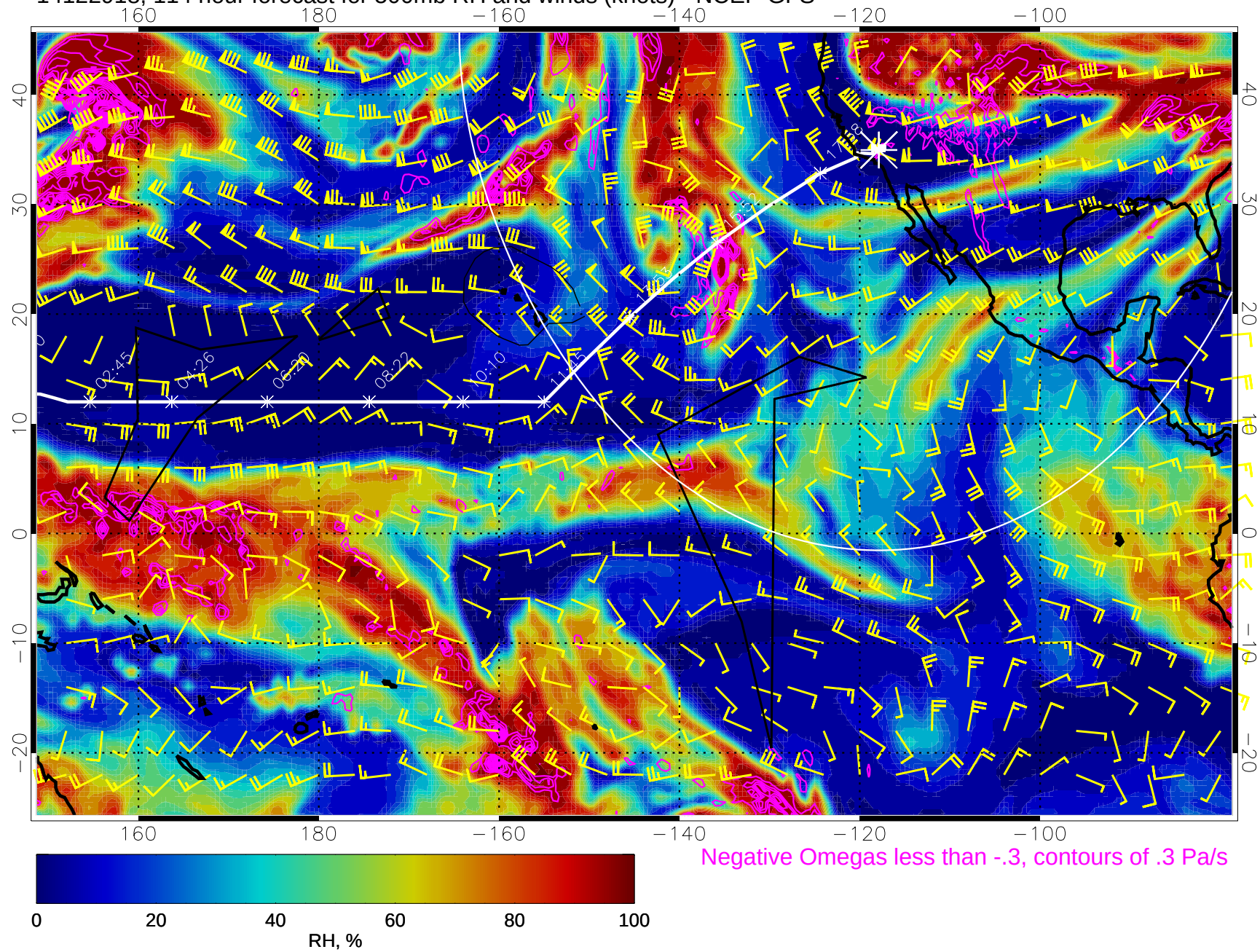
14122918, 114 hour forecast for 500mb RH and winds (knots) - NCEP GFS
