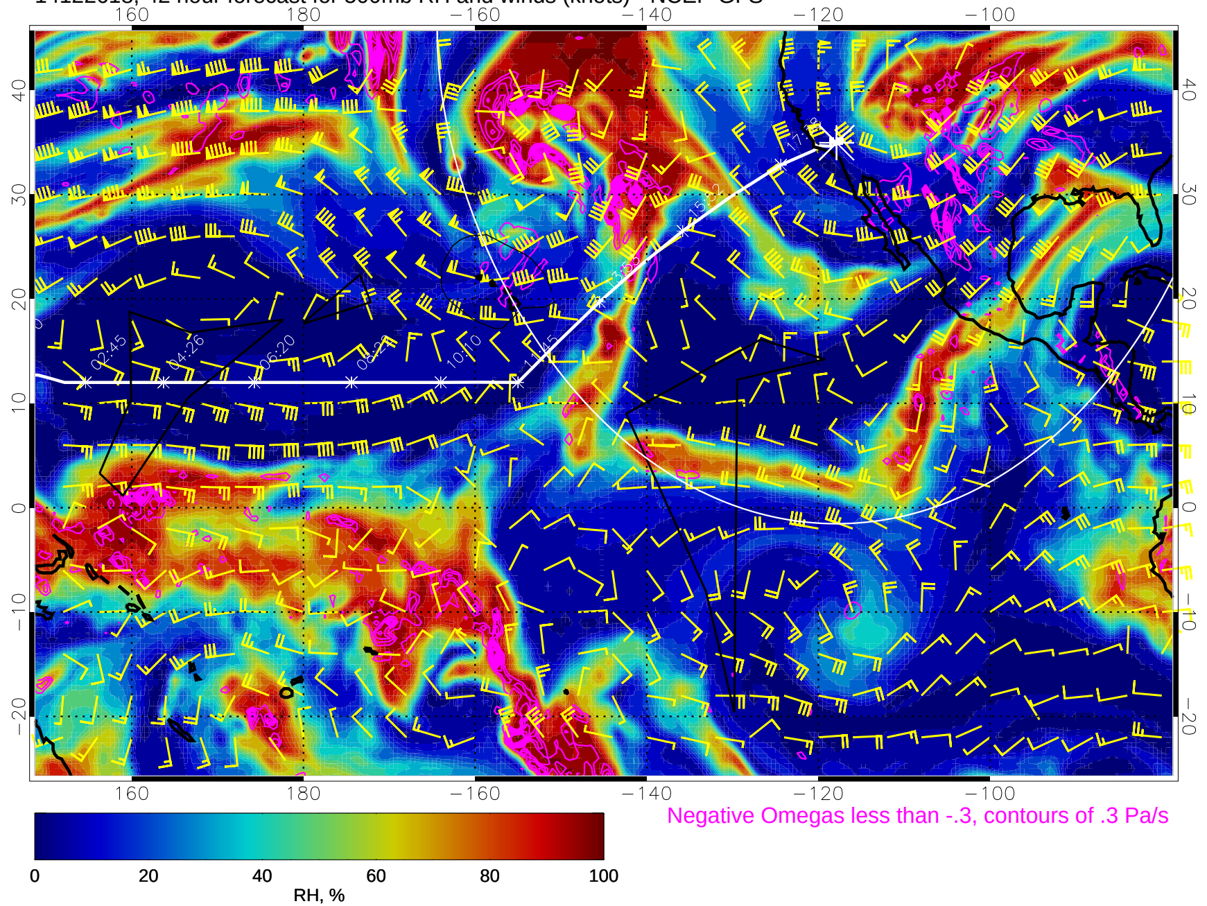
14122618, 42 hour forecast for 500mb RH and winds (knots) - NCEP GFS
