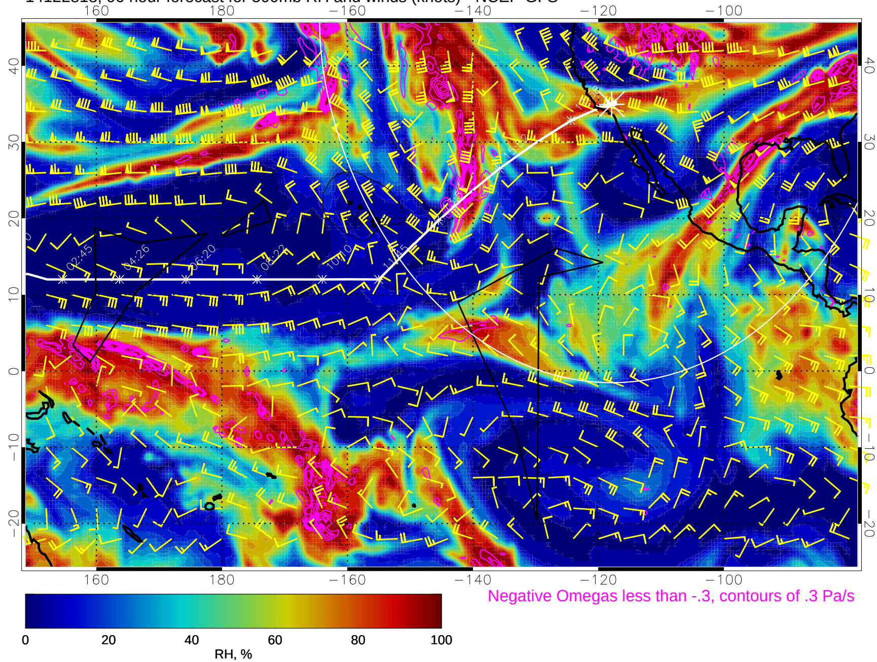
14122818, 90 hour forecast for 500mb RH and winds (knots) - NCEP GFS
