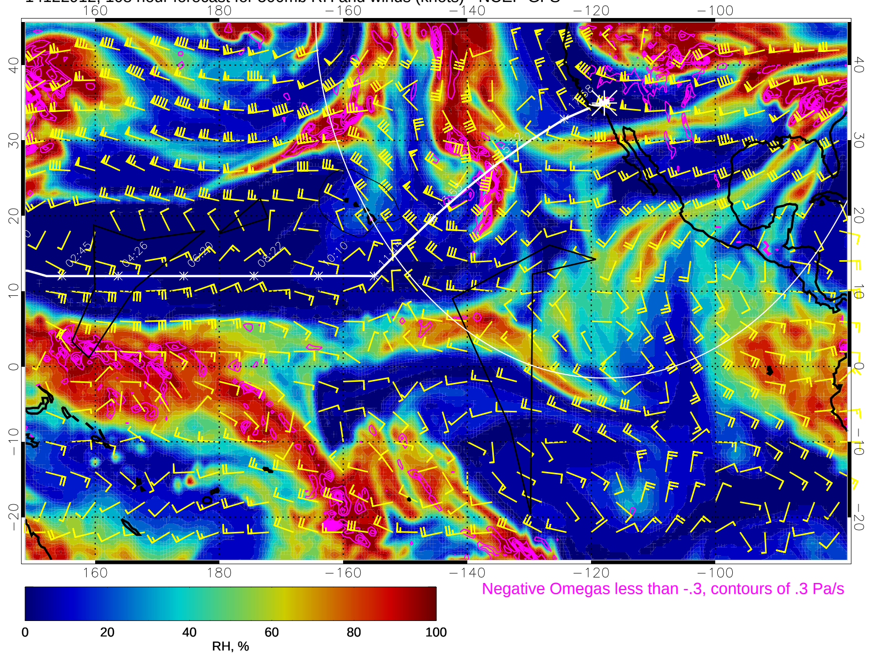
14122912, 108 hour forecast for 500mb RH and winds (knots) - NCEP GFS
