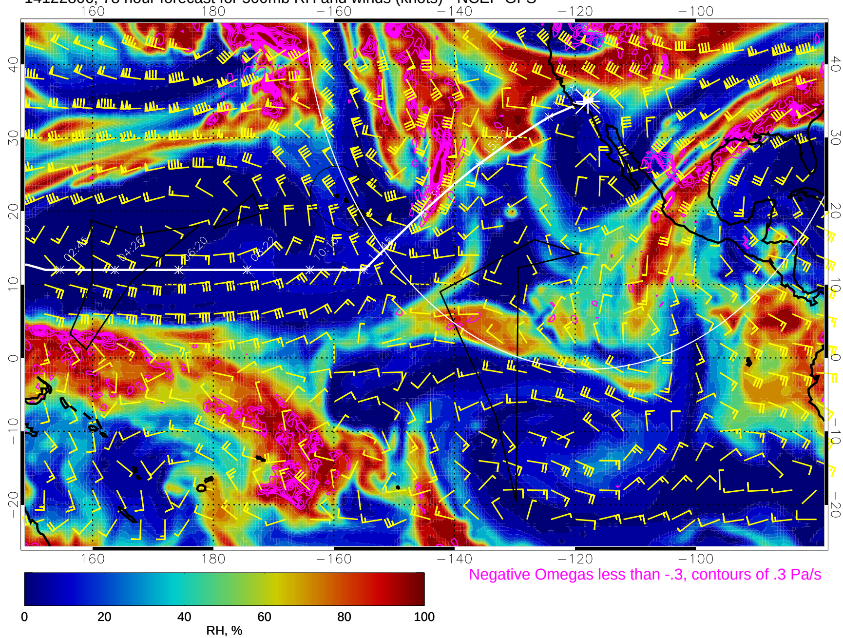
14122806, 78 hour forecast for 500mb RH and winds (knots) - NCEP GFS
