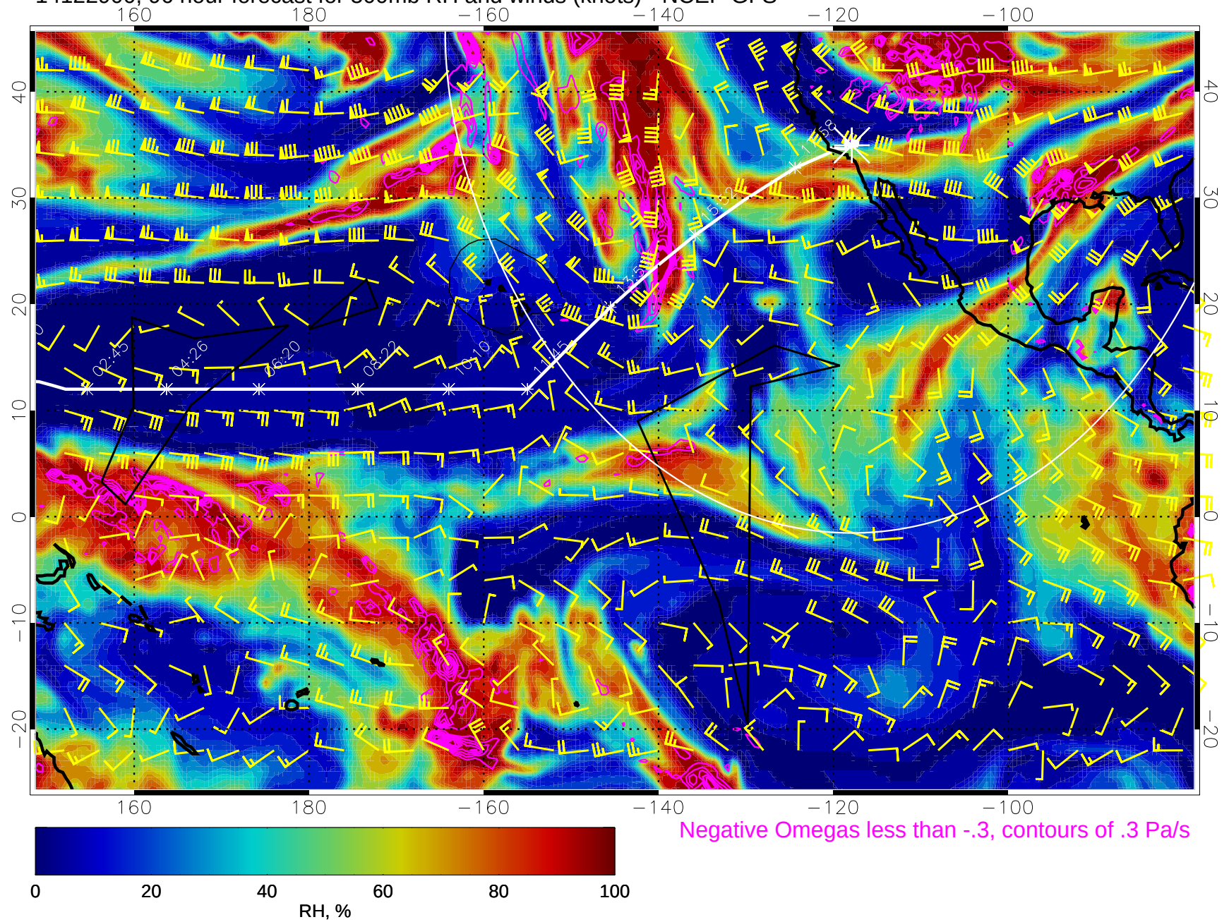
14122900, 96 hour forecast for 500mb RH and winds (knots) - NCEP GFS
