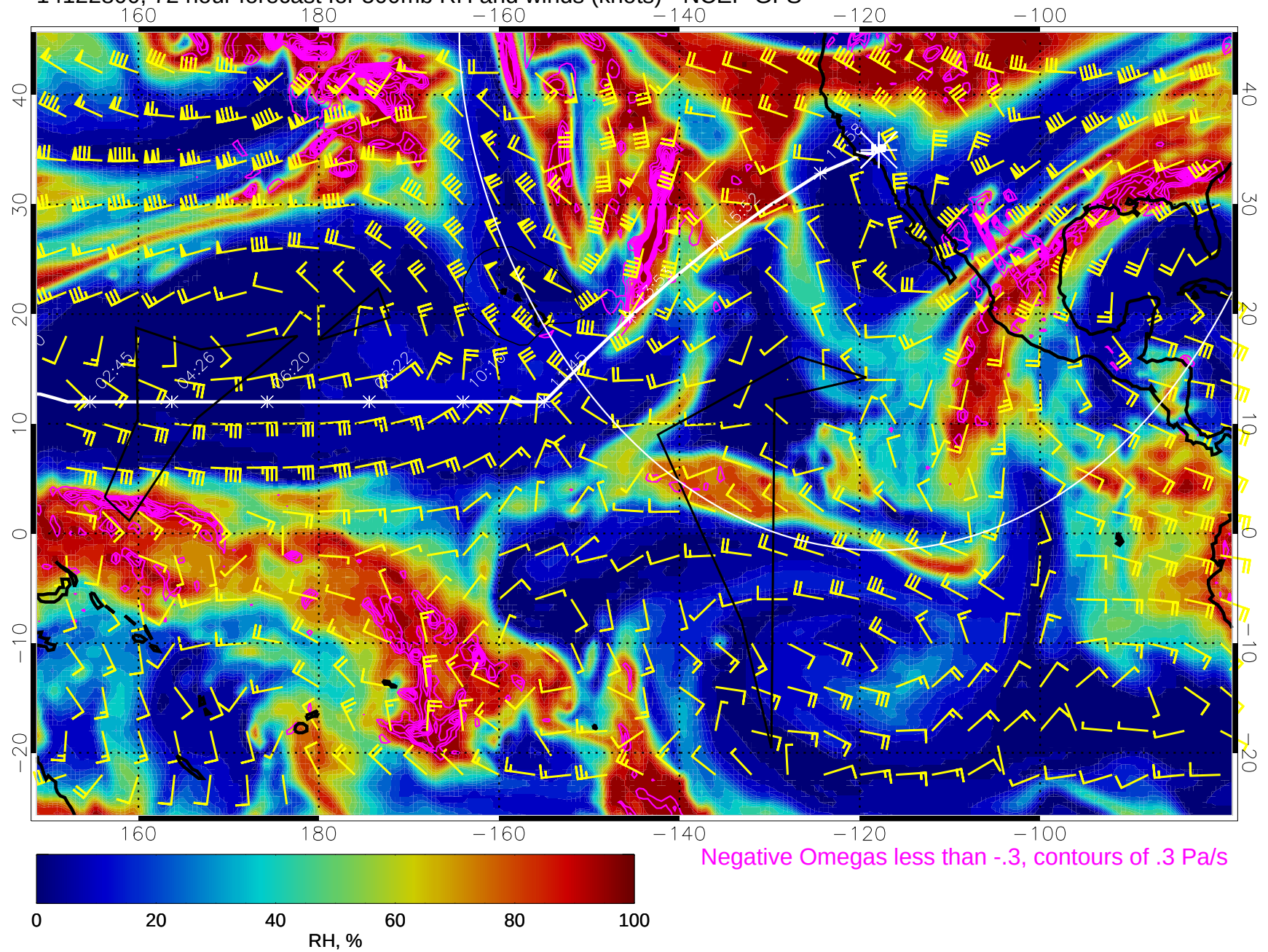
14122800, 72 hour forecast for 500mb RH and winds (knots) - NCEP GFS
