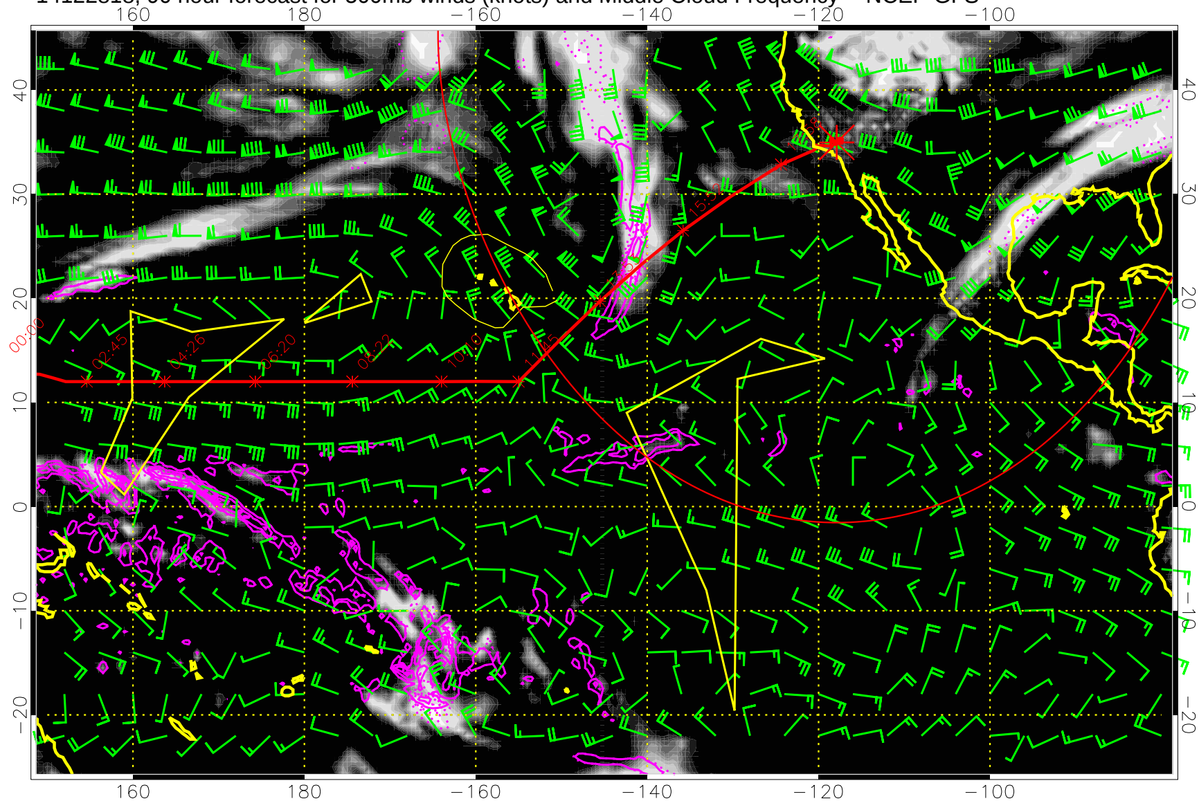
14122818, 90 hour forecast for 500mb winds (knots) and Middle Cloud Frequency -- NCEP GFS
