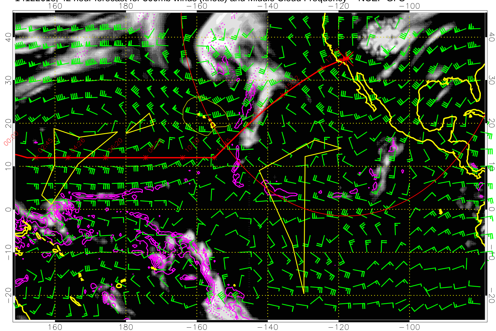
14122618, 42 hour forecast for 500mb winds (knots) and Middle Cloud Frequency -- NCEP GFS
