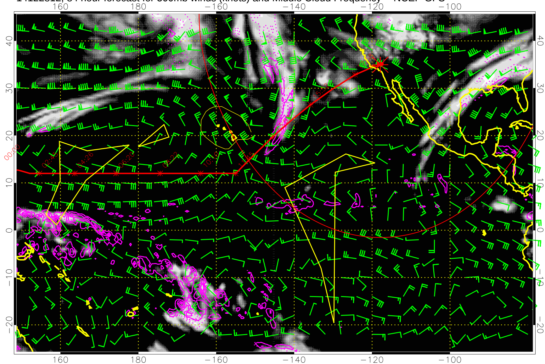
14122812, 84 hour forecast for 500mb winds (knots) and Middle Cloud Frequency -- NCEP GFS
