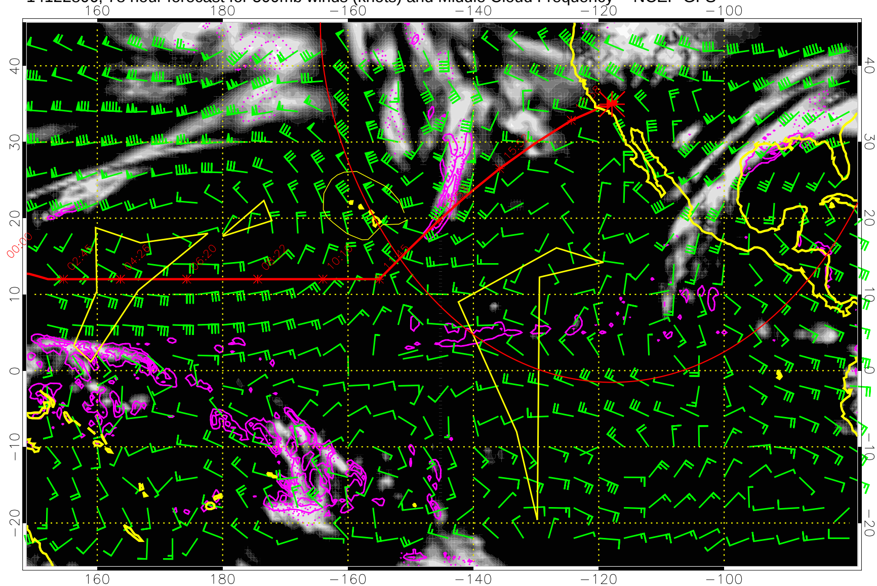
14122806, 78 hour forecast for 500mb winds (knots) and Middle Cloud Frequency -- NCEP GFS
