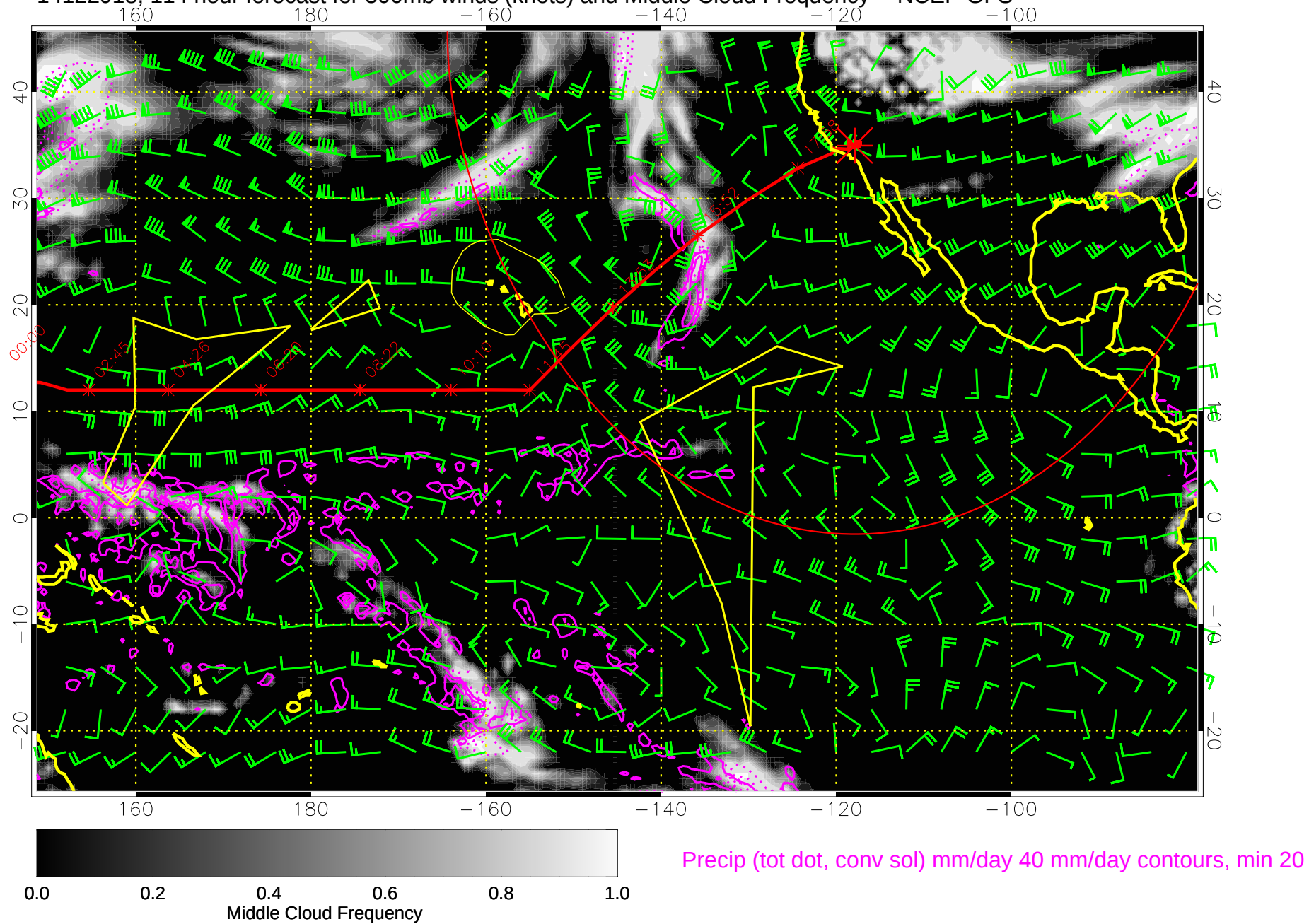
14122918, 114 hour forecast for 500mb winds (knots) and Middle Cloud Frequency -- NCEP GFS
