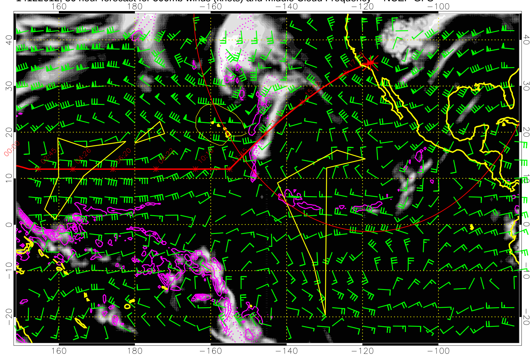
14122612, 36 hour forecast for 500mb winds (knots) and Middle Cloud Frequency -- NCEP GFS
