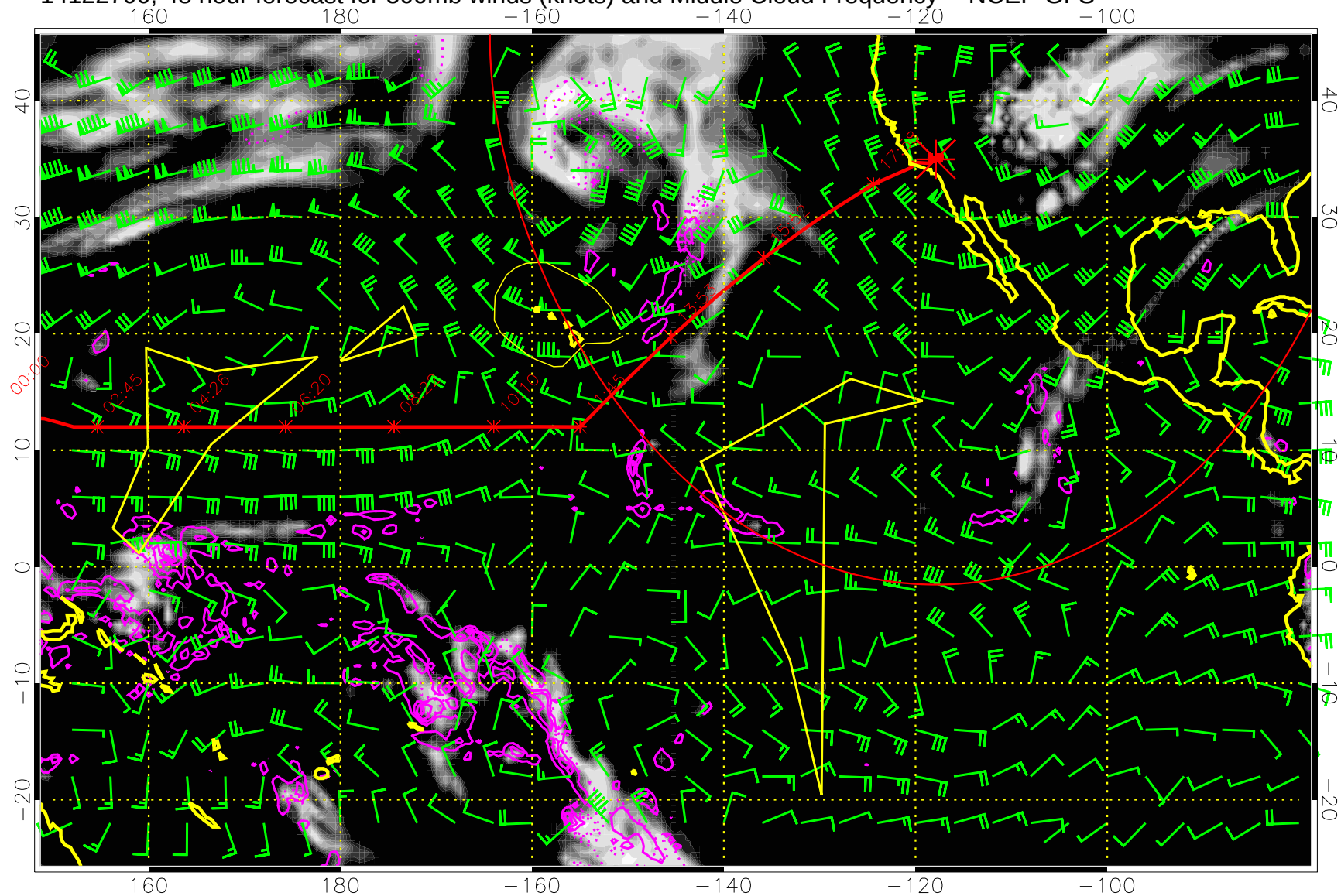
14122700, 48 hour forecast for 500mb winds (knots) and Middle Cloud Frequency -- NCEP GFS
