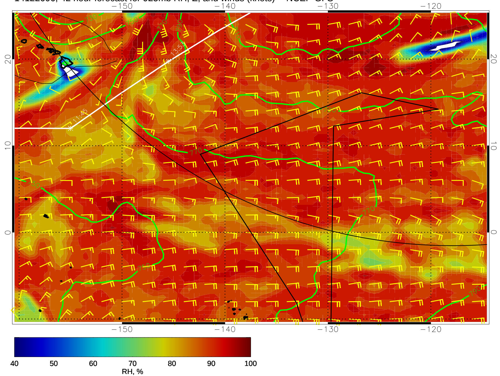
14122606, 42 hour forecast for 925mb RH, Z, and winds (knots) -- NCEP GFS
