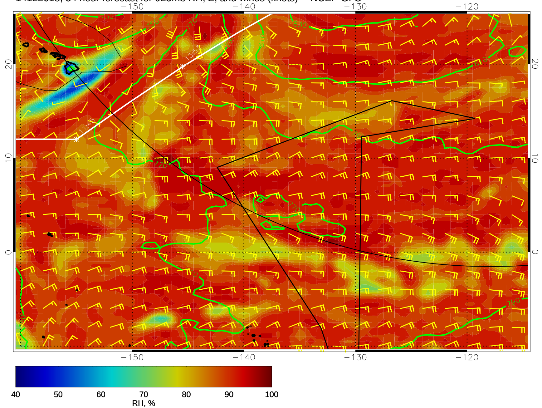
14122618, 54 hour forecast for 925mb RH, Z, and winds (knots) -- NCEP GFS
