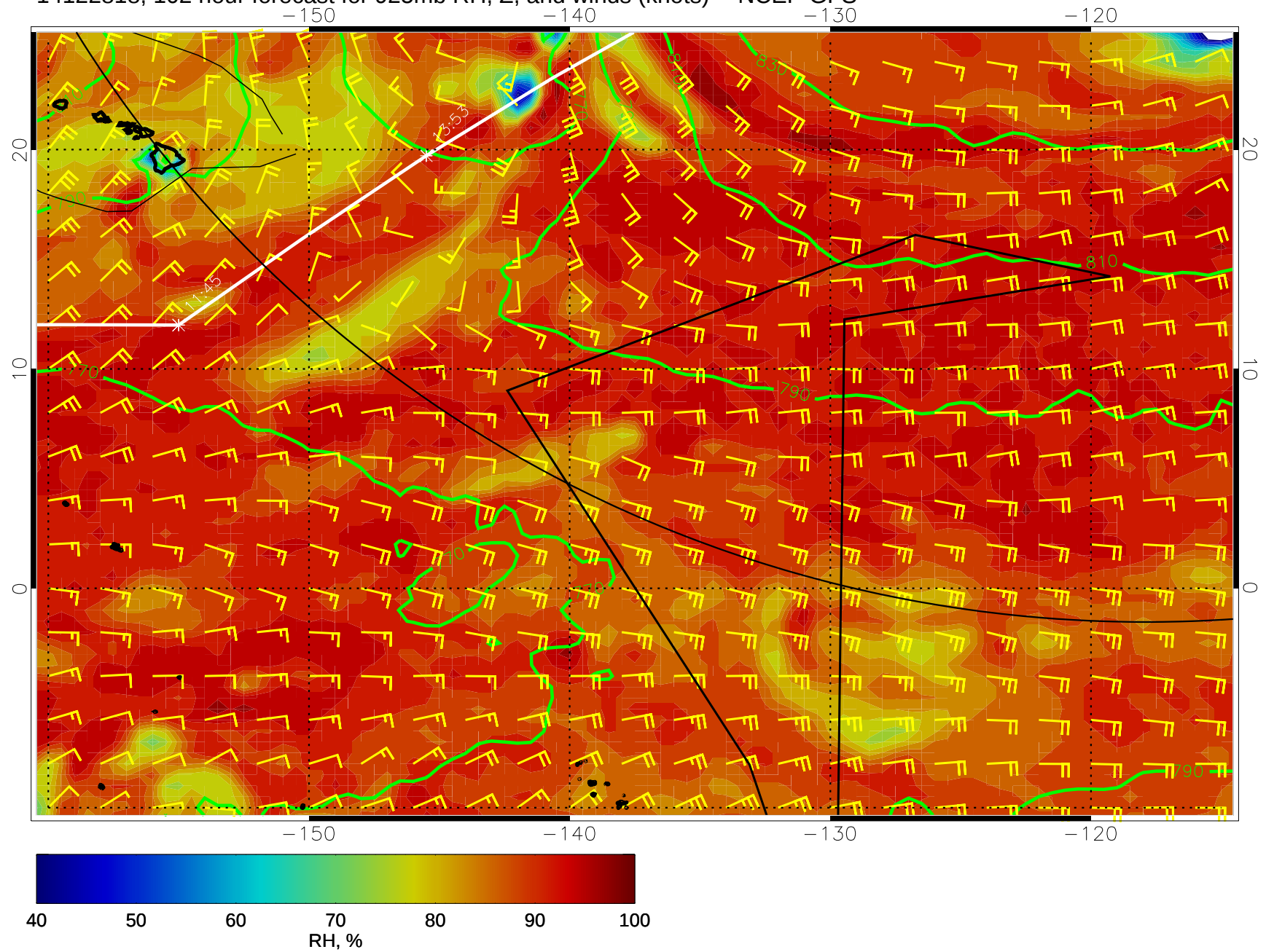
14122818, 102 hour forecast for 925mb RH, Z, and winds (knots) -- NCEP GFS
