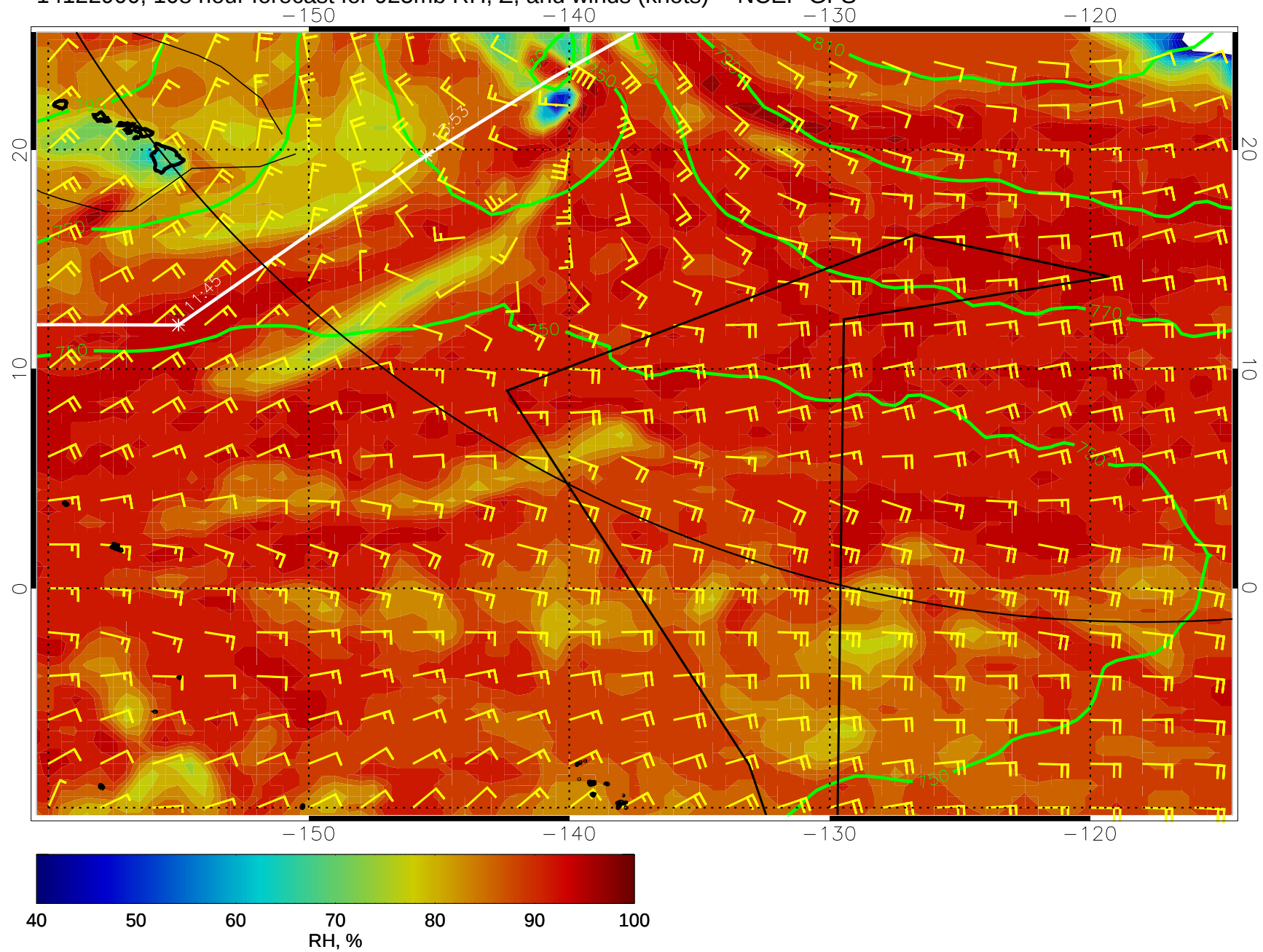
14122900, 108 hour forecast for 925mb RH, Z, and winds (knots) -- NCEP GFS
