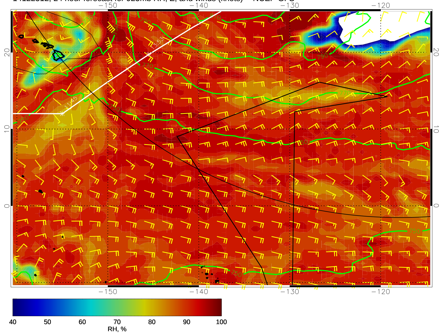
14122512, 24 hour forecast for 925mb RH, Z, and winds (knots) -- NCEP GFS
