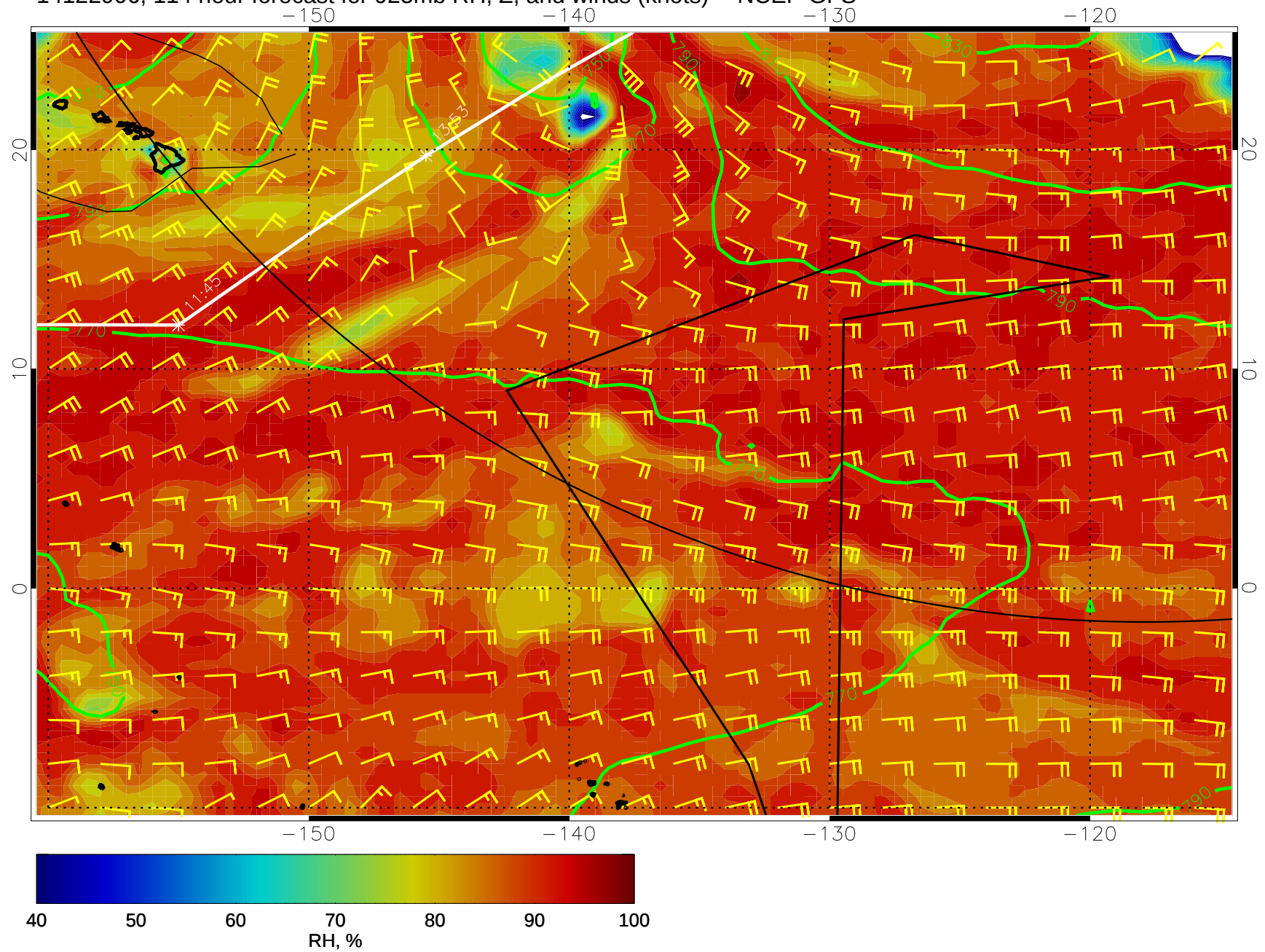
14122906, 114 hour forecast for 925mb RH, Z, and winds (knots) -- NCEP GFS
