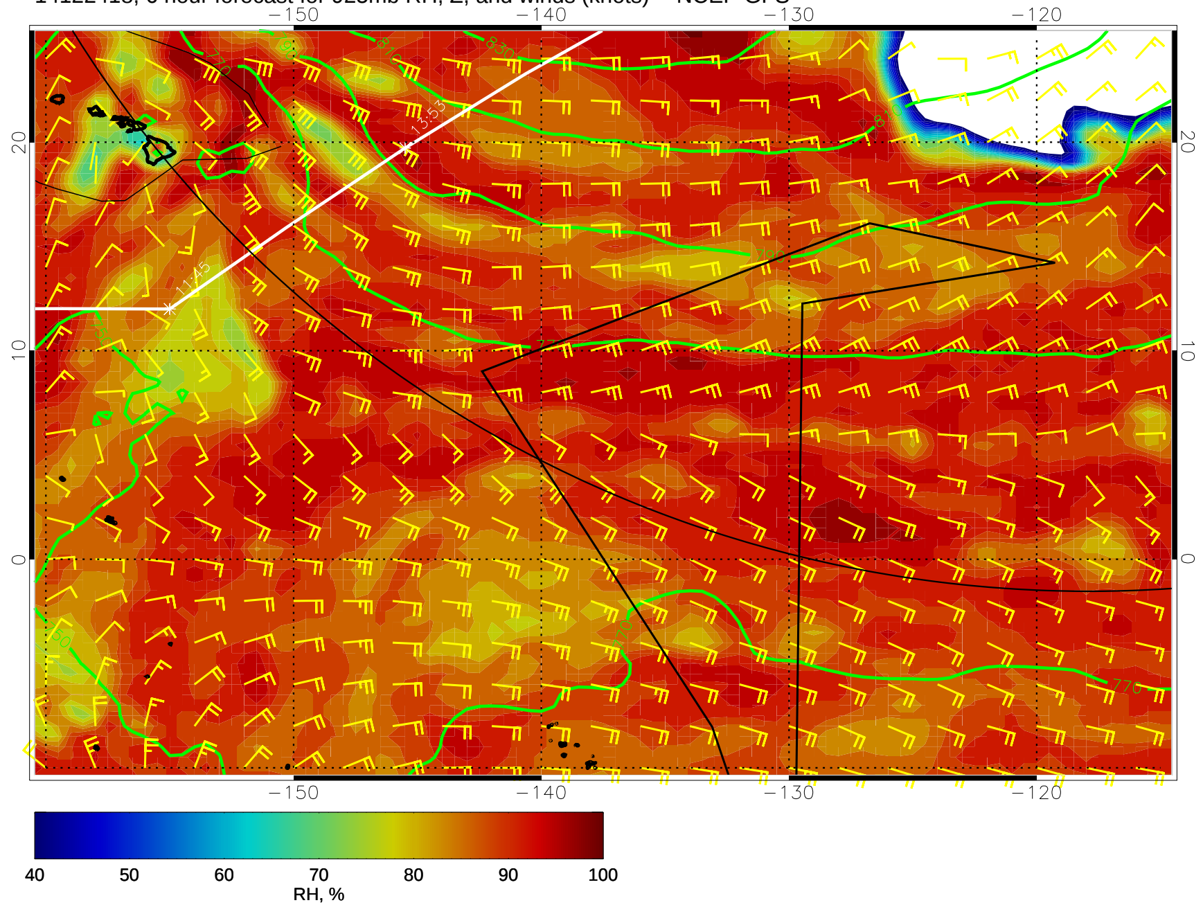
14122418, 6 hour forecast for 925mb RH, Z, and winds (knots) -- NCEP GFS
