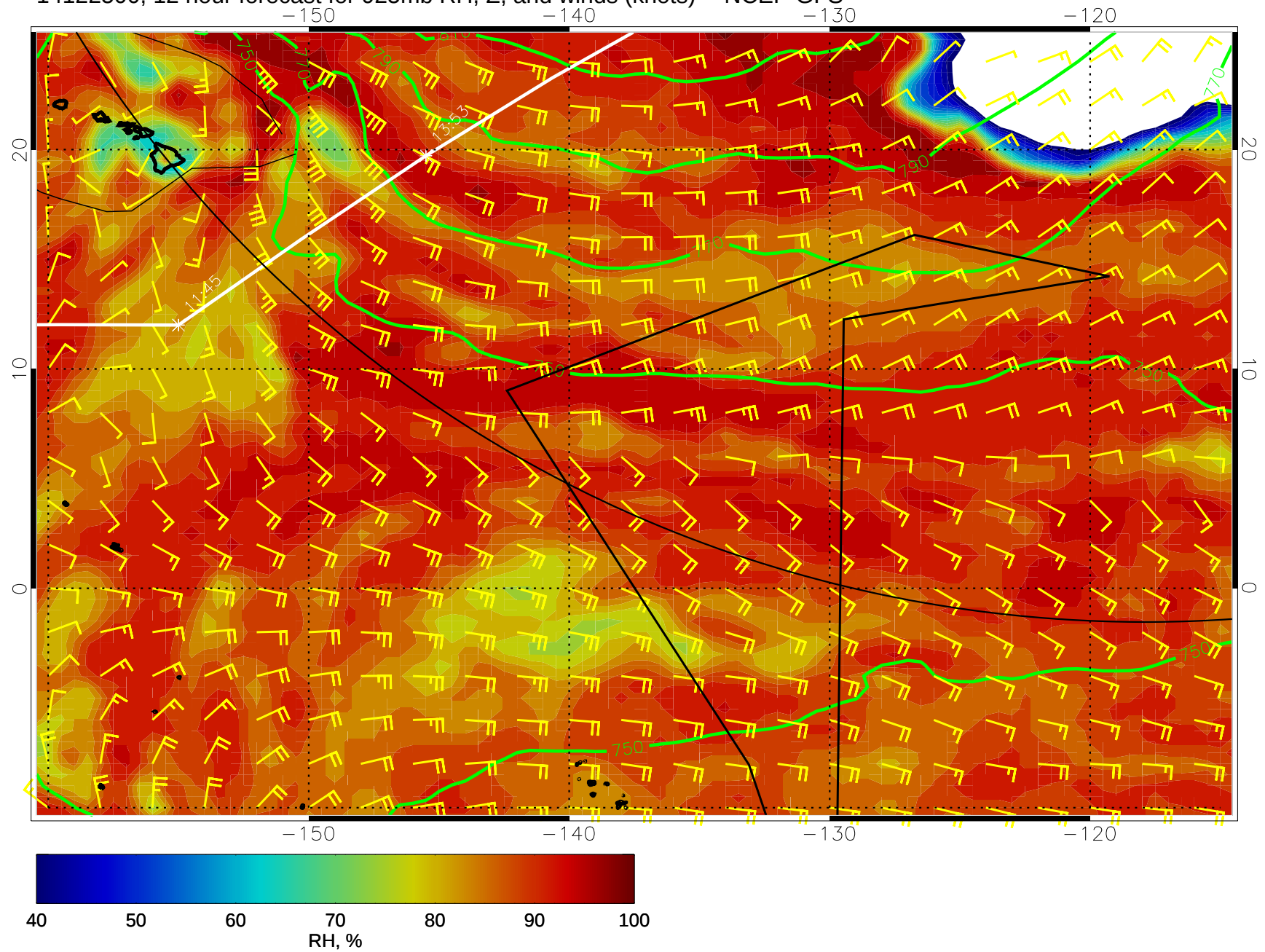
14122500, 12 hour forecast for 925mb RH, Z, and winds (knots) -- NCEP GFS
