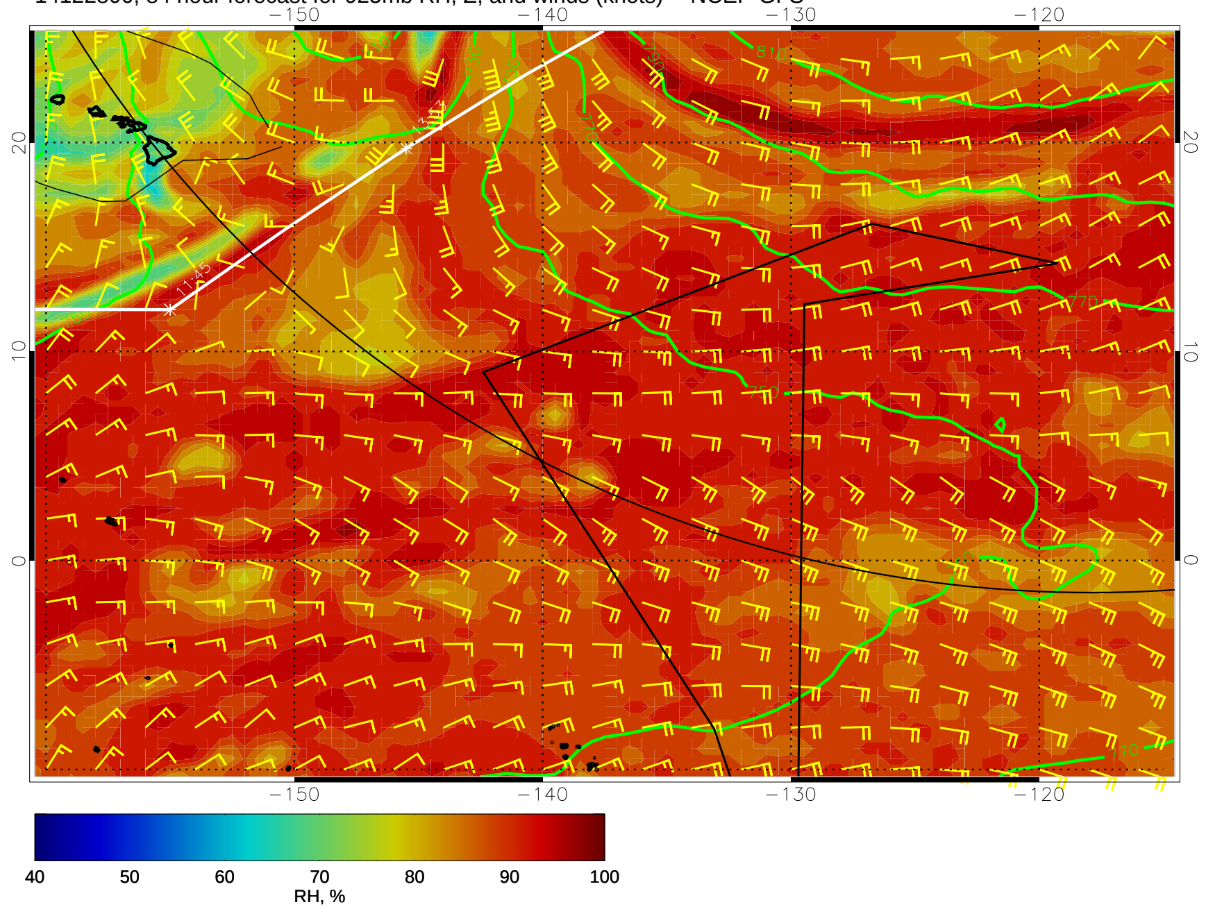
14122800, 84 hour forecast for 925mb RH, Z, and winds (knots) -- NCEP GFS
