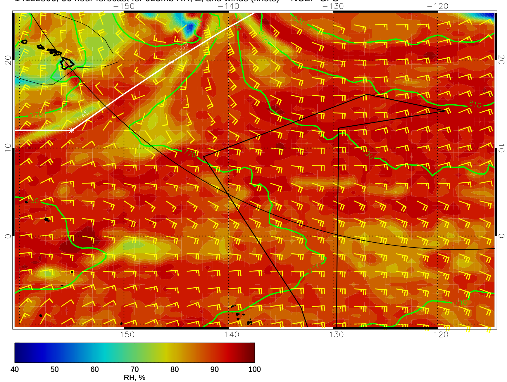
14122806, 90 hour forecast for 925mb RH, Z, and winds (knots) -- NCEP GFS
