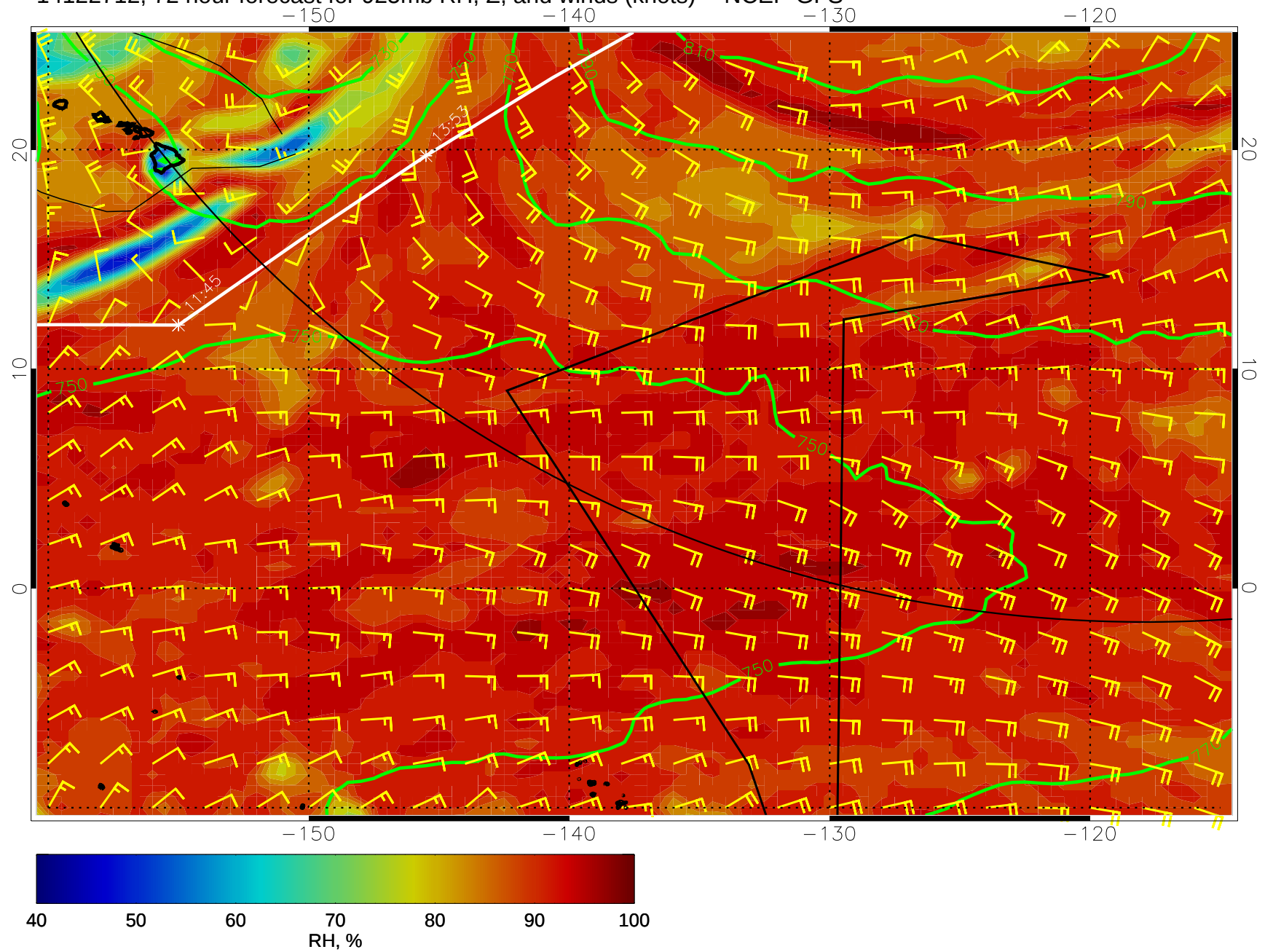
14122712, 72 hour forecast for 925mb RH, Z, and winds (knots) -- NCEP GFS
