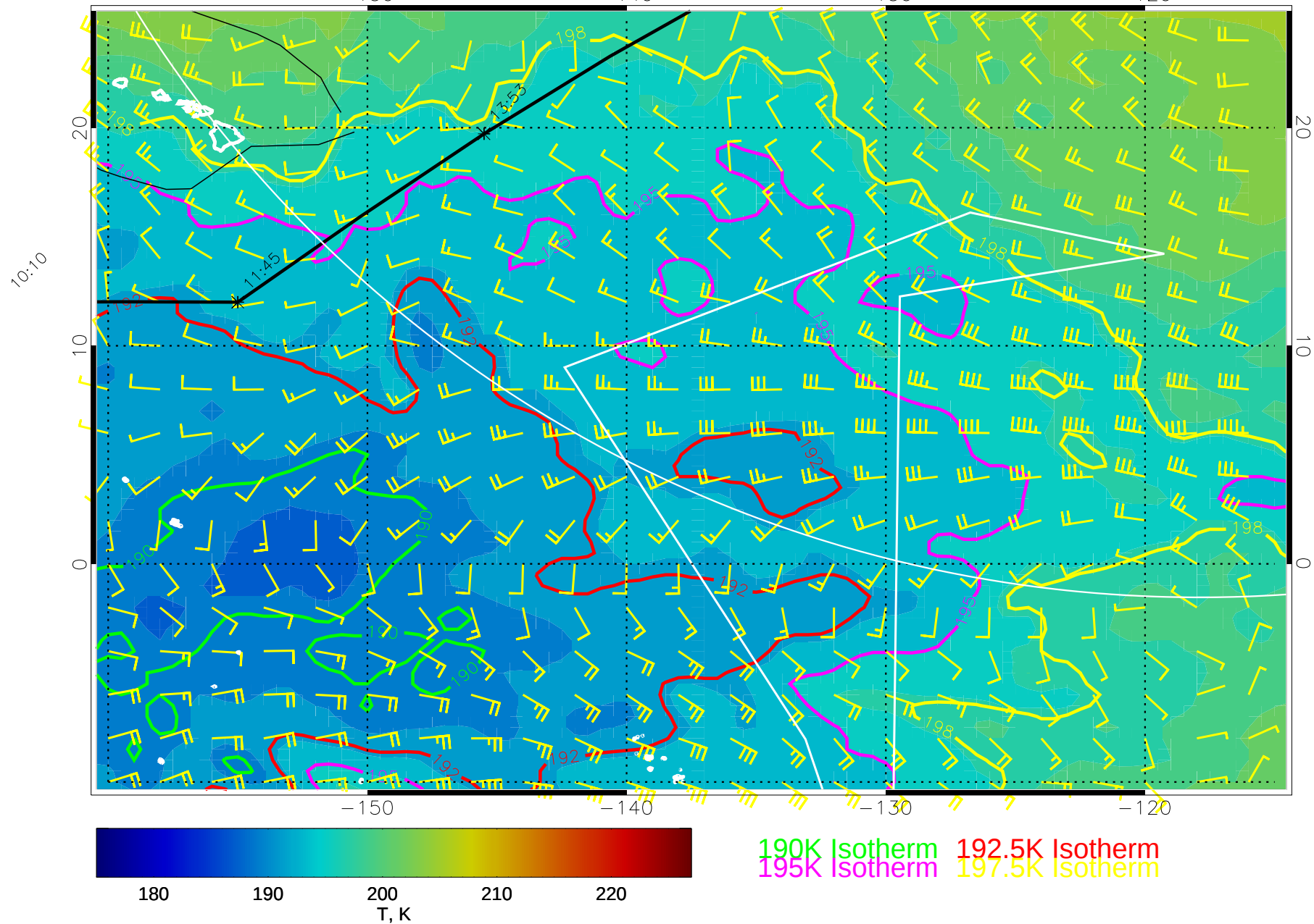
14122618, 54 hour forecast for 70mb T and winds (knots) -- NCEP GFS
