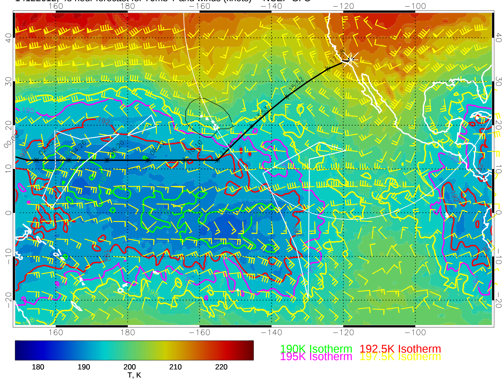
14122612, 48 hour forecast for 70mb T and winds (knots) -- NCEP GFS
