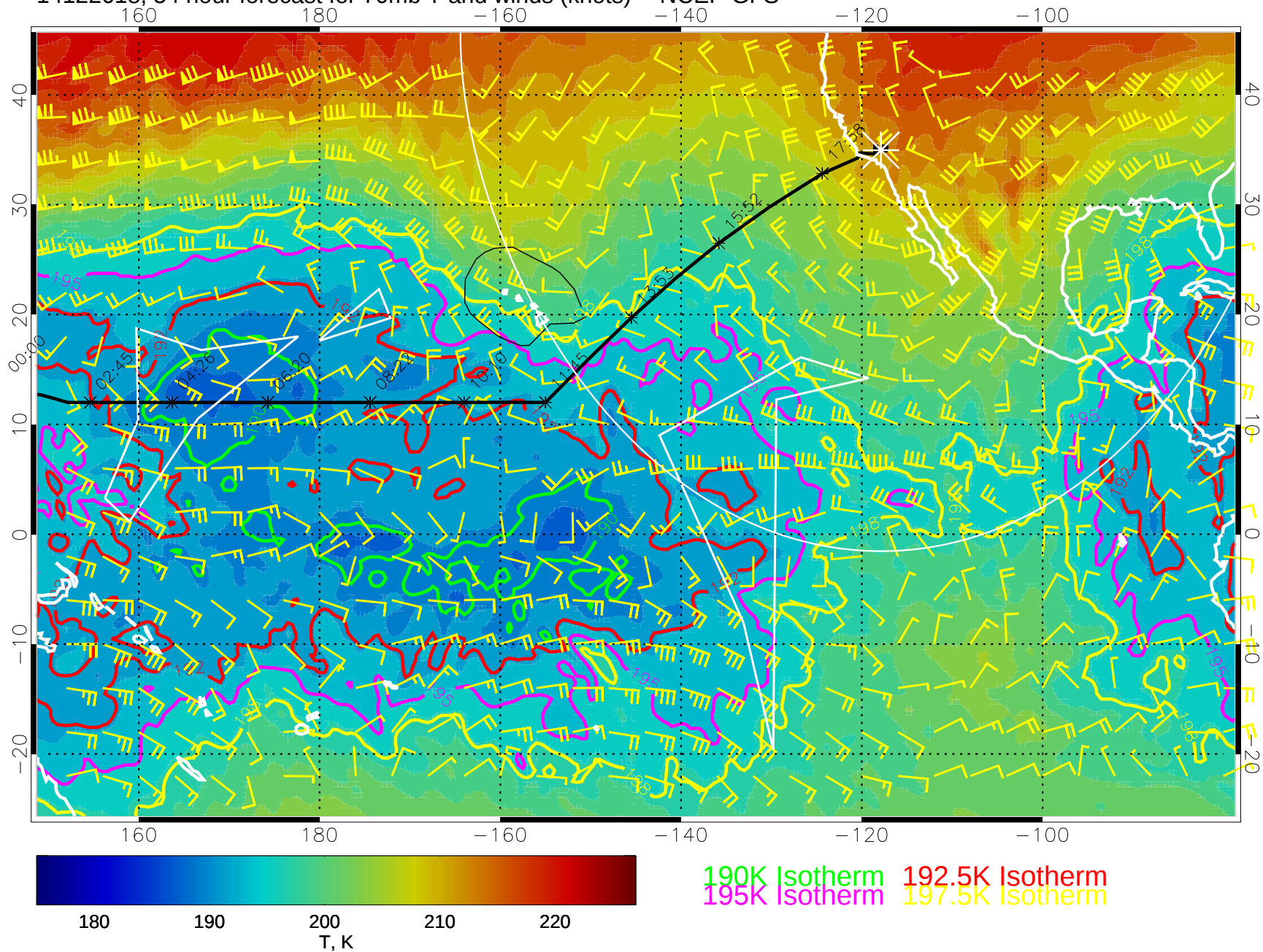
14122618, 54 hour forecast for 70mb T and winds (knots) -- NCEP GFS
