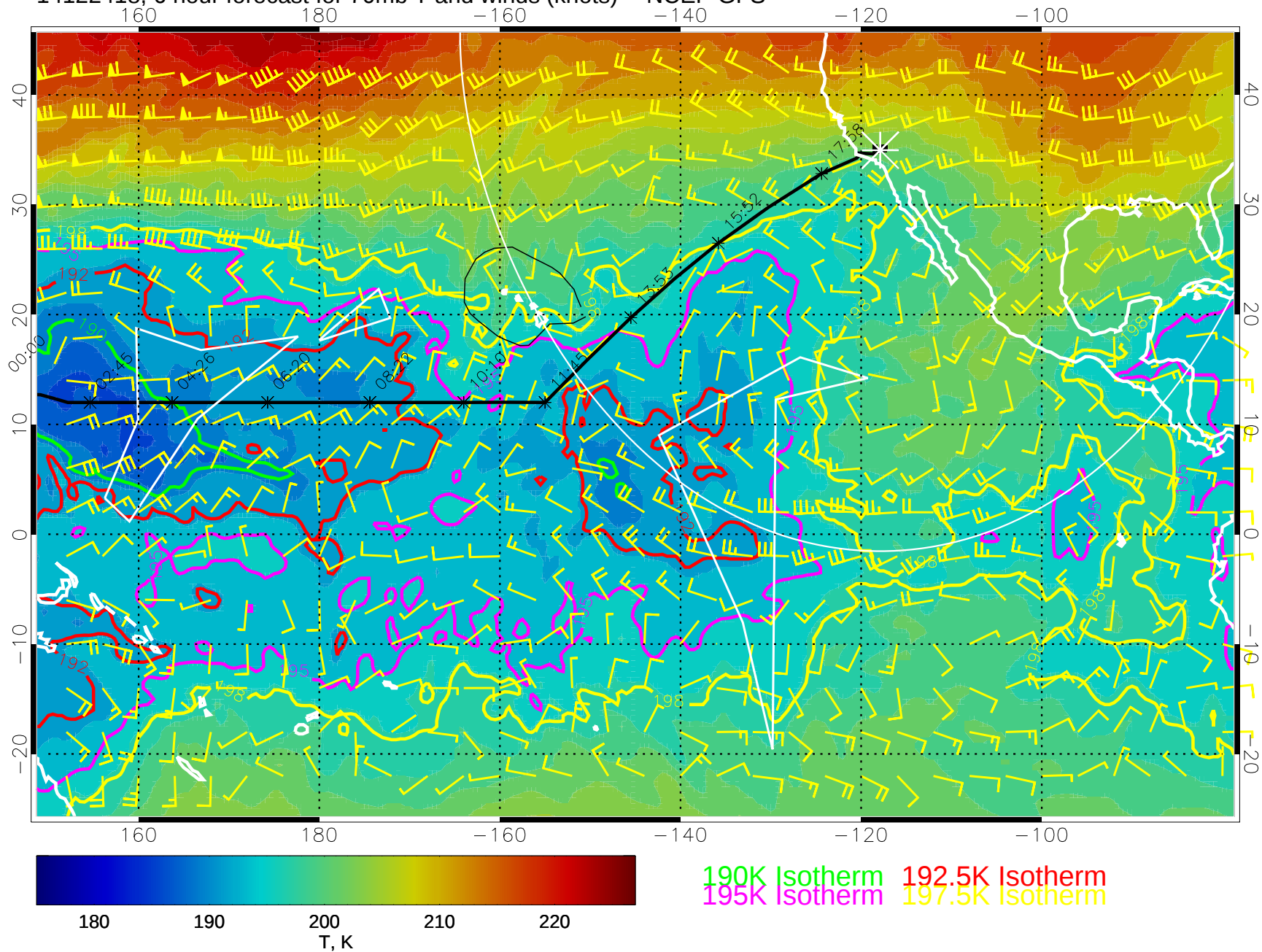
14122418, 6 hour forecast for 70mb T and winds (knots) -- NCEP GFS
