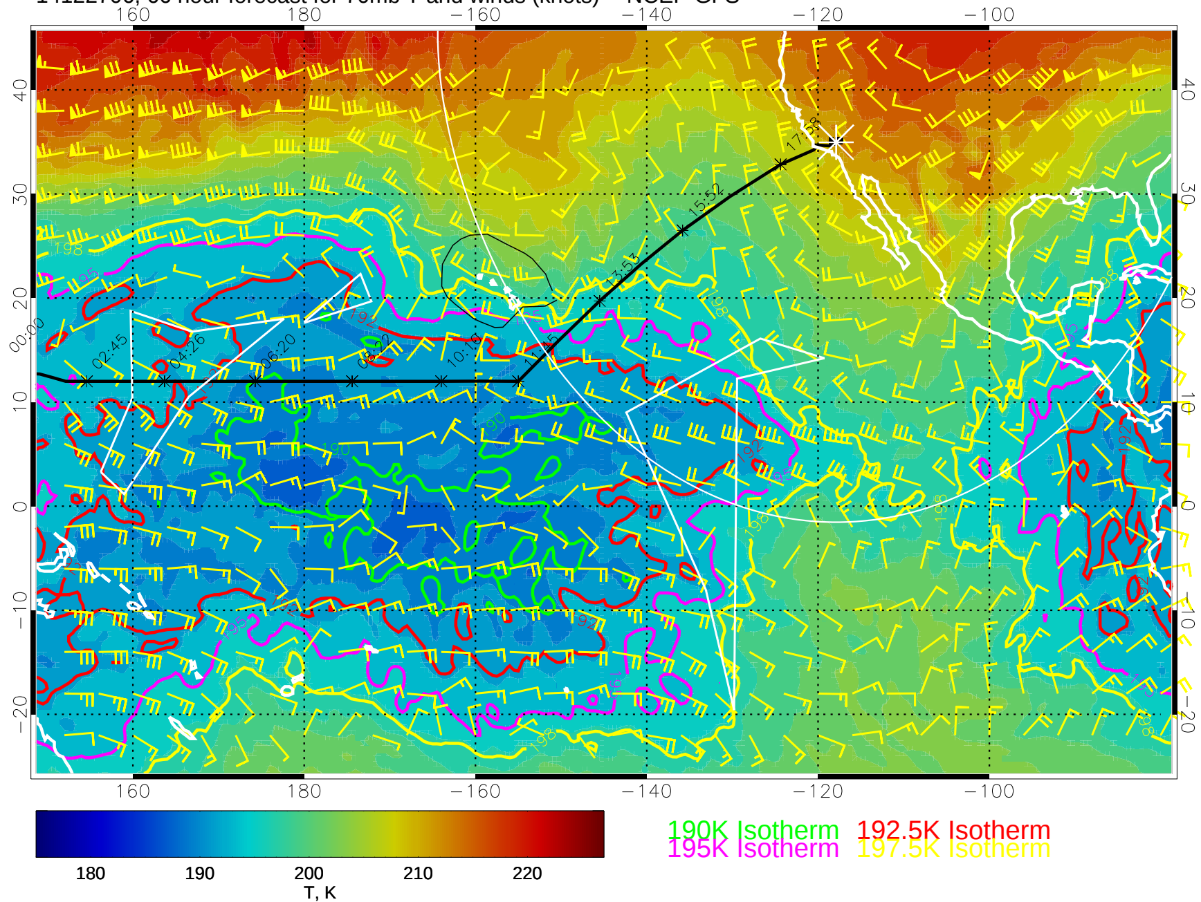
14122706, 66 hour forecast for 70mb T and winds (knots) -- NCEP GFS
