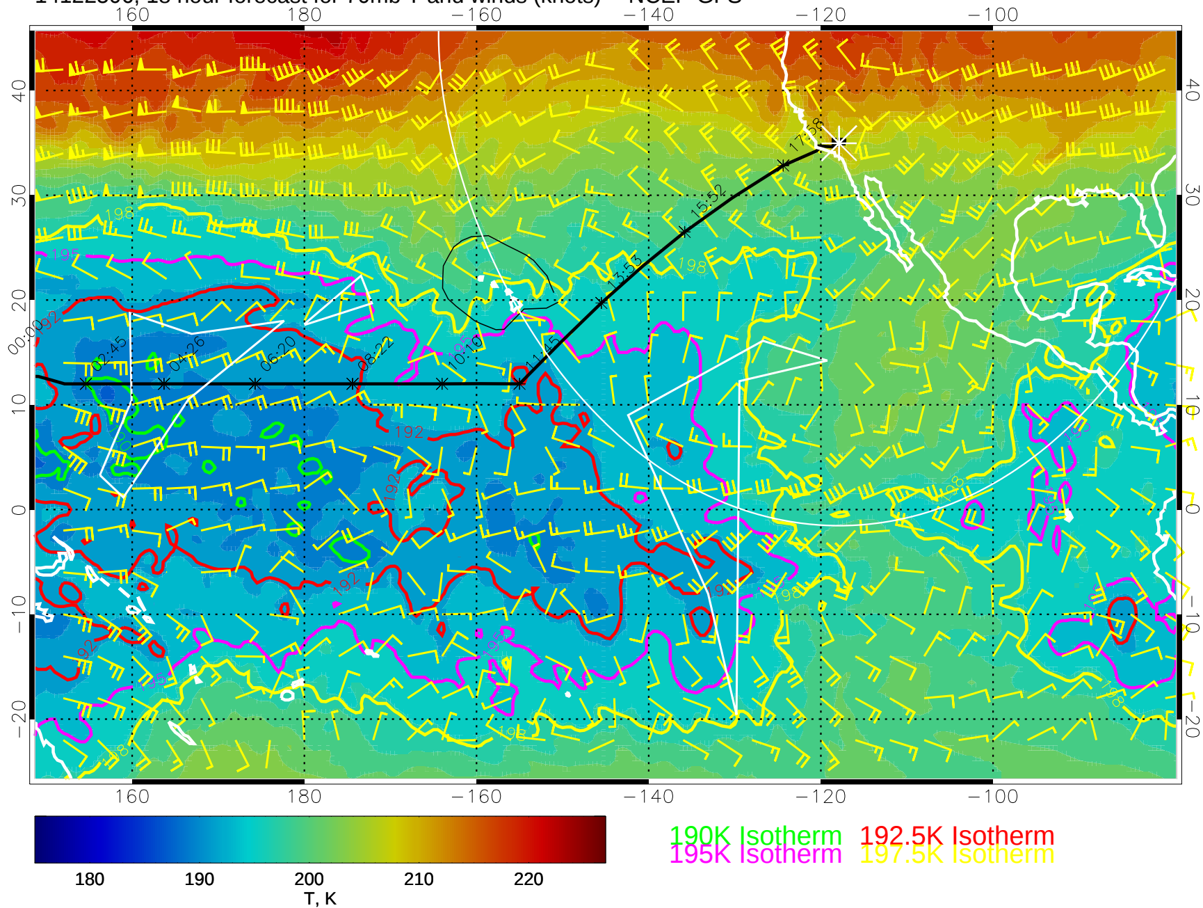
14122506, 18 hour forecast for 70mb T and winds (knots) -- NCEP GFS
