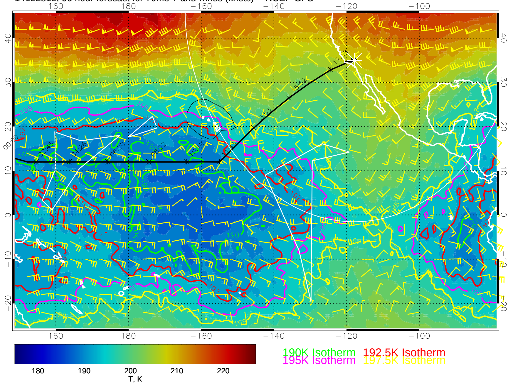
14122812, 96 hour forecast for 70mb T and winds (knots) -- NCEP GFS
