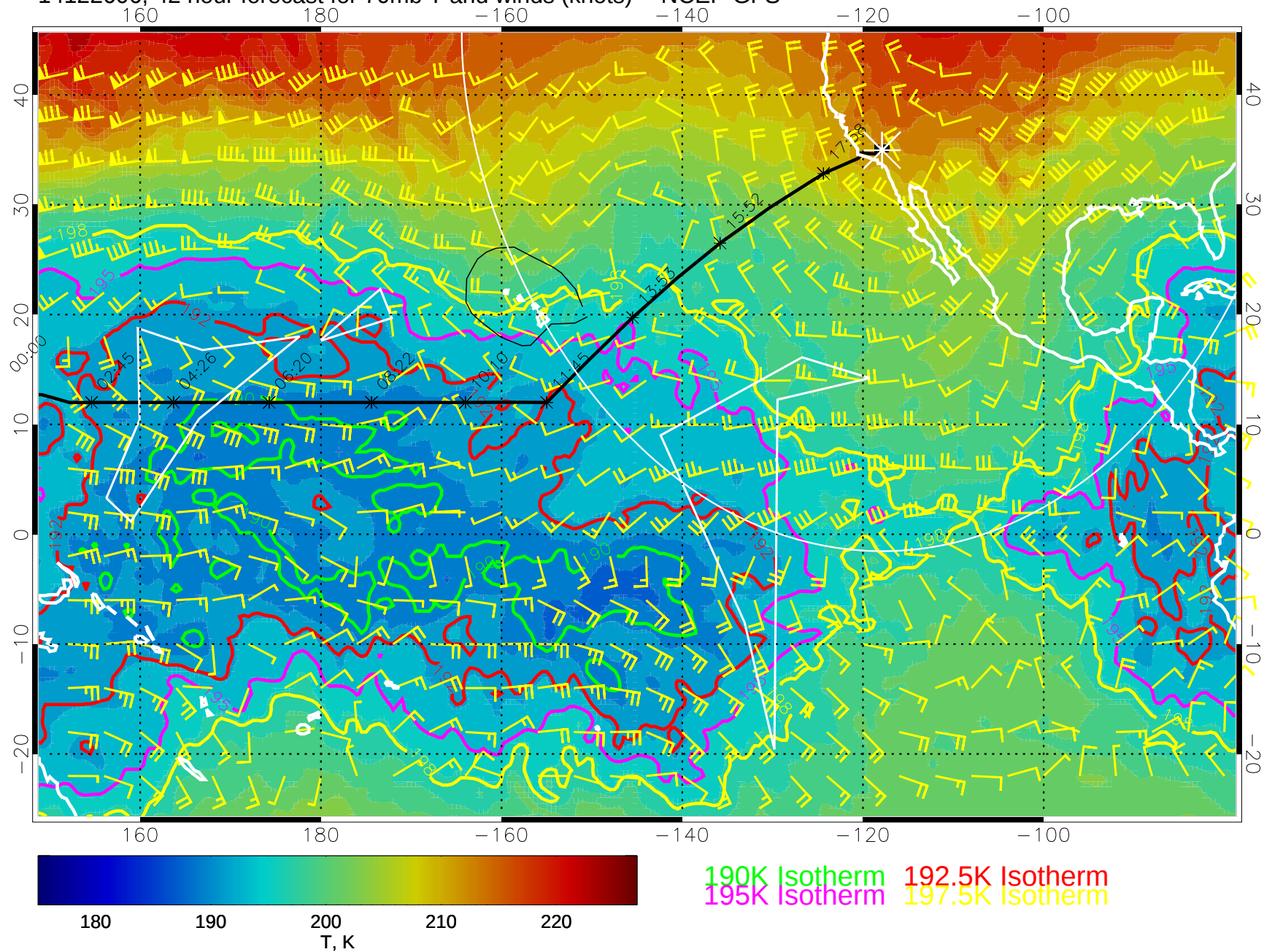
14122606, 42 hour forecast for 70mb T and winds (knots) -- NCEP GFS
