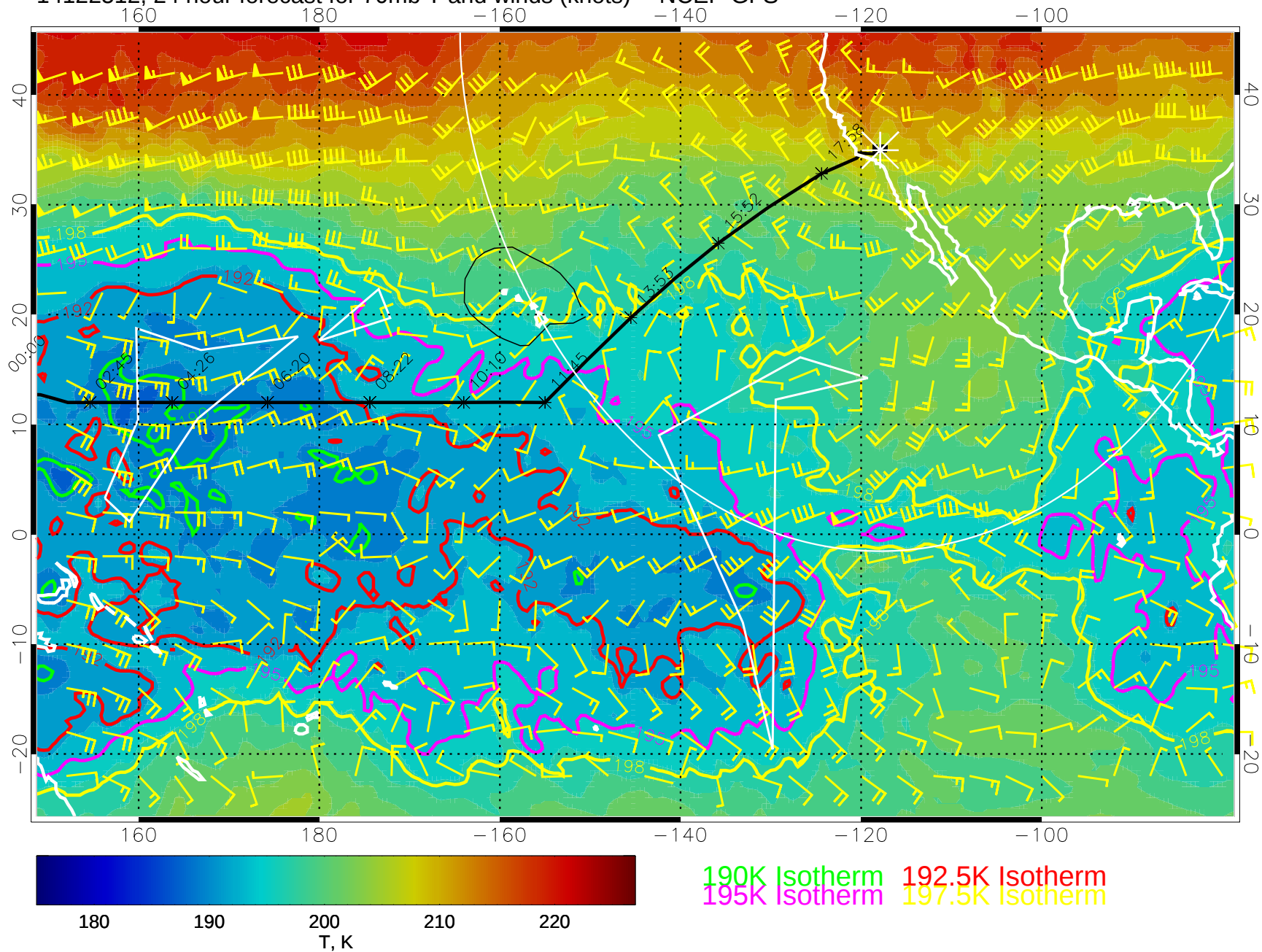
14122512, 24 hour forecast for 70mb T and winds (knots) -- NCEP GFS
