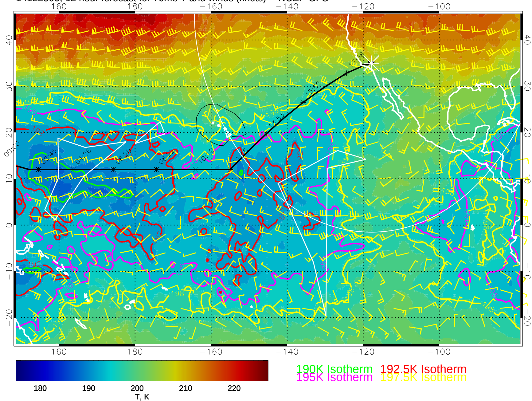
14122500, 12 hour forecast for 70mb T and winds (knots) -- NCEP GFS
