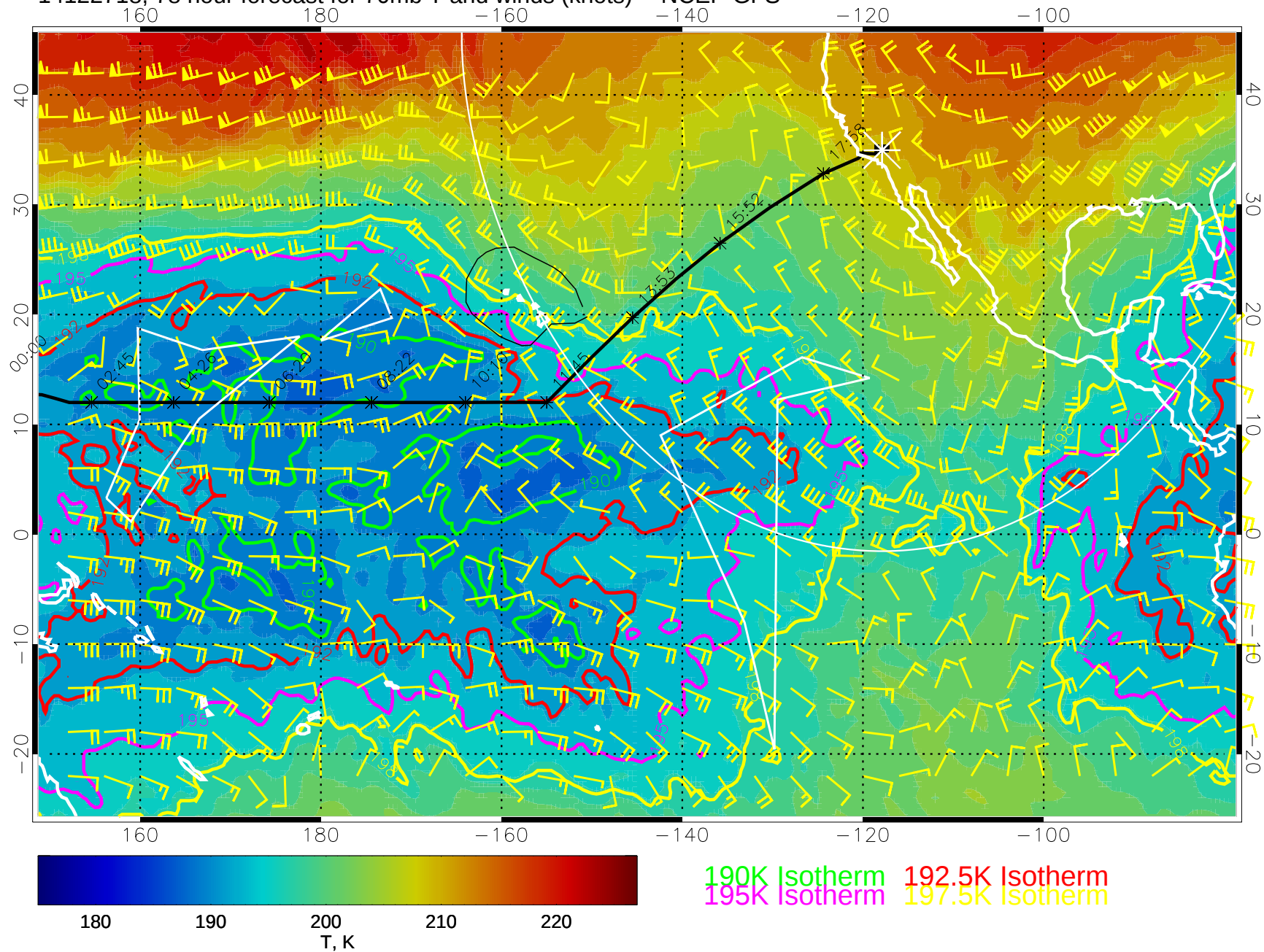
14122718, 78 hour forecast for 70mb T and winds (knots) -- NCEP GFS
