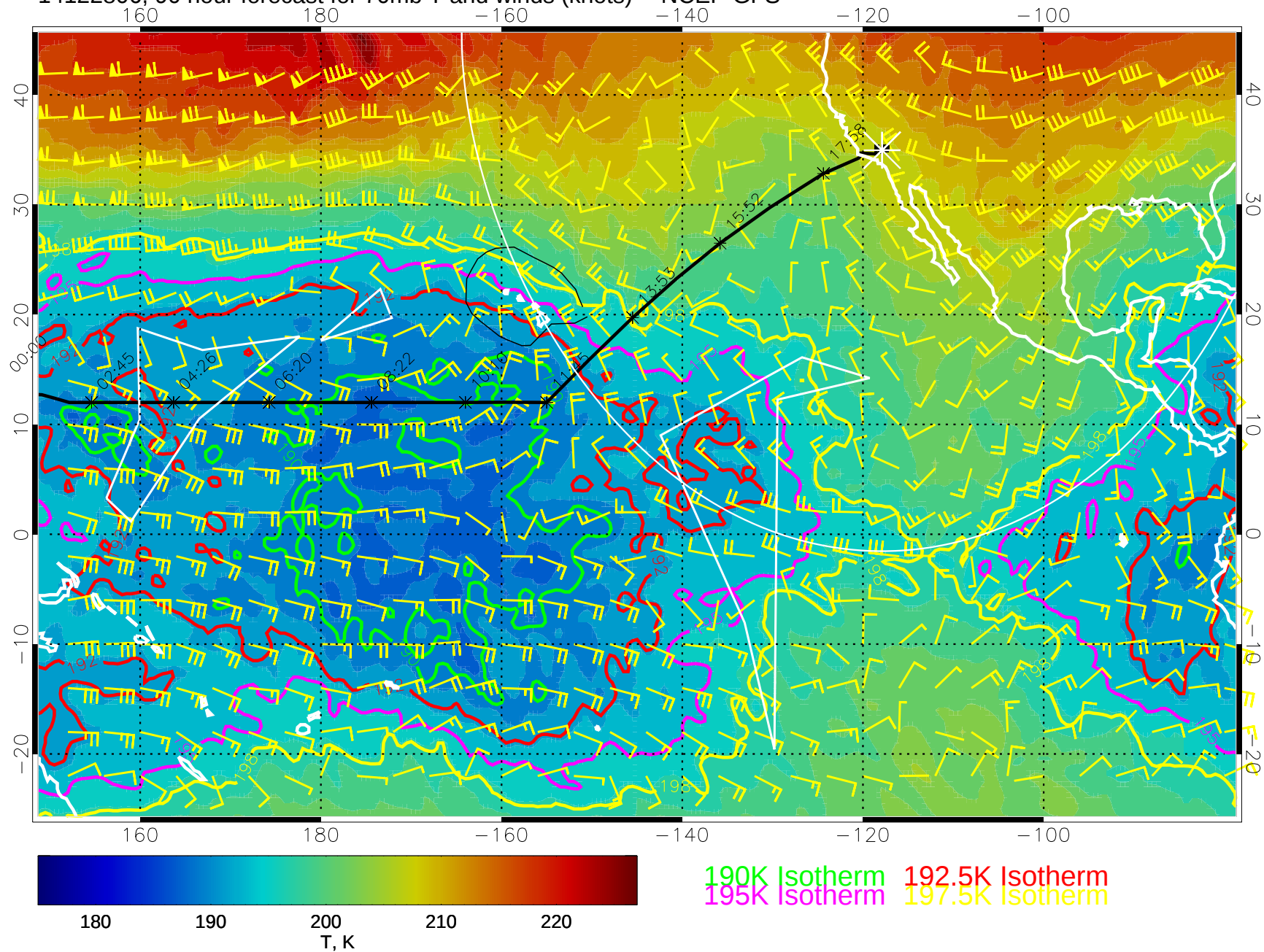
14122806, 90 hour forecast for 70mb T and winds (knots) -- NCEP GFS
