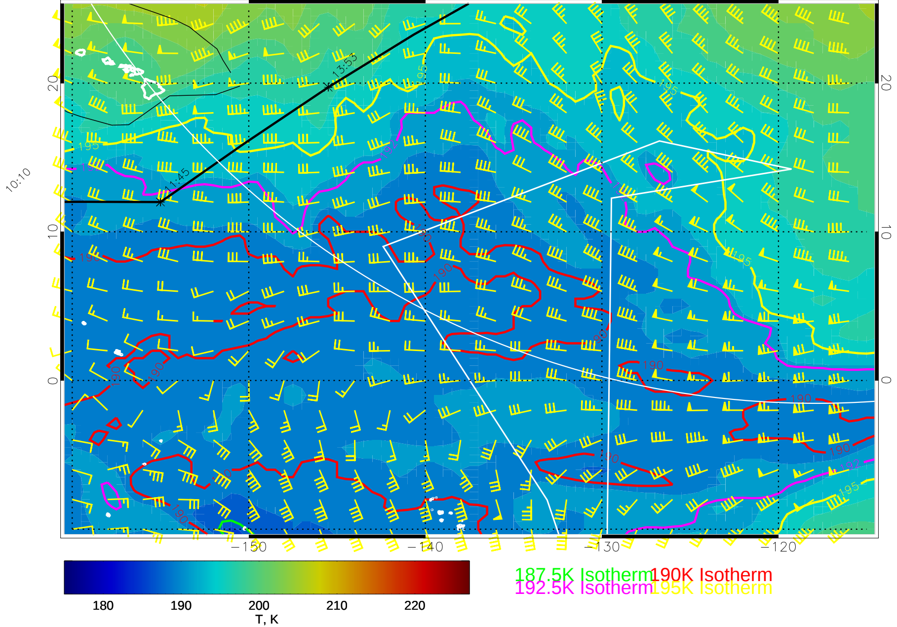
14122618, 54 hour forecast for 100mb T and winds (knots) -- NCEP GFS
