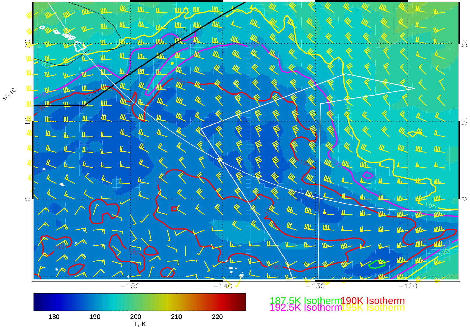
14122512, 24 hour forecast for 100mb T and winds (knots) -- NCEP GFS
