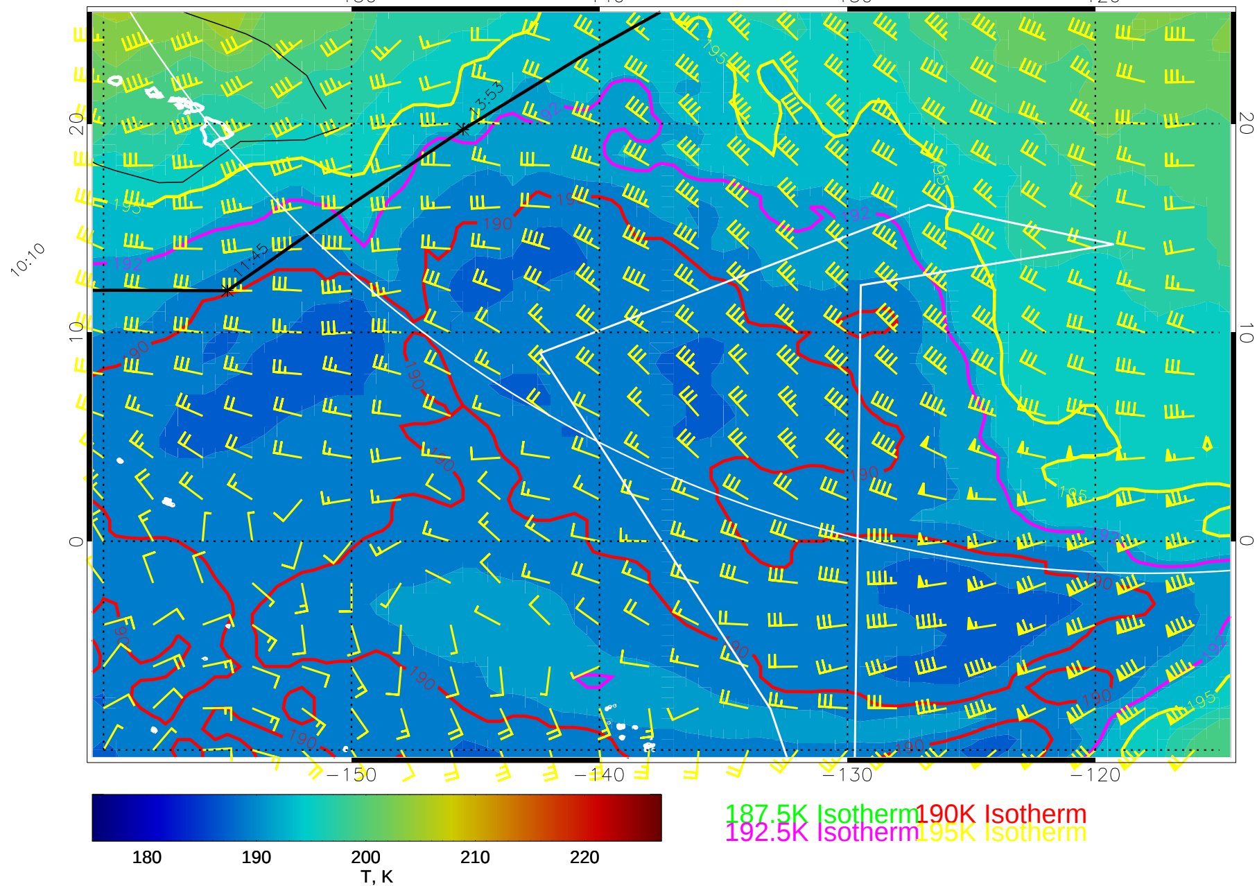
14122600, 36 hour forecast for 100mb T and winds (knots) -- NCEP GFS
