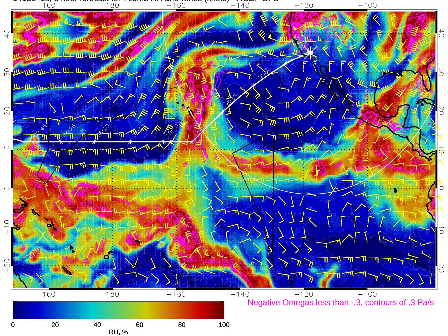
14122418, 6 hour forecast for 700mb RH and winds (knots) - NCEP GFS
