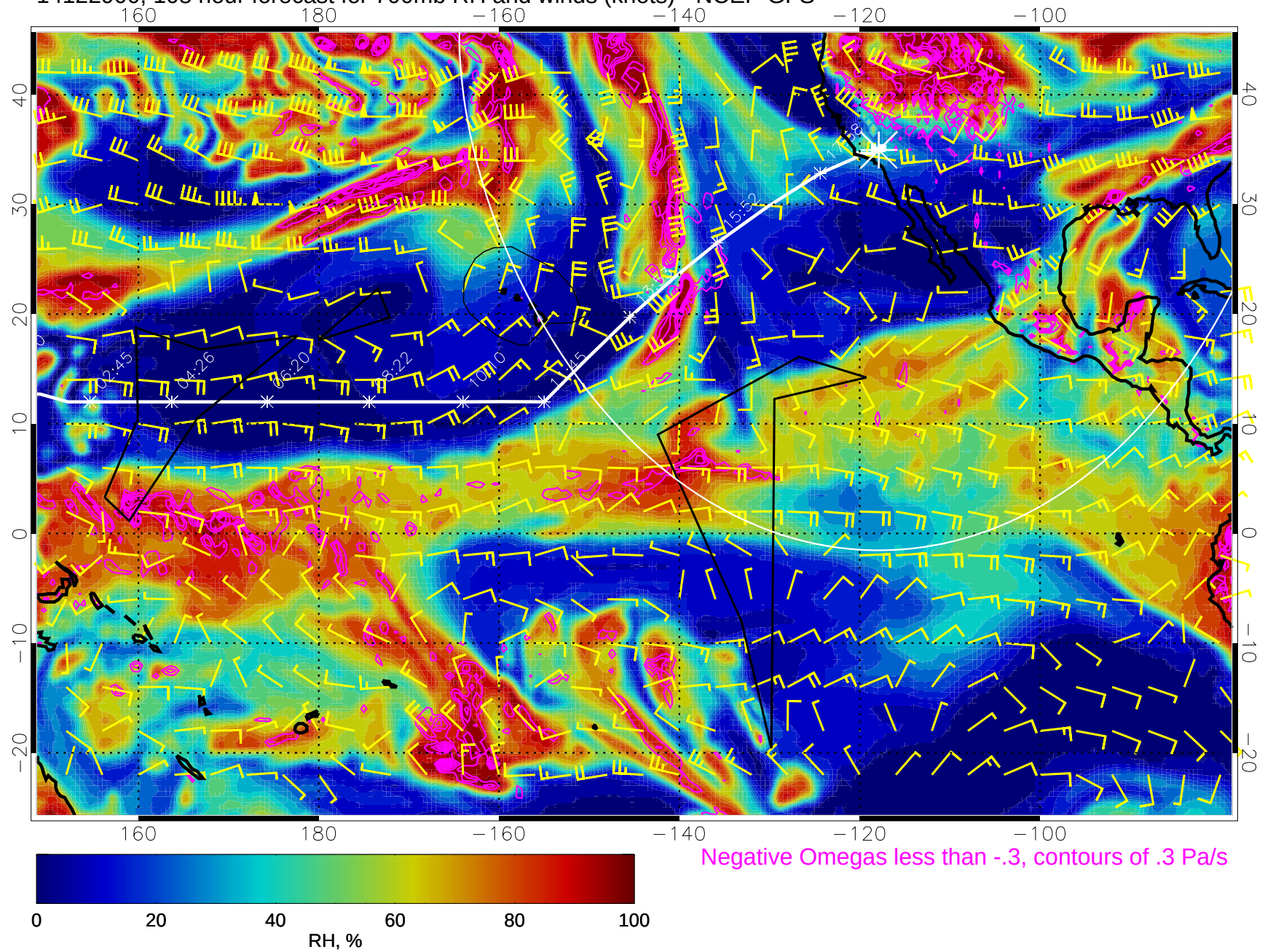
14122900, 108 hour forecast for 700mb RH and winds (knots) - NCEP GFS
