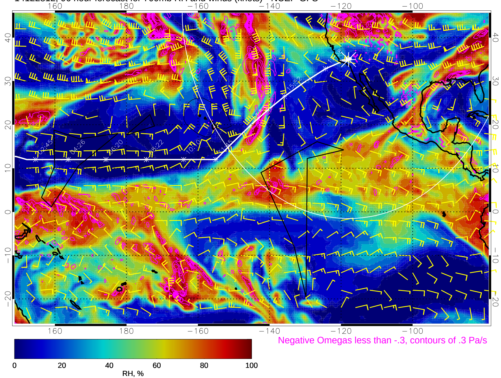
14122812, 96 hour forecast for 700mb RH and winds (knots) - NCEP GFS
