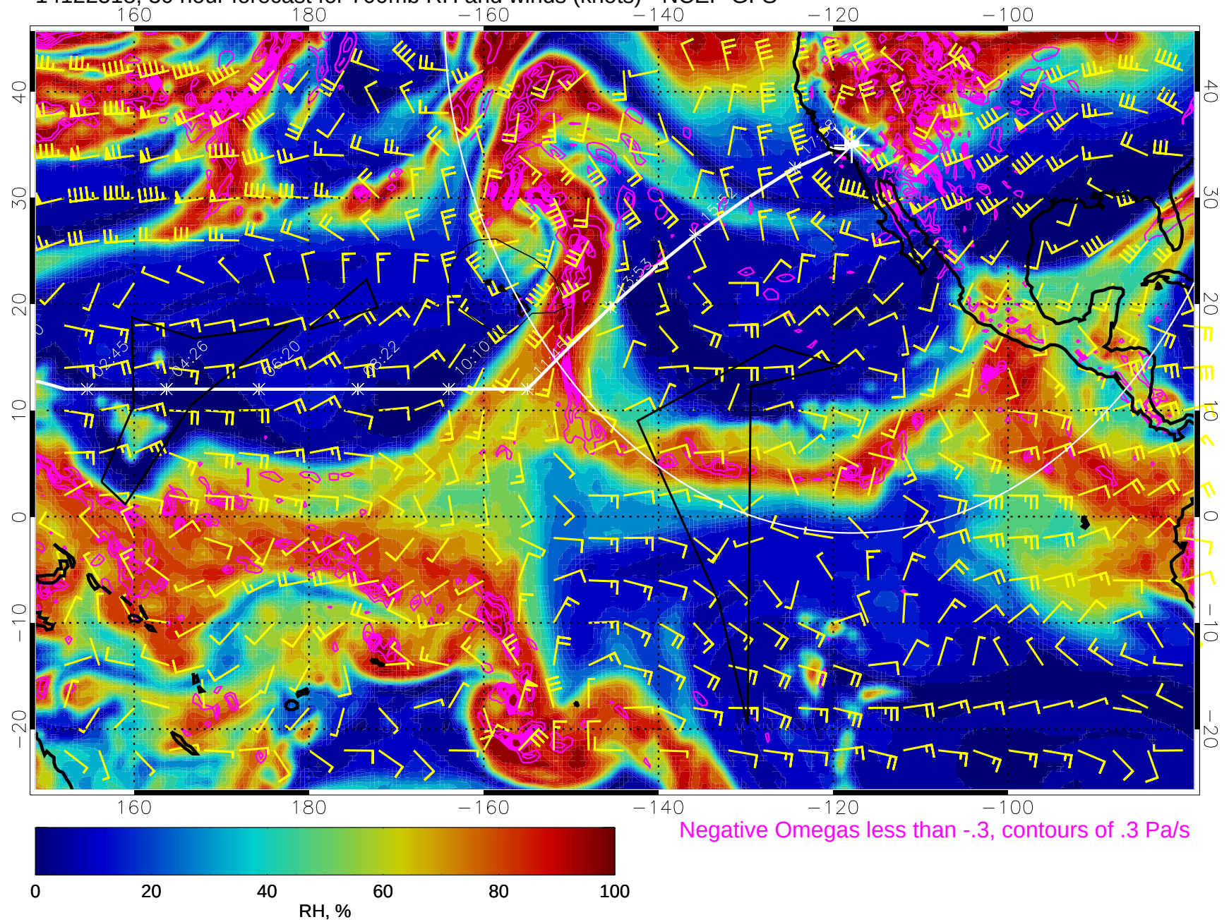
14122518, 30 hour forecast for 700mb RH and winds (knots) - NCEP GFS
