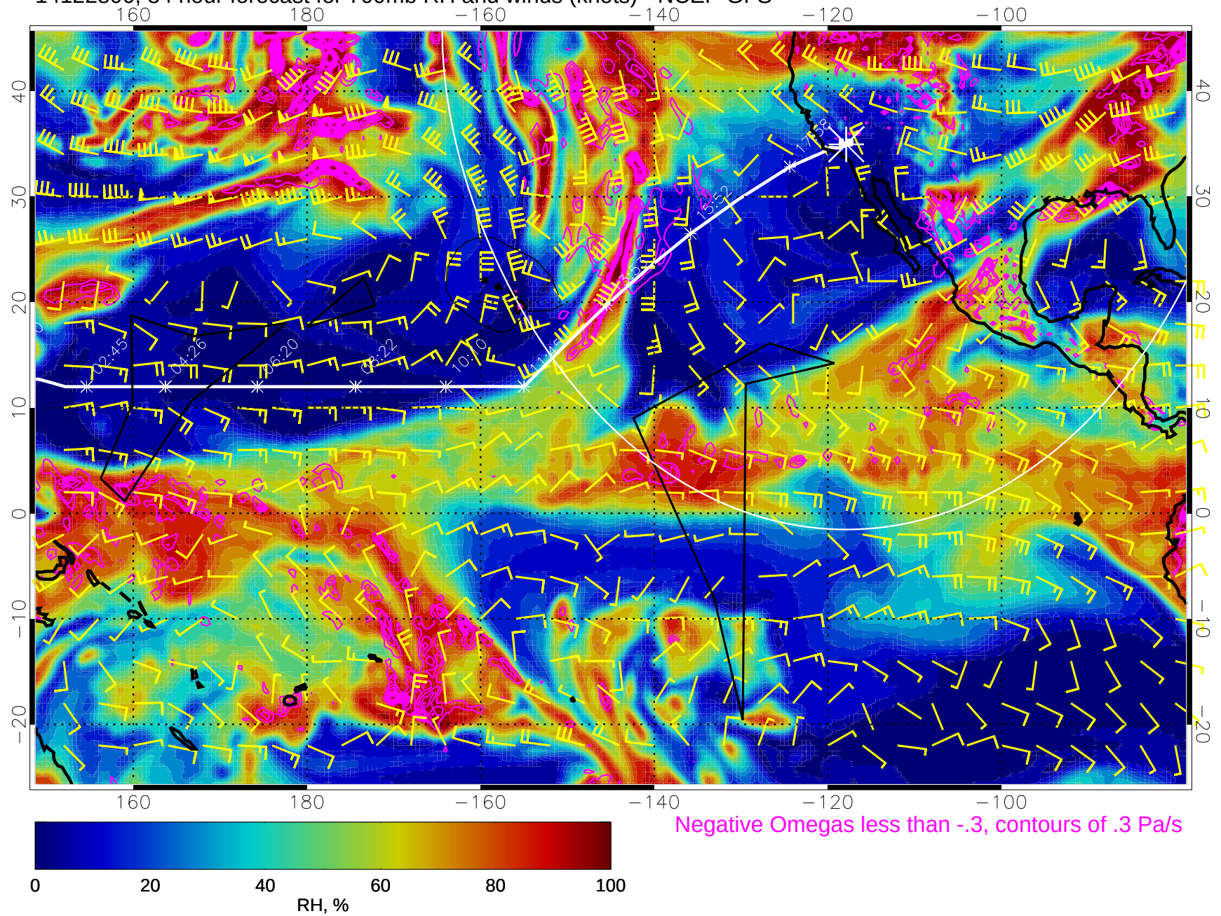
14122800, 84 hour forecast for 700mb RH and winds (knots) - NCEP GFS
