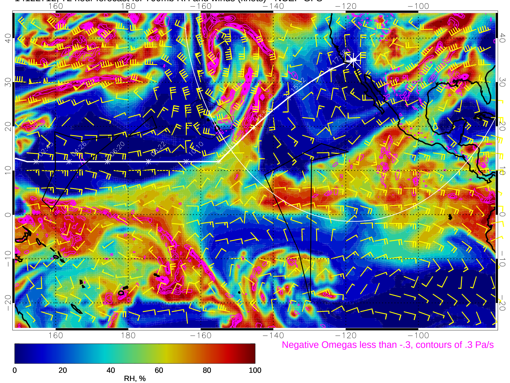
14122712, 72 hour forecast for 700mb RH and winds (knots) - NCEP GFS
