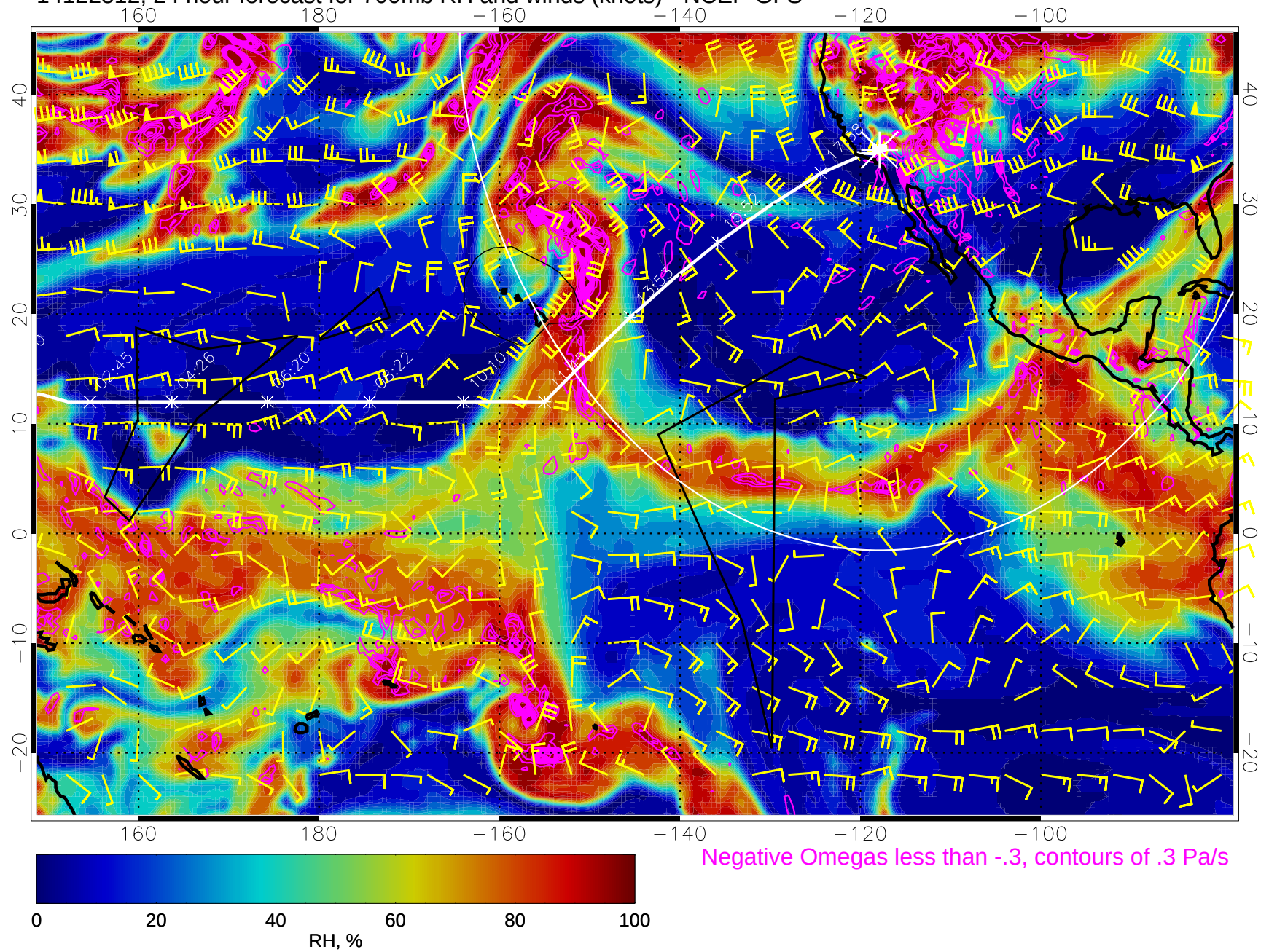
14122512, 24 hour forecast for 700mb RH and winds (knots) - NCEP GFS
