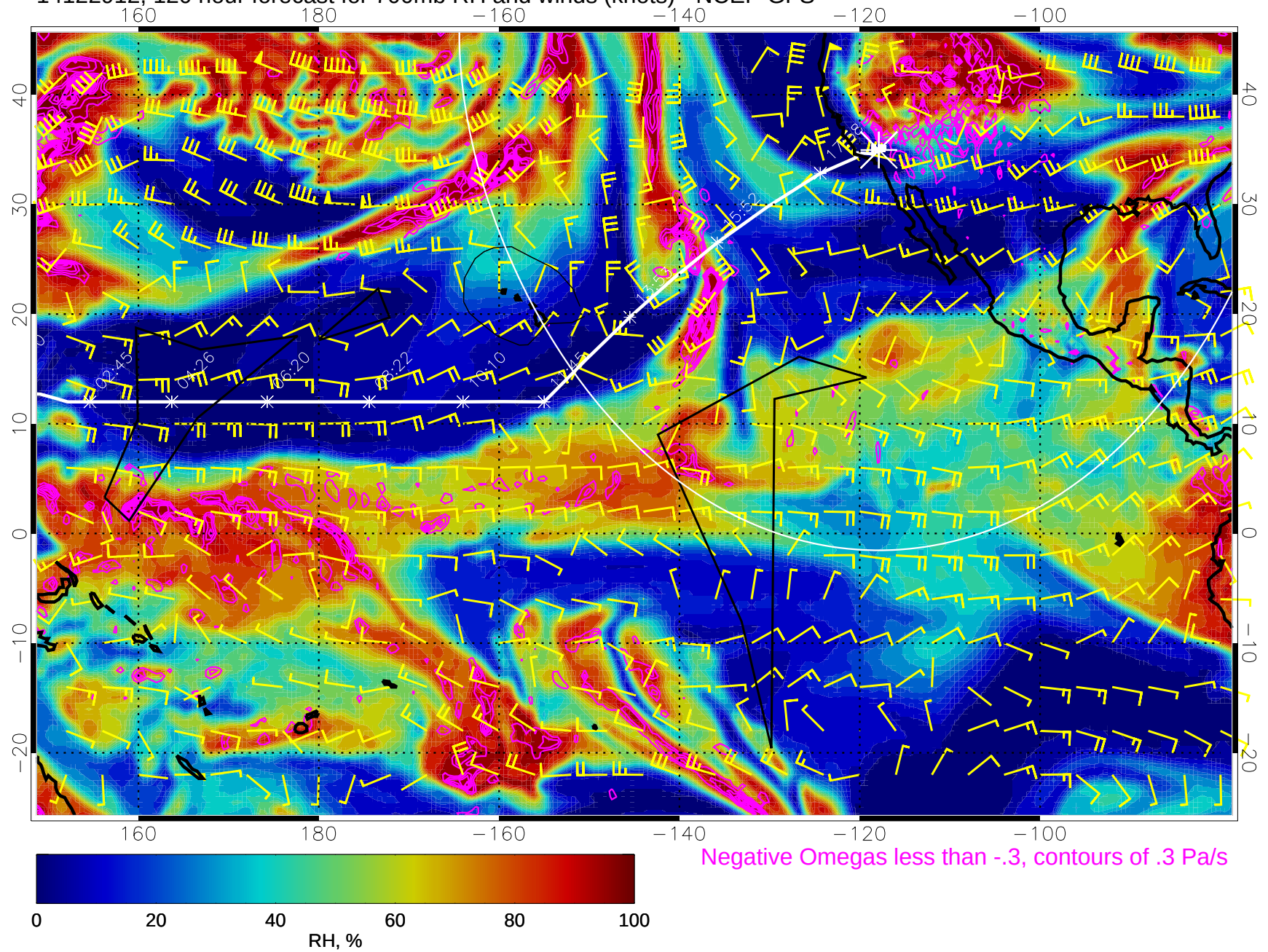
14122912, 120 hour forecast for 700mb RH and winds (knots) - NCEP GFS
