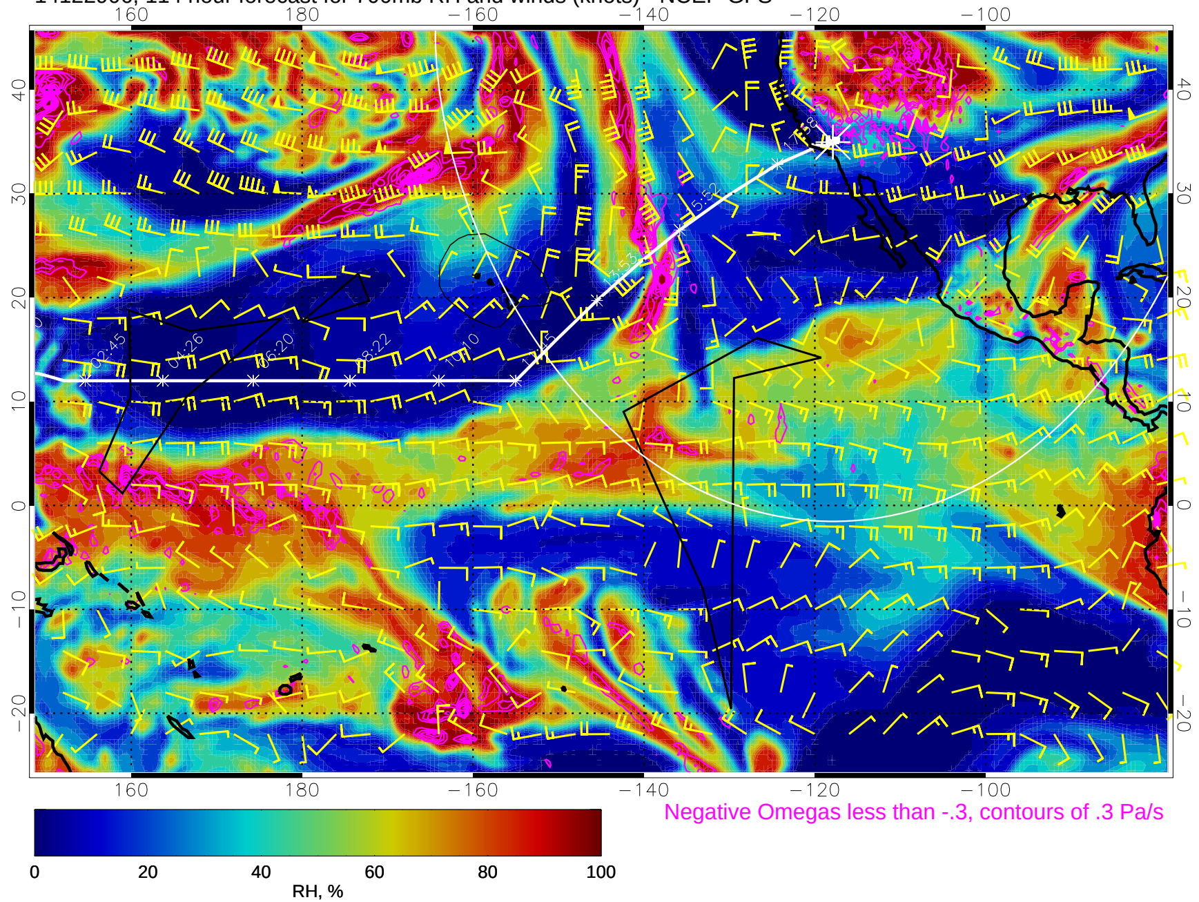
14122906, 114 hour forecast for 700mb RH and winds (knots) - NCEP GFS
