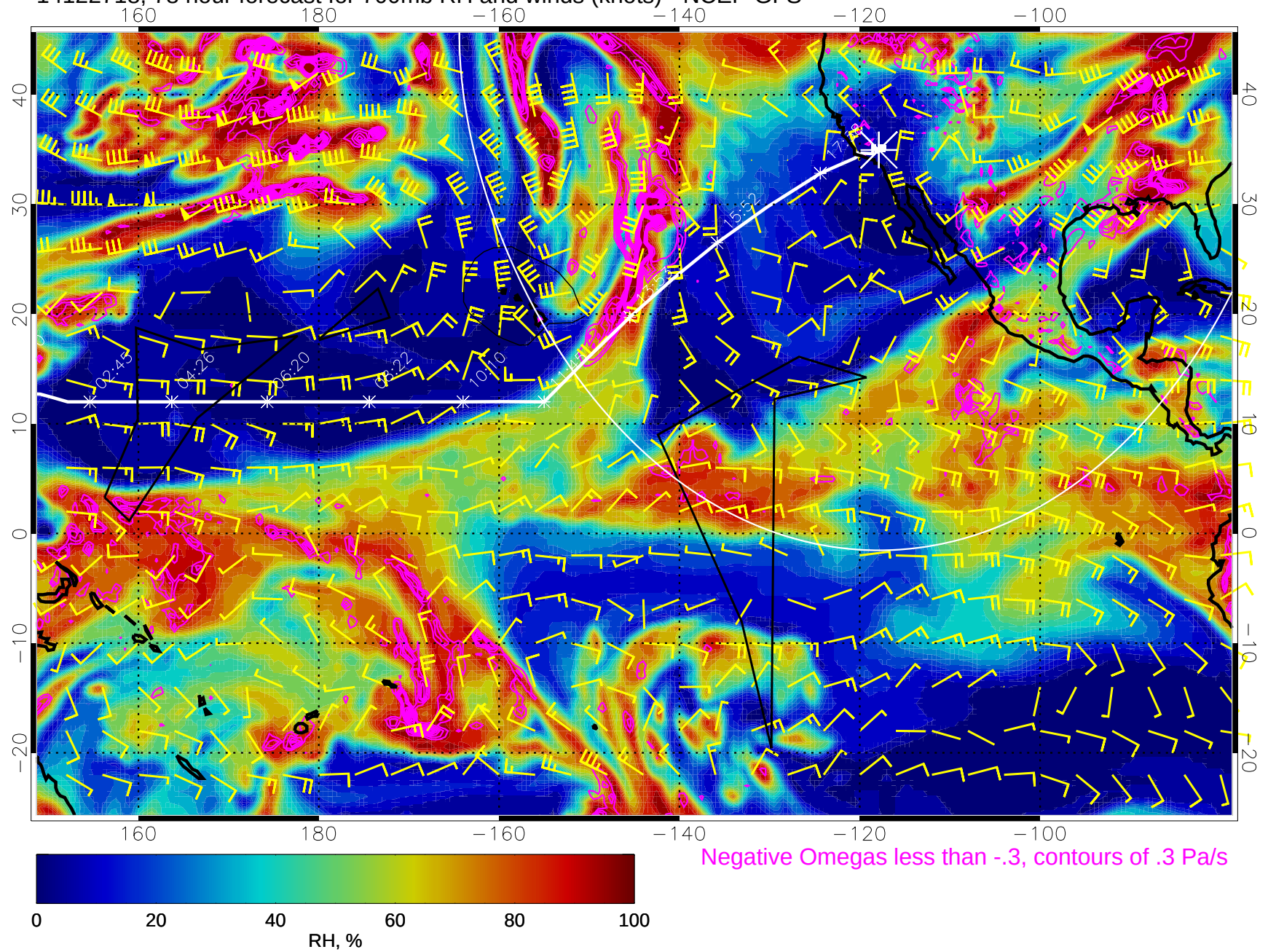
14122718, 78 hour forecast for 700mb RH and winds (knots) - NCEP GFS
