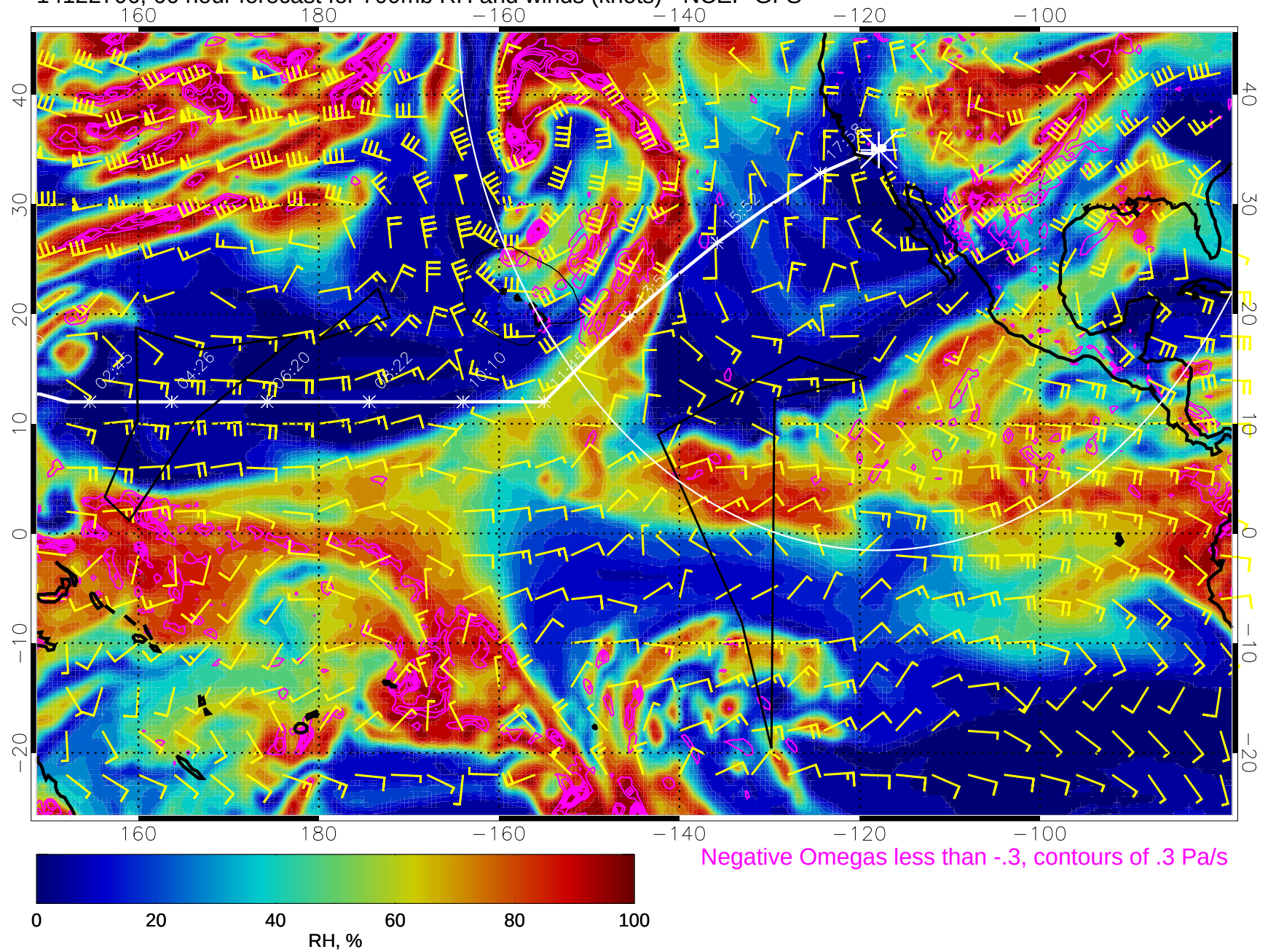
14122706, 66 hour forecast for 700mb RH and winds (knots) - NCEP GFS
