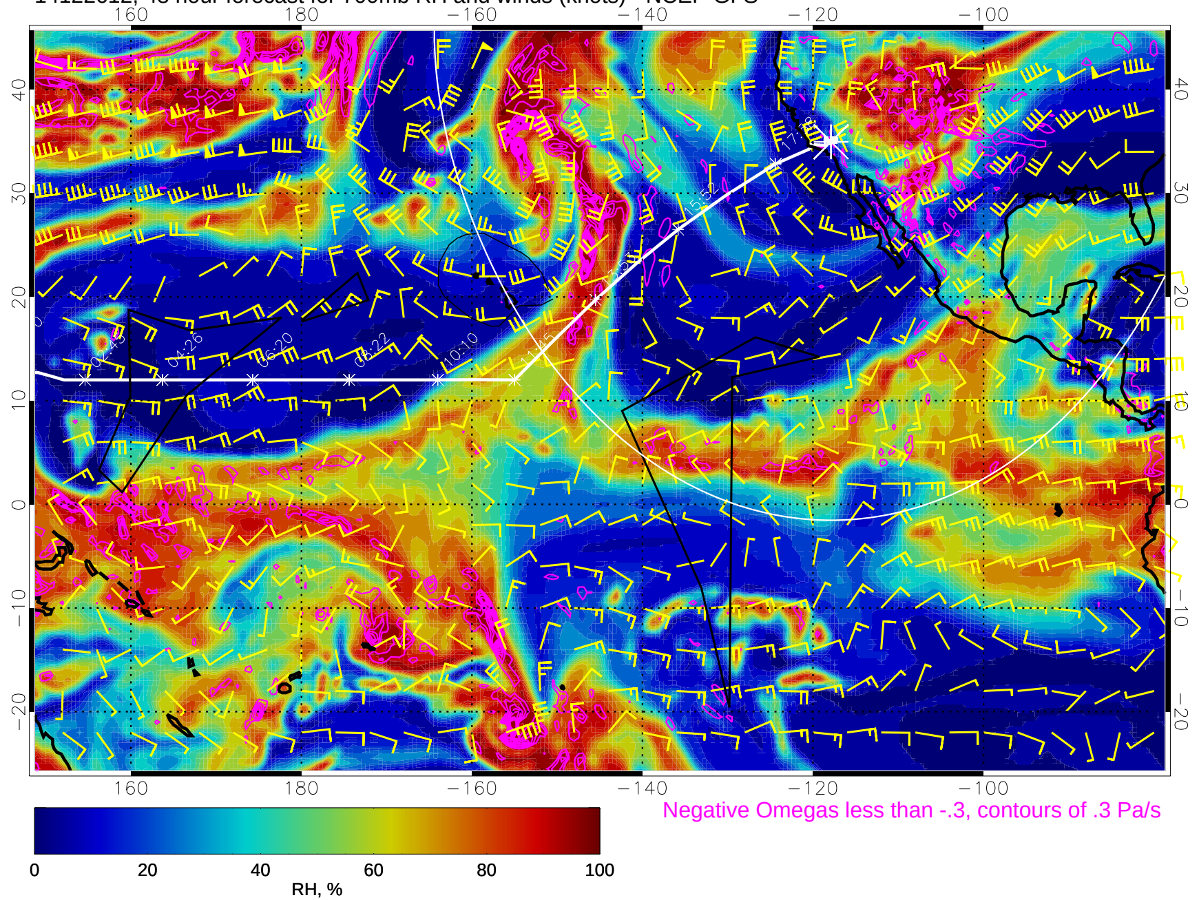
14122612, 48 hour forecast for 700mb RH and winds (knots) - NCEP GFS
