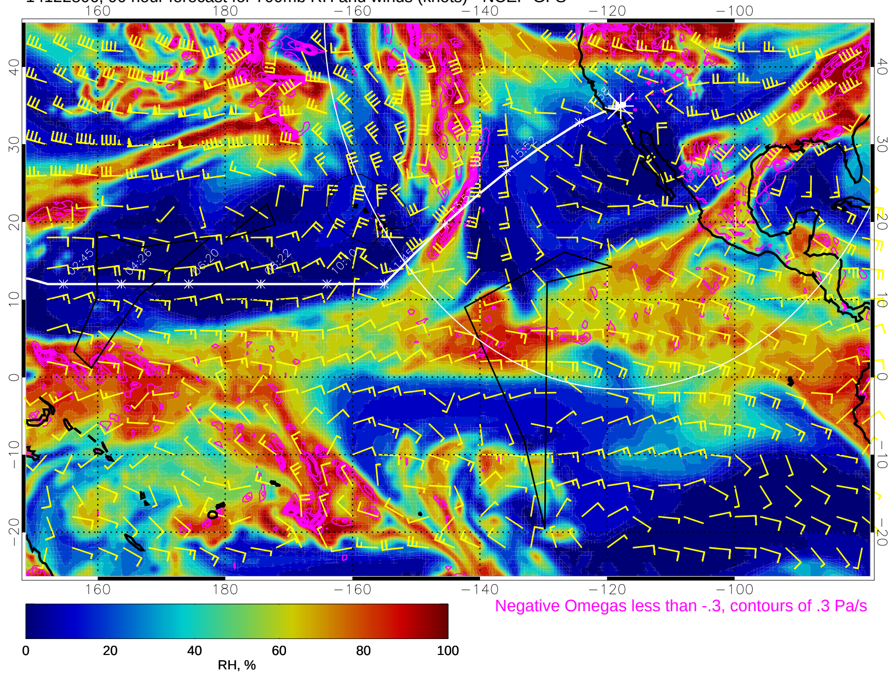
14122806, 90 hour forecast for 700mb RH and winds (knots) - NCEP GFS
