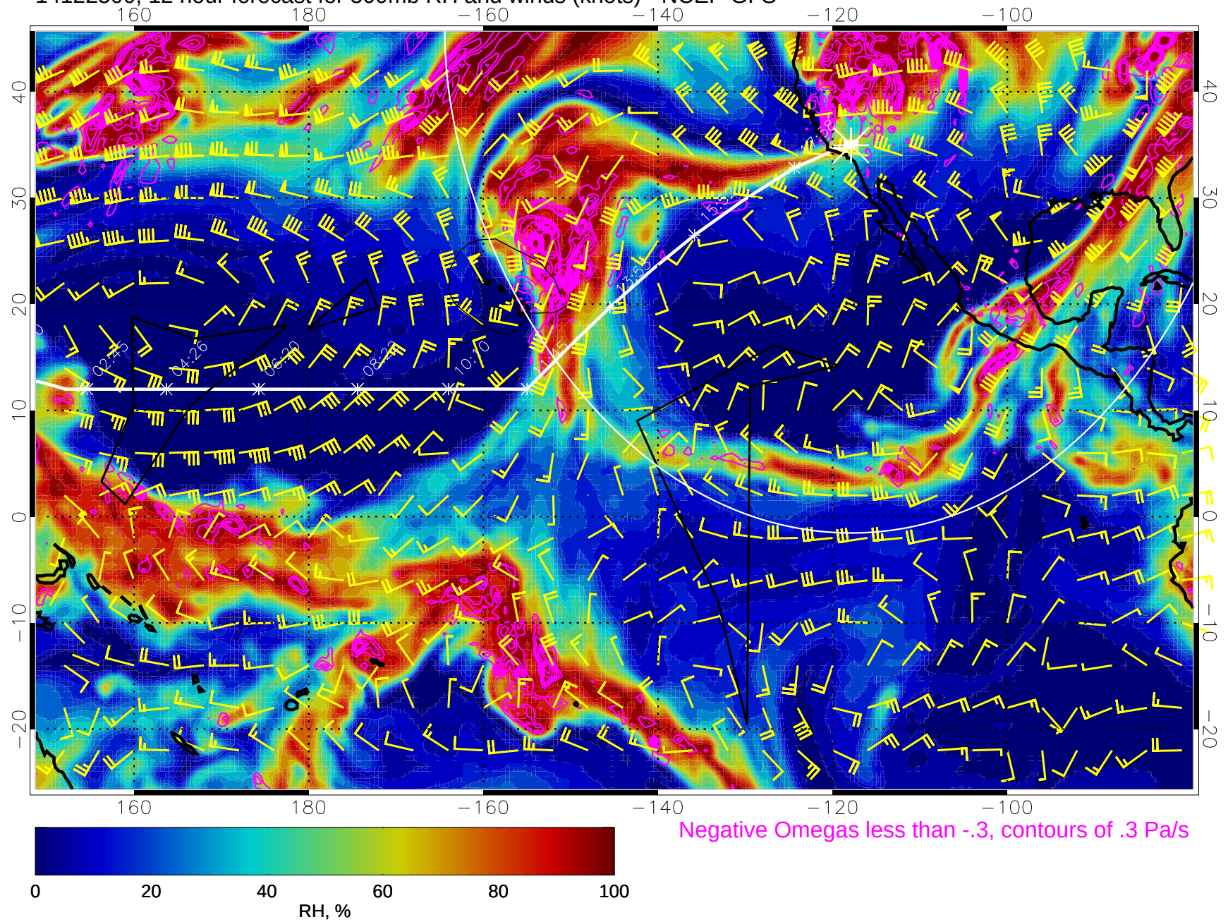
14122500, 12 hour forecast for 500mb RH and winds (knots) - NCEP GFS
