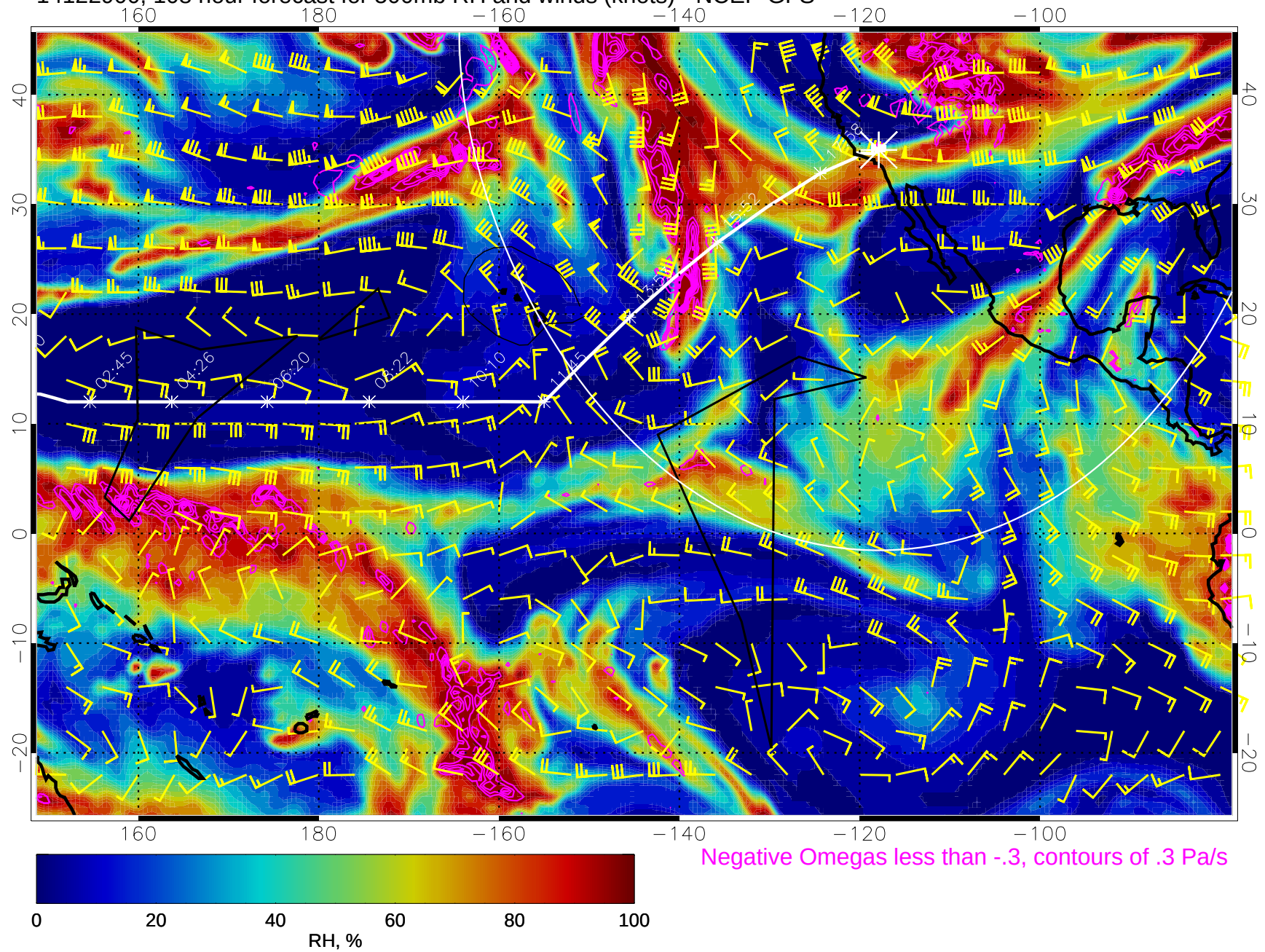
14122900, 108 hour forecast for 500mb RH and winds (knots) - NCEP GFS
