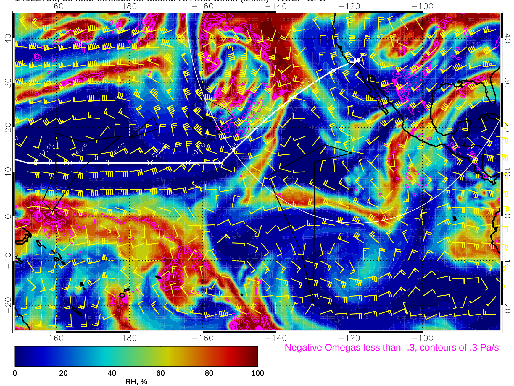
14122706, 66 hour forecast for 500mb RH and winds (knots) - NCEP GFS
