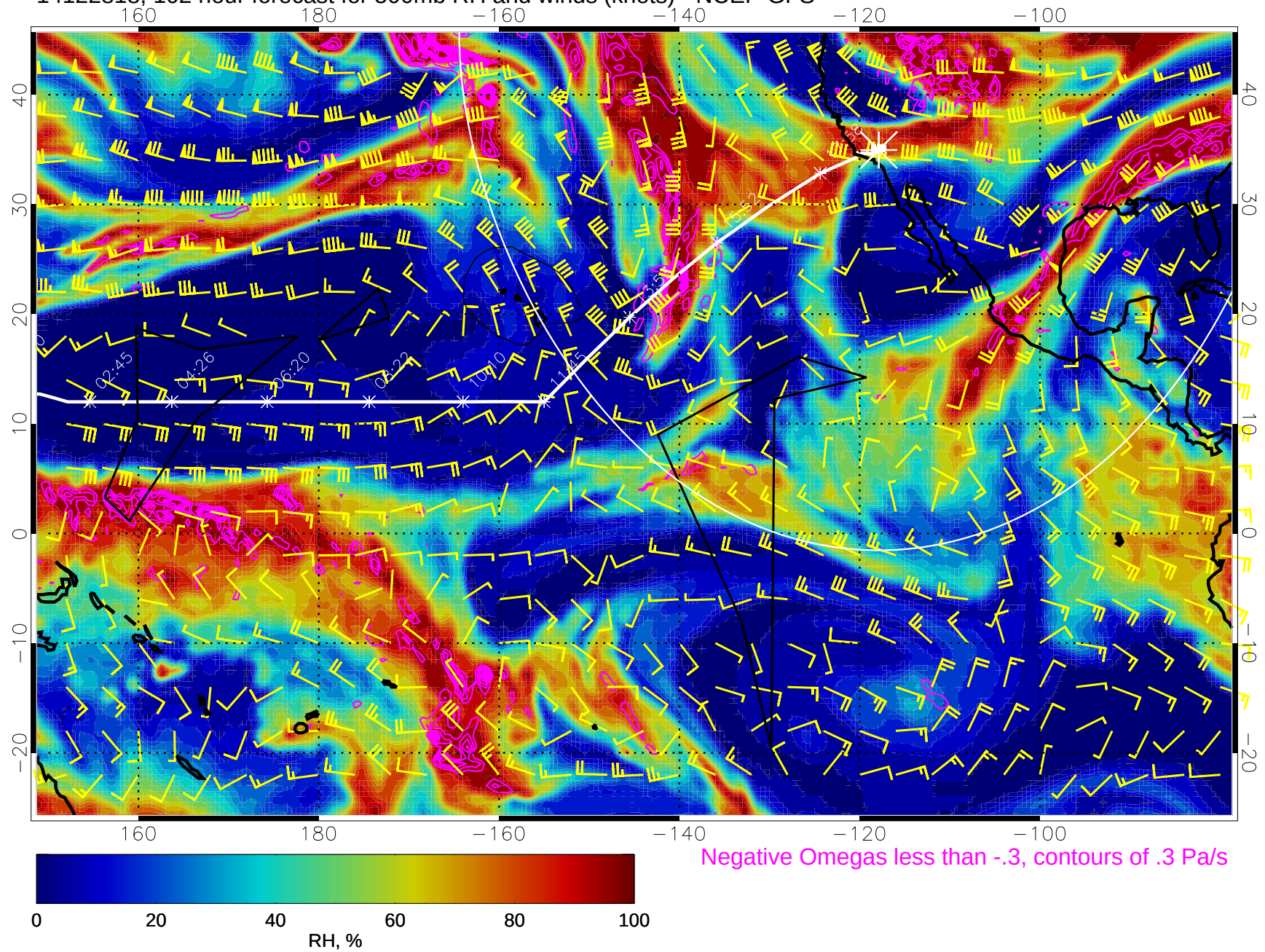
14122818, 102 hour forecast for 500mb RH and winds (knots) - NCEP GFS
