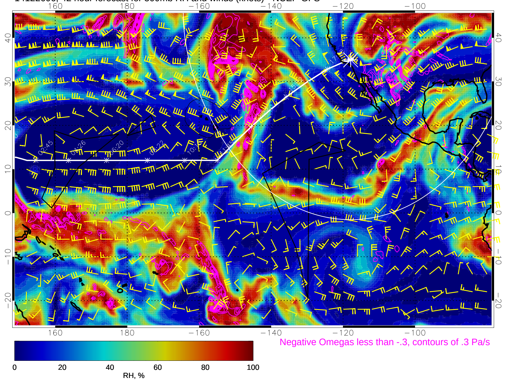
14122606, 42 hour forecast for 500mb RH and winds (knots) - NCEP GFS
