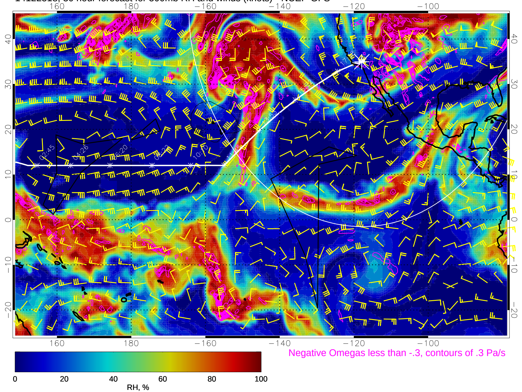
14122518, 30 hour forecast for 500mb RH and winds (knots) - NCEP GFS
