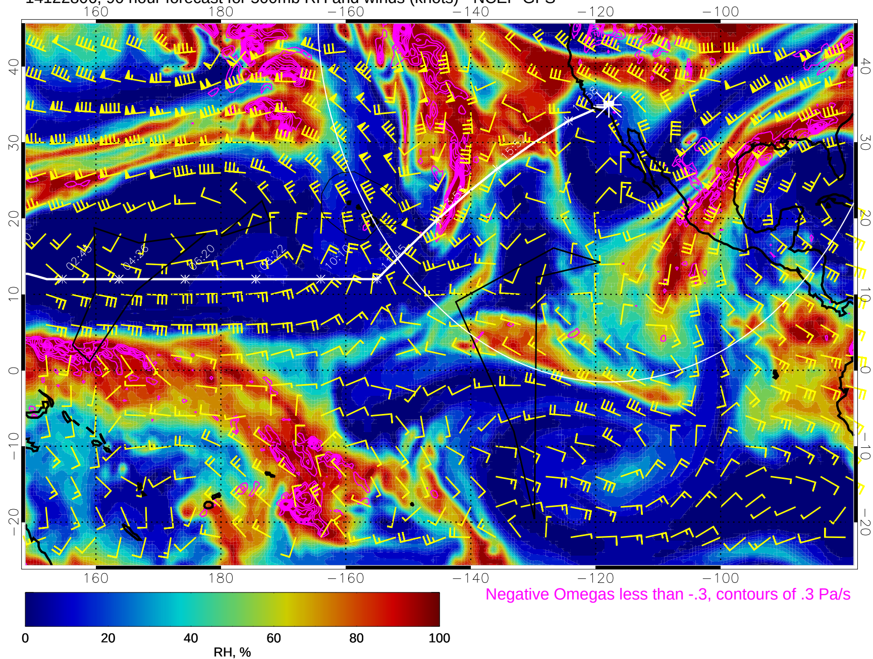
14122806, 90 hour forecast for 500mb RH and winds (knots) - NCEP GFS
