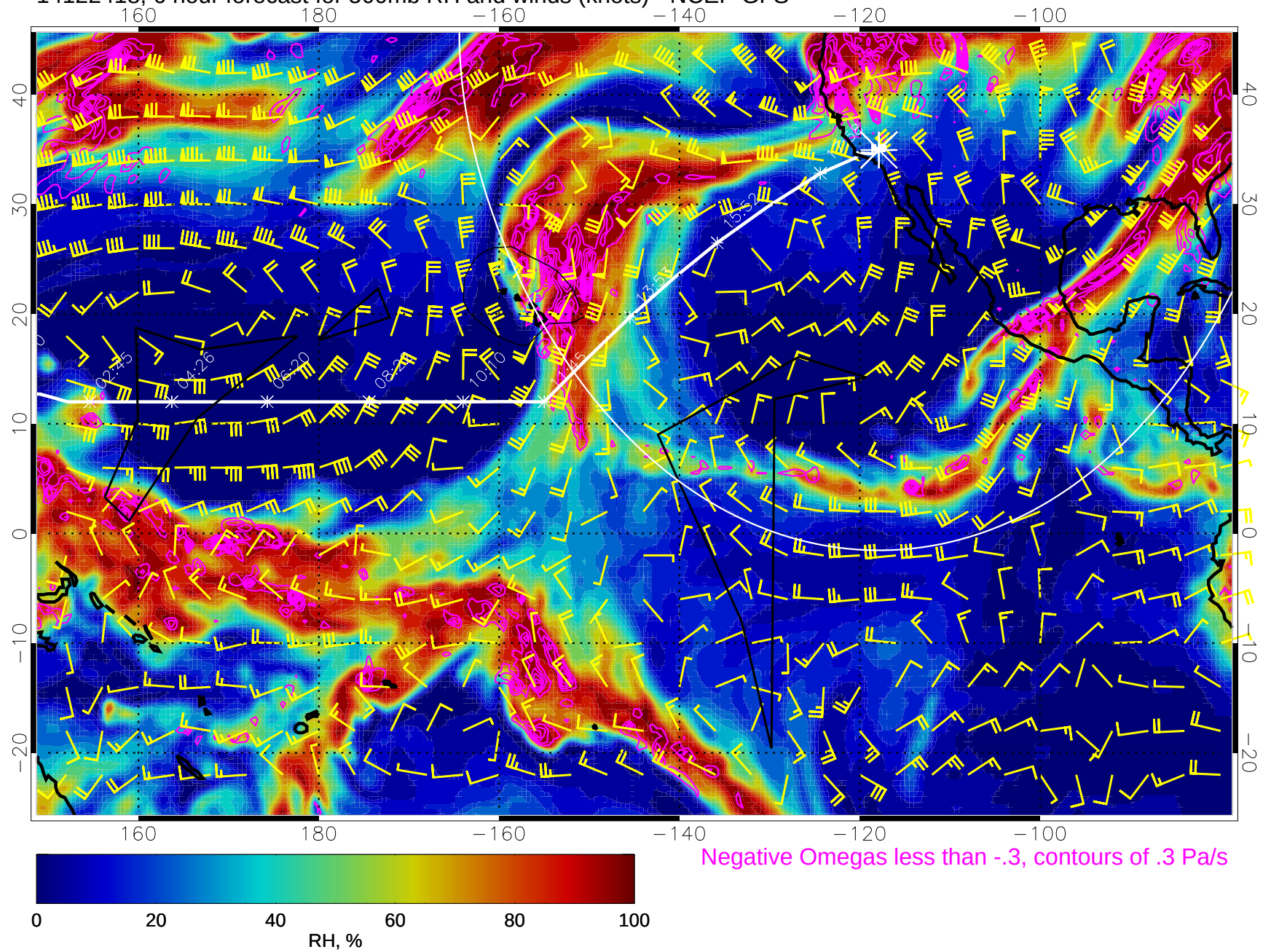
14122418, 6 hour forecast for 500mb RH and winds (knots) - NCEP GFS
