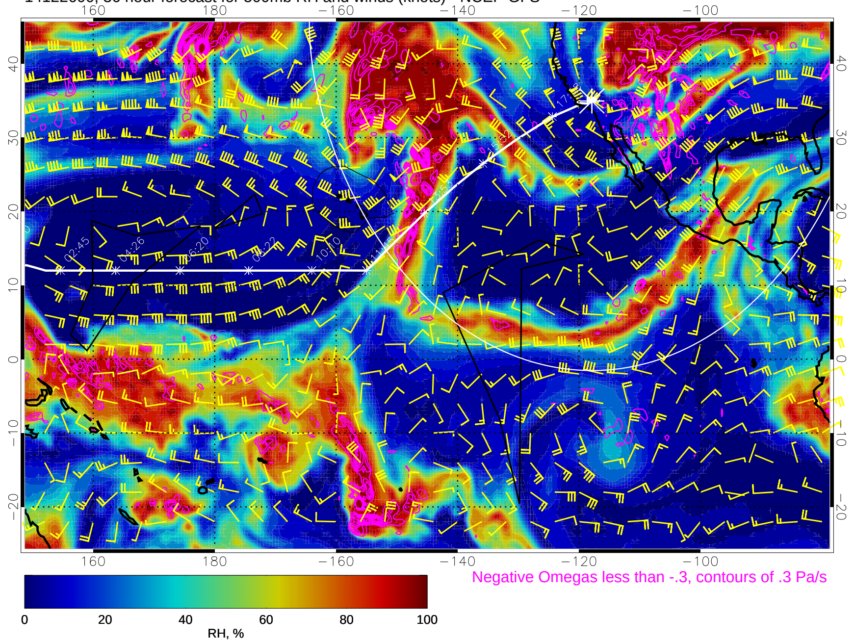
14122600, 36 hour forecast for 500mb RH and winds (knots) - NCEP GFS
