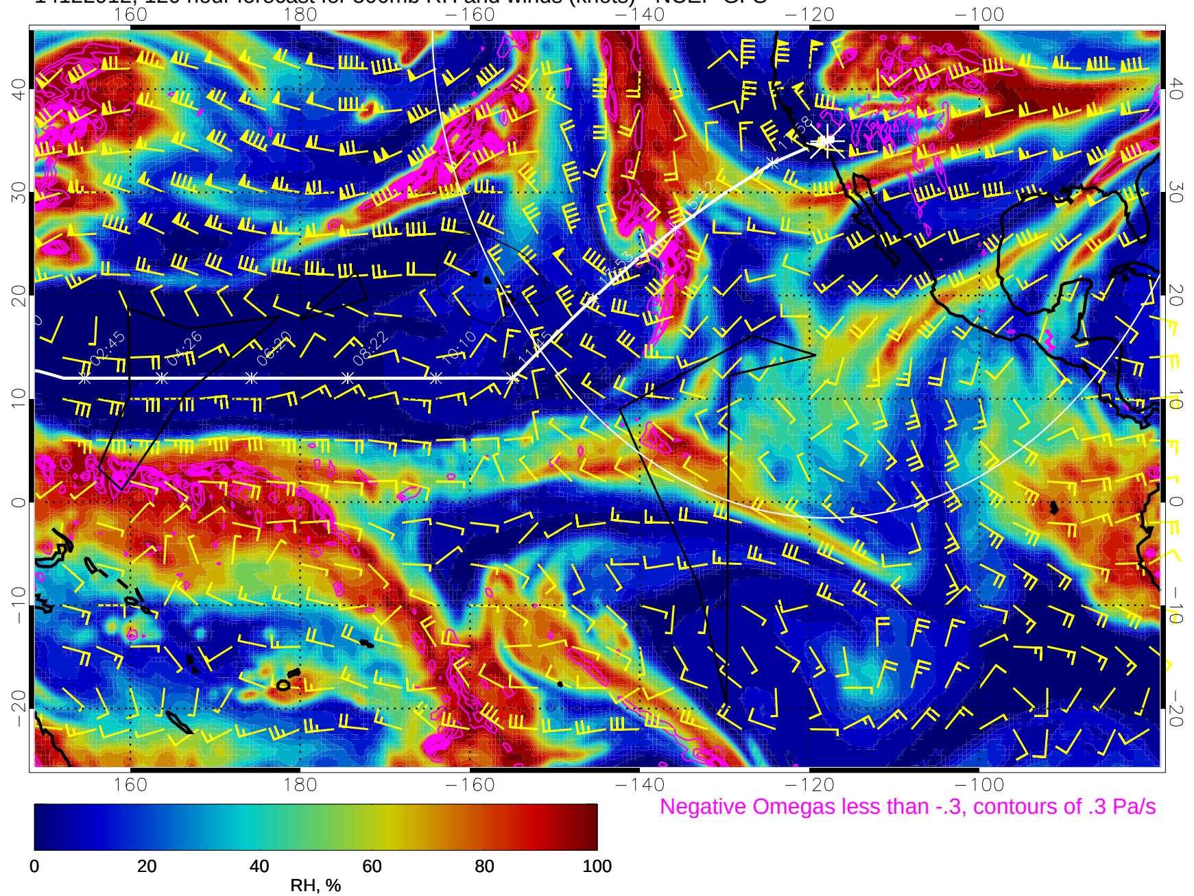
14122912, 120 hour forecast for 500mb RH and winds (knots) - NCEP GFS
