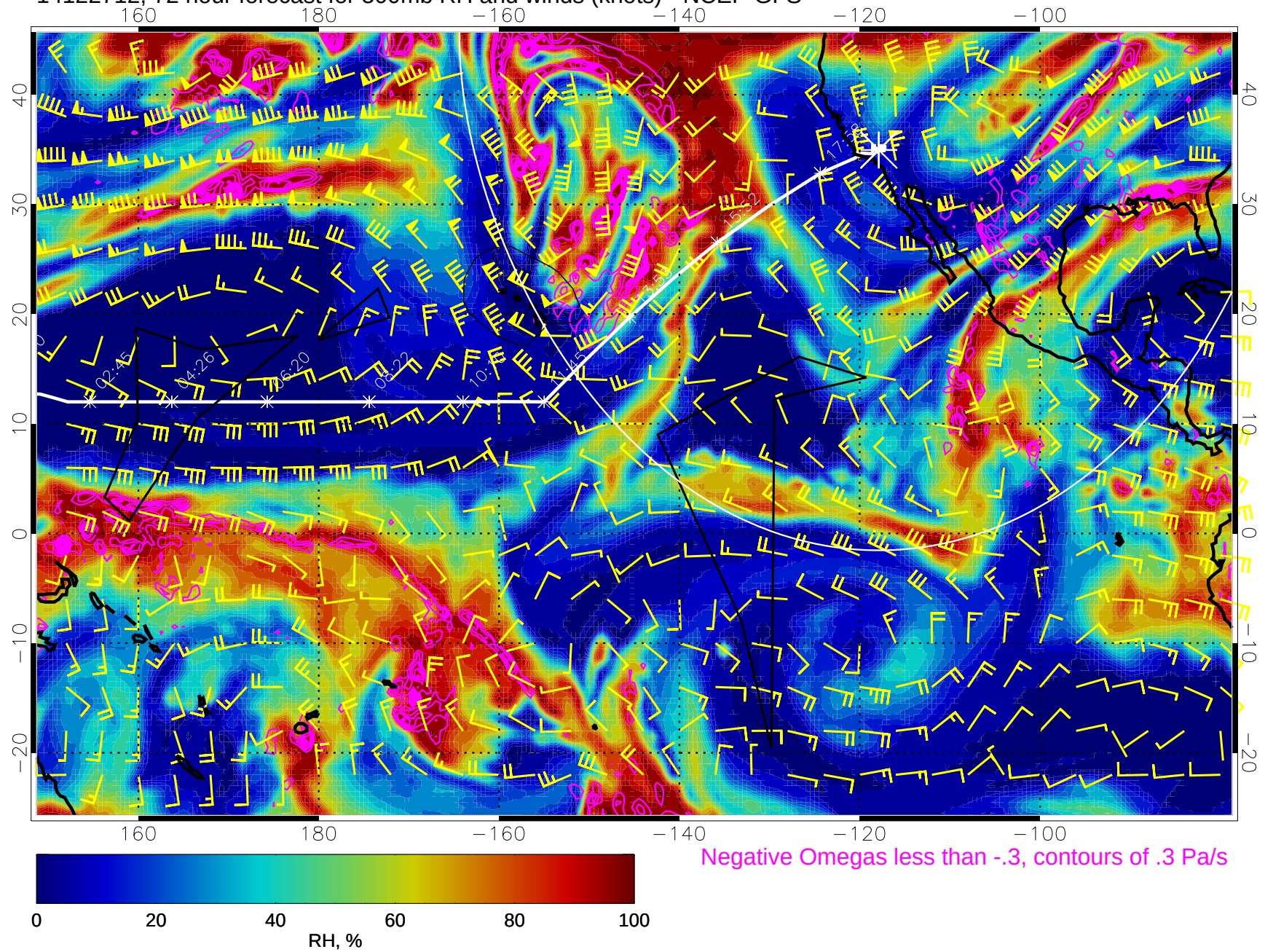
14122712, 72 hour forecast for 500mb RH and winds (knots) - NCEP GFS
