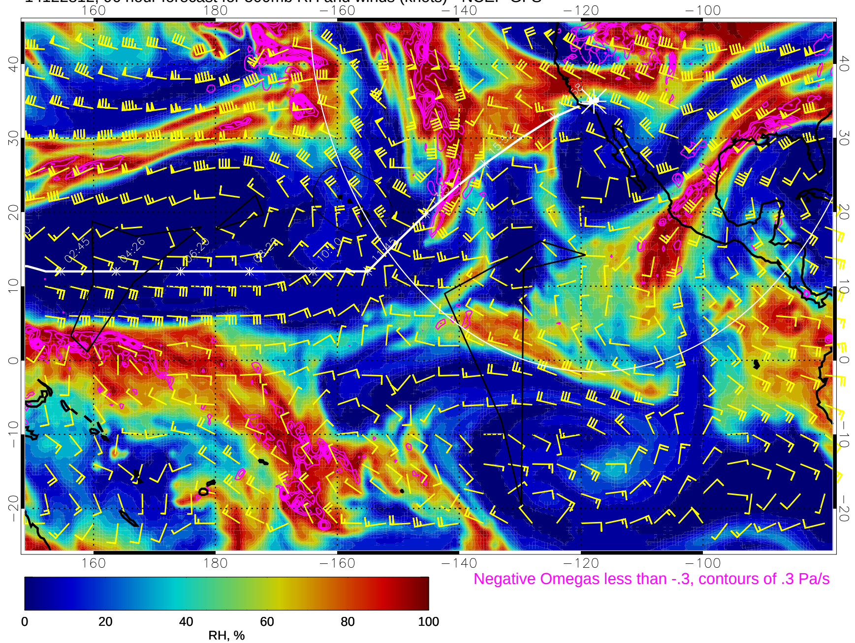
14122812, 96 hour forecast for 500mb RH and winds (knots) - NCEP GFS
