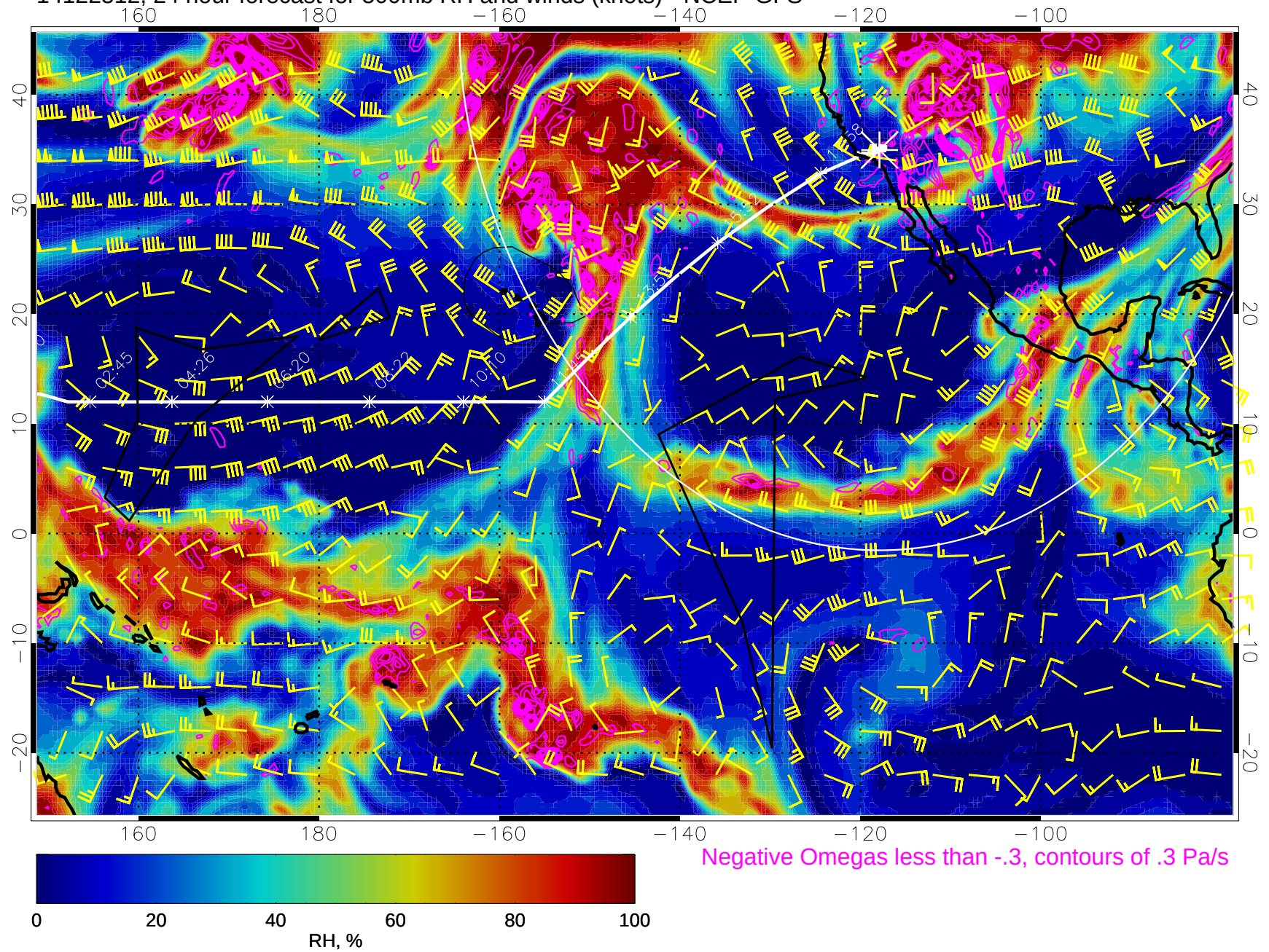
14122512, 24 hour forecast for 500mb RH and winds (knots) - NCEP GFS
