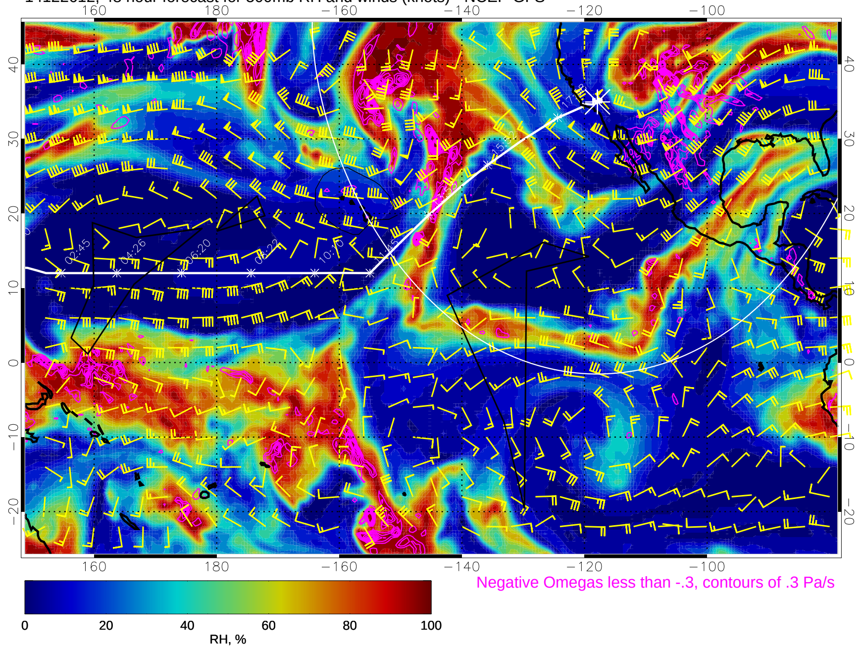
14122612, 48 hour forecast for 500mb RH and winds (knots) - NCEP GFS
