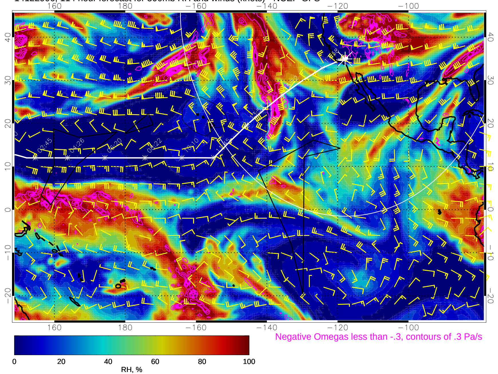
14122906, 114 hour forecast for 500mb RH and winds (knots) - NCEP GFS
