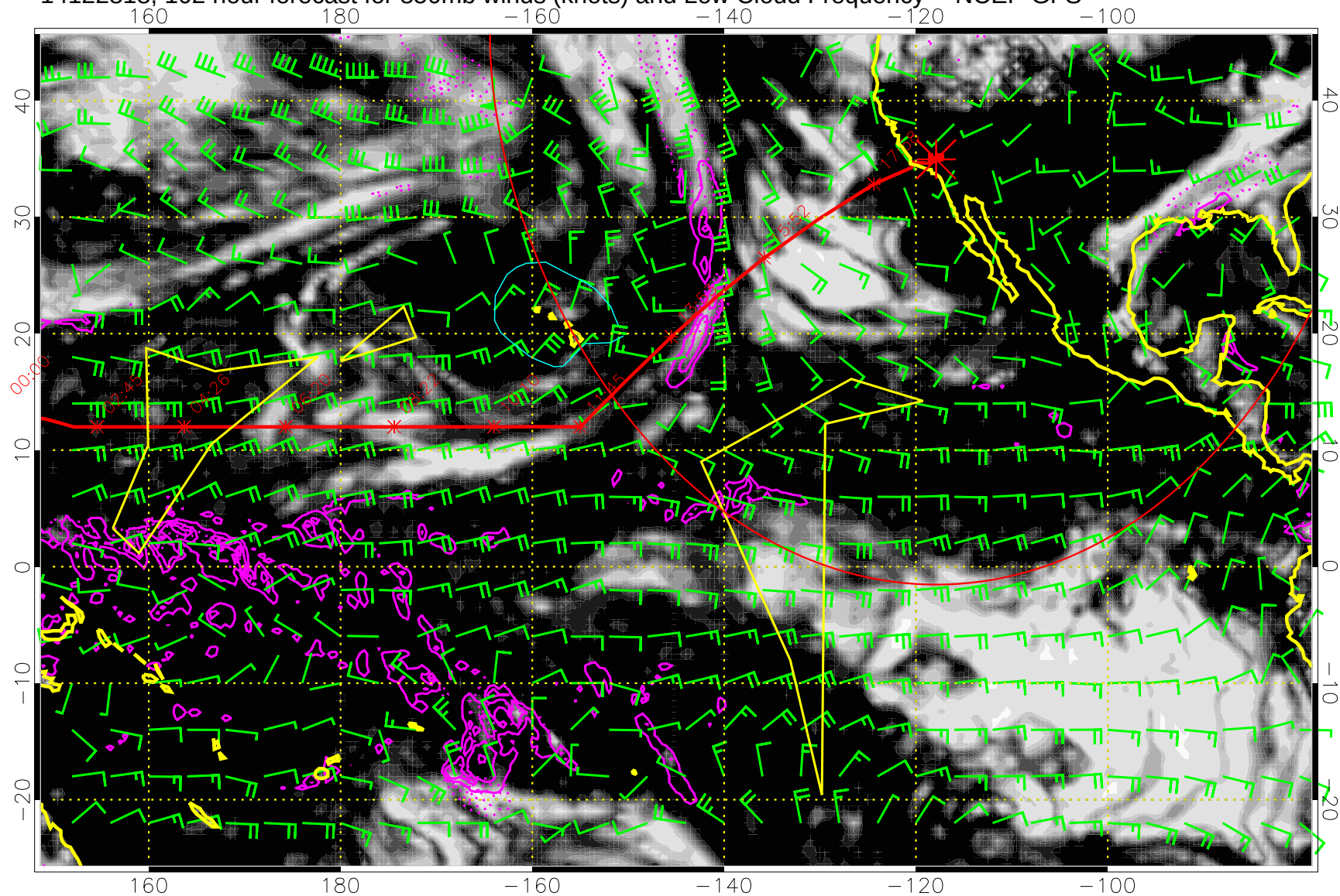
14122818, 102 hour forecast for 850mb winds (knots) and Low Cloud Frequency -- NCEP GFS
