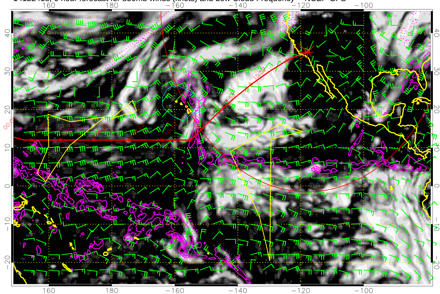
14122418, 6 hour forecast for 850mb winds (knots) and Low Cloud Frequency -- NCEP GFS
