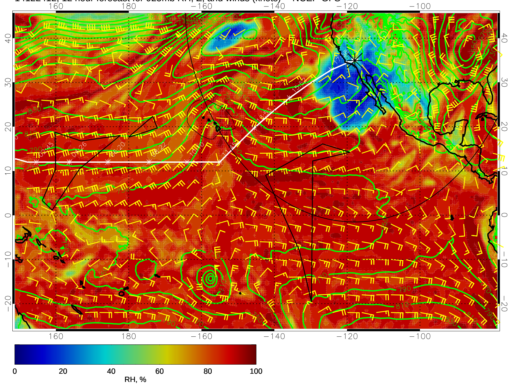
14122412, 12 hour forecast for 925mb RH, Z, and winds (knots) -- NCEP GFS
