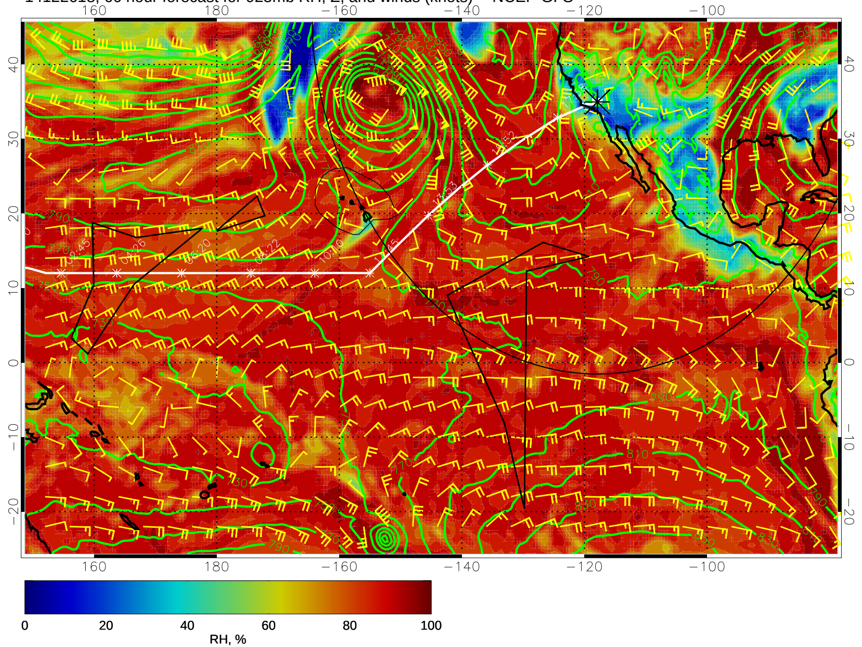
14122618, 66 hour forecast for 925mb RH, Z, and winds (knots) -- NCEP GFS
