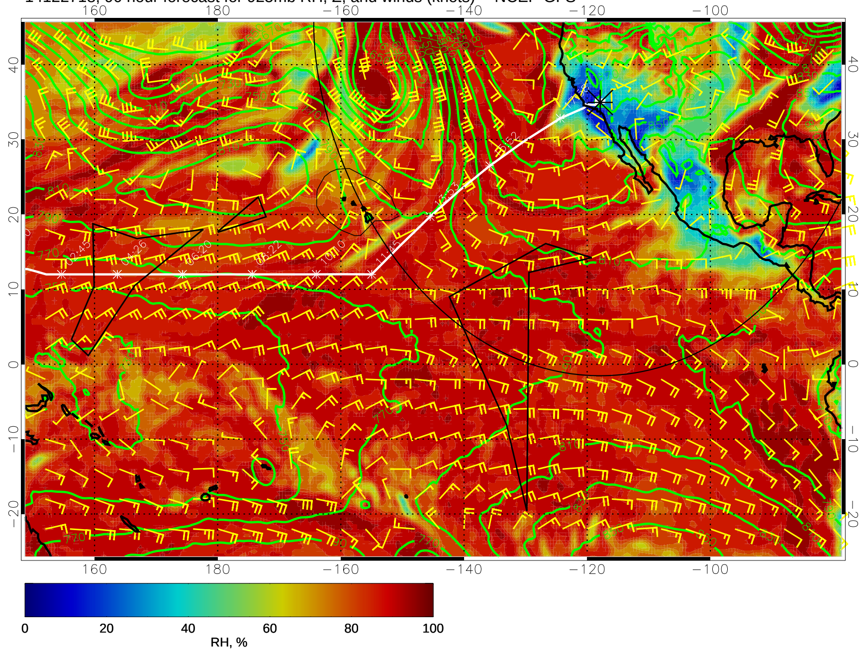
14122718, 90 hour forecast for 925mb RH, Z, and winds (knots) -- NCEP GFS
