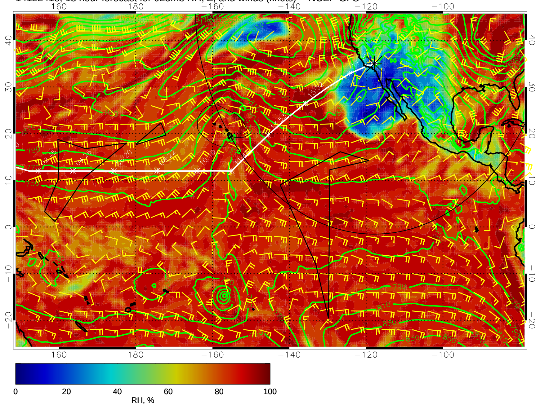
14122418, 18 hour forecast for 925mb RH, Z, and winds (knots) -- NCEP GFS
