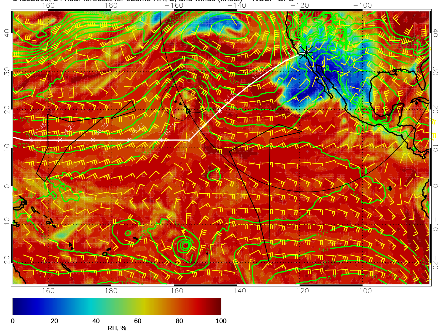
14122500, 24 hour forecast for 925mb RH, Z, and winds (knots) -- NCEP GFS
