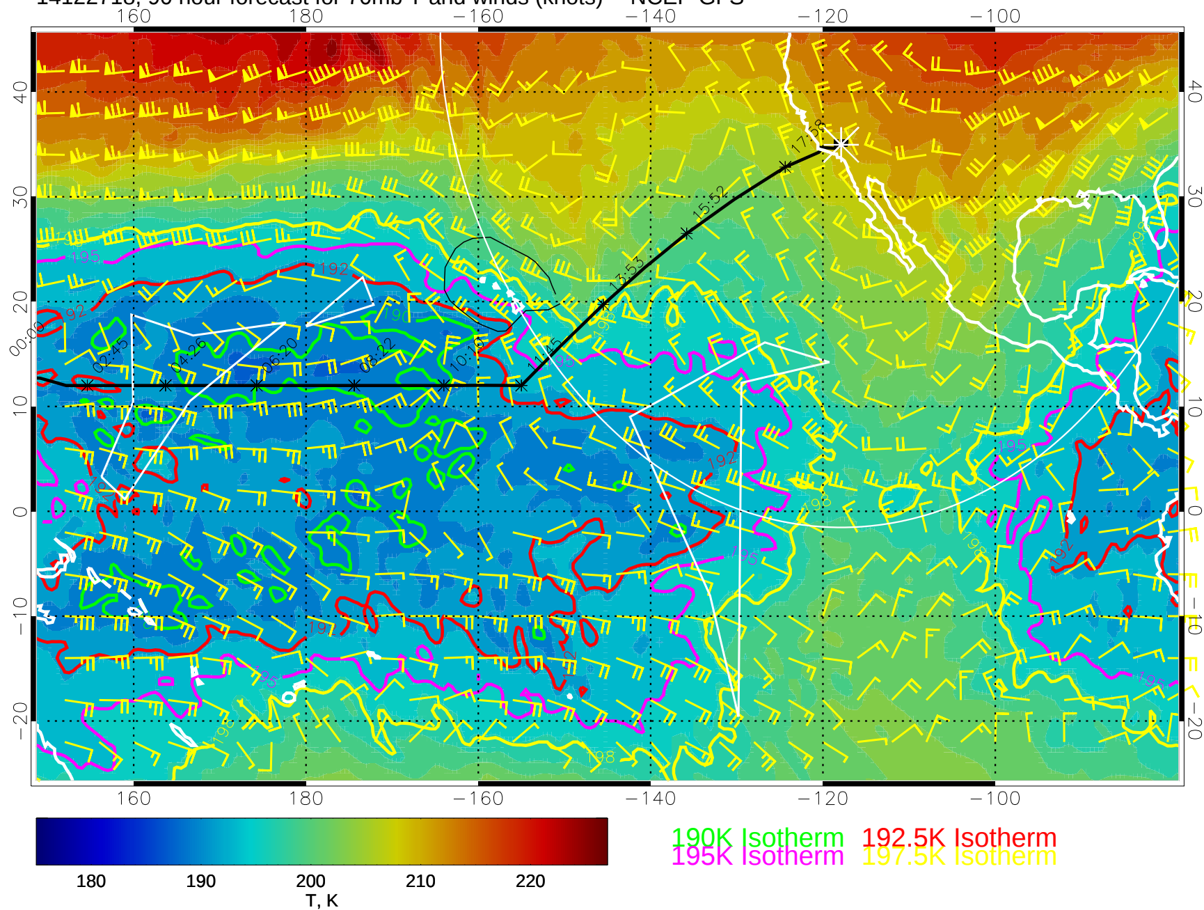
14122718, 90 hour forecast for 70mb T and winds (knots) -- NCEP GFS
