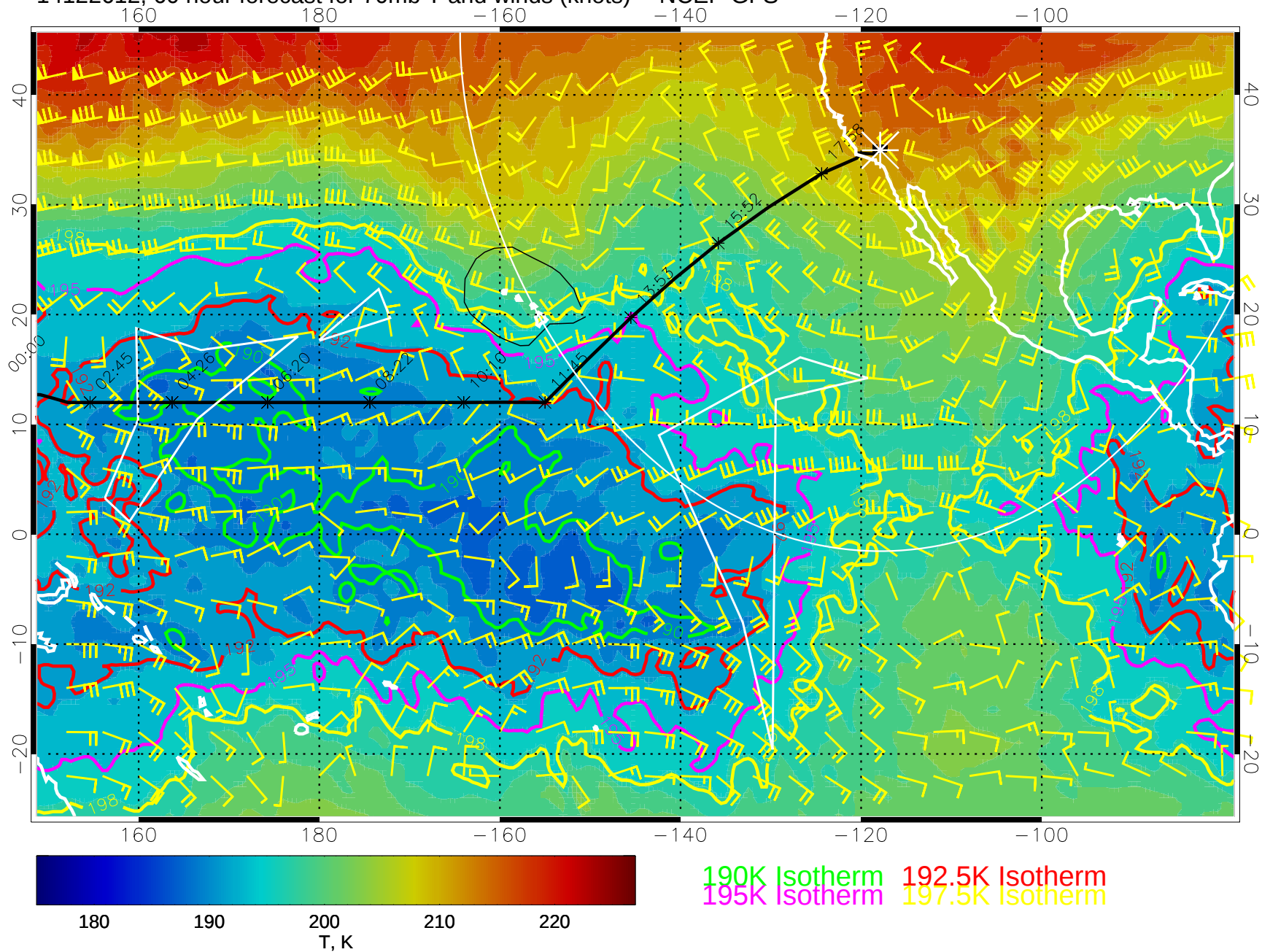
14122612, 60 hour forecast for 70mb T and winds (knots) -- NCEP GFS
