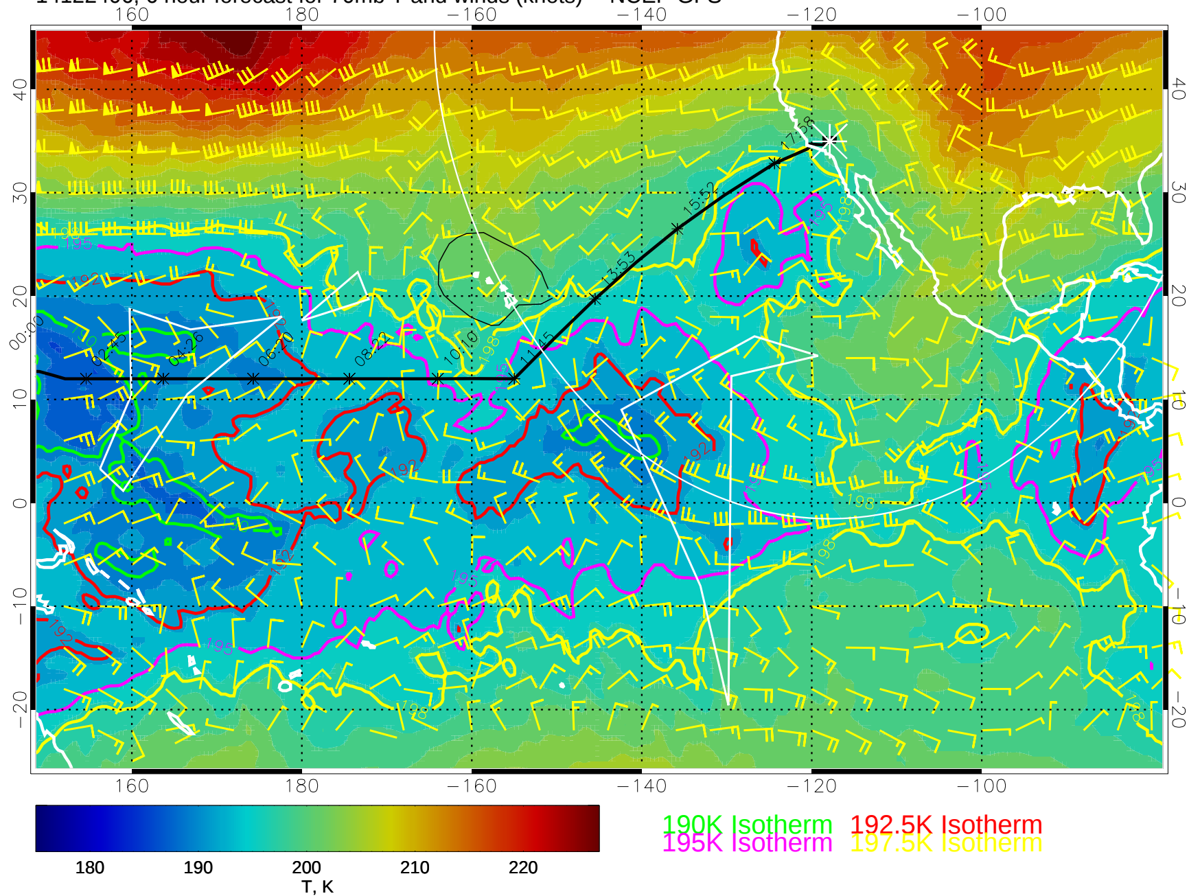
14122406, 6 hour forecast for 70mb T and winds (knots) -- NCEP GFS
