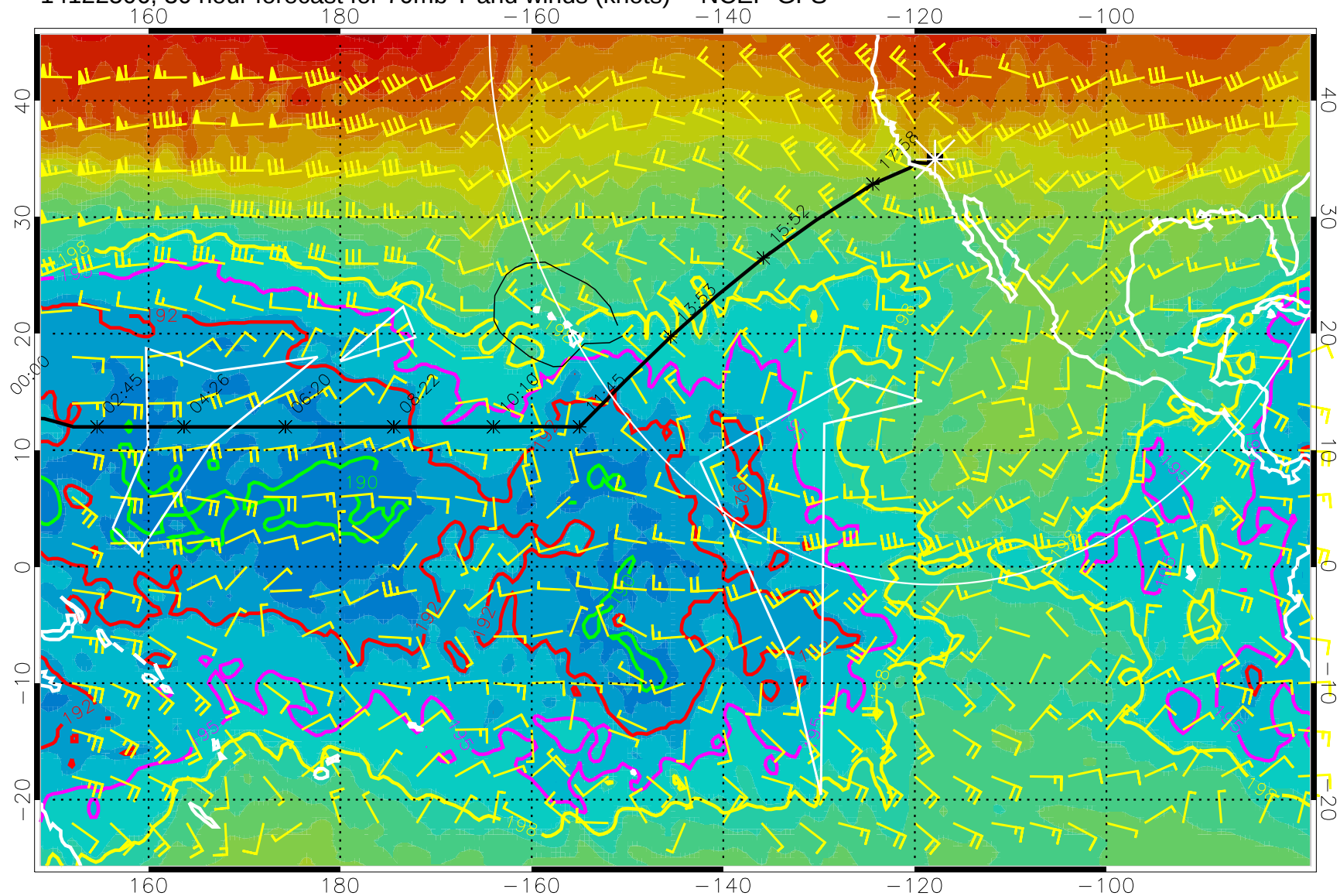
14122506, 30 hour forecast for 70mb T and winds (knots) -- NCEP GFS
