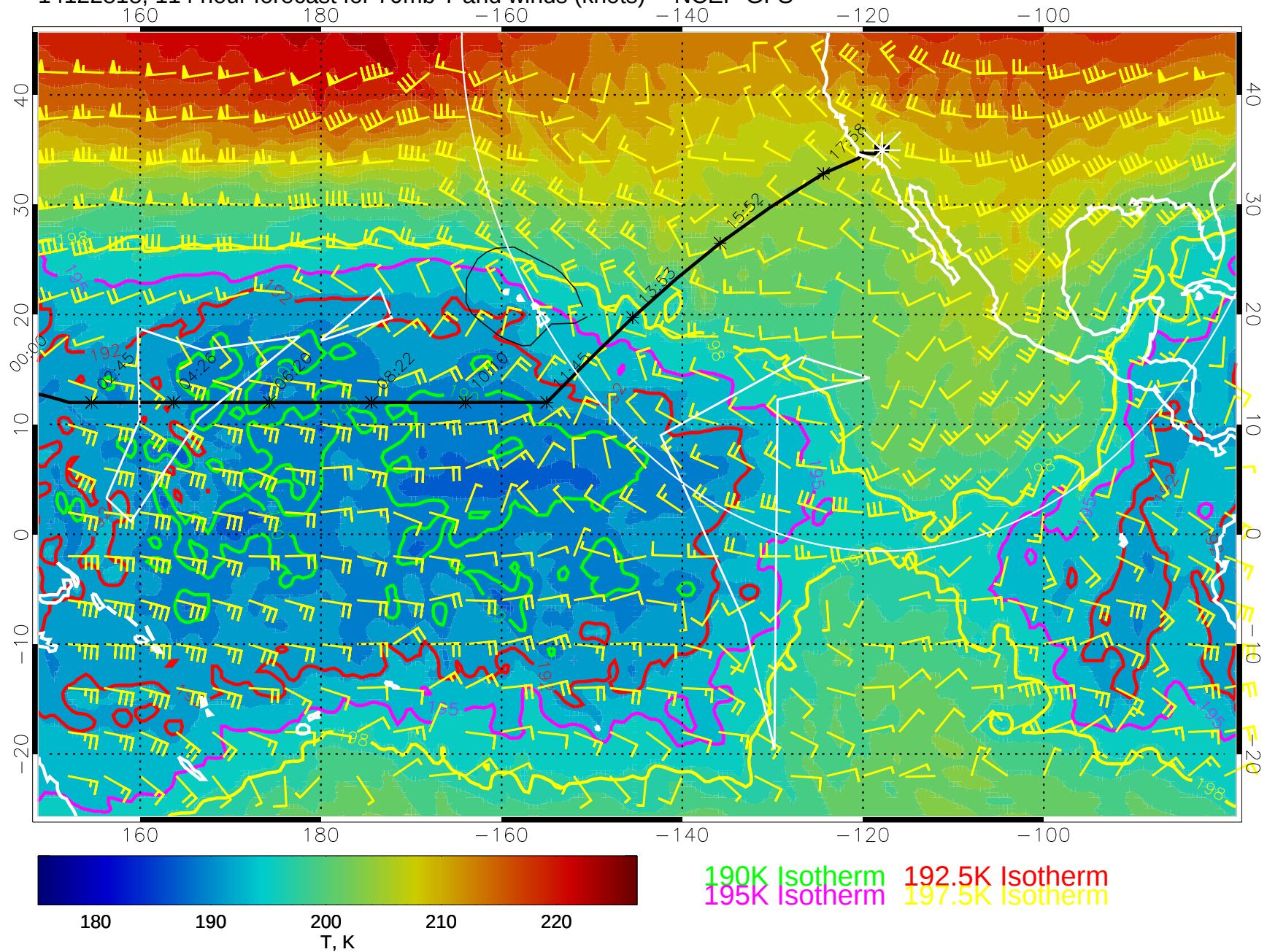
14122818, 114 hour forecast for 70mb T and winds (knots) -- NCEP GFS
