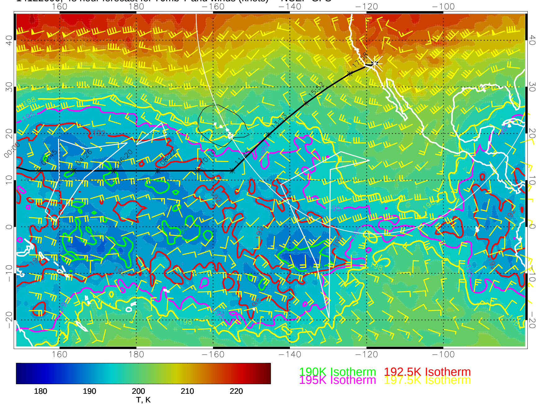
14122600, 48 hour forecast for 70mb T and winds (knots) -- NCEP GFS
