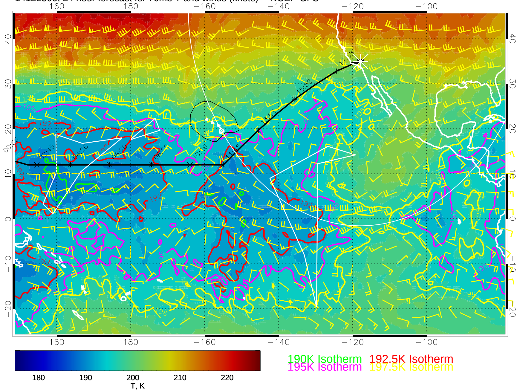
14122500, 24 hour forecast for 70mb T and winds (knots) -- NCEP GFS
