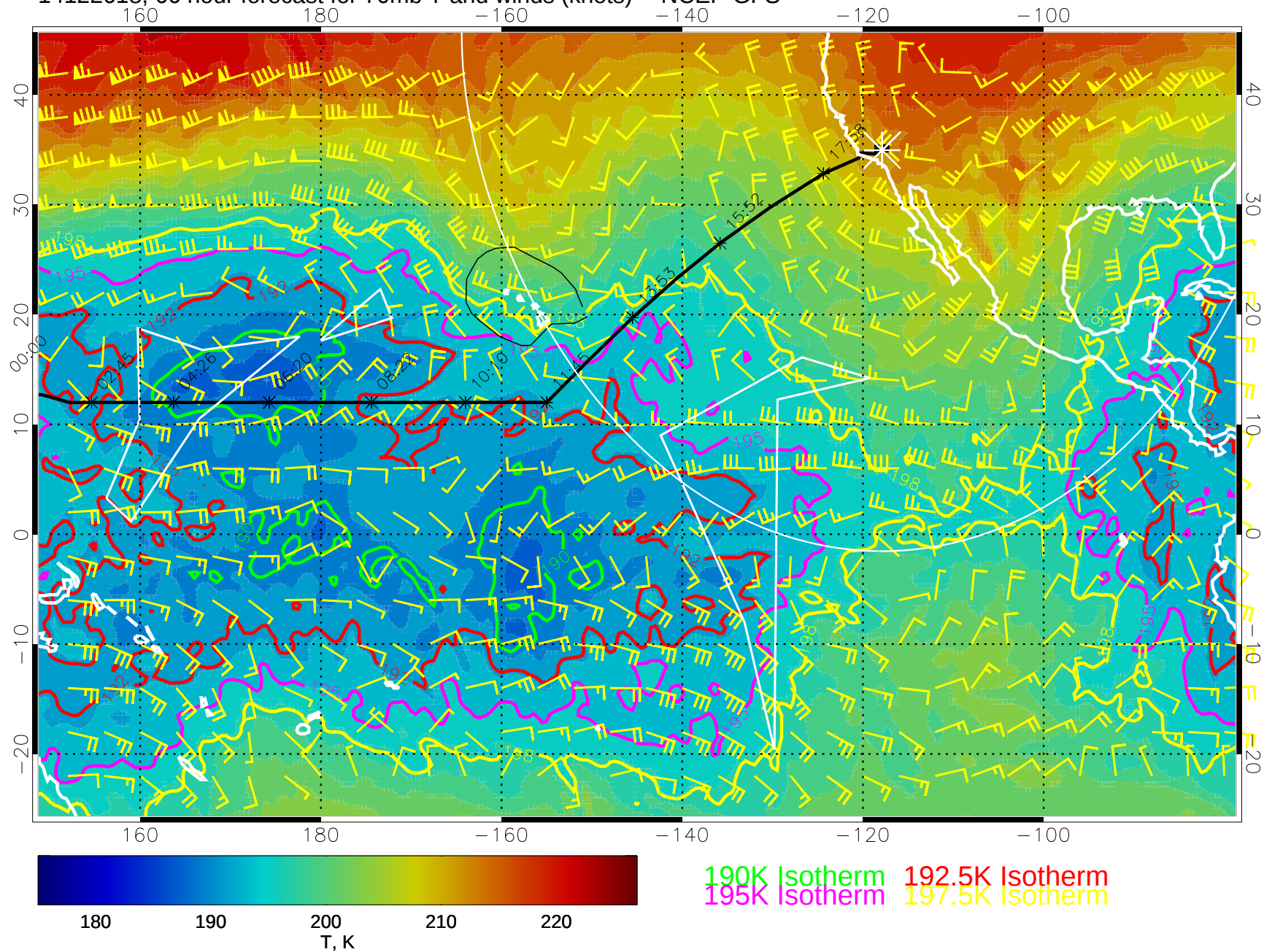
14122618, 66 hour forecast for 70mb T and winds (knots) -- NCEP GFS
