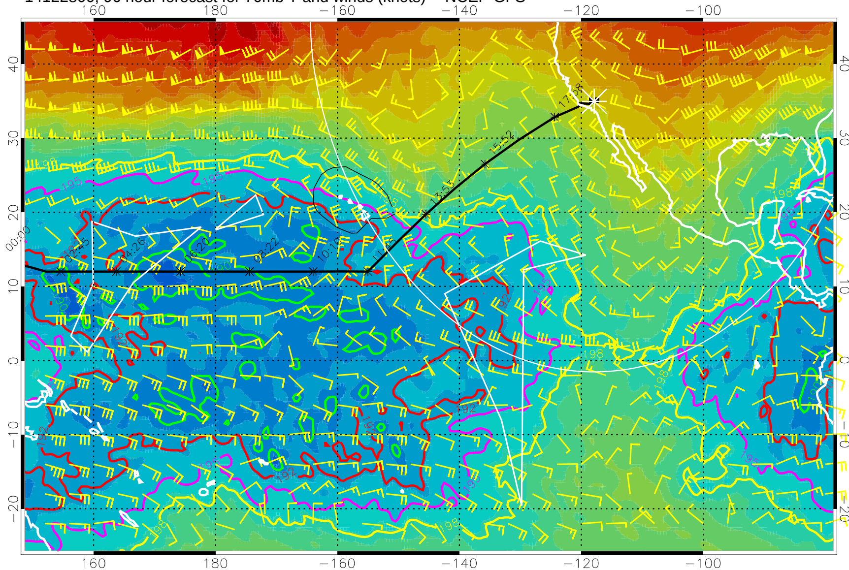
14122800, 96 hour forecast for 70mb T and winds (knots) -- NCEP GFS
