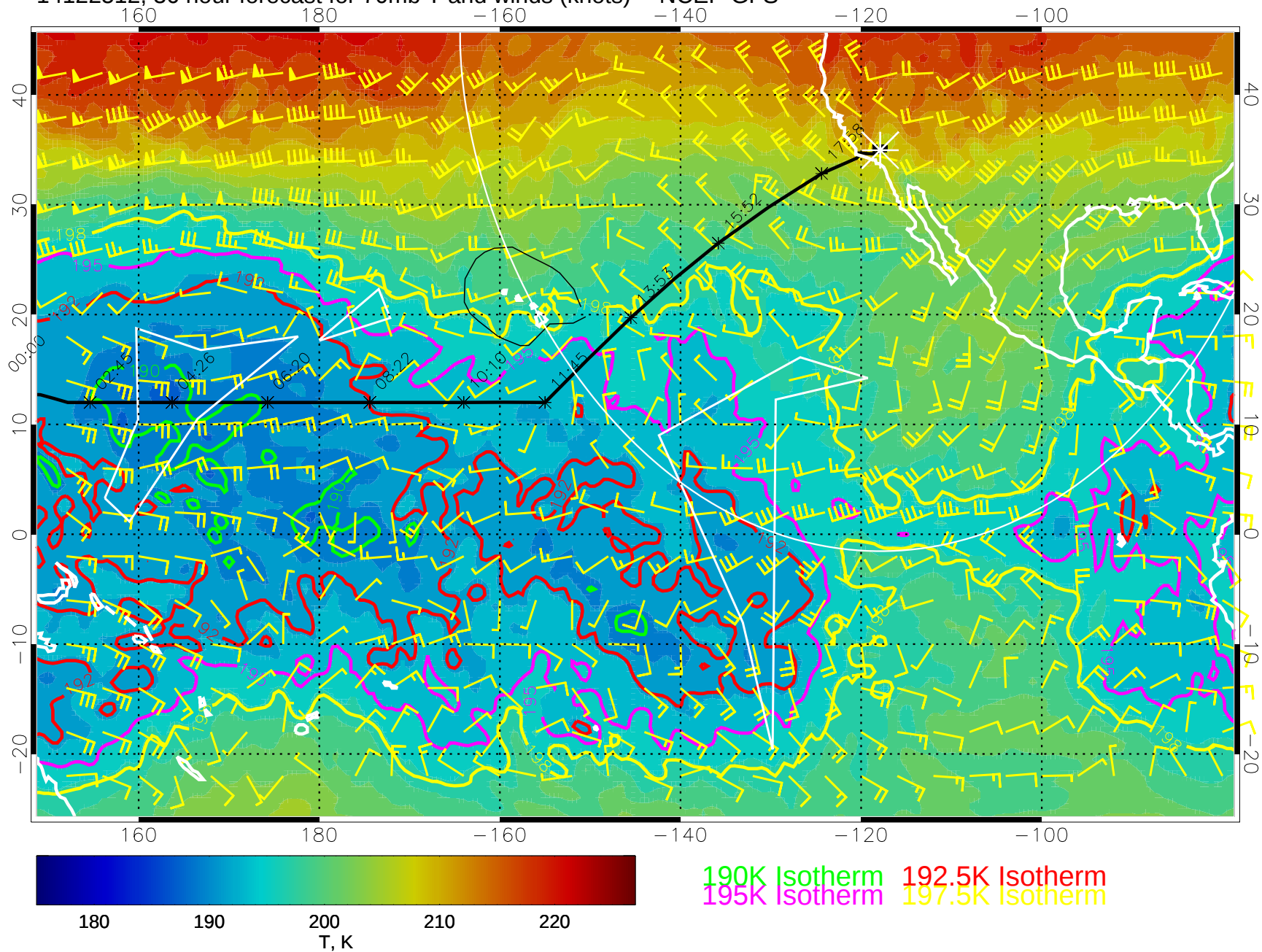
14122512, 36 hour forecast for 70mb T and winds (knots) -- NCEP GFS
