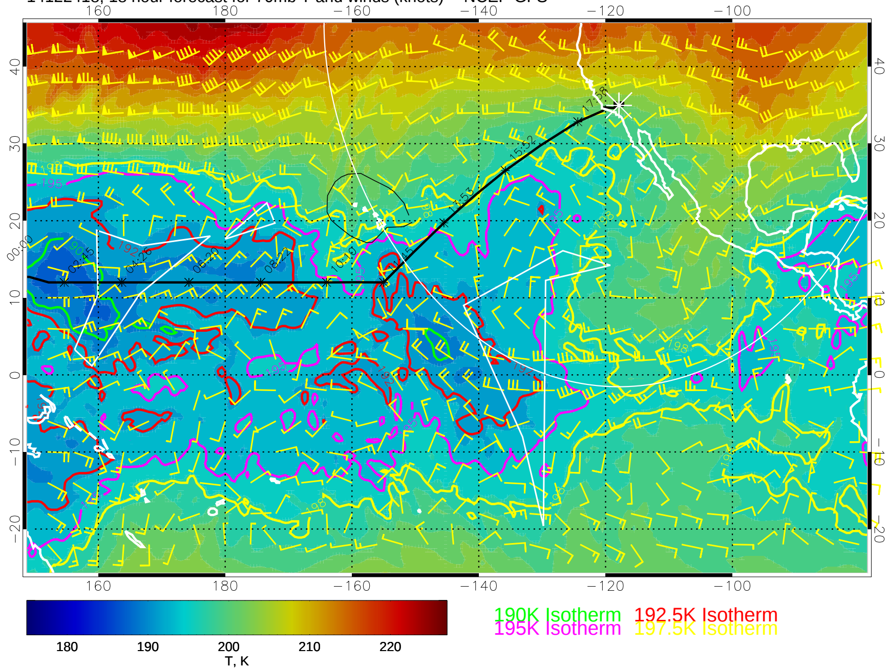
14122418, 18 hour forecast for 70mb T and winds (knots) -- NCEP GFS
