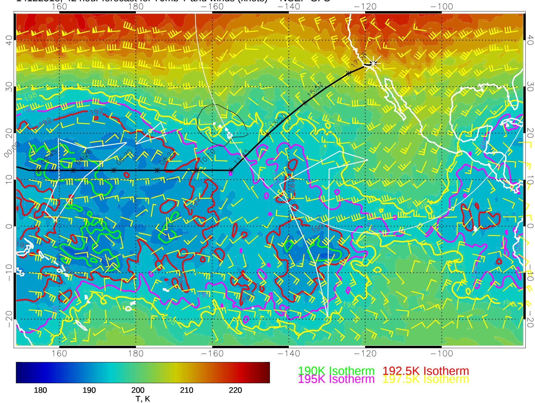
14122518, 42 hour forecast for 70mb T and winds (knots) -- NCEP GFS
