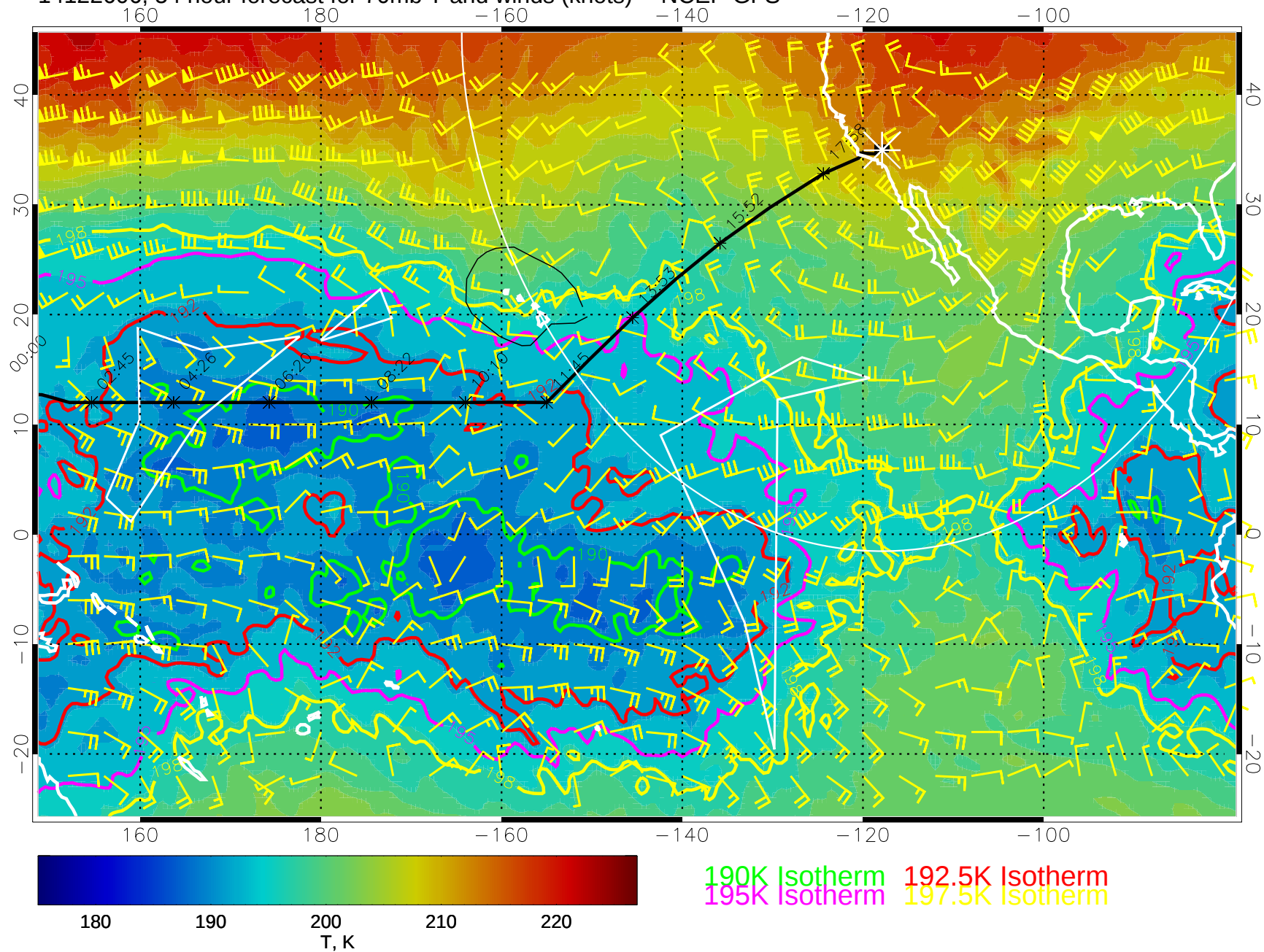
14122606, 54 hour forecast for 70mb T and winds (knots) -- NCEP GFS
