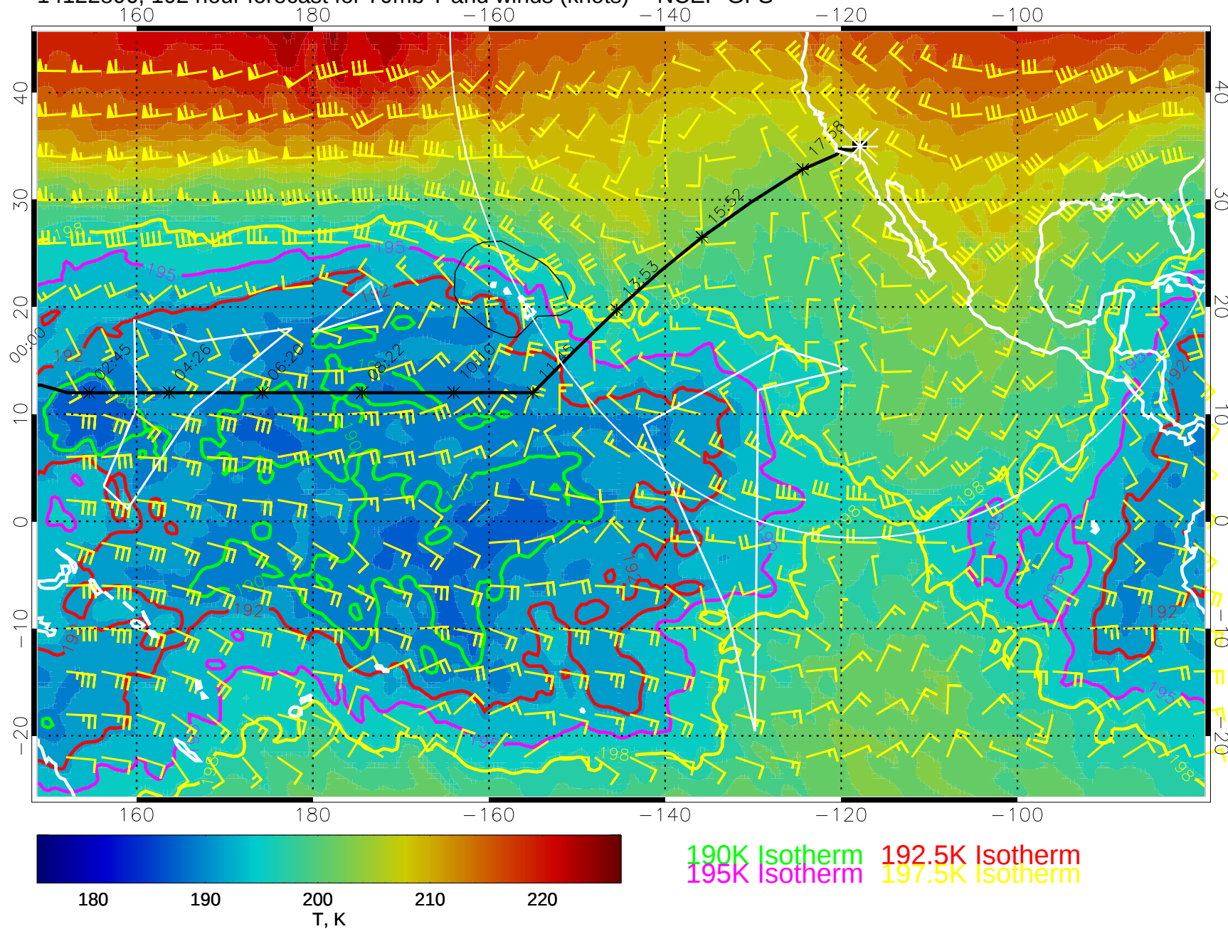
14122806, 102 hour forecast for 70mb T and winds (knots) -- NCEP GFS
