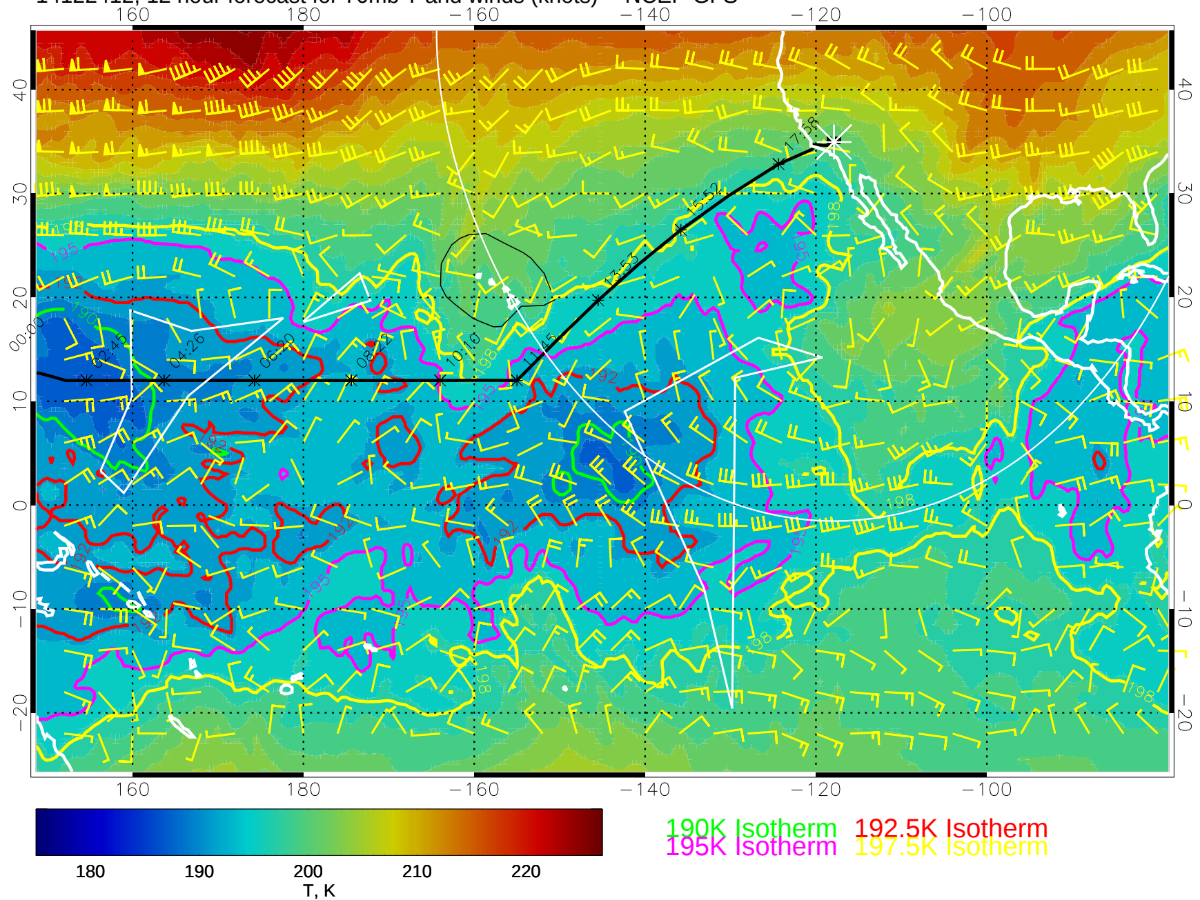
14122412, 12 hour forecast for 70mb T and winds (knots) -- NCEP GFS
