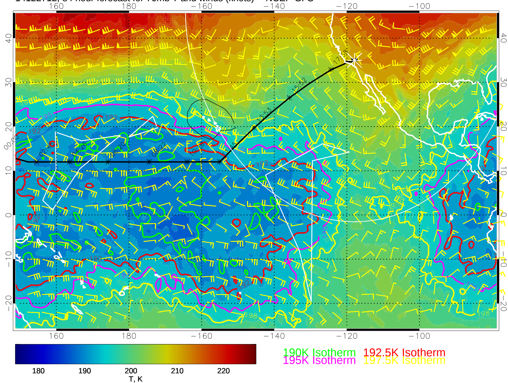
14122712, 84 hour forecast for 70mb T and winds (knots) -- NCEP GFS
