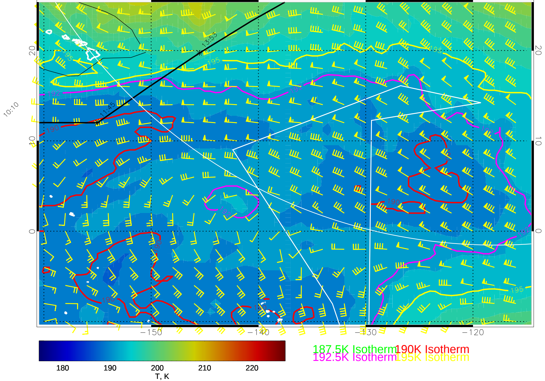
14122712, 84 hour forecast for 100mb T and winds (knots) -- NCEP GFS
