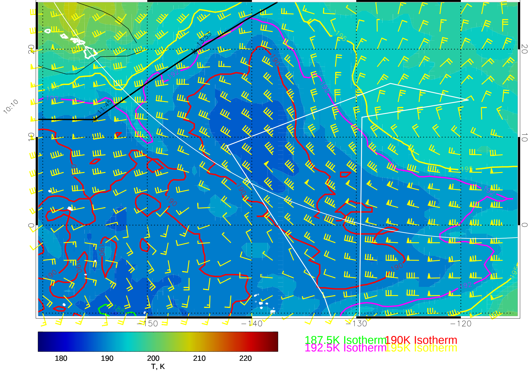
14122412, 12 hour forecast for 100mb T and winds (knots) -- NCEP GFS
