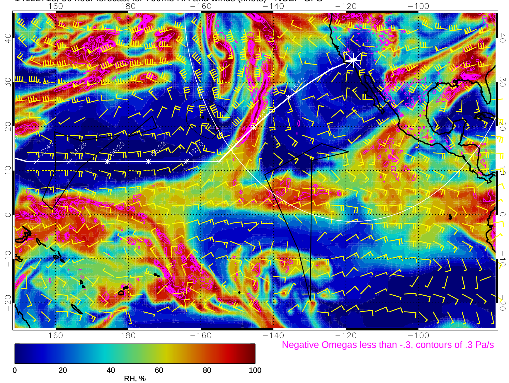
14122718, 90 hour forecast for 700mb RH and winds (knots) - NCEP GFS
