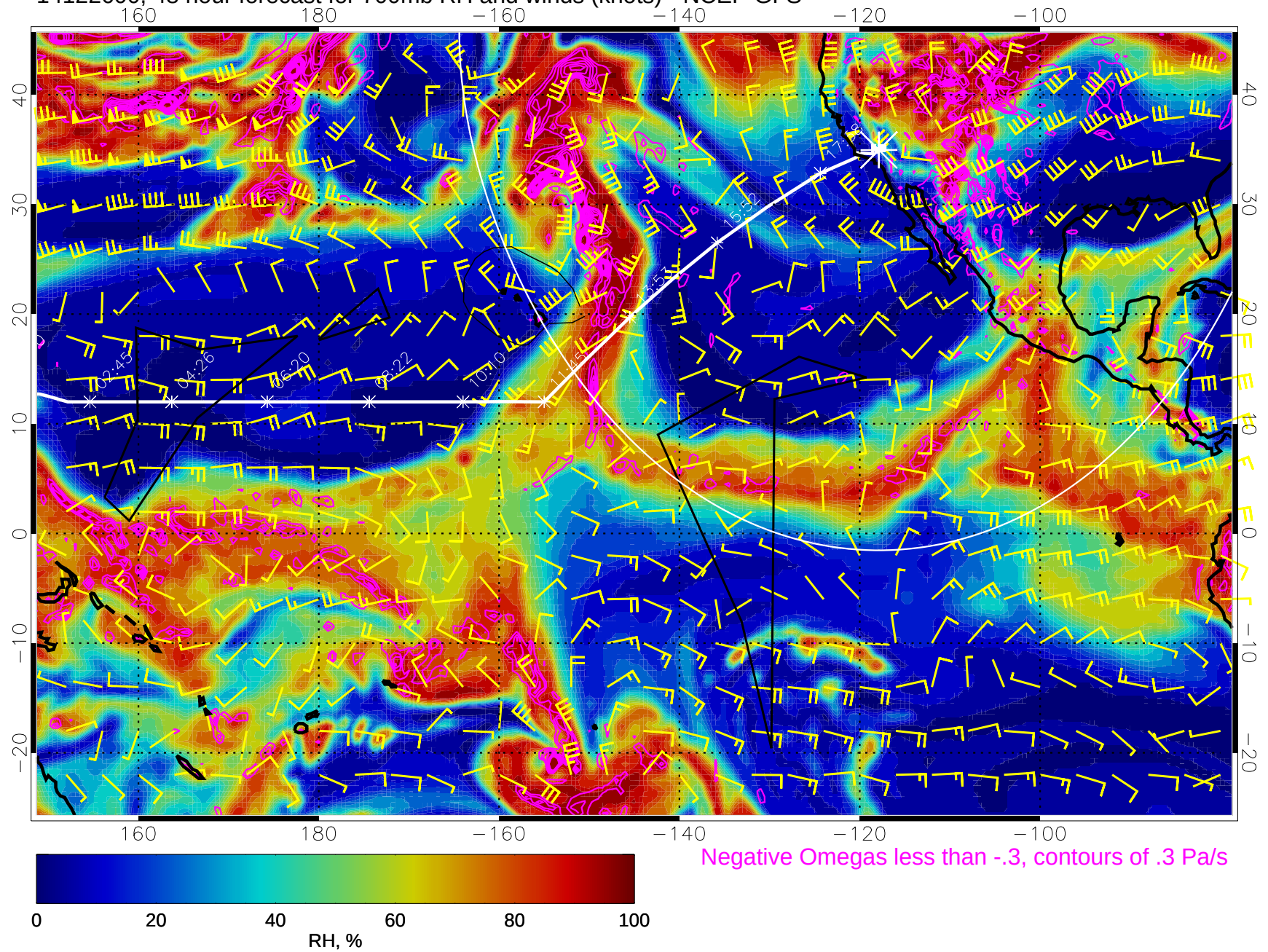
14122600, 48 hour forecast for 700mb RH and winds (knots) - NCEP GFS
