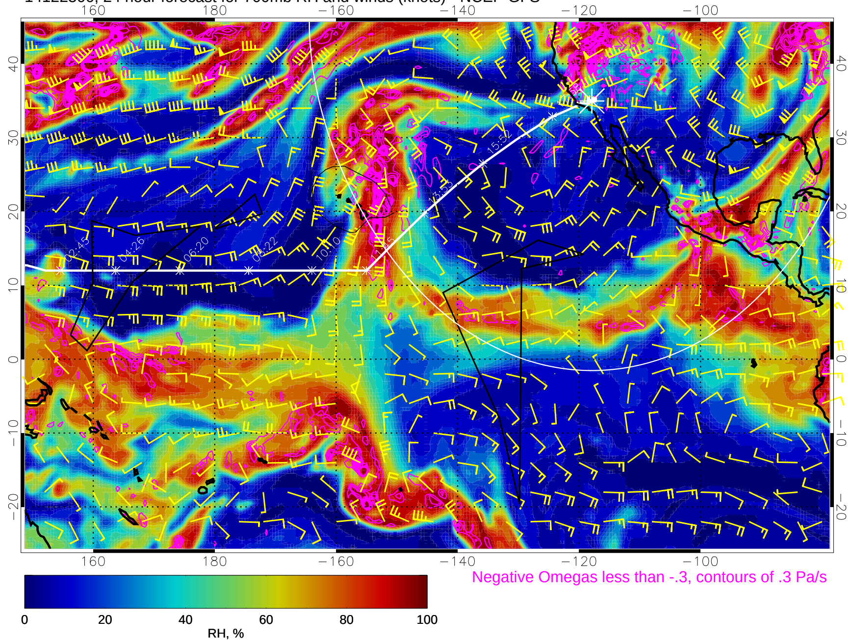
14122500, 24 hour forecast for 700mb RH and winds (knots) - NCEP GFS
