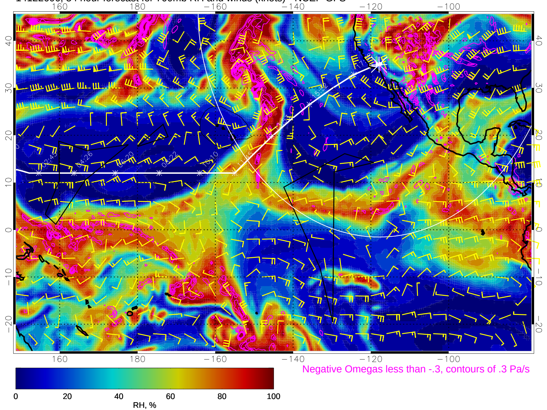
14122606, 54 hour forecast for 700mb RH and winds (knots) - NCEP GFS
