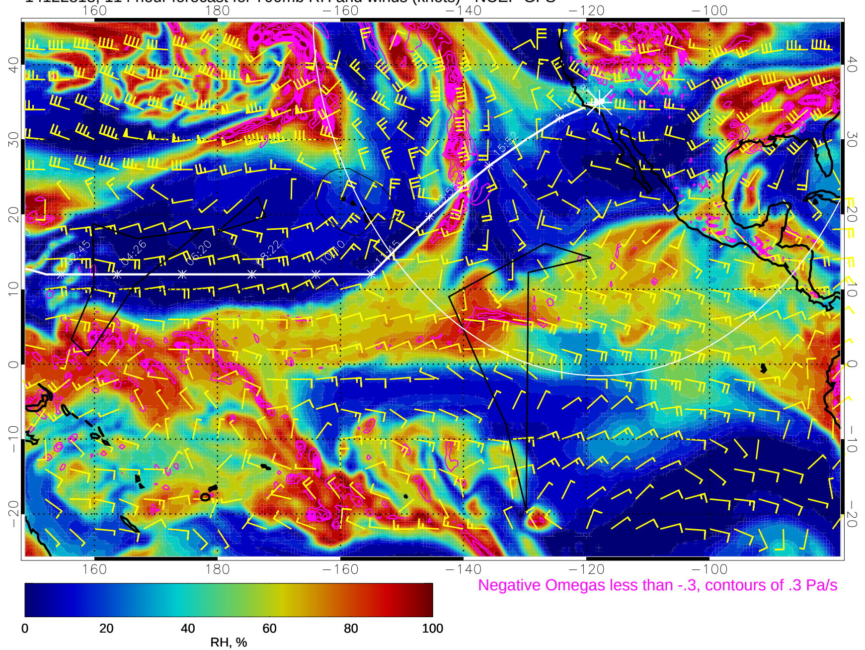
14122818, 114 hour forecast for 700mb RH and winds (knots) - NCEP GFS
