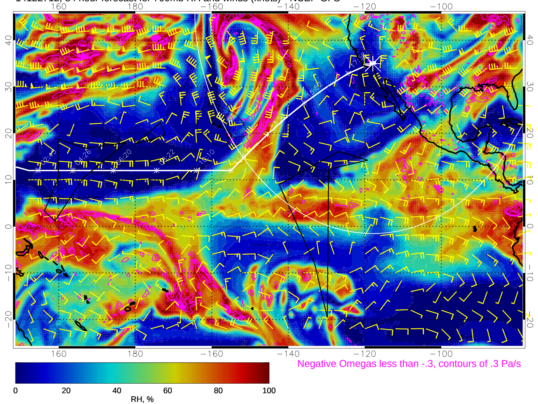
14122712, 84 hour forecast for 700mb RH and winds (knots) - NCEP GFS
