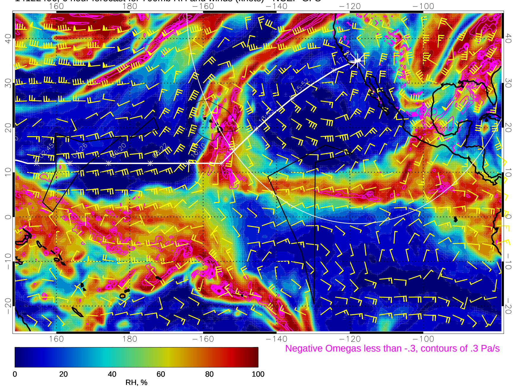
14122406, 6 hour forecast for 700mb RH and winds (knots) - NCEP GFS
