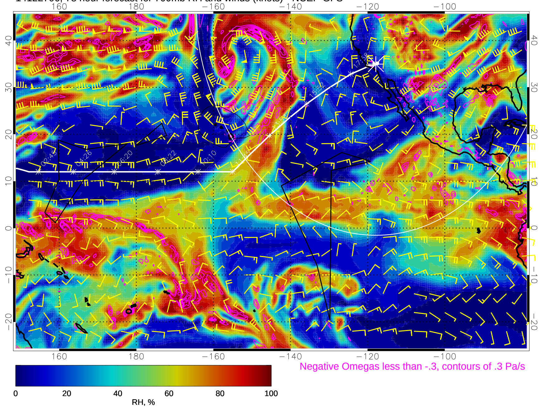
14122706, 78 hour forecast for 700mb RH and winds (knots) - NCEP GFS
