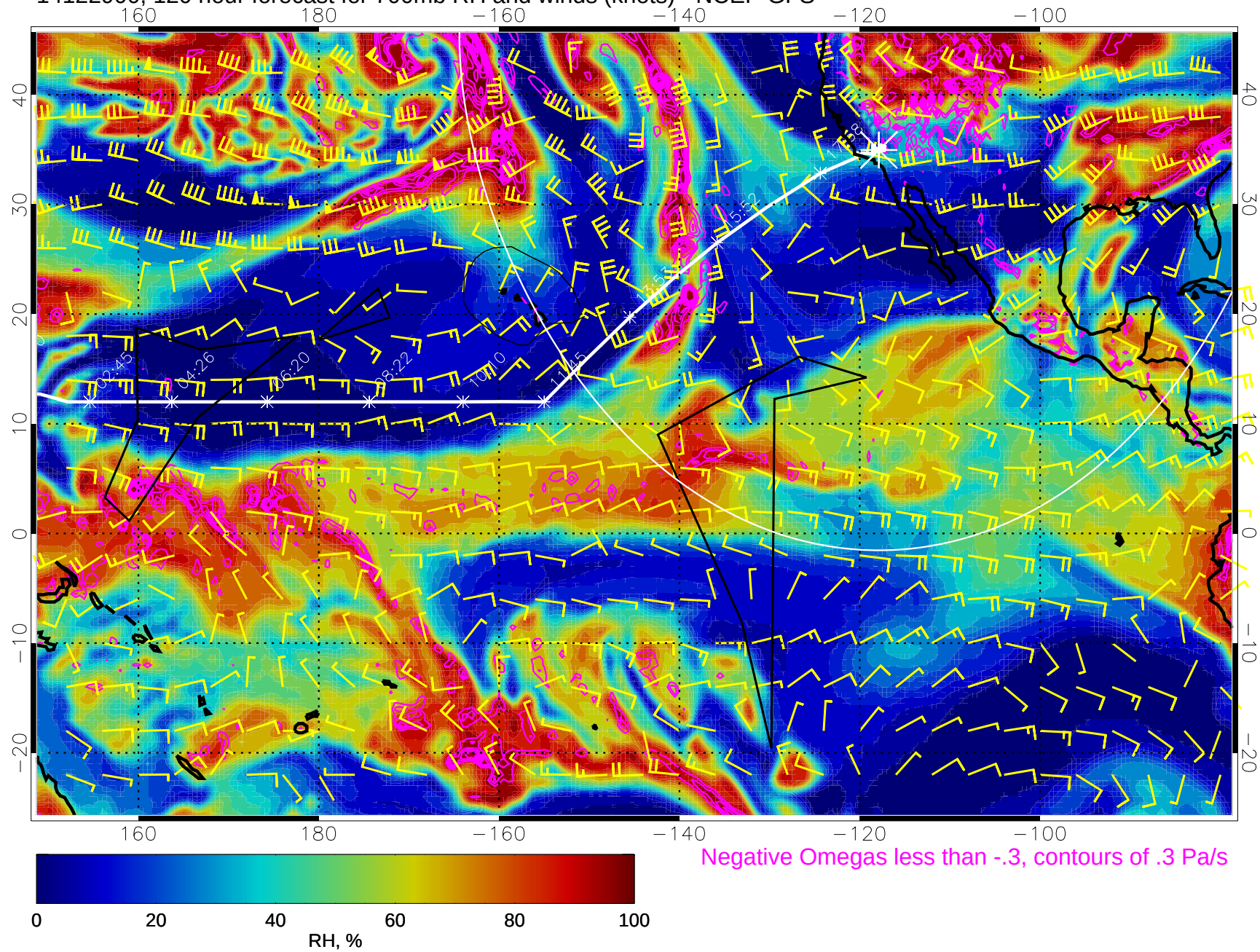
14122900, 120 hour forecast for 700mb RH and winds (knots) - NCEP GFS
