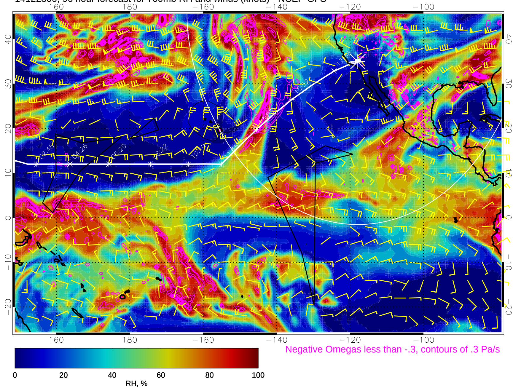
14122800, 96 hour forecast for 700mb RH and winds (knots) - NCEP GFS
