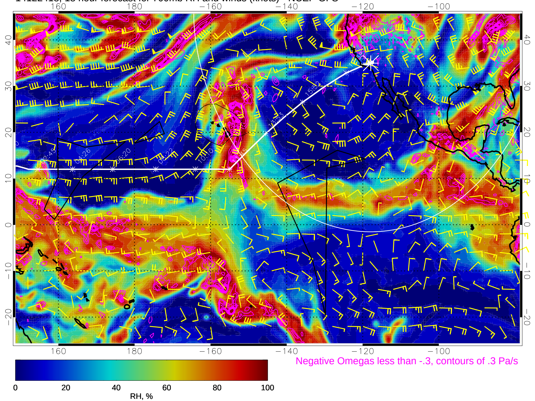
14122418, 18 hour forecast for 700mb RH and winds (knots) - NCEP GFS
