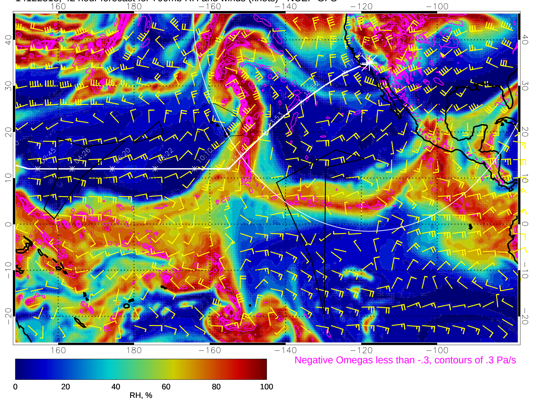
14122518, 42 hour forecast for 700mb RH and winds (knots) - NCEP GFS
