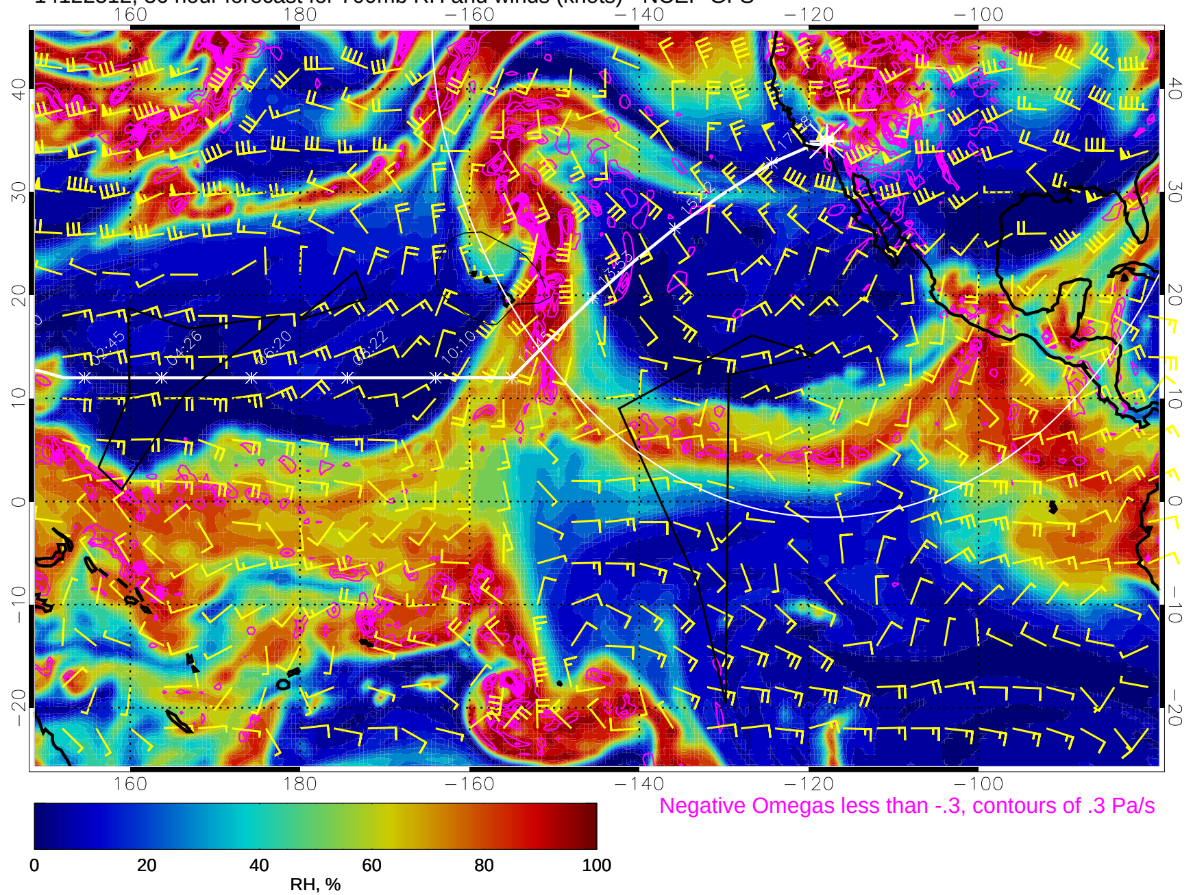
14122512, 36 hour forecast for 700mb RH and winds (knots) - NCEP GFS
