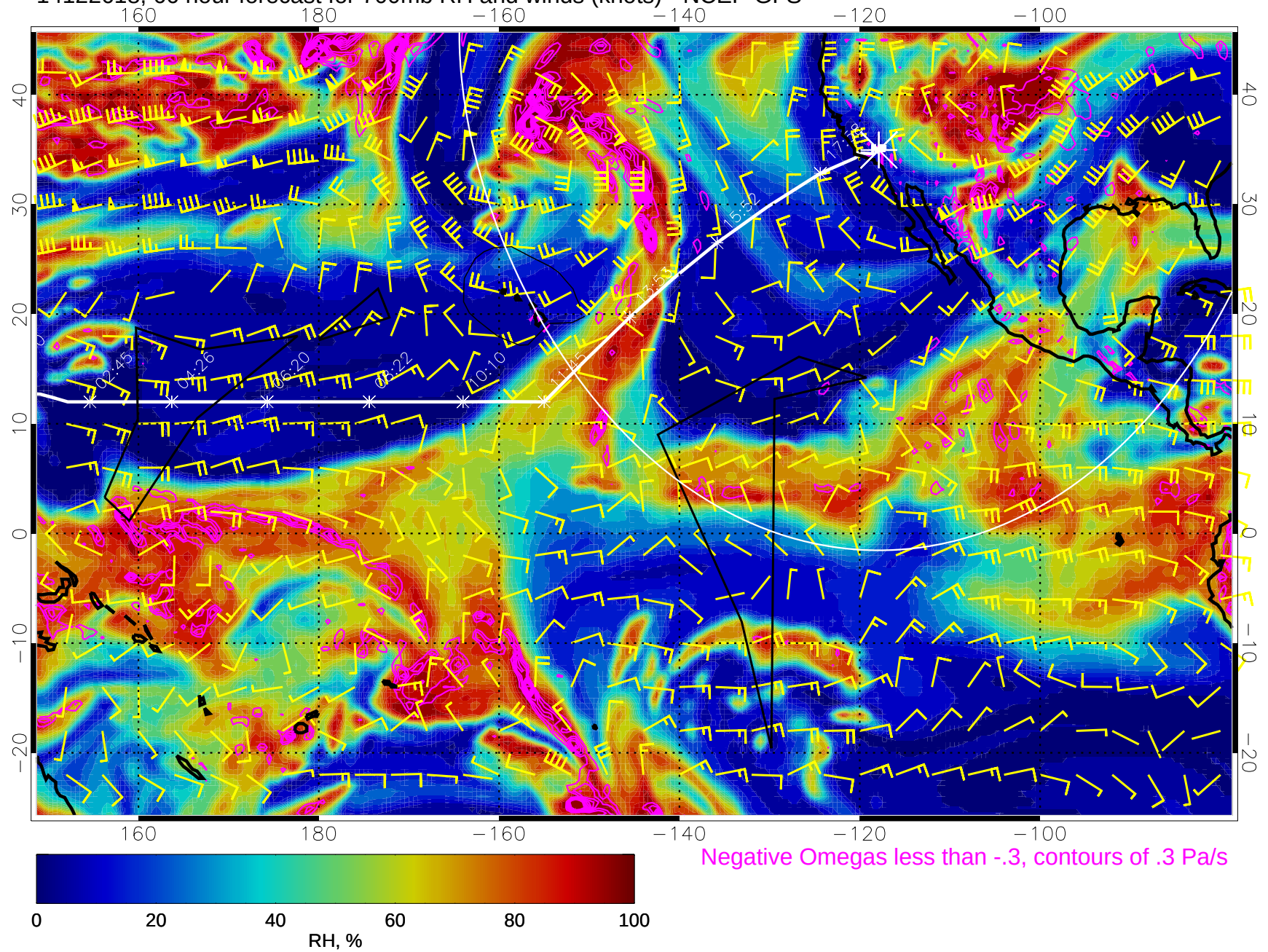
14122618, 66 hour forecast for 700mb RH and winds (knots) - NCEP GFS
