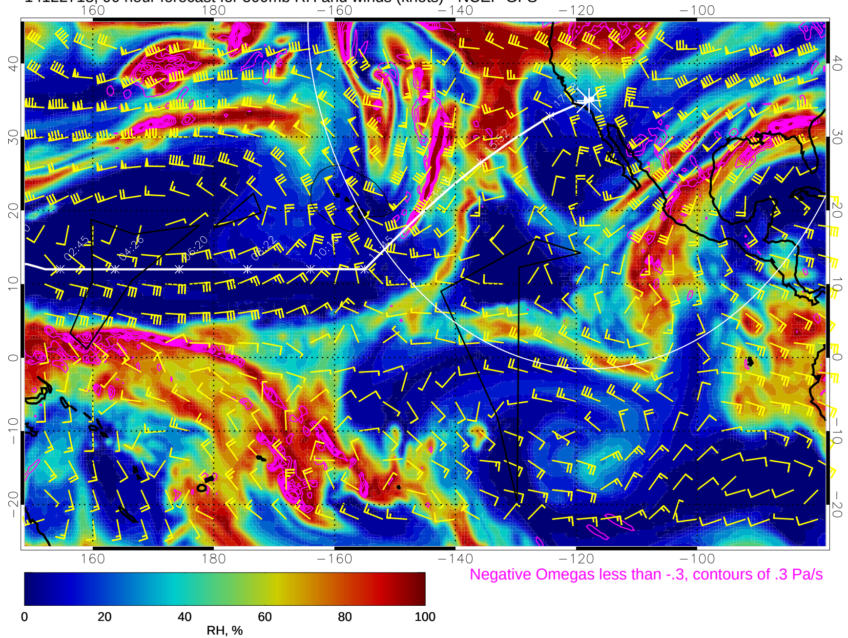
14122718, 90 hour forecast for 500mb RH and winds (knots) - NCEP GFS
