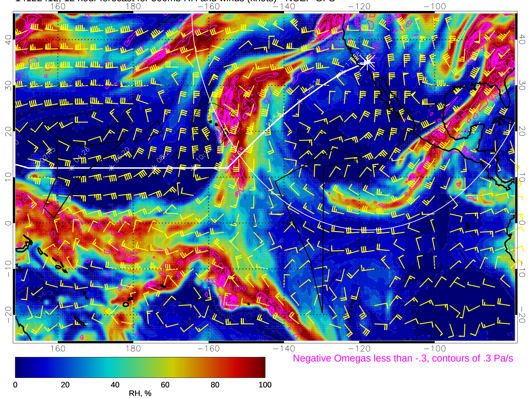
14122412, 12 hour forecast for 500mb RH and winds (knots) - NCEP GFS
