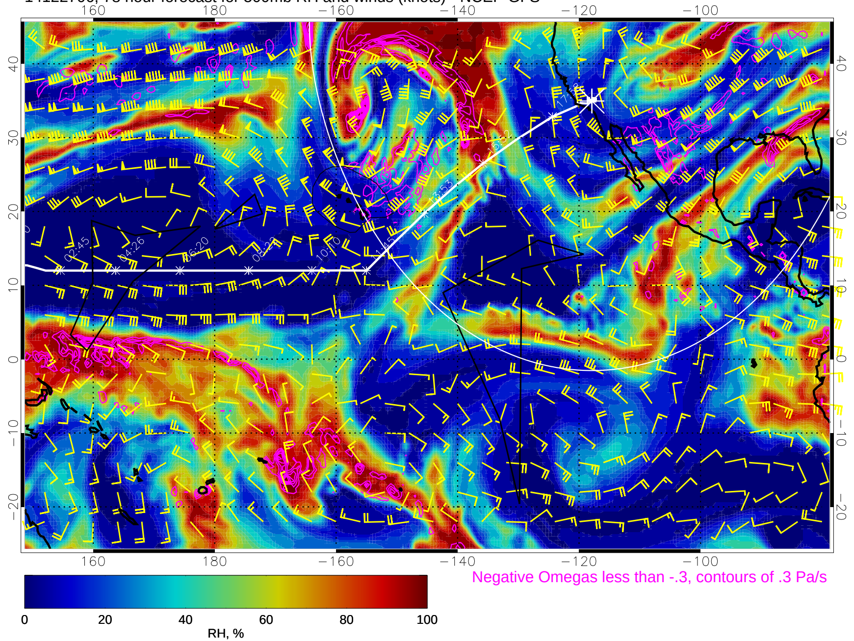
14122706, 78 hour forecast for 500mb RH and winds (knots) - NCEP GFS
