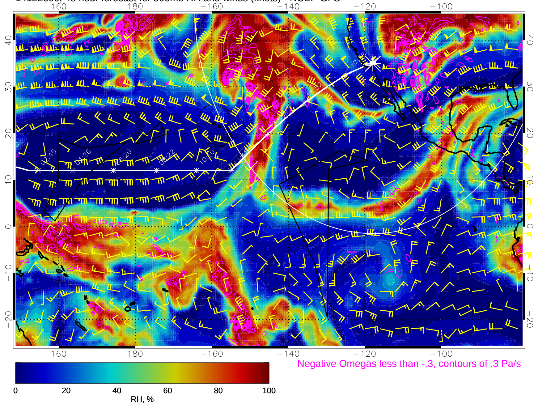
14122600, 48 hour forecast for 500mb RH and winds (knots) - NCEP GFS
