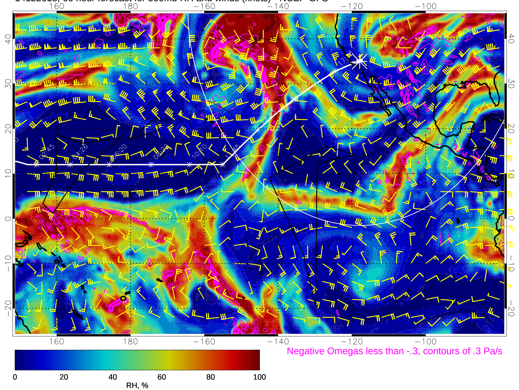
14122618, 66 hour forecast for 500mb RH and winds (knots) - NCEP GFS
