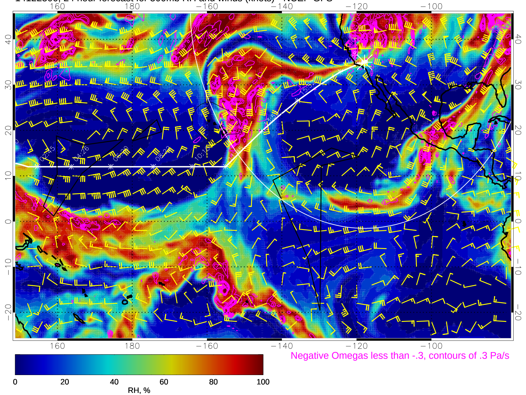
14122500, 24 hour forecast for 500mb RH and winds (knots) - NCEP GFS
