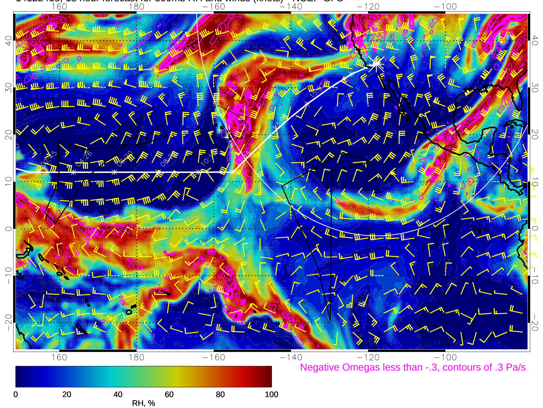
14122418, 18 hour forecast for 500mb RH and winds (knots) - NCEP GFS
