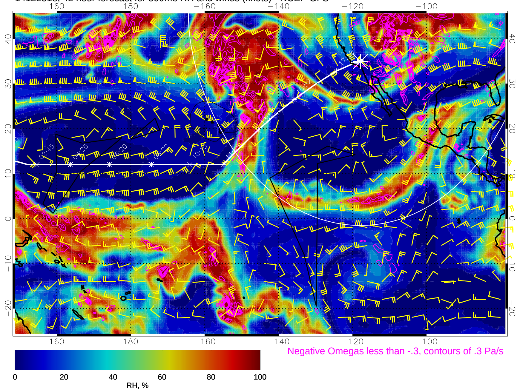
14122518, 42 hour forecast for 500mb RH and winds (knots) - NCEP GFS
