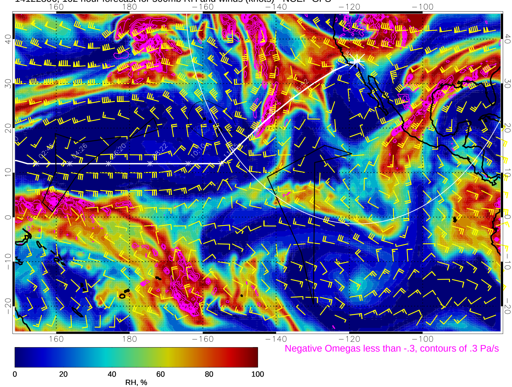
14122806, 102 hour forecast for 500mb RH and winds (knots) - NCEP GFS
