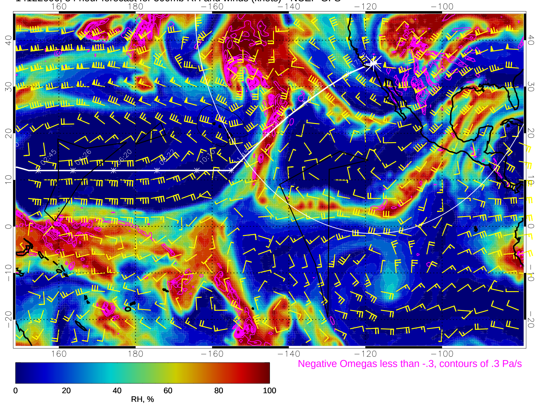
14122606, 54 hour forecast for 500mb RH and winds (knots) - NCEP GFS
