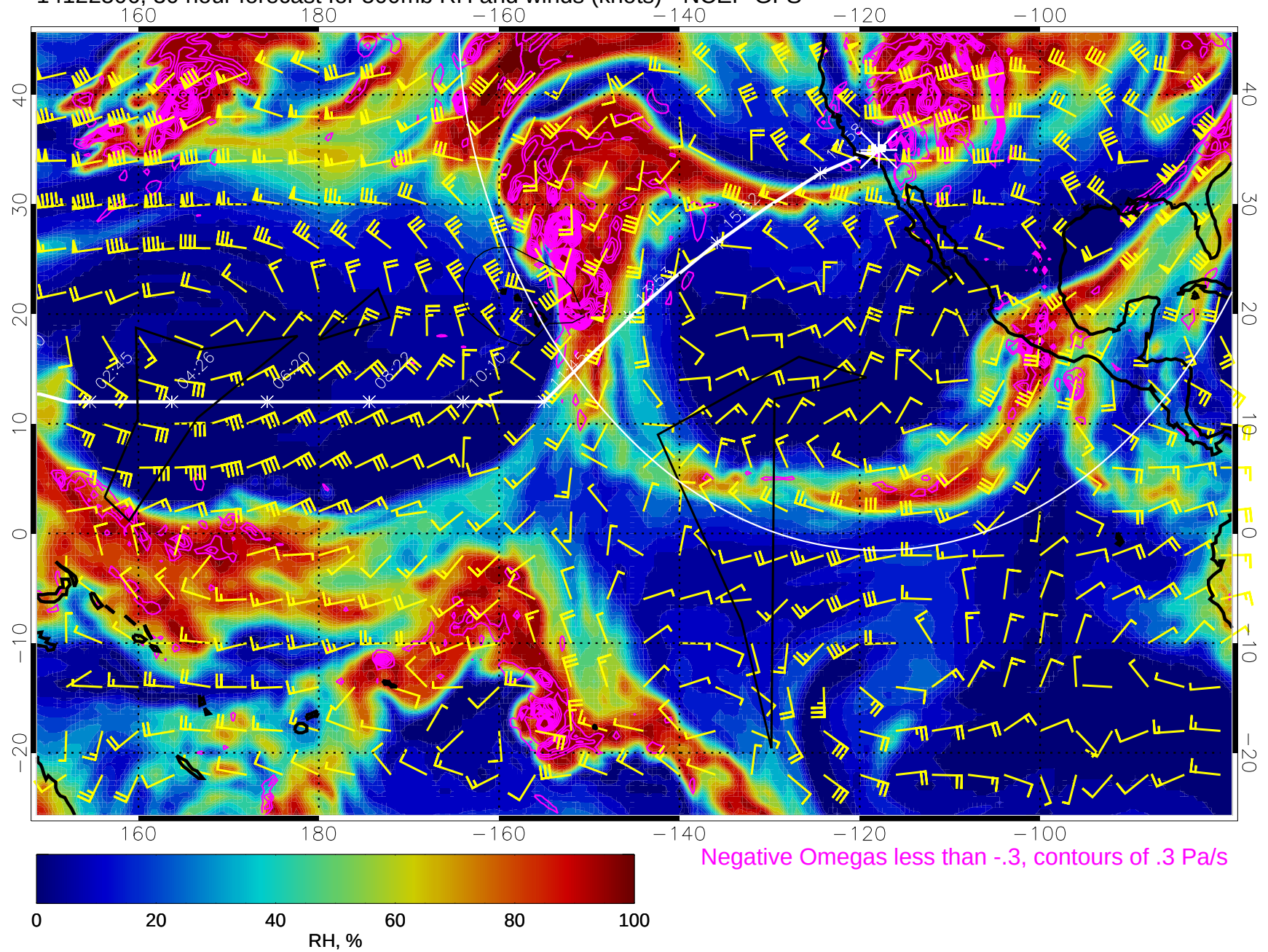
14122506, 30 hour forecast for 500mb RH and winds (knots) - NCEP GFS
