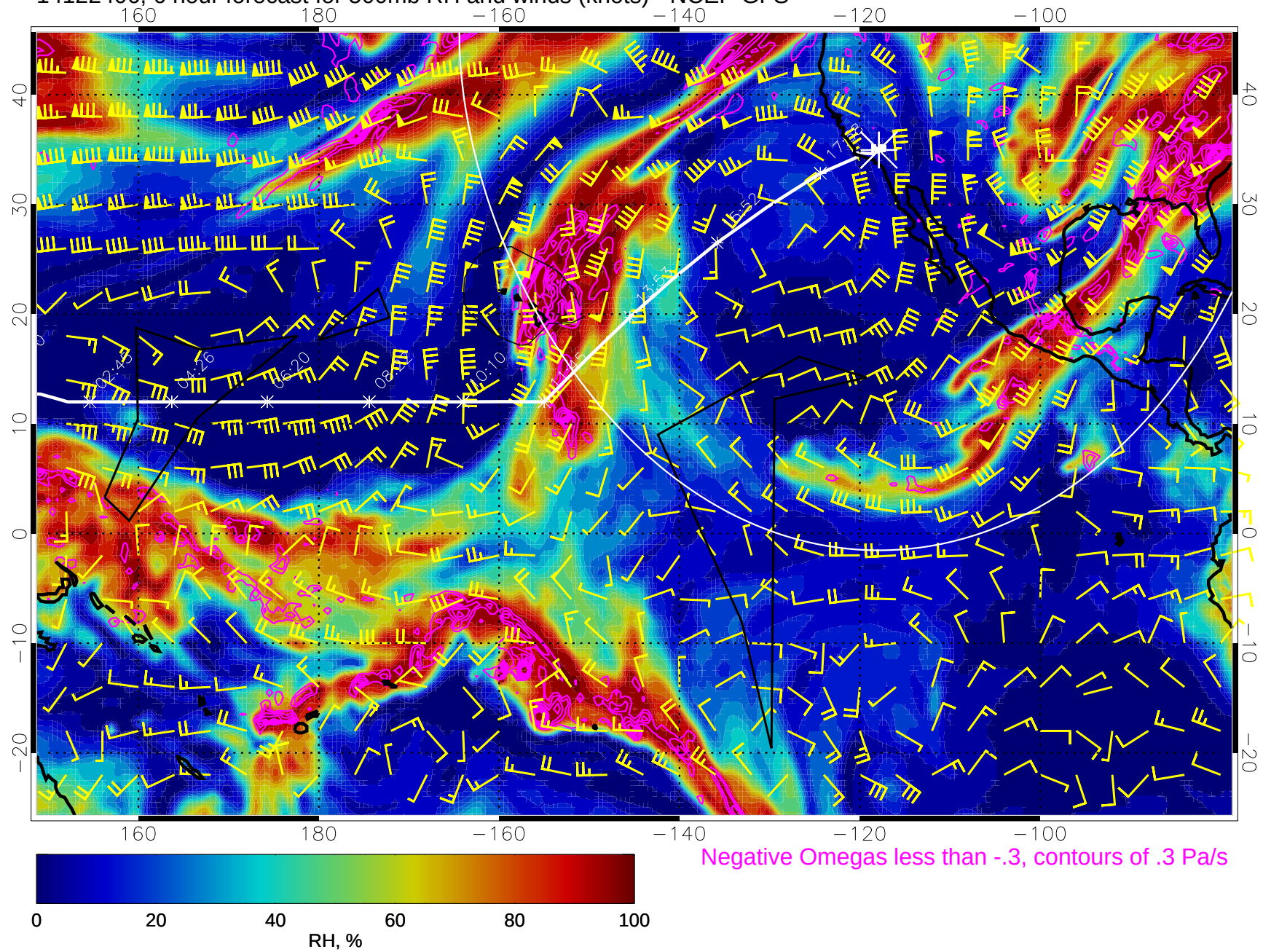
14122406, 6 hour forecast for 500mb RH and winds (knots) - NCEP GFS
