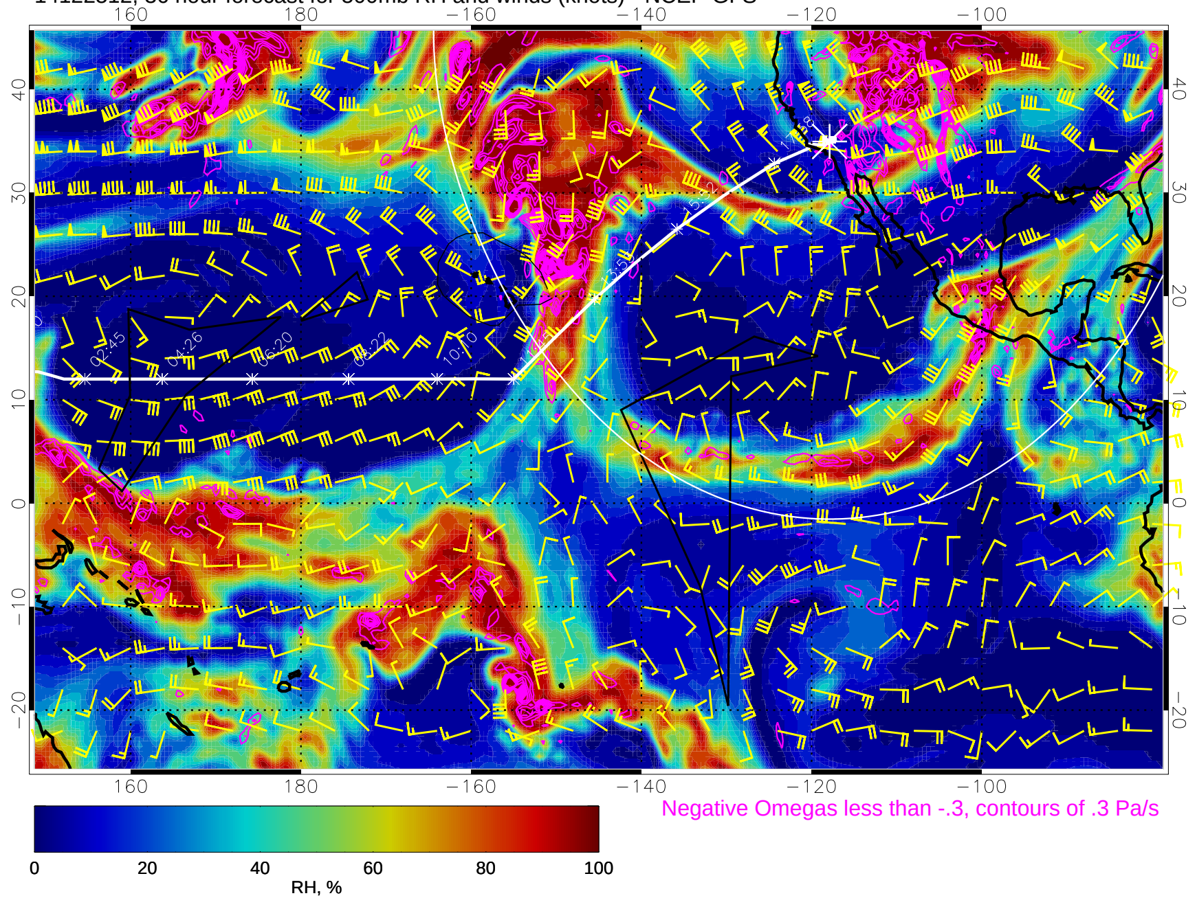
14122512, 36 hour forecast for 500mb RH and winds (knots) - NCEP GFS
