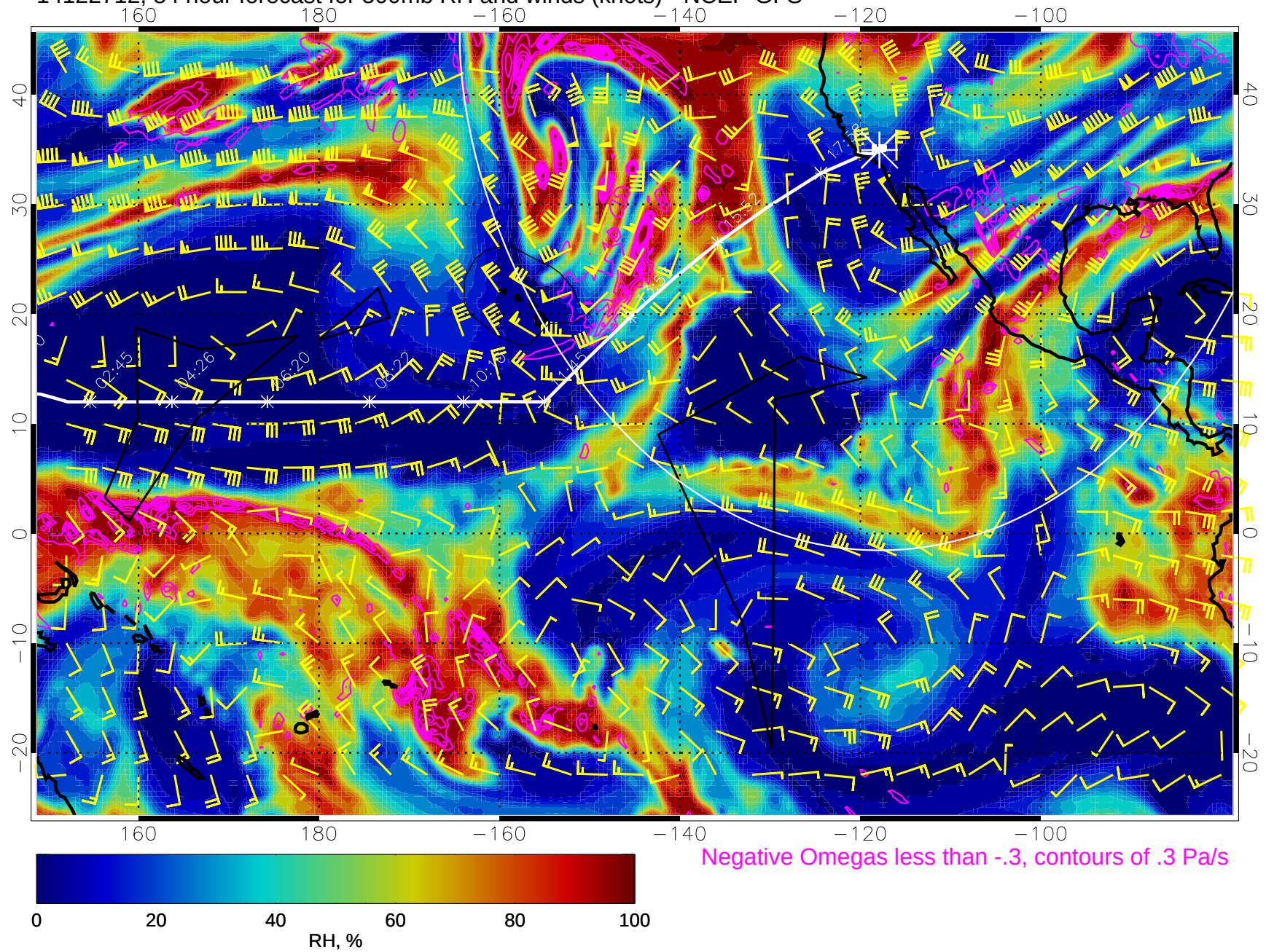
14122712, 84 hour forecast for 500mb RH and winds (knots) - NCEP GFS
