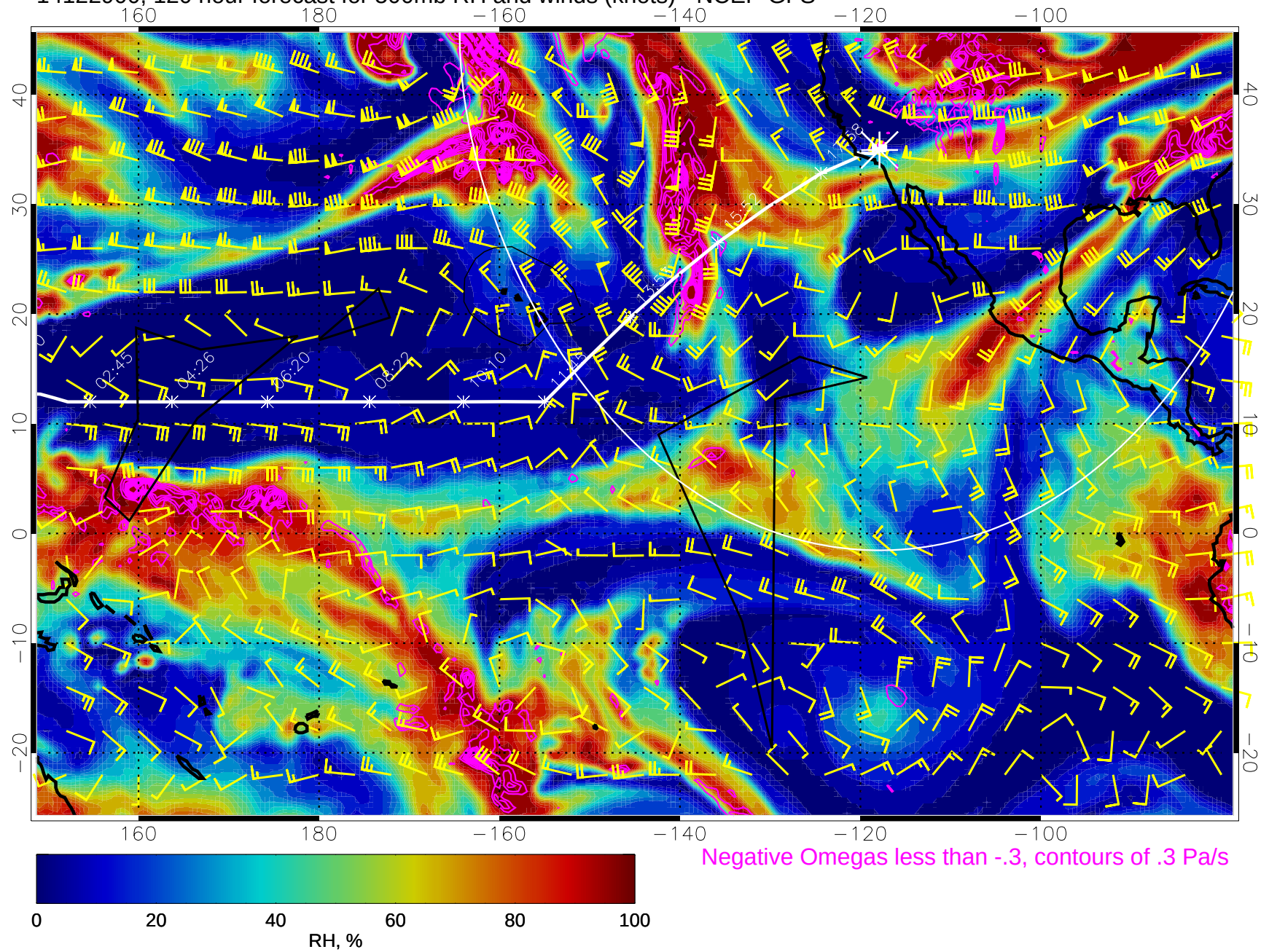
14122900, 120 hour forecast for 500mb RH and winds (knots) - NCEP GFS
