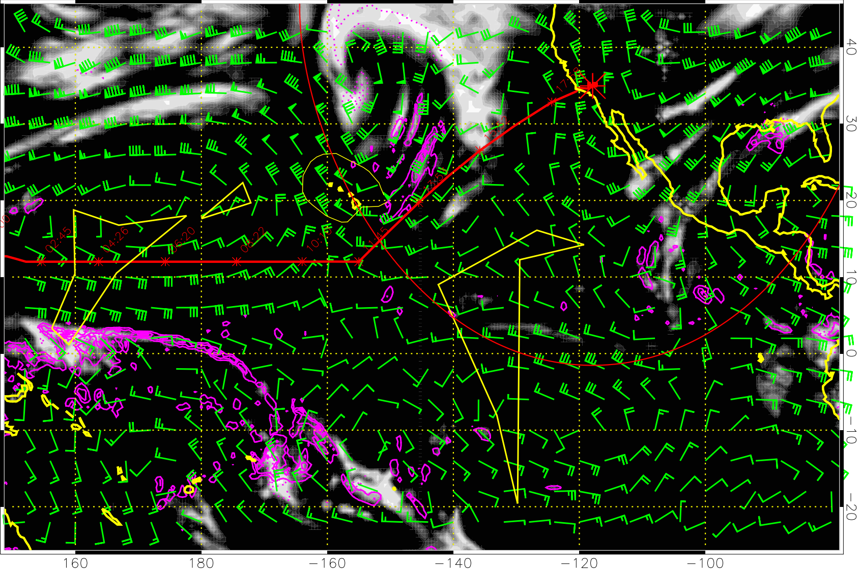
14122712, 84 hour forecast for 500mb winds (knots) and Middle Cloud Frequency -- NCEP GFS
