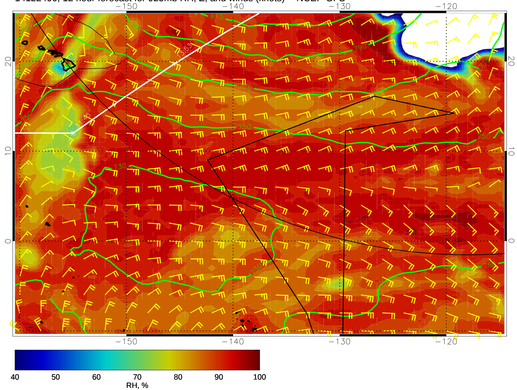
14122400, 12 hour forecast for 925mb RH, Z, and winds (knots) -- NCEP GFS
