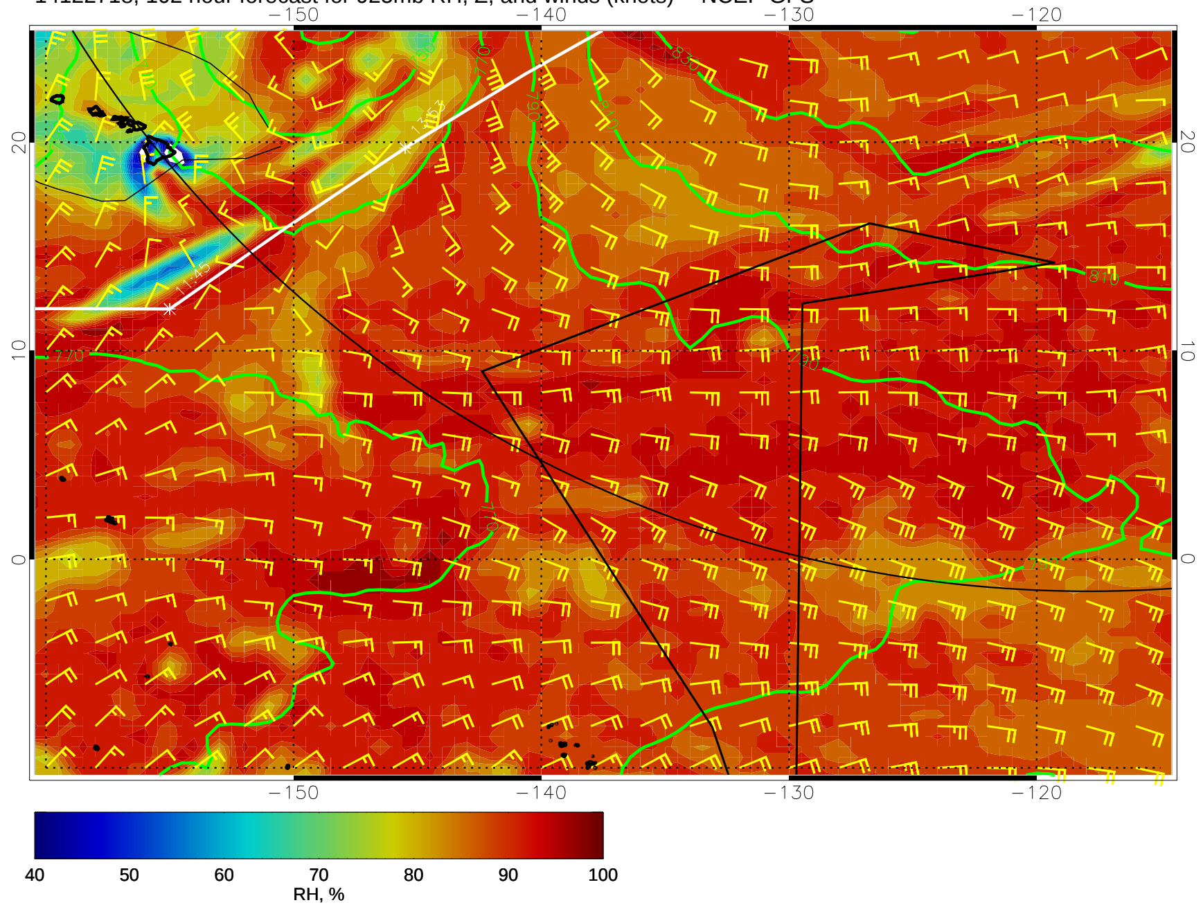
14122718, 102 hour forecast for 925mb RH, Z, and winds (knots) -- NCEP GFS
