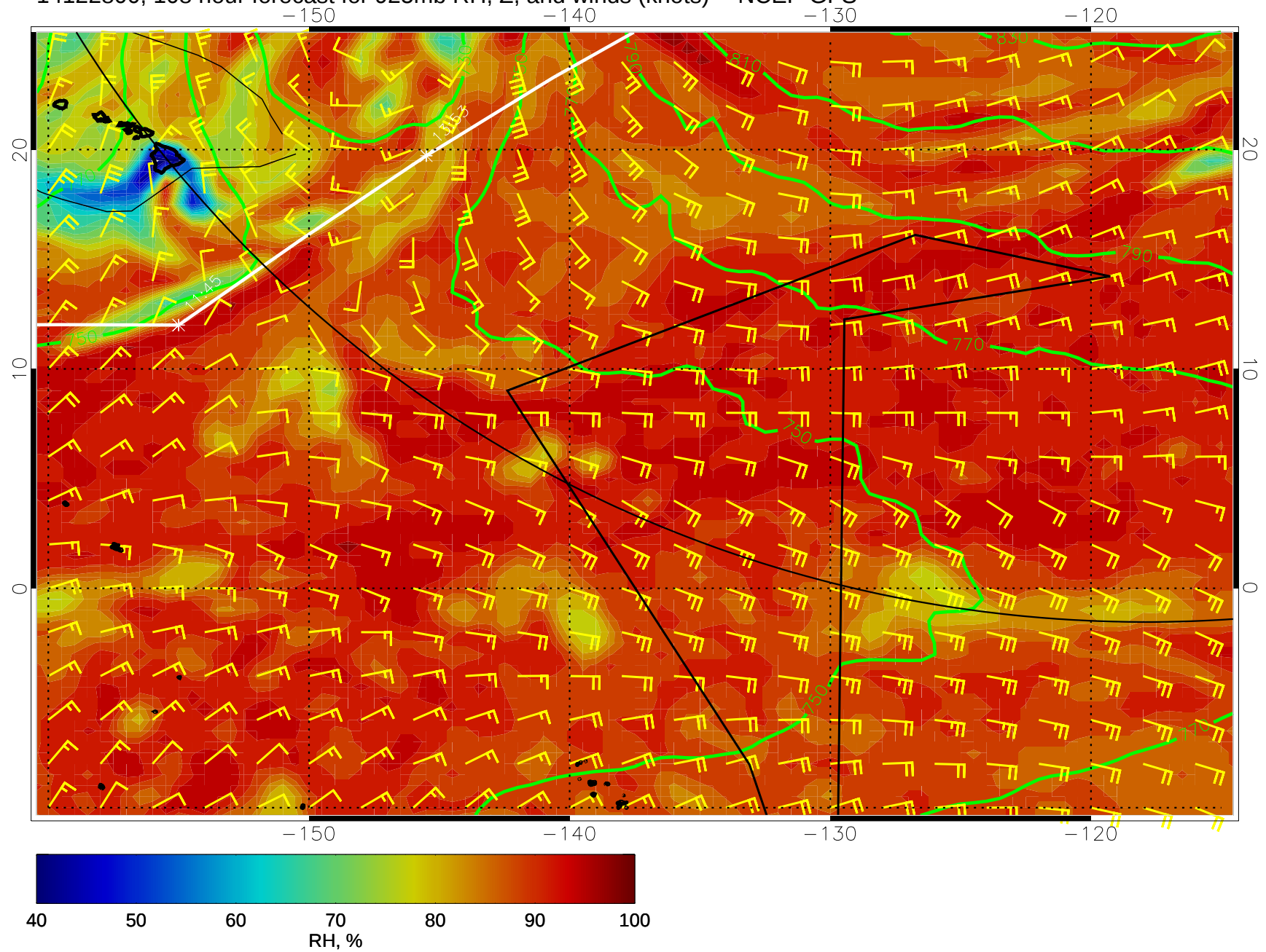
14122800, 108 hour forecast for 925mb RH, Z, and winds (knots) -- NCEP GFS
