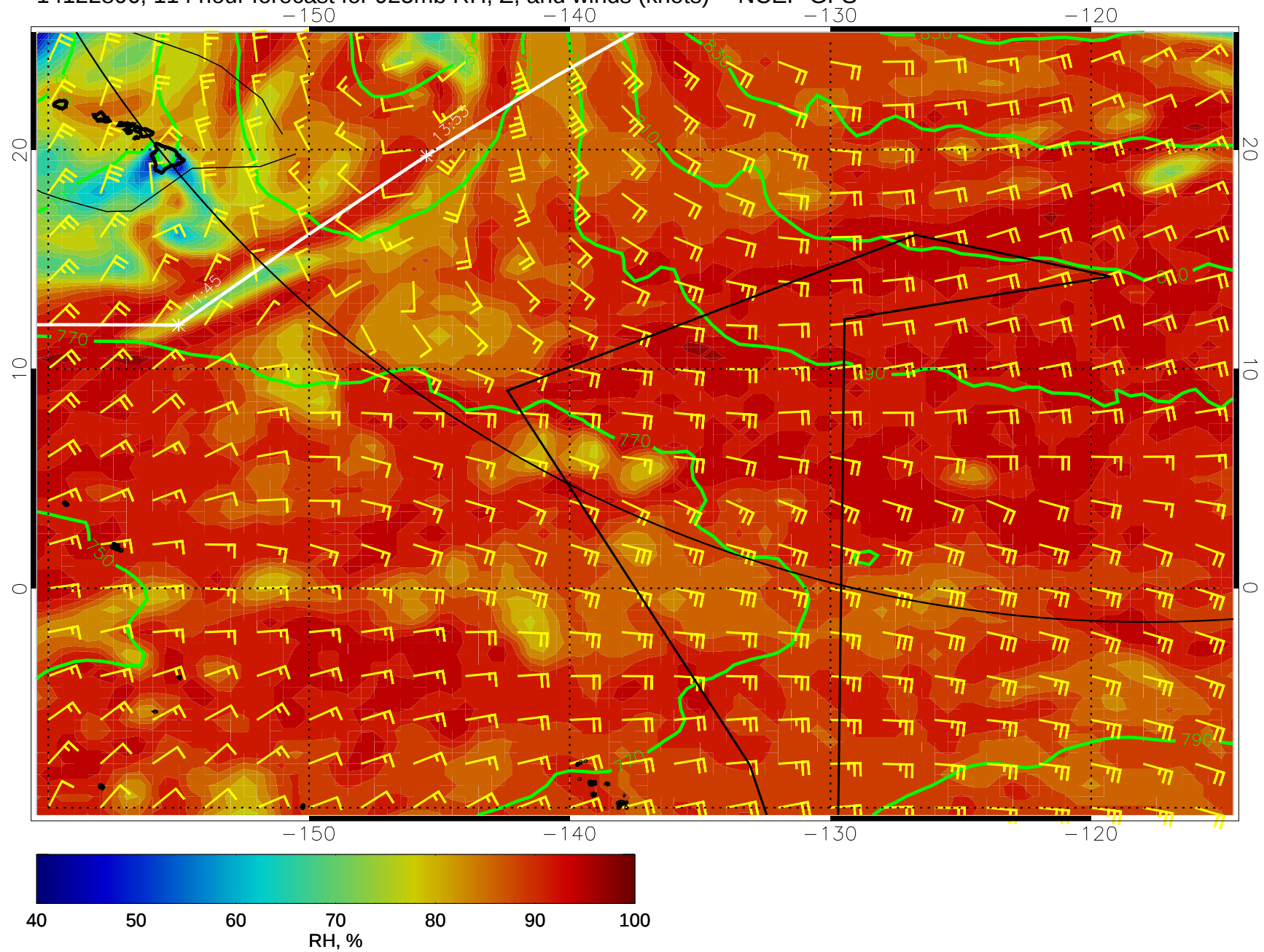
14122806, 114 hour forecast for 925mb RH, Z, and winds (knots) -- NCEP GFS
