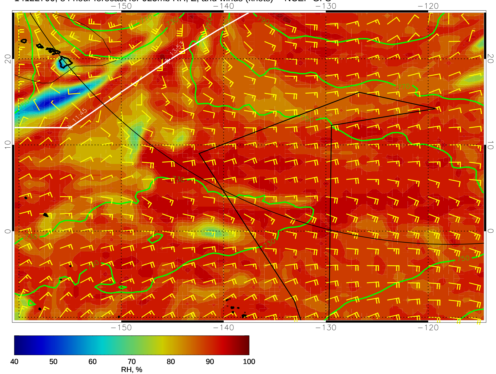
14122700, 84 hour forecast for 925mb RH, Z, and winds (knots) -- NCEP GFS
