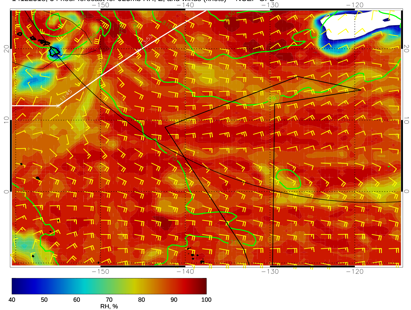
14122518, 54 hour forecast for 925mb RH, Z, and winds (knots) -- NCEP GFS
