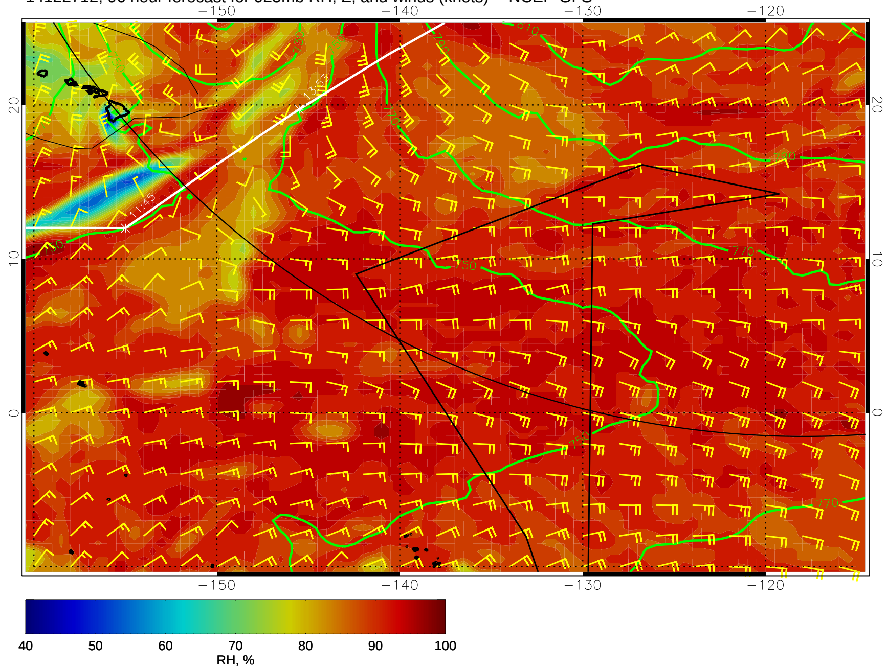
14122712, 96 hour forecast for 925mb RH, Z, and winds (knots) -- NCEP GFS
