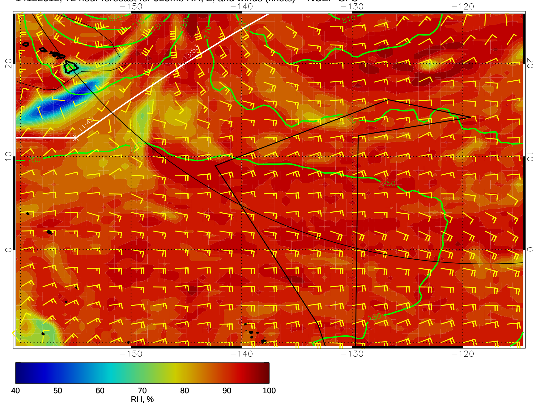
14122612, 72 hour forecast for 925mb RH, Z, and winds (knots) -- NCEP GFS
