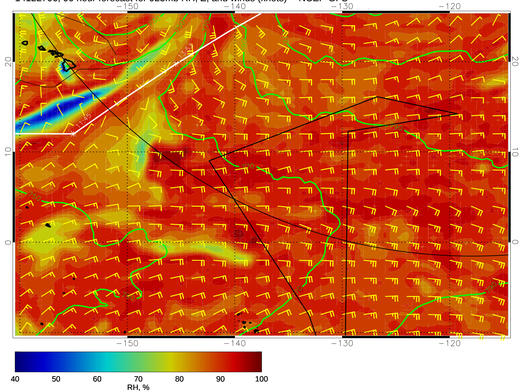
14122706, 90 hour forecast for 925mb RH, Z, and winds (knots) -- NCEP GFS
