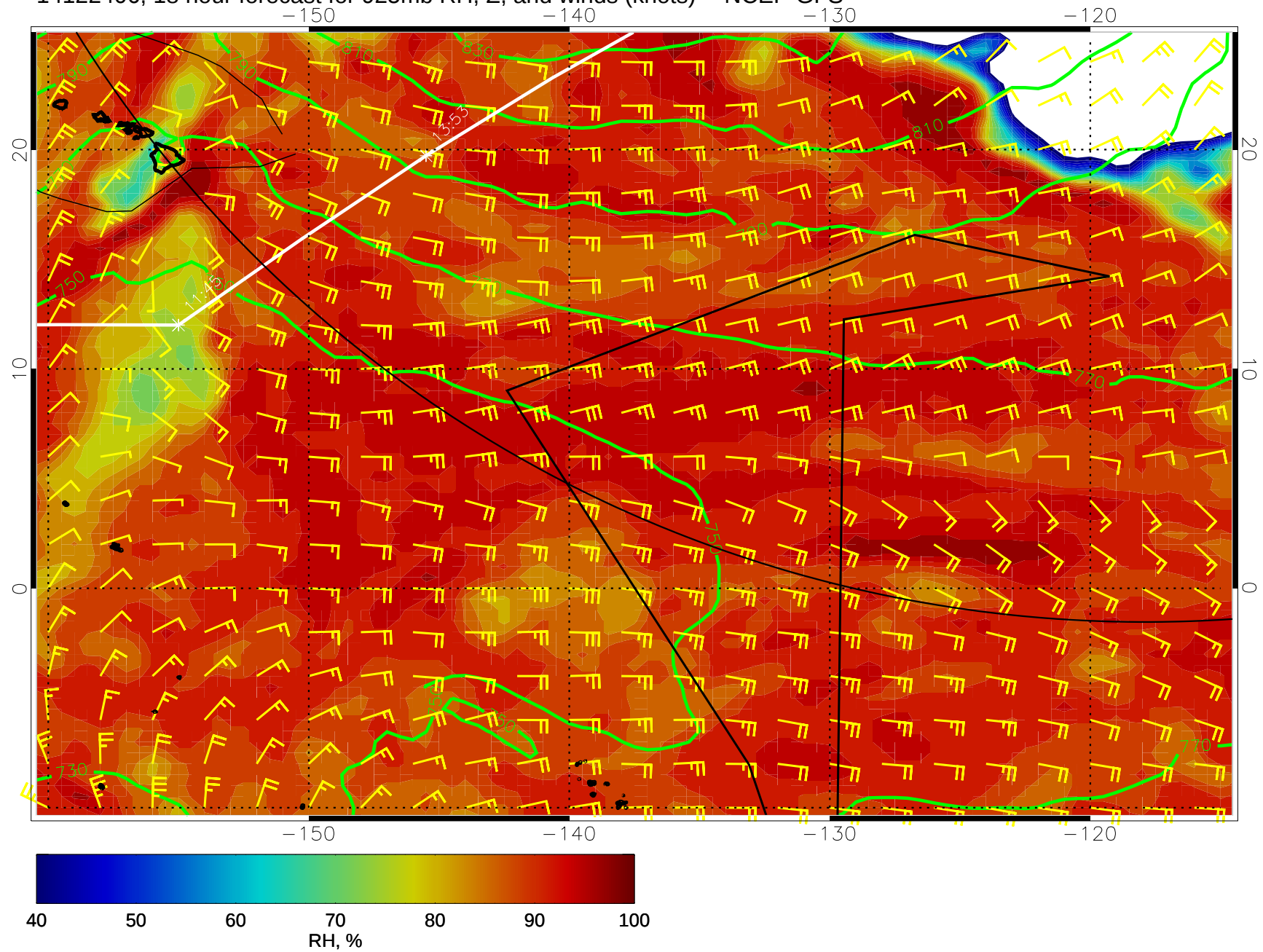
14122406, 18 hour forecast for 925mb RH, Z, and winds (knots) -- NCEP GFS
