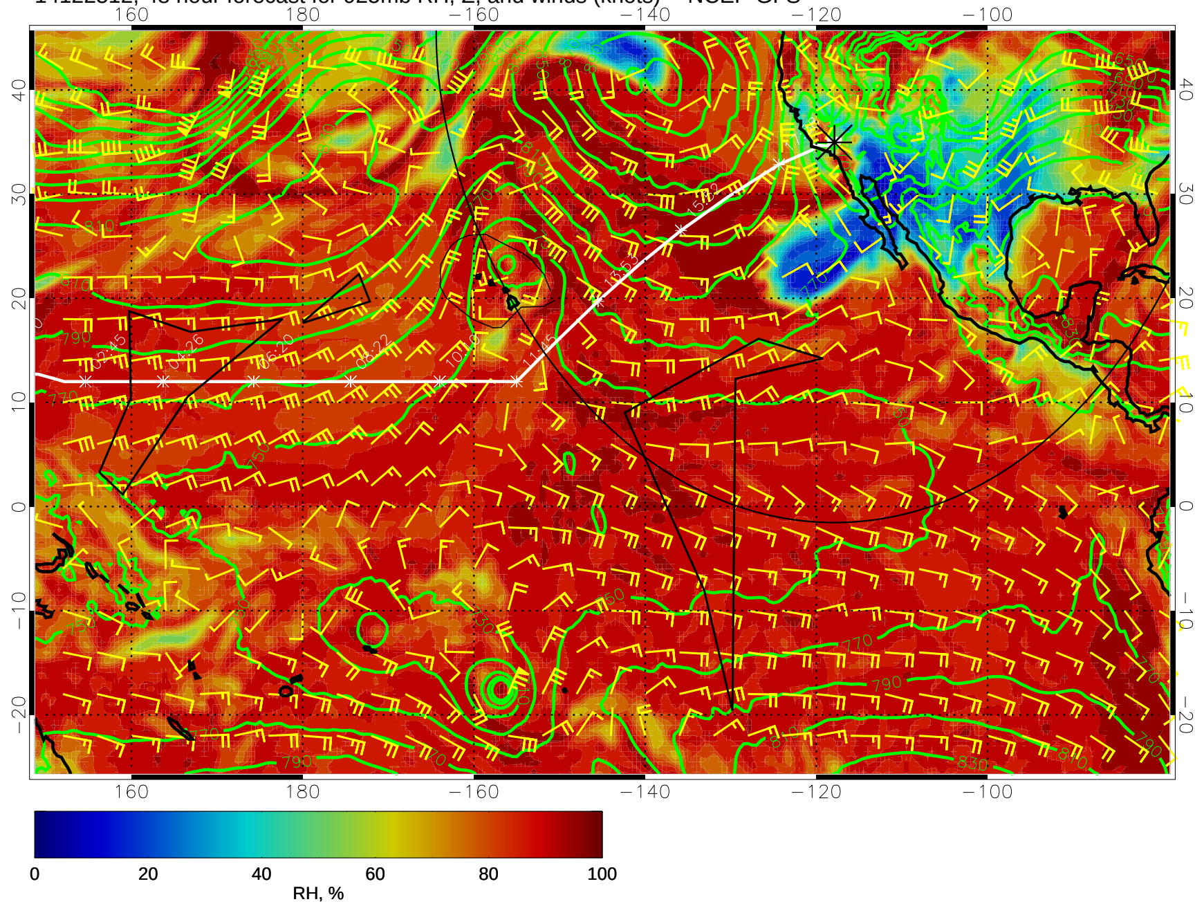
14122512, 48 hour forecast for 925mb RH, Z, and winds (knots) -- NCEP GFS
