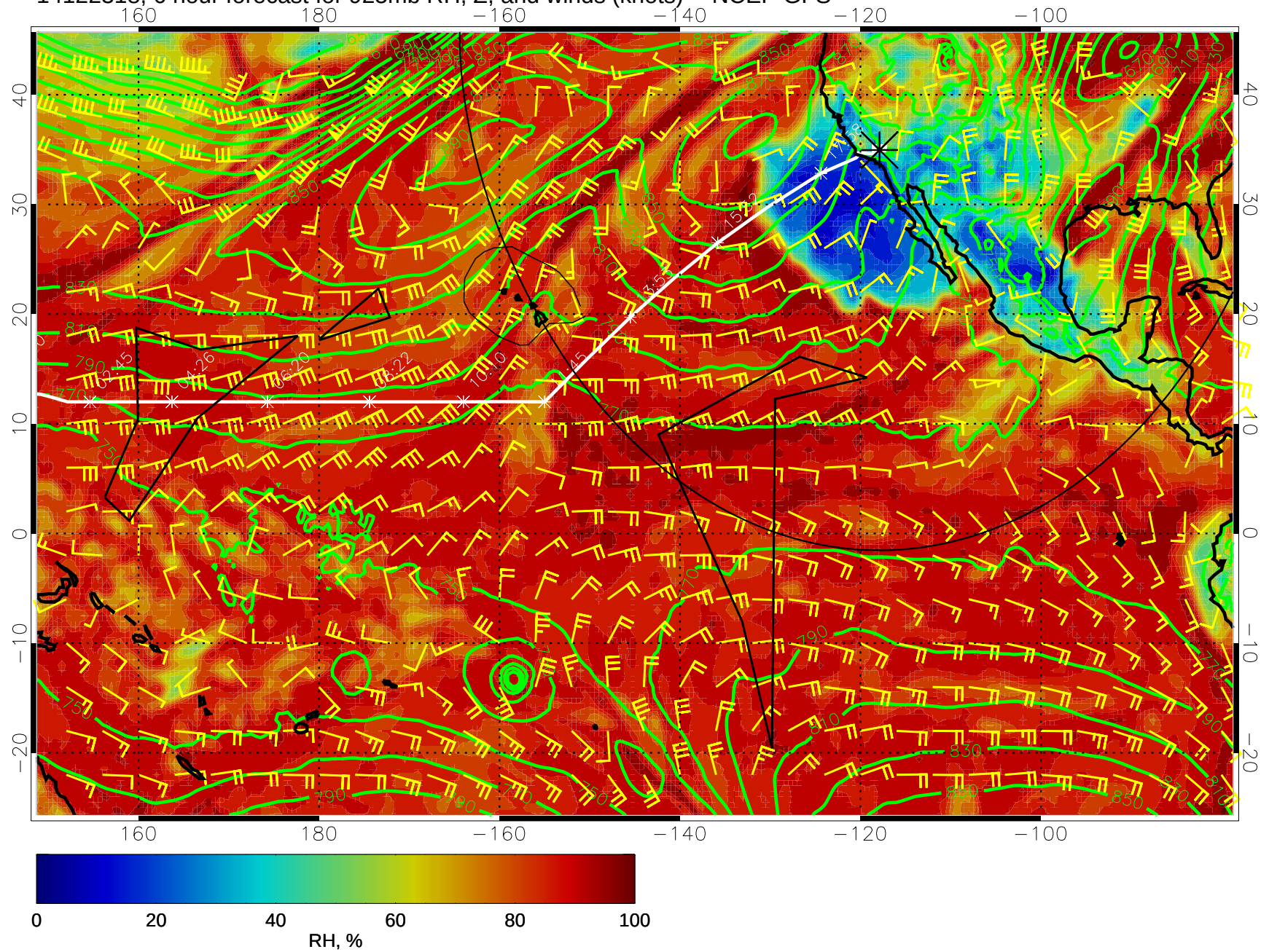
14122318, 6 hour forecast for 925mb RH, Z, and winds (knots) -- NCEP GFS
