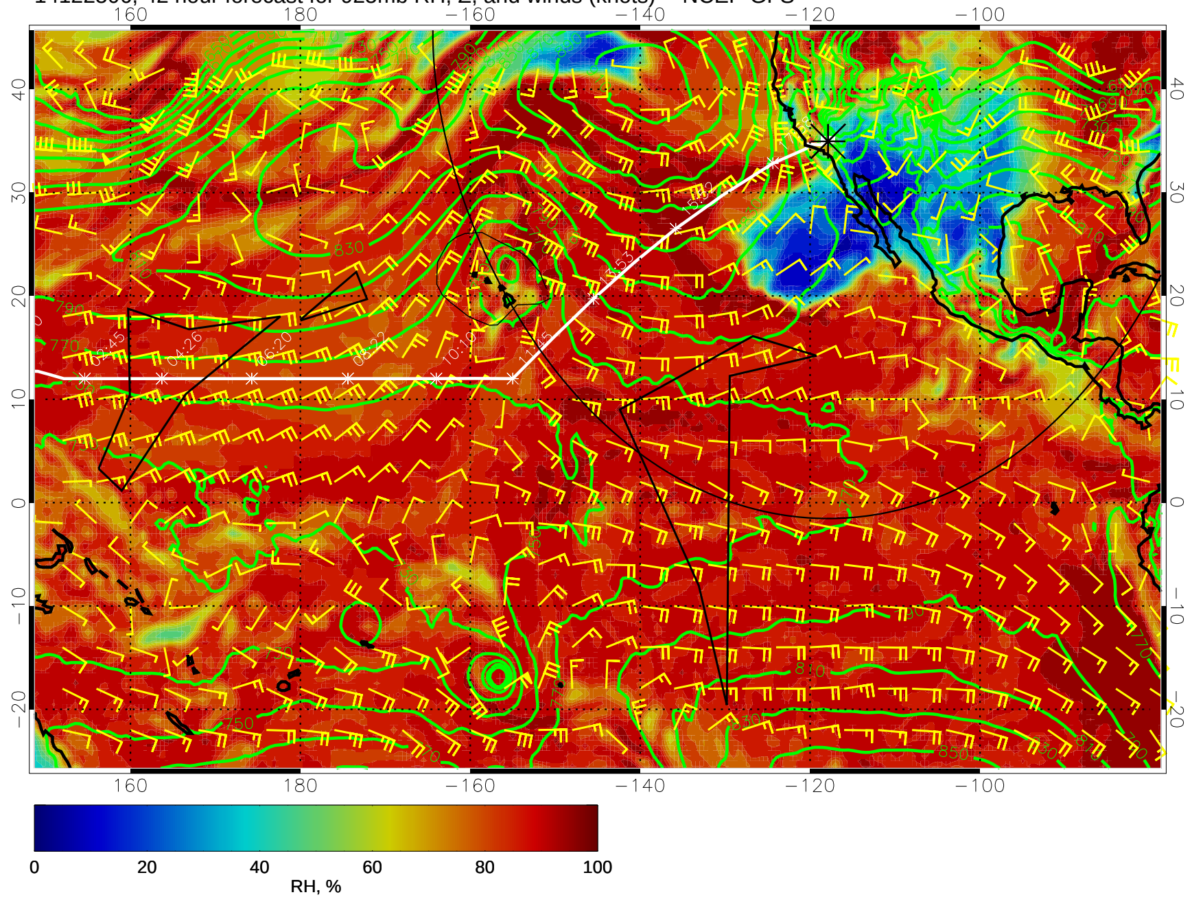
14122506, 42 hour forecast for 925mb RH, Z, and winds (knots) -- NCEP GFS
