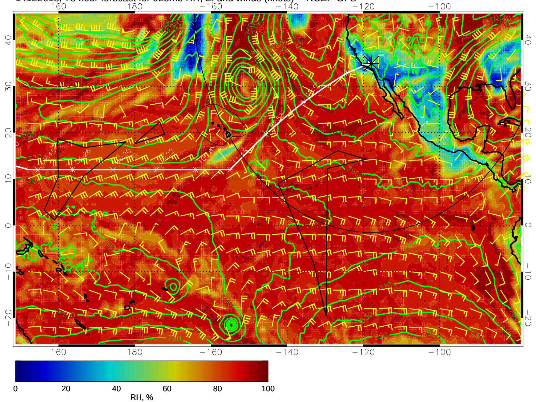
14122618, 78 hour forecast for 925mb RH, Z, and winds (knots) -- NCEP GFS
