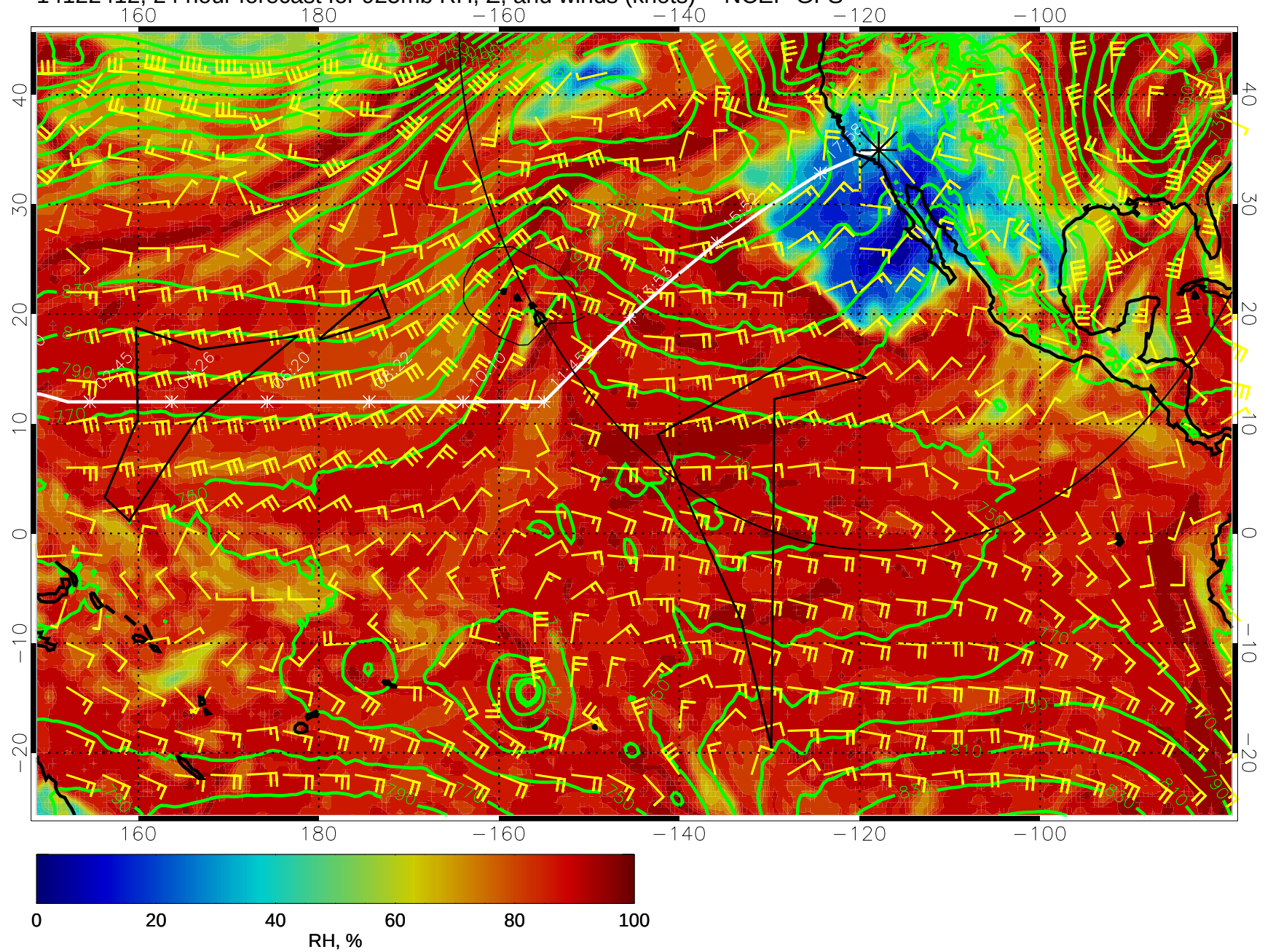
14122412, 24 hour forecast for 925mb RH, Z, and winds (knots) -- NCEP GFS
