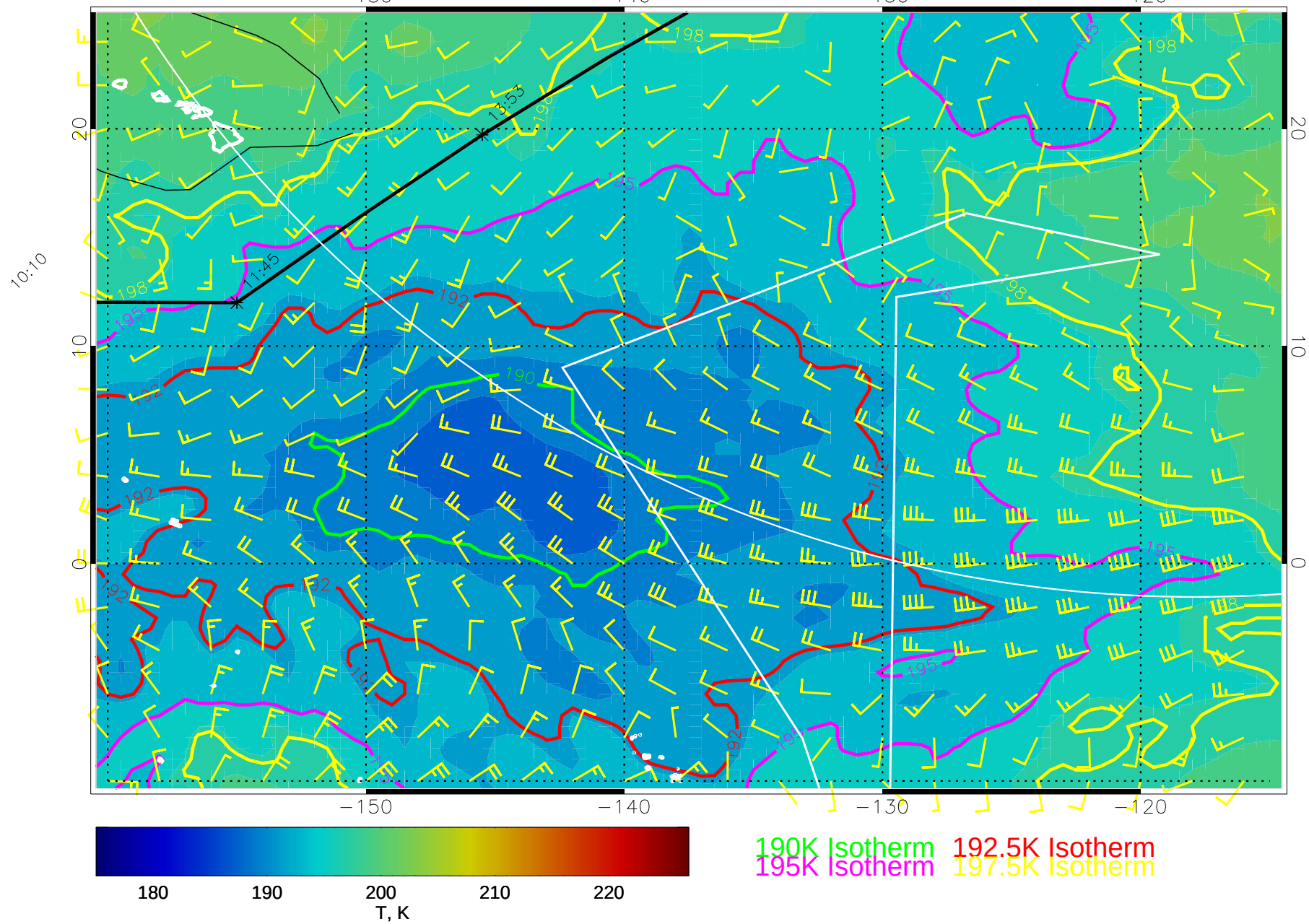
14122412, 24 hour forecast for 70mb T and winds (knots) -- NCEP GFS
