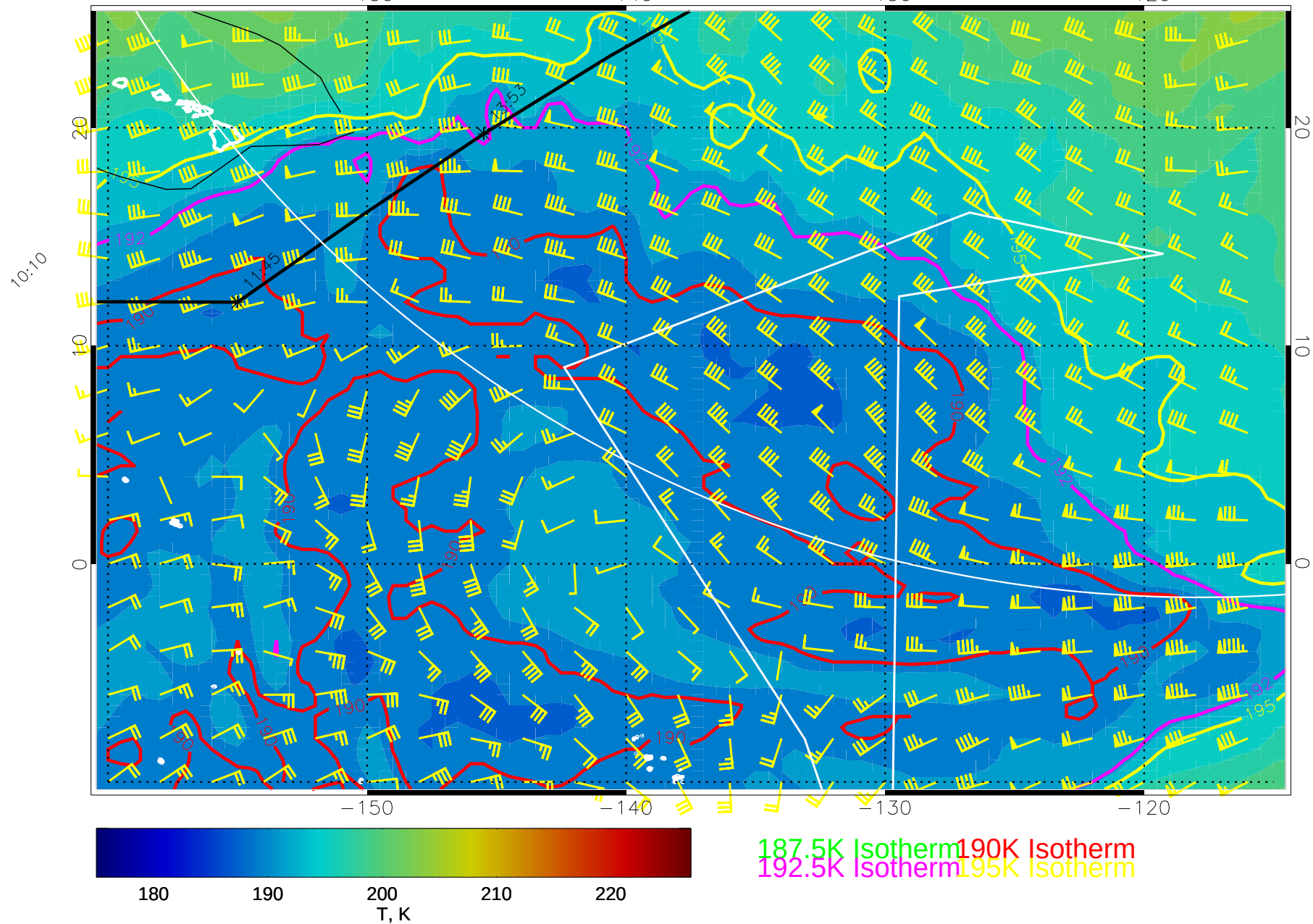
14122518, 54 hour forecast for 100mb T and winds (knots) -- NCEP GFS
