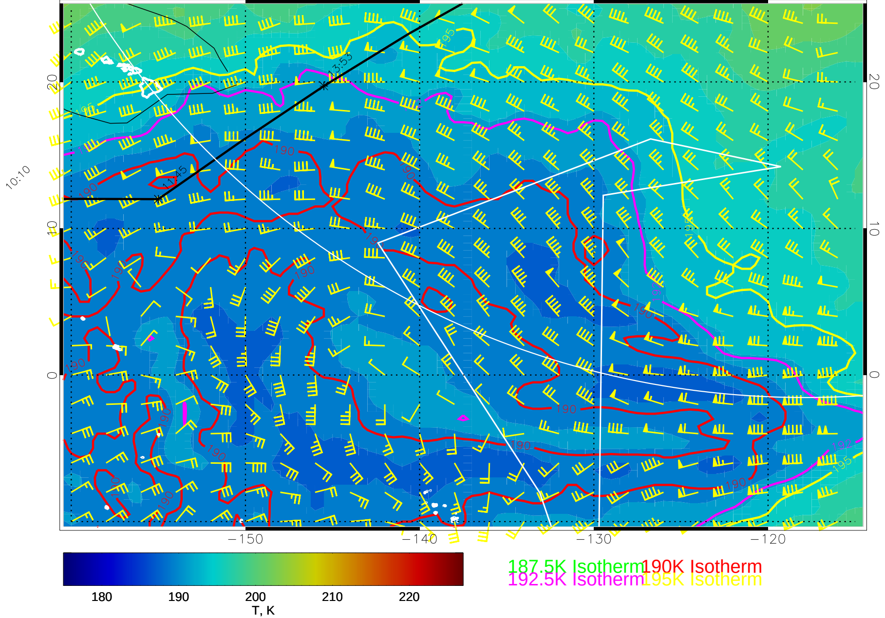
14122512, 48 hour forecast for 100mb T and winds (knots) -- NCEP GFS
