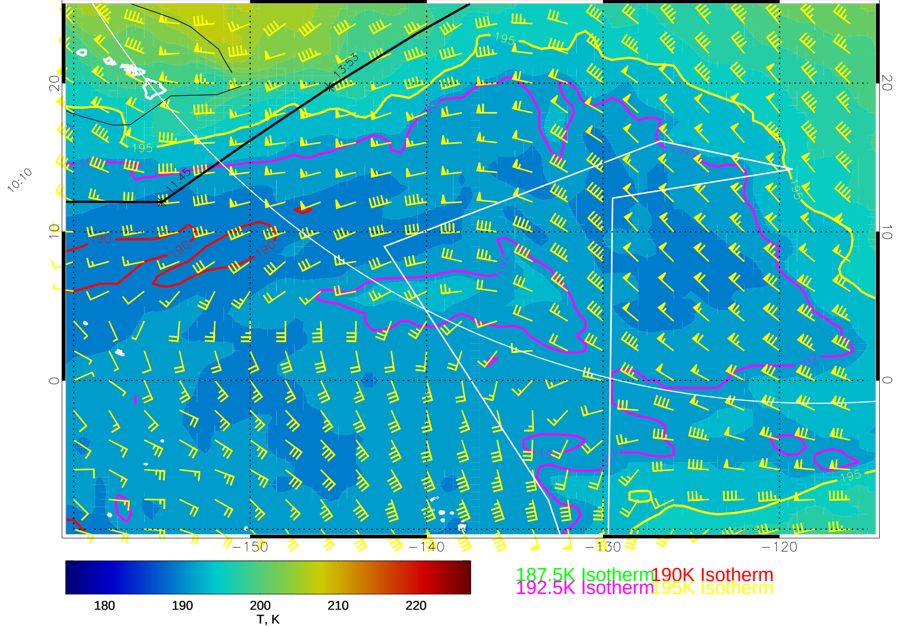
14122706, 90 hour forecast for 100mb T and winds (knots) -- NCEP GFS
