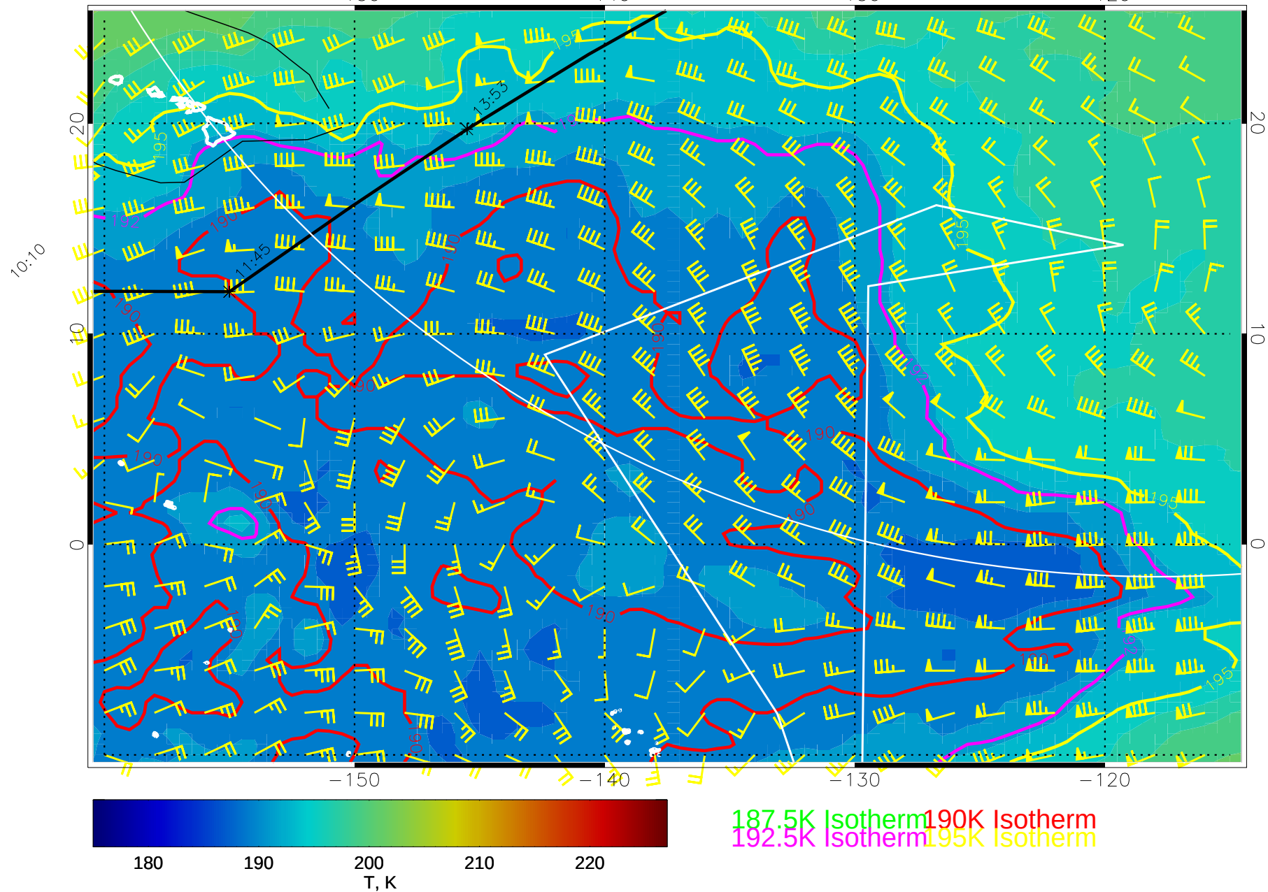
14122506, 42 hour forecast for 100mb T and winds (knots) -- NCEP GFS
