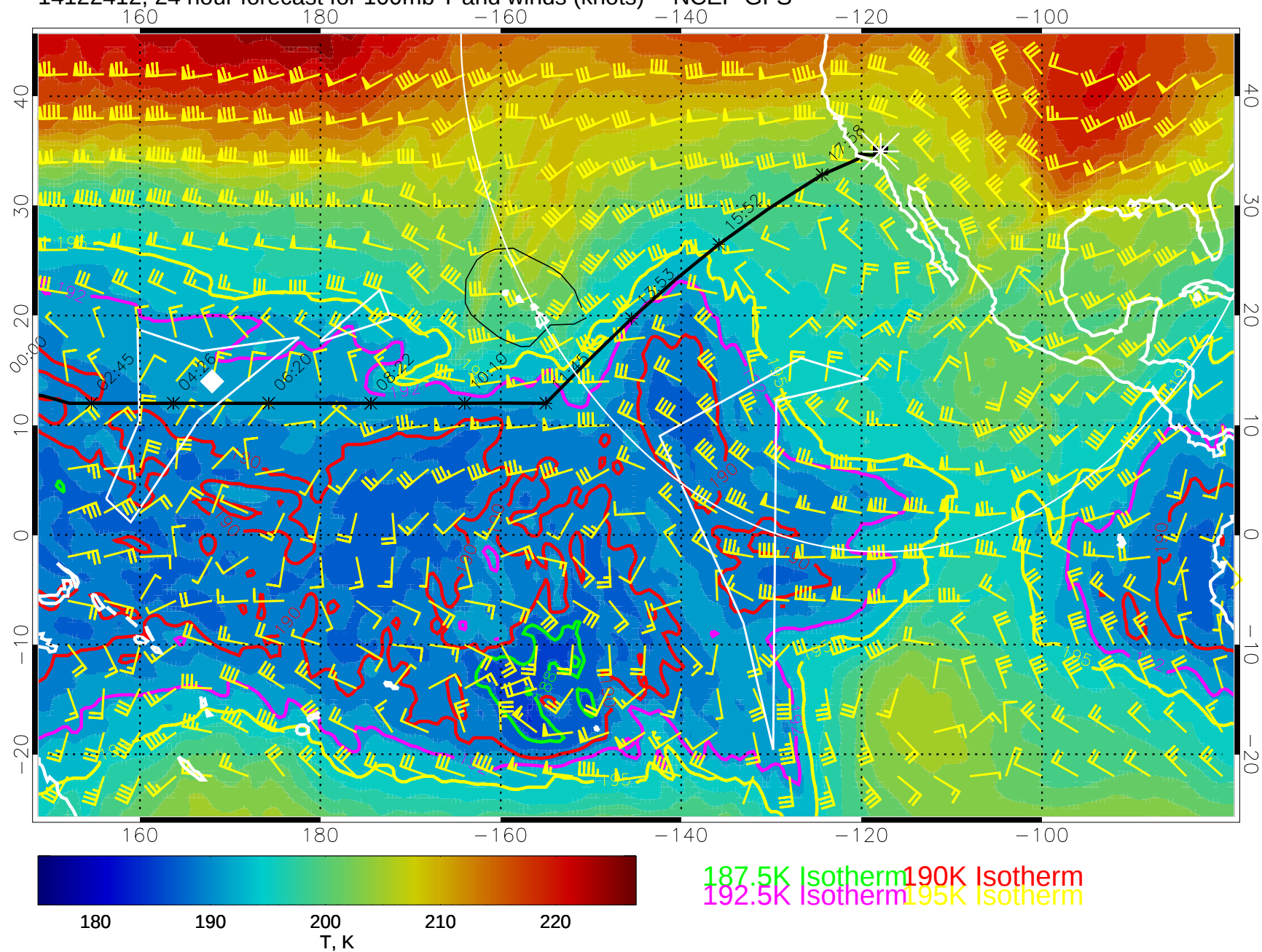
14122412, 24 hour forecast for 100mb T and winds (knots) -- NCEP GFS
