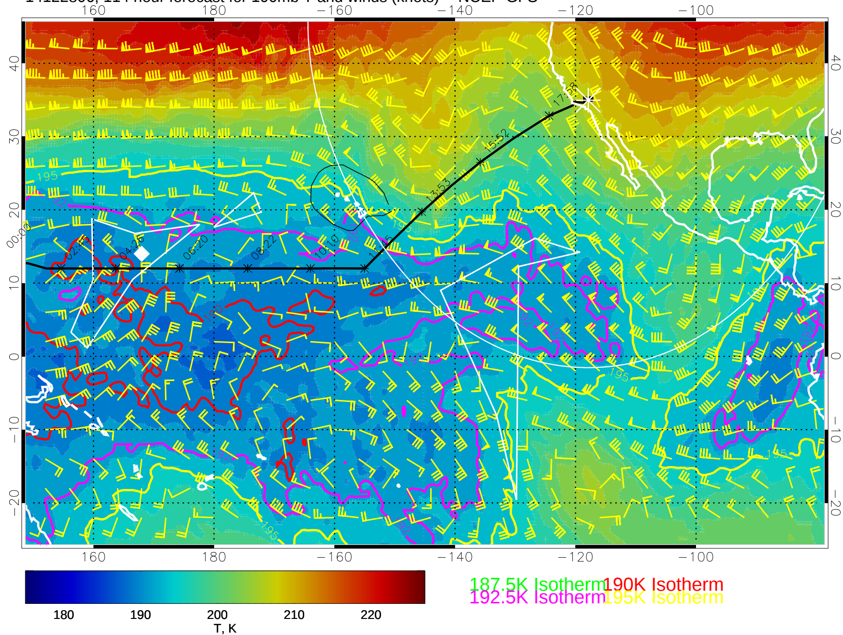
14122806, 114 hour forecast for 100mb T and winds (knots) -- NCEP GFS
