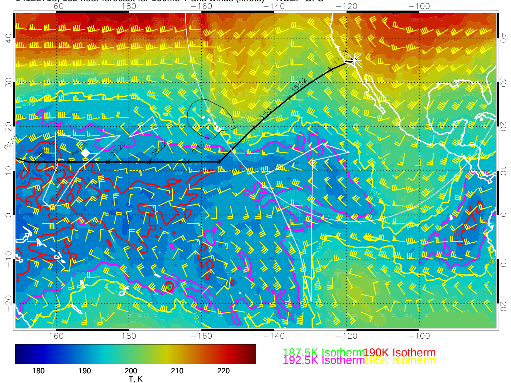
14122718, 102 hour forecast for 100mb T and winds (knots) -- NCEP GFS
