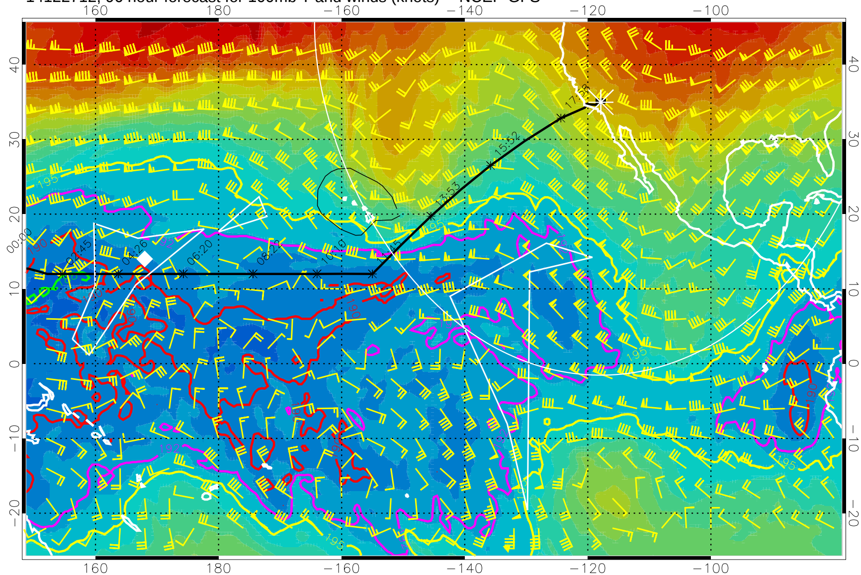
14122712, 96 hour forecast for 100mb T and winds (knots) -- NCEP GFS
