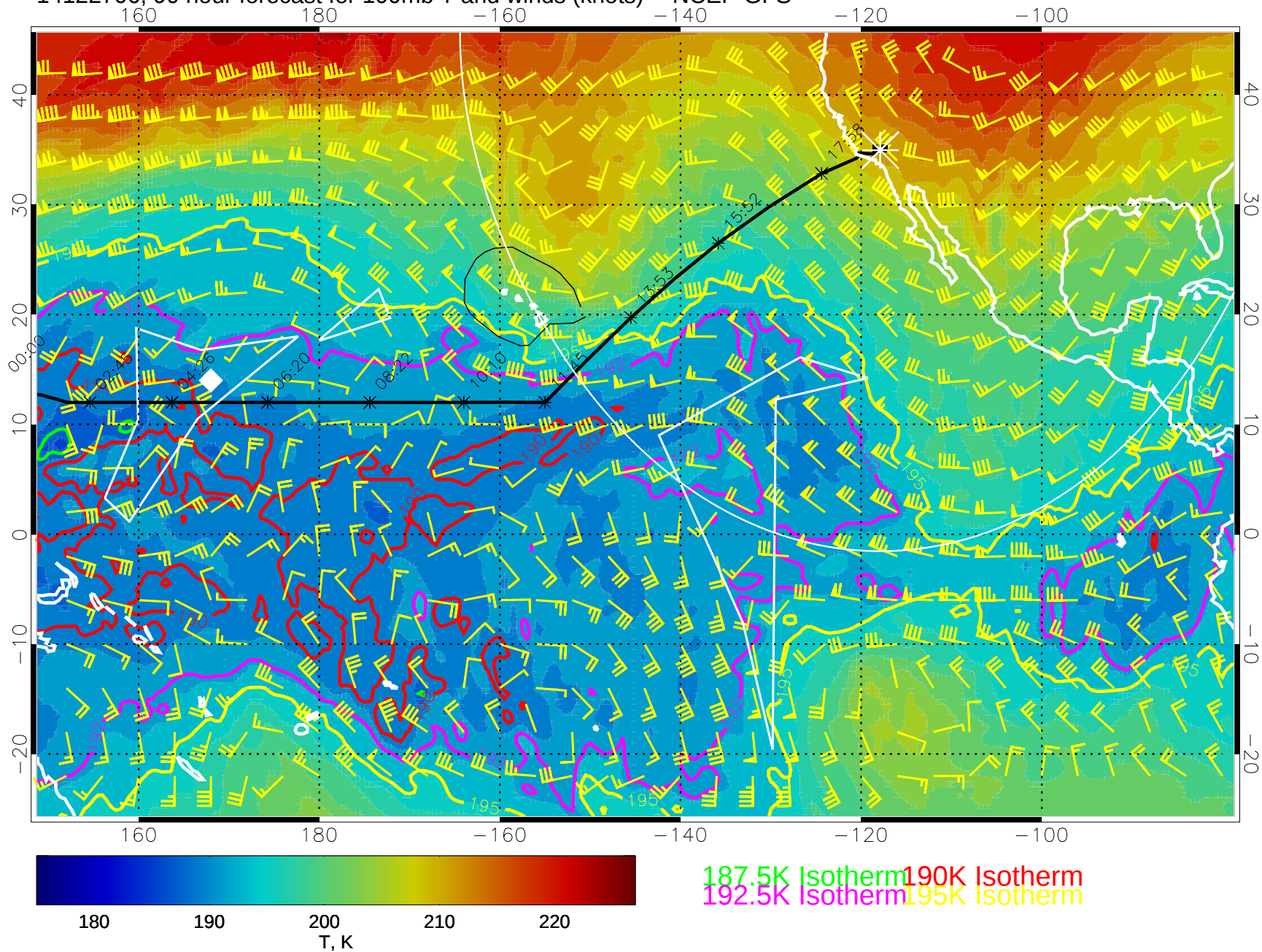
14122706, 90 hour forecast for 100mb T and winds (knots) -- NCEP GFS
