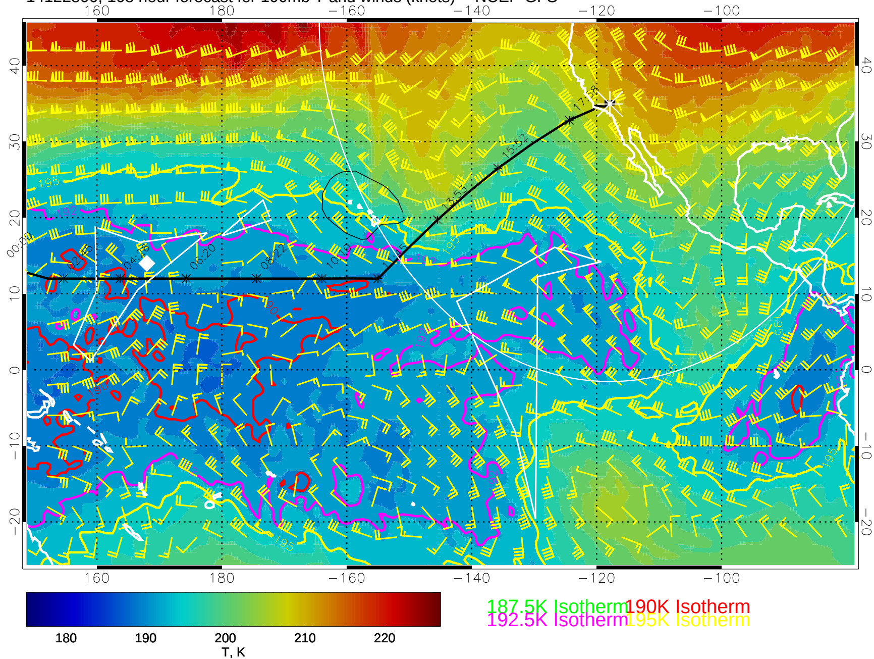
14122800, 108 hour forecast for 100mb T and winds (knots) -- NCEP GFS
