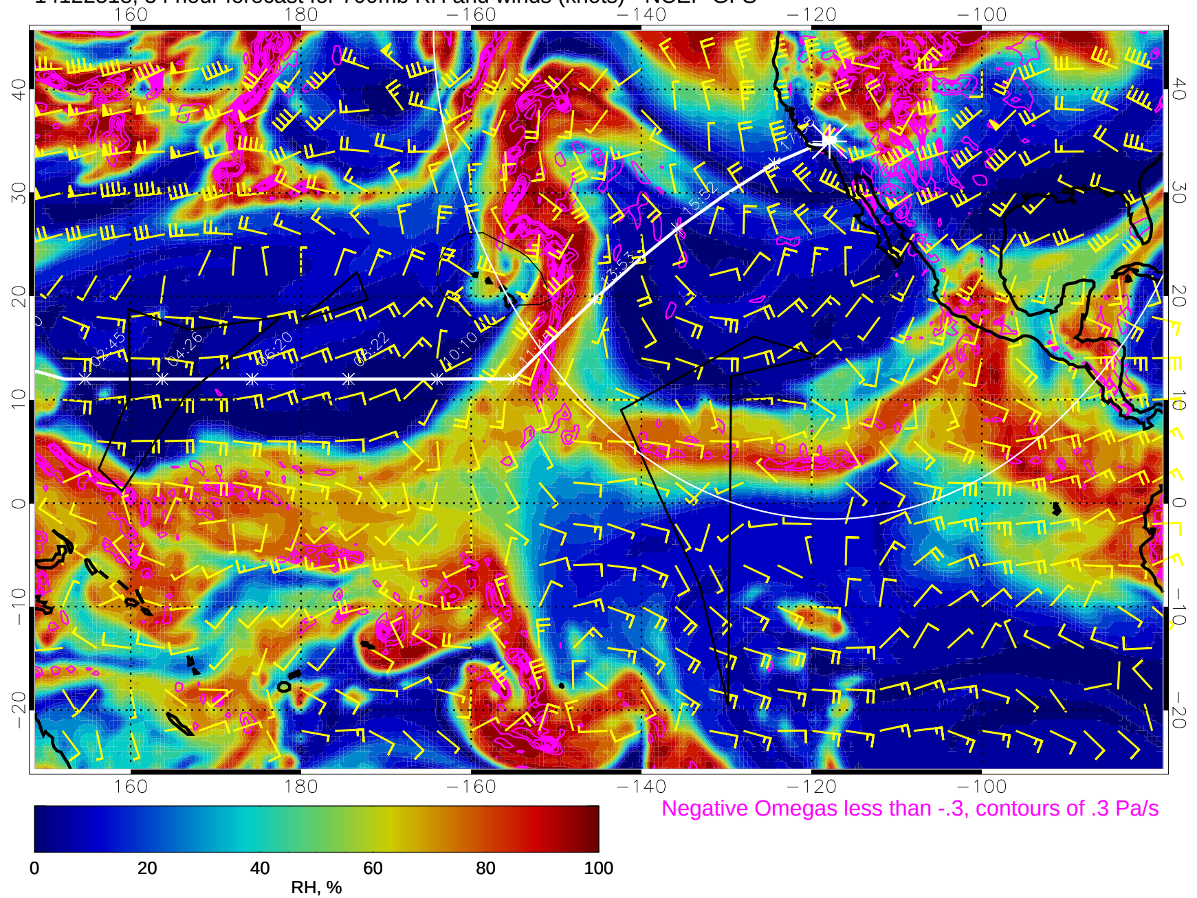
14122518, 54 hour forecast for 700mb RH and winds (knots) - NCEP GFS
