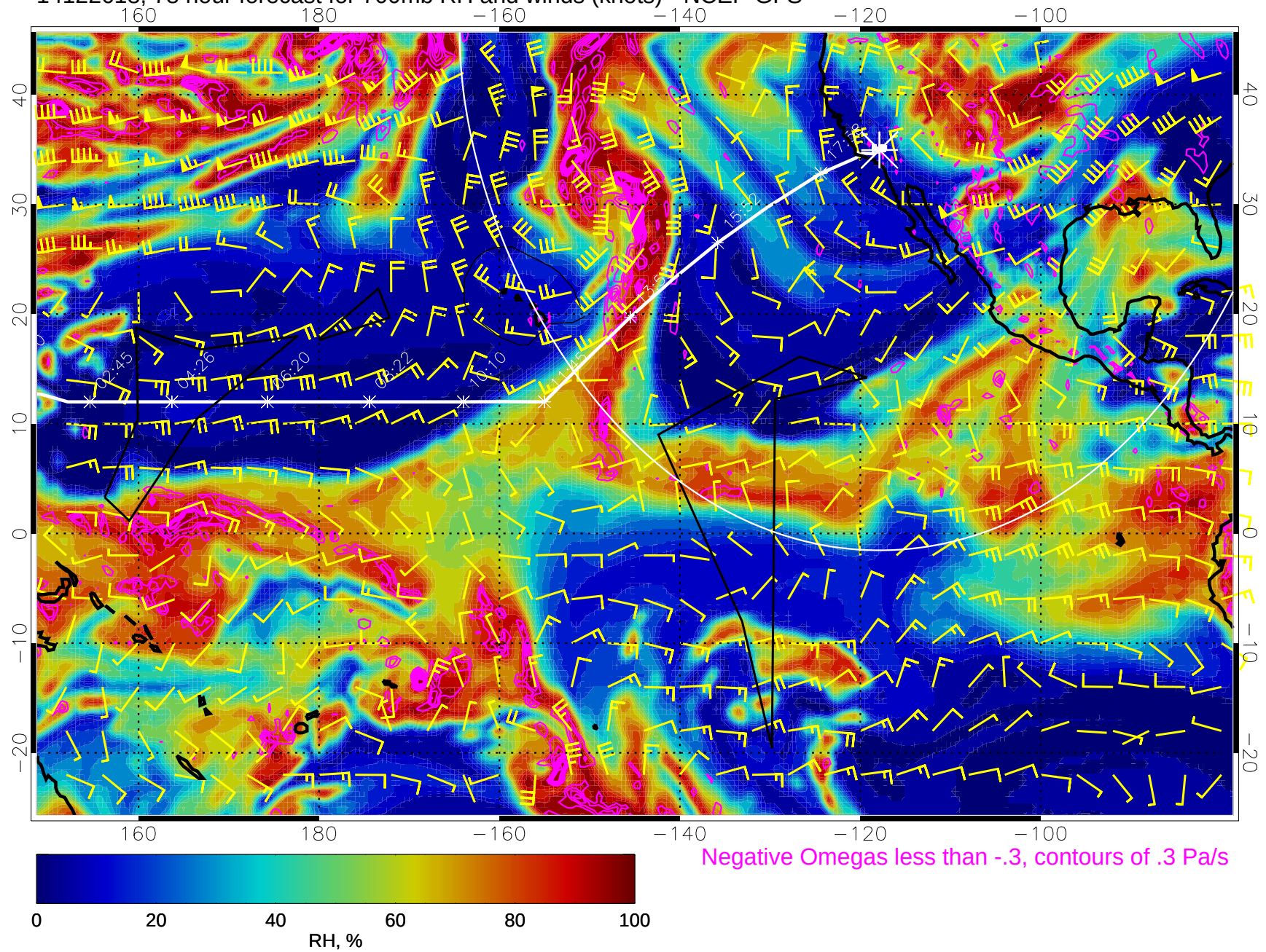
14122618, 78 hour forecast for 700mb RH and winds (knots) - NCEP GFS
