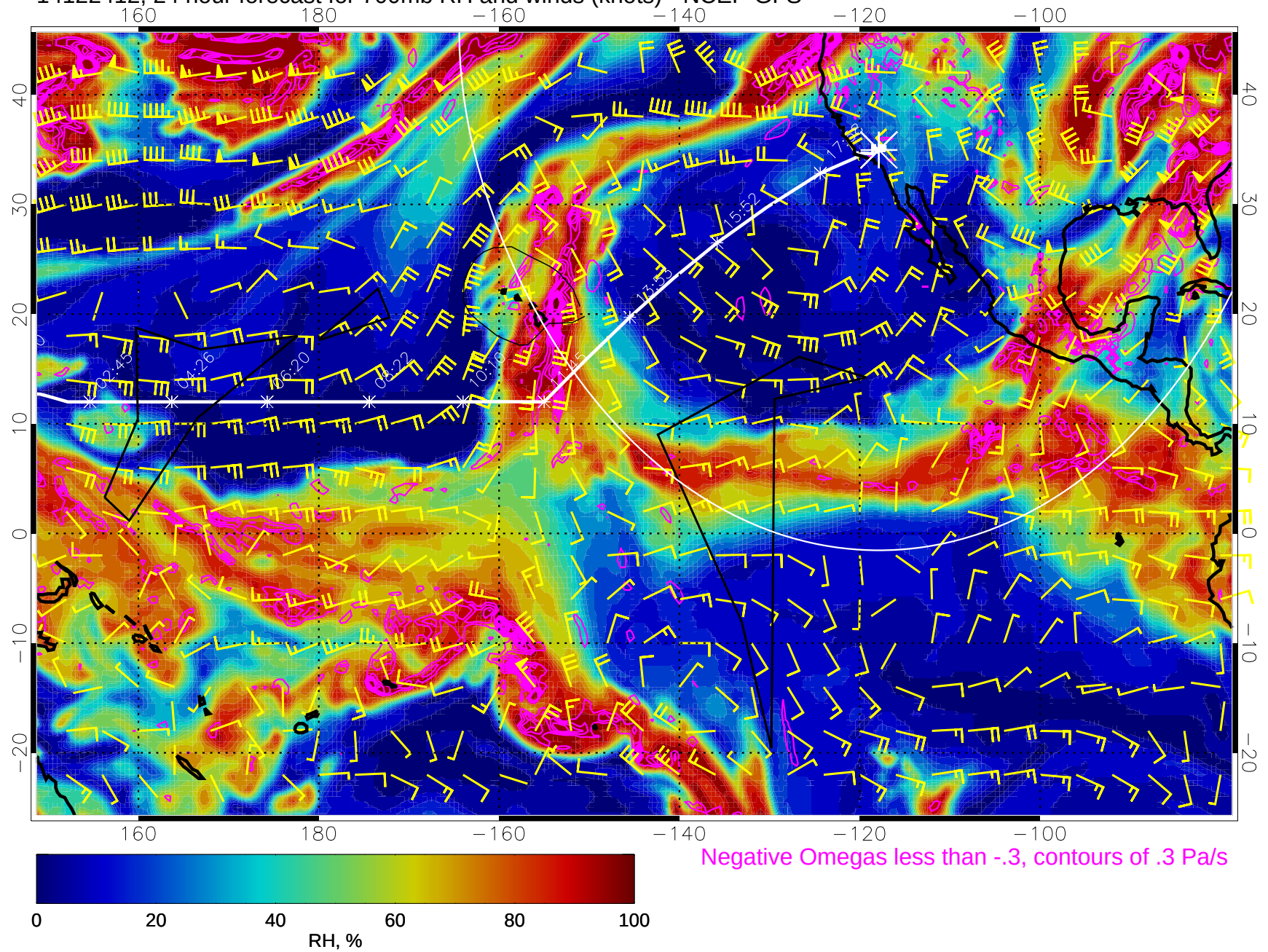
14122412, 24 hour forecast for 700mb RH and winds (knots) - NCEP GFS
