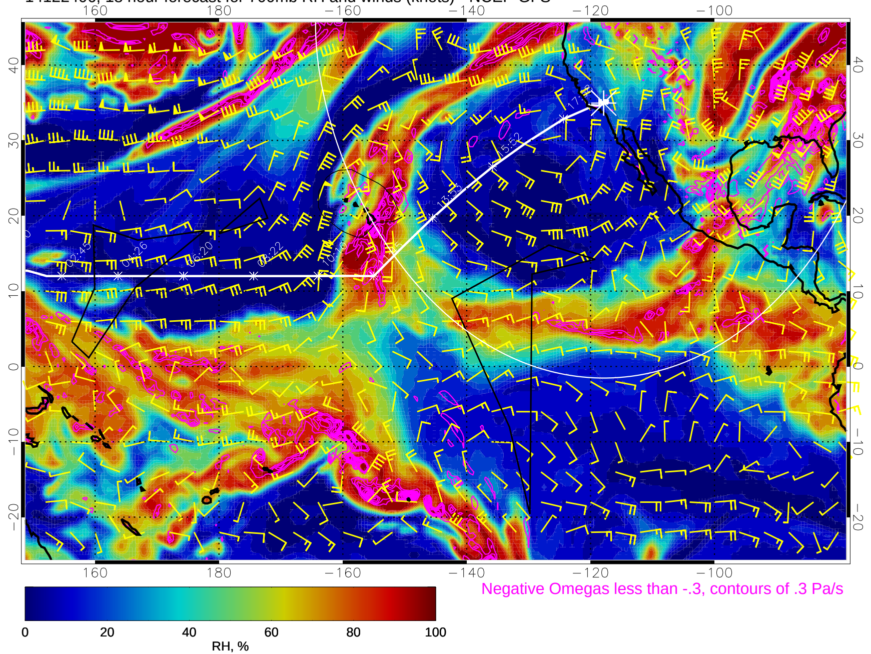
14122406, 18 hour forecast for 700mb RH and winds (knots) - NCEP GFS
