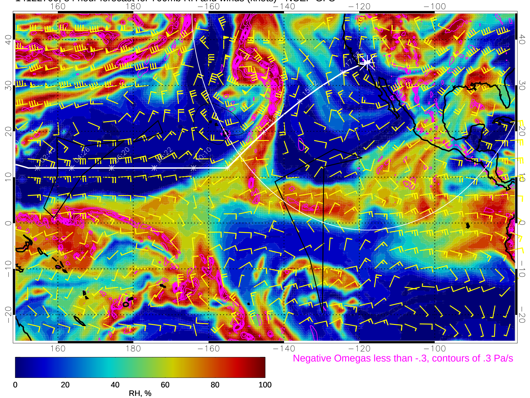
14122700, 84 hour forecast for 700mb RH and winds (knots) - NCEP GFS
