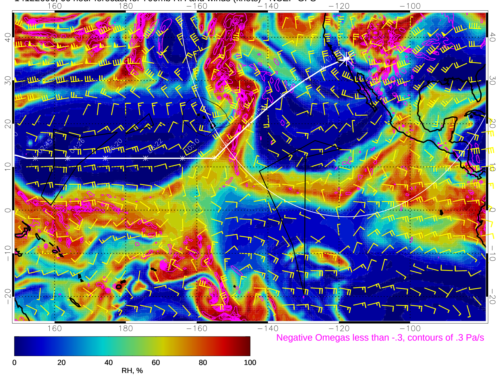
14122606, 66 hour forecast for 700mb RH and winds (knots) - NCEP GFS
