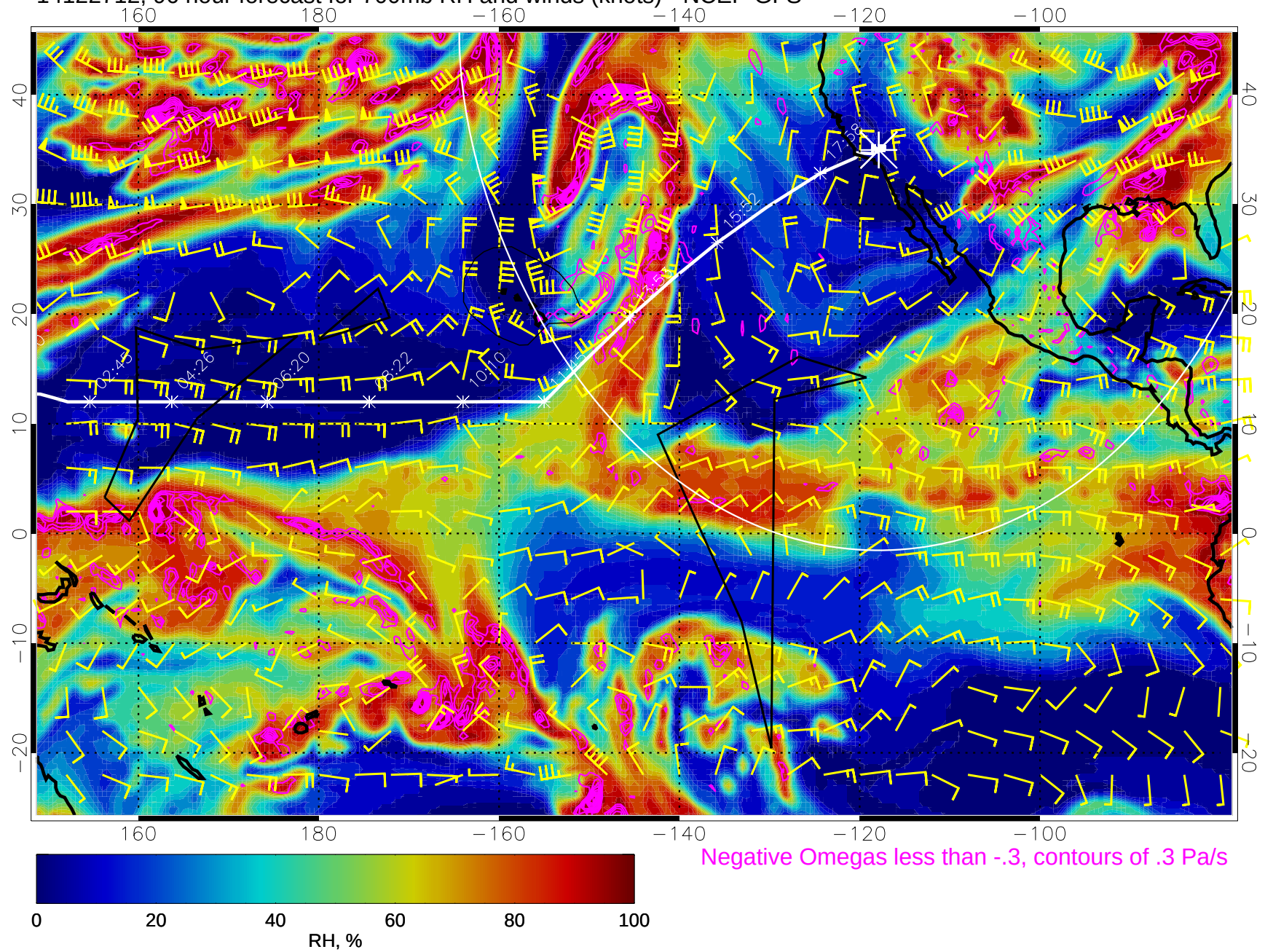
14122712, 96 hour forecast for 700mb RH and winds (knots) - NCEP GFS
