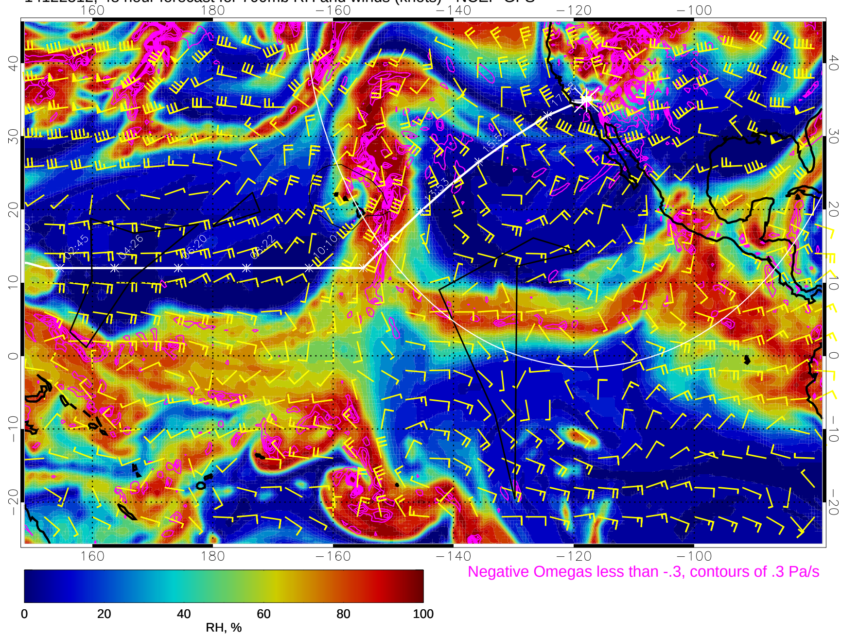
14122512, 48 hour forecast for 700mb RH and winds (knots) - NCEP GFS
