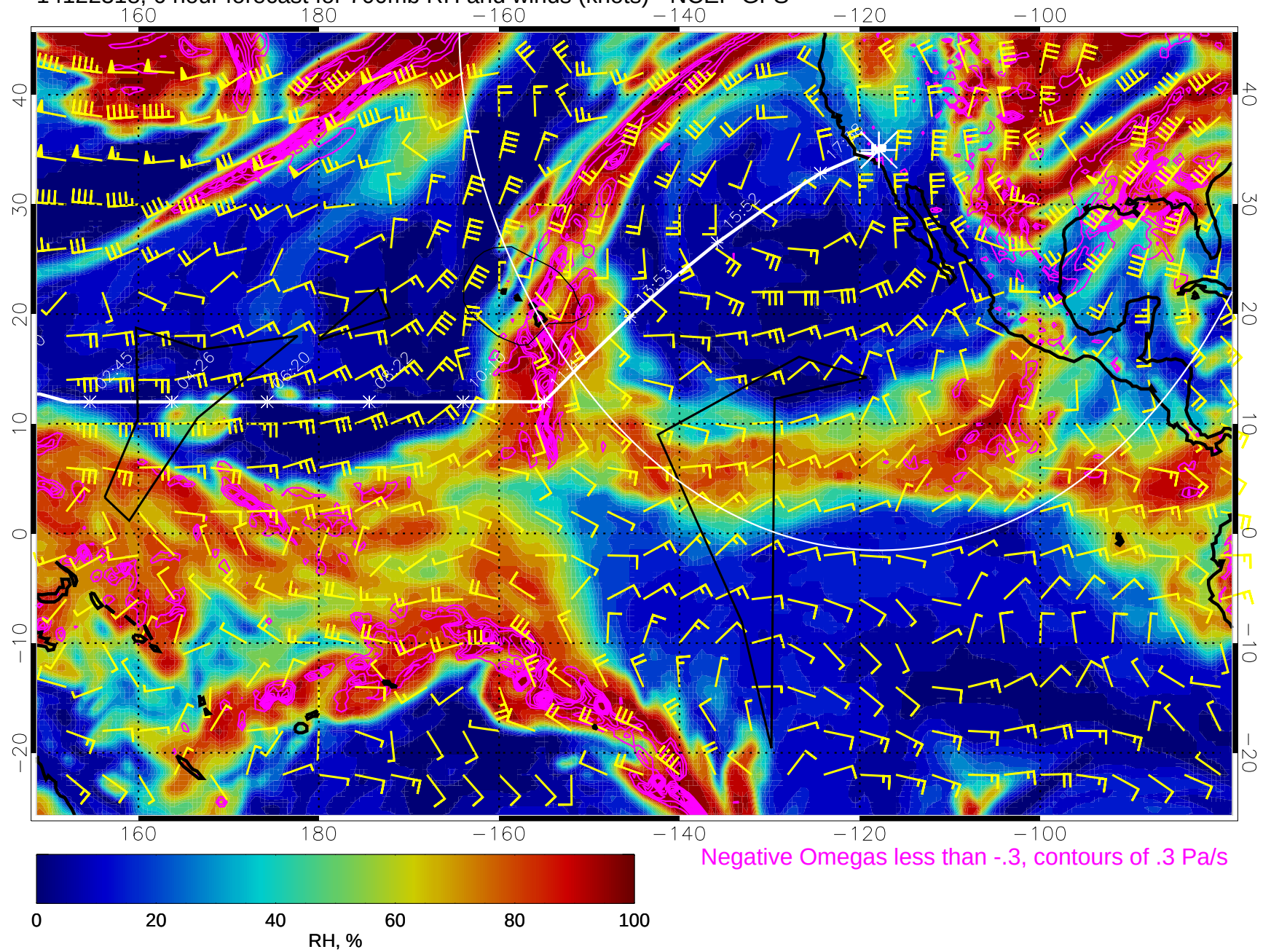
14122318, 6 hour forecast for 700mb RH and winds (knots) - NCEP GFS
