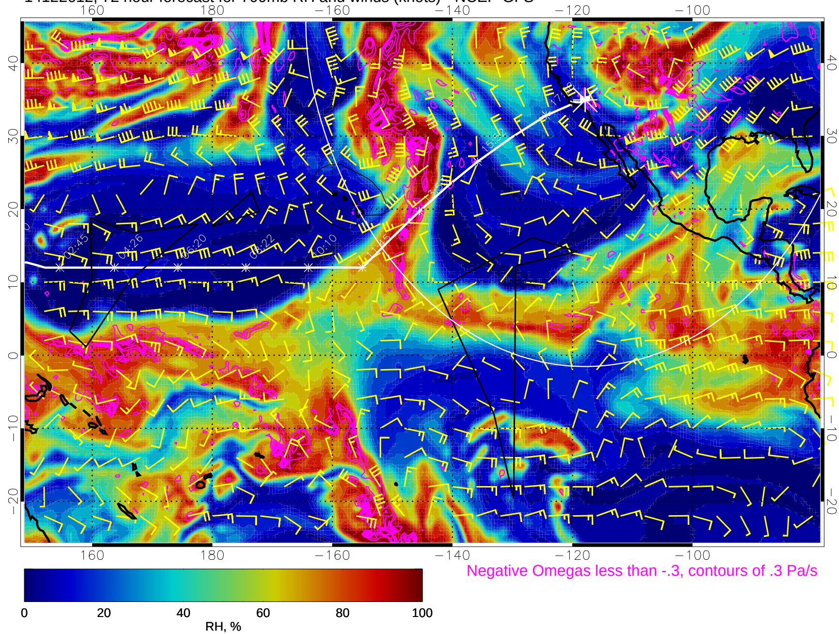
14122612, 72 hour forecast for 700mb RH and winds (knots) - NCEP GFS
