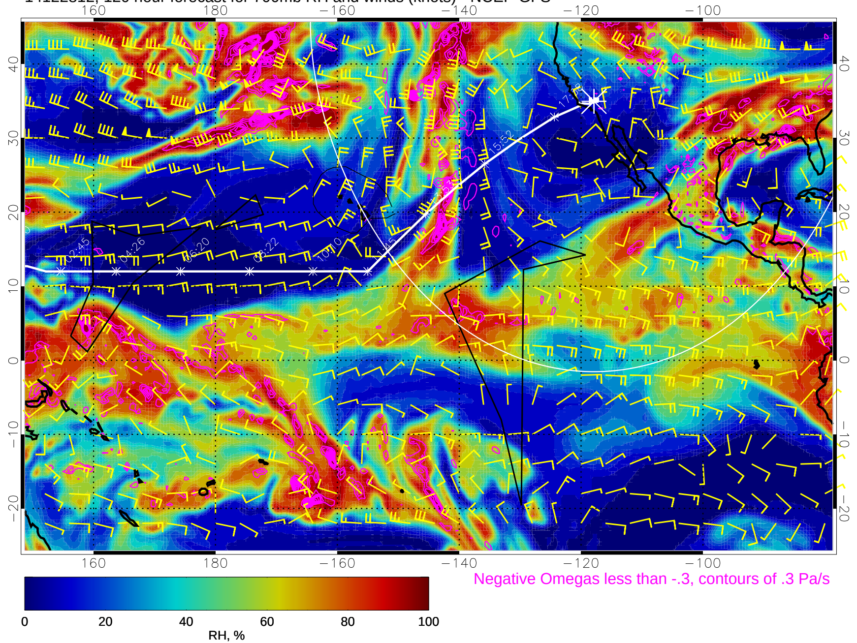
14122812, 120 hour forecast for 700mb RH and winds (knots) - NCEP GFS
