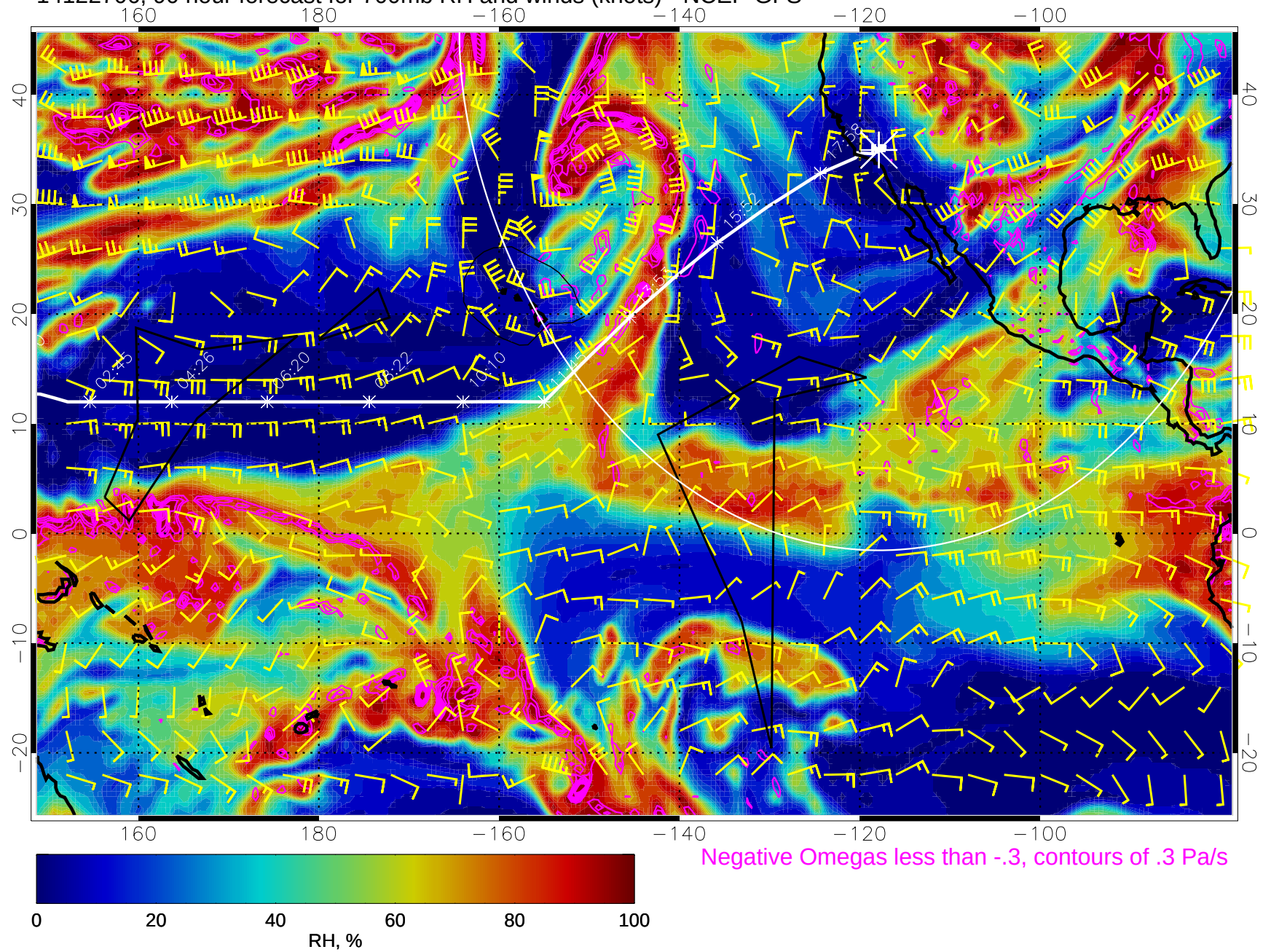
14122706, 90 hour forecast for 700mb RH and winds (knots) - NCEP GFS
