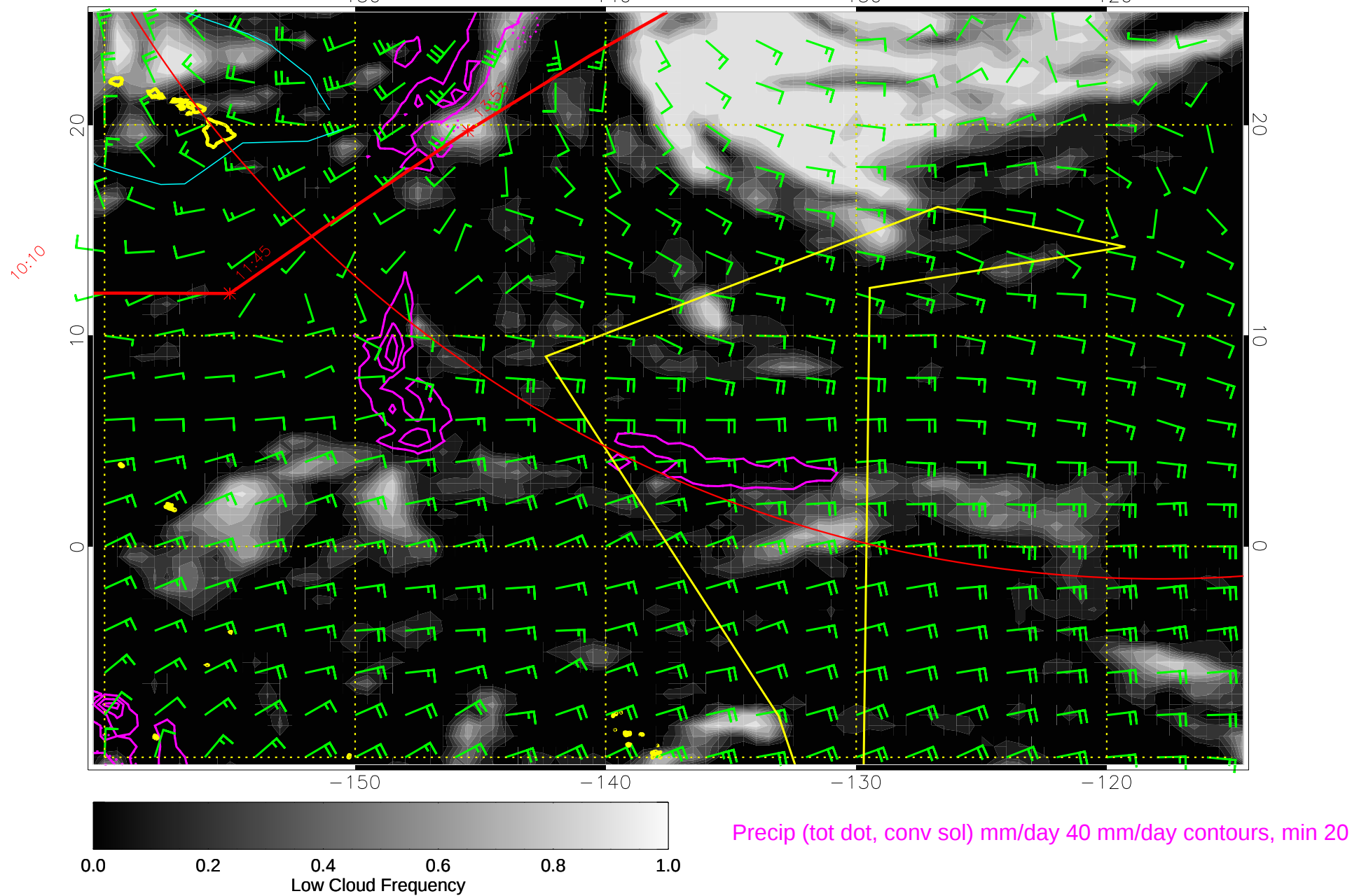
14122700, 84 hour forecast for 850mb winds (knots) and Low Cloud Frequency -- NCEP GFS
