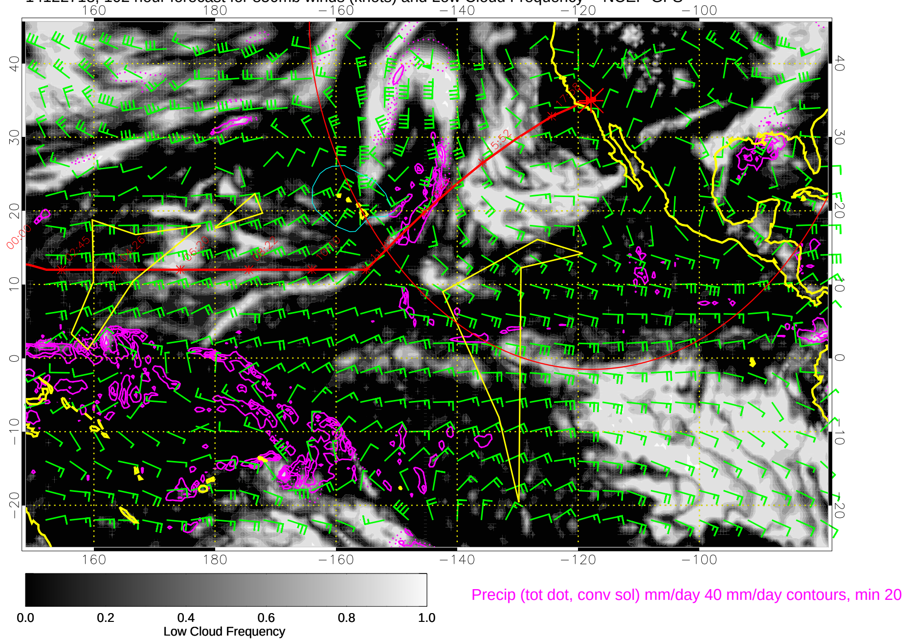
14122718, 102 hour forecast for 850mb winds (knots) and Low Cloud Frequency -- NCEP GFS
