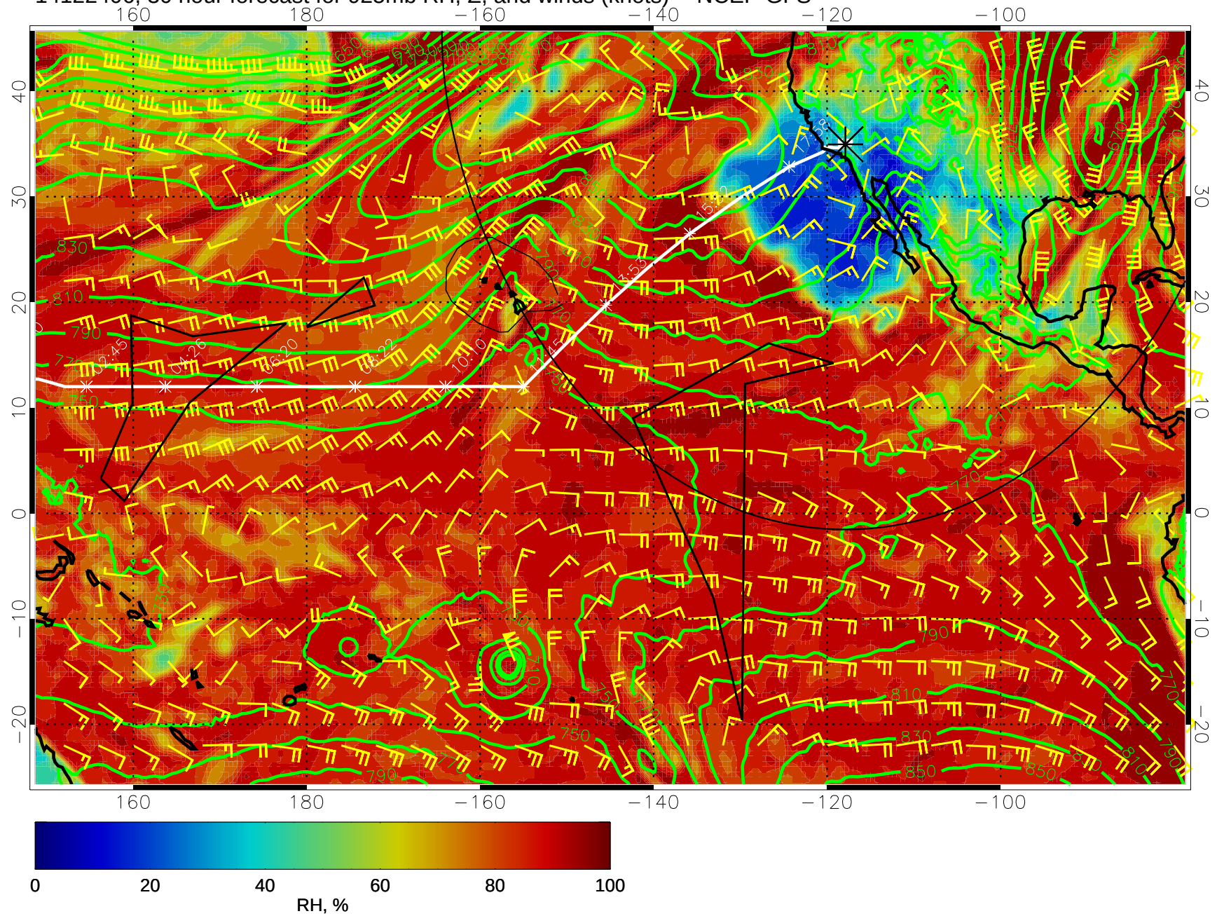
14122406, 30 hour forecast for 925mb RH, Z, and winds (knots) -- NCEP GFS
