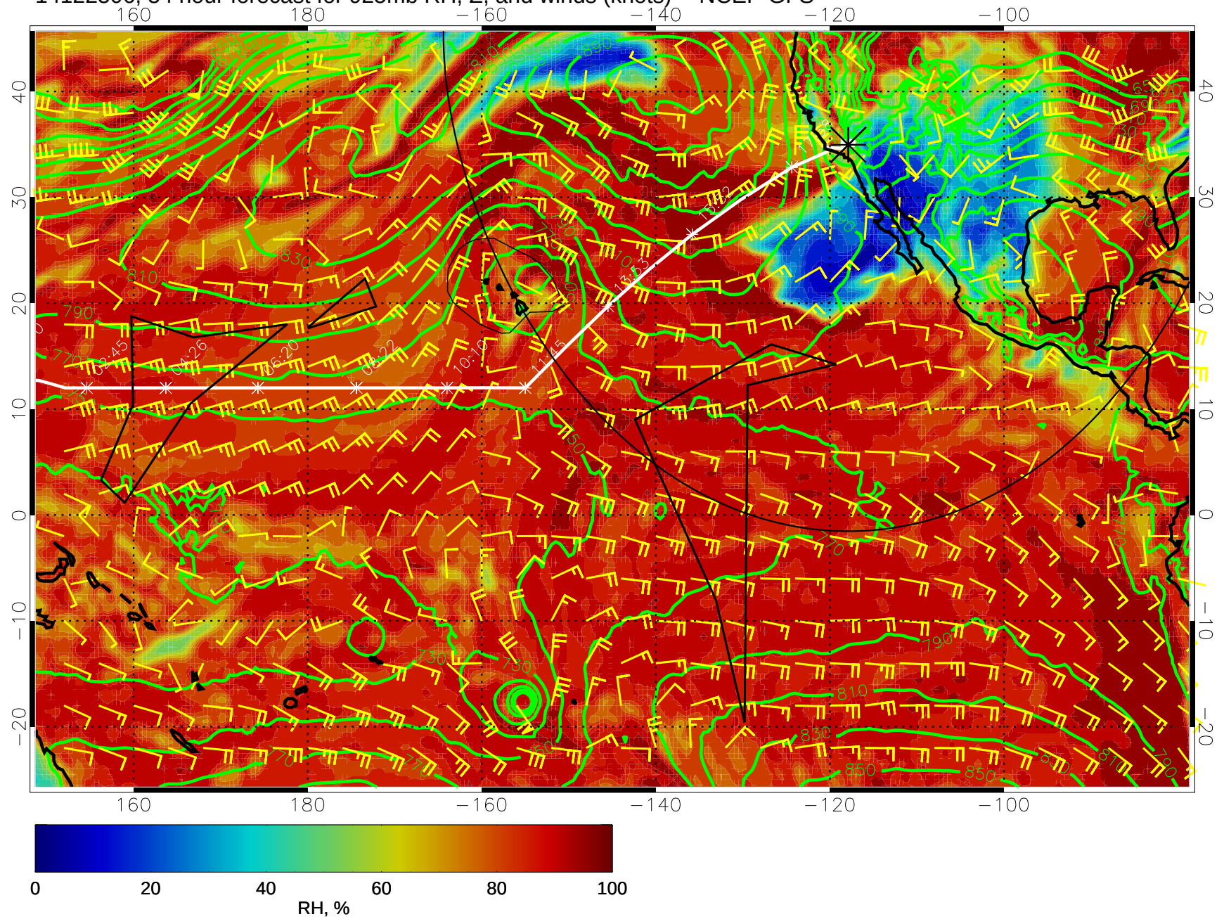
14122506, 54 hour forecast for 925mb RH, Z, and winds (knots) -- NCEP GFS
