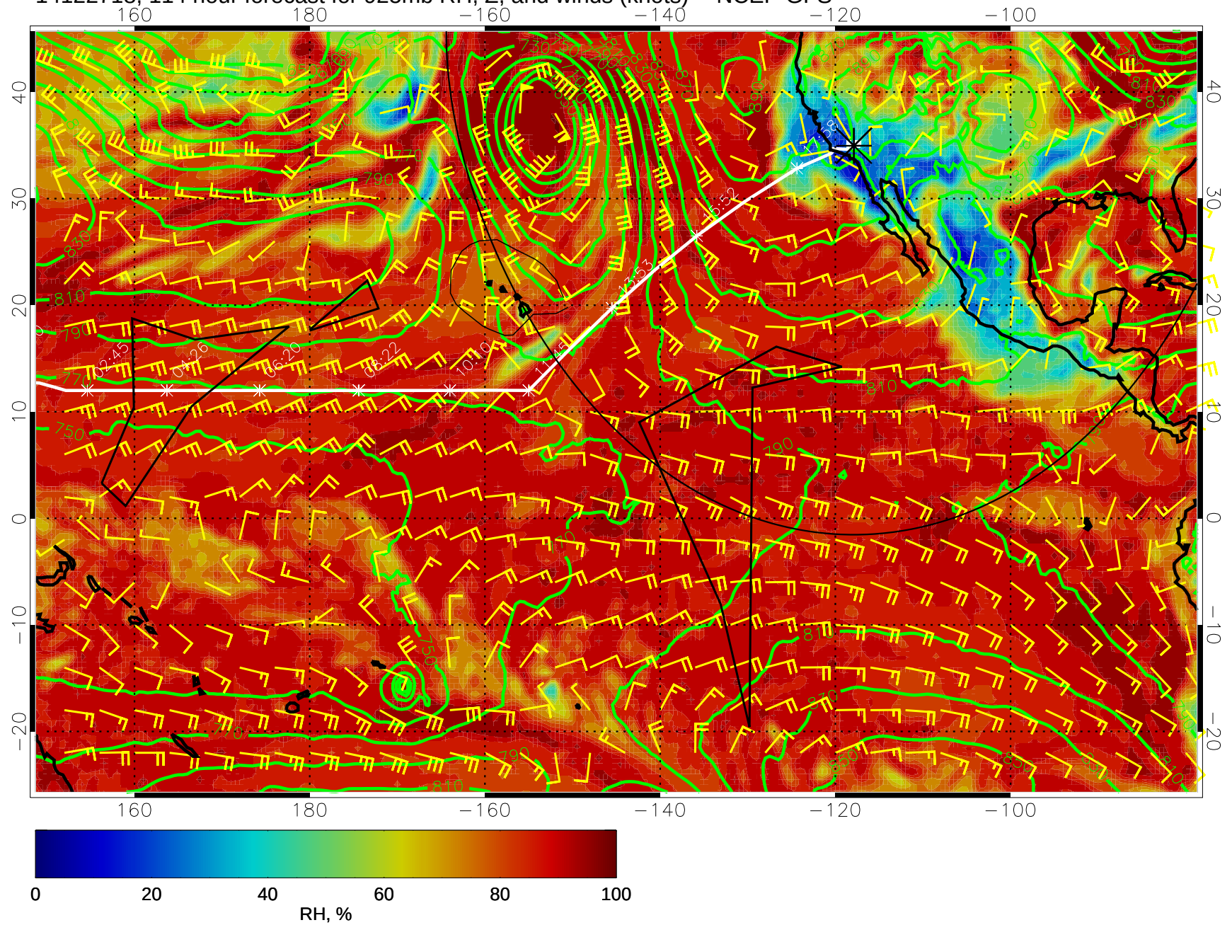
14122718, 114 hour forecast for 925mb RH, Z, and winds (knots) -- NCEP GFS
