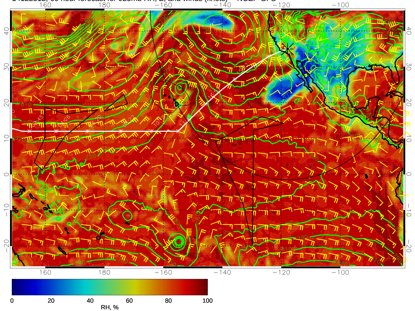
14122512, 60 hour forecast for 925mb RH, Z, and winds (knots) -- NCEP GFS
