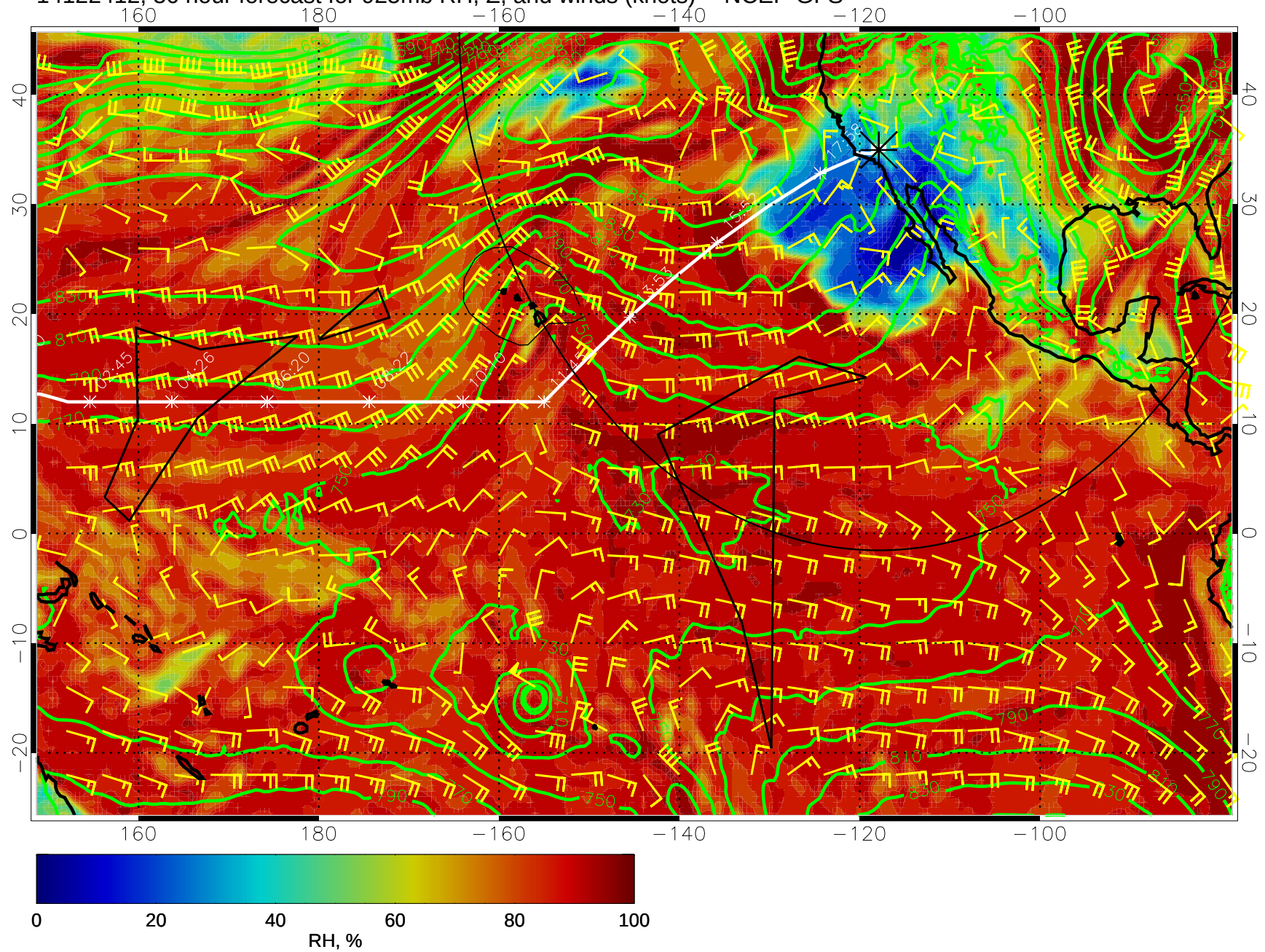
14122412, 36 hour forecast for 925mb RH, Z, and winds (knots) -- NCEP GFS
