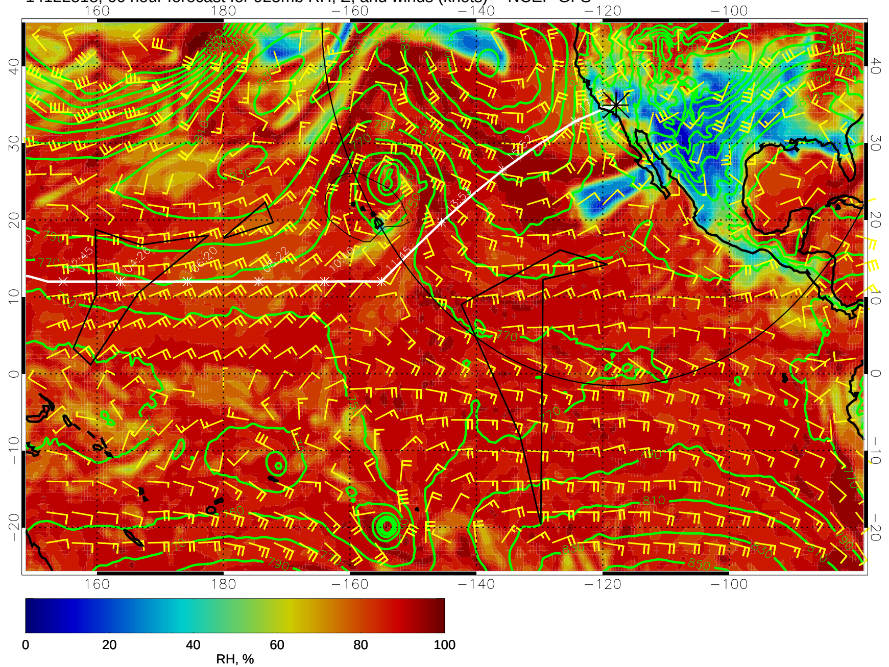
14122518, 66 hour forecast for 925mb RH, Z, and winds (knots) -- NCEP GFS
