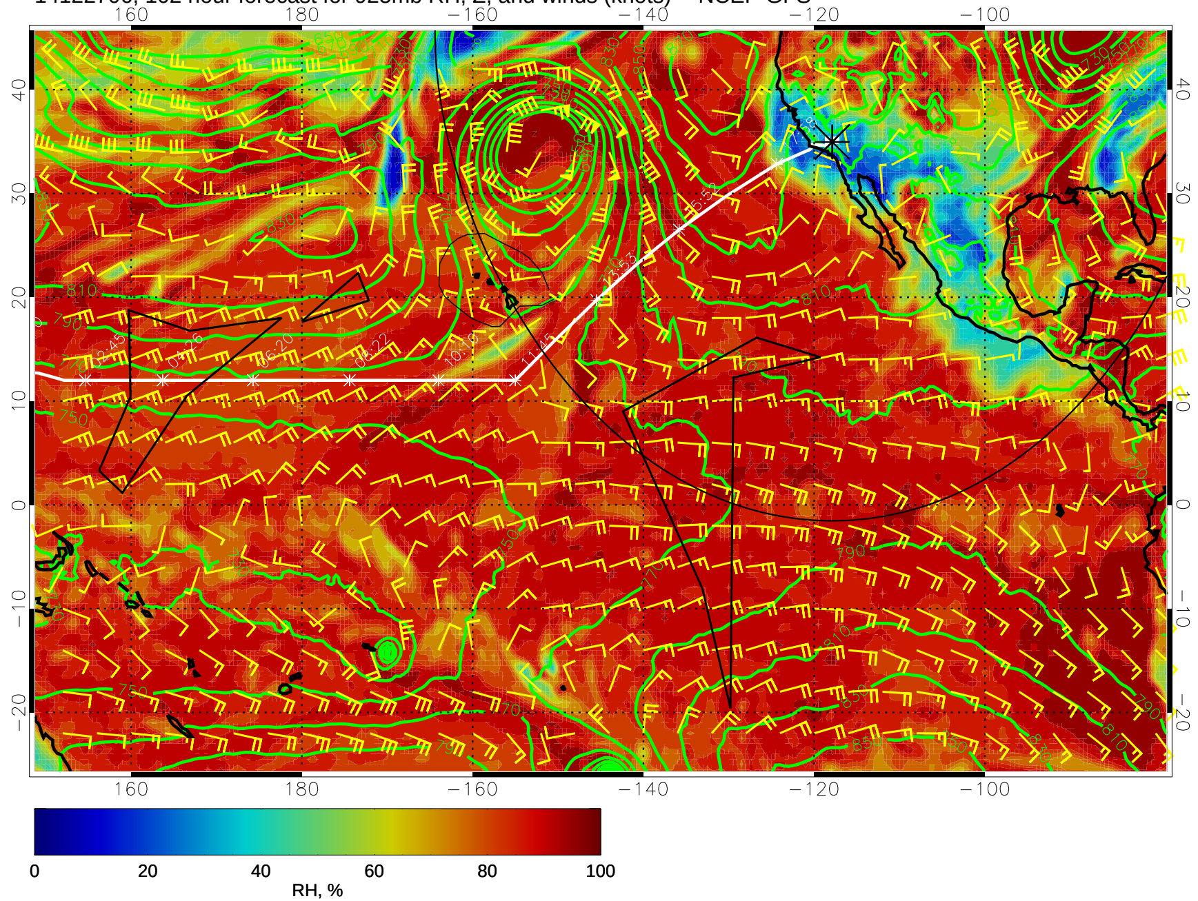
14122706, 102 hour forecast for 925mb RH, Z, and winds (knots) -- NCEP GFS
