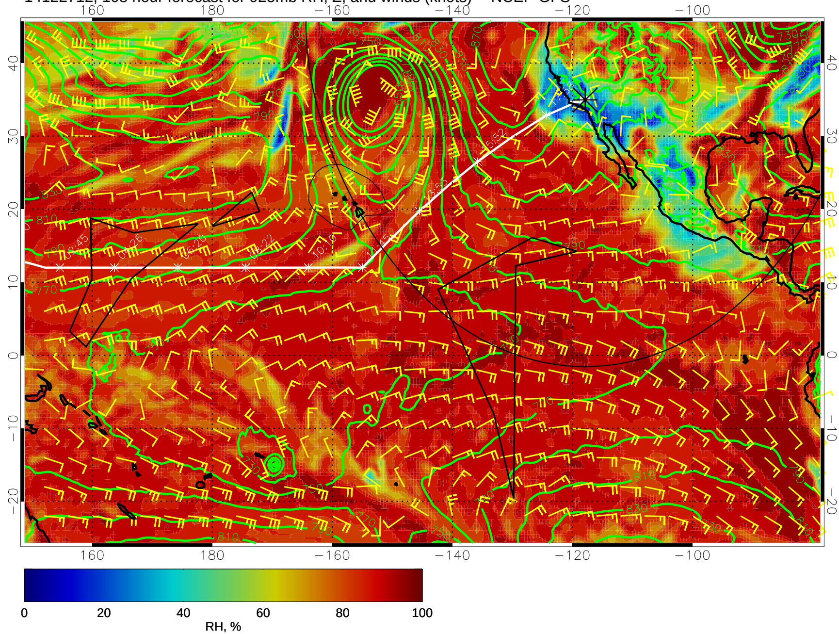
14122712, 108 hour forecast for 925mb RH, Z, and winds (knots) -- NCEP GFS
