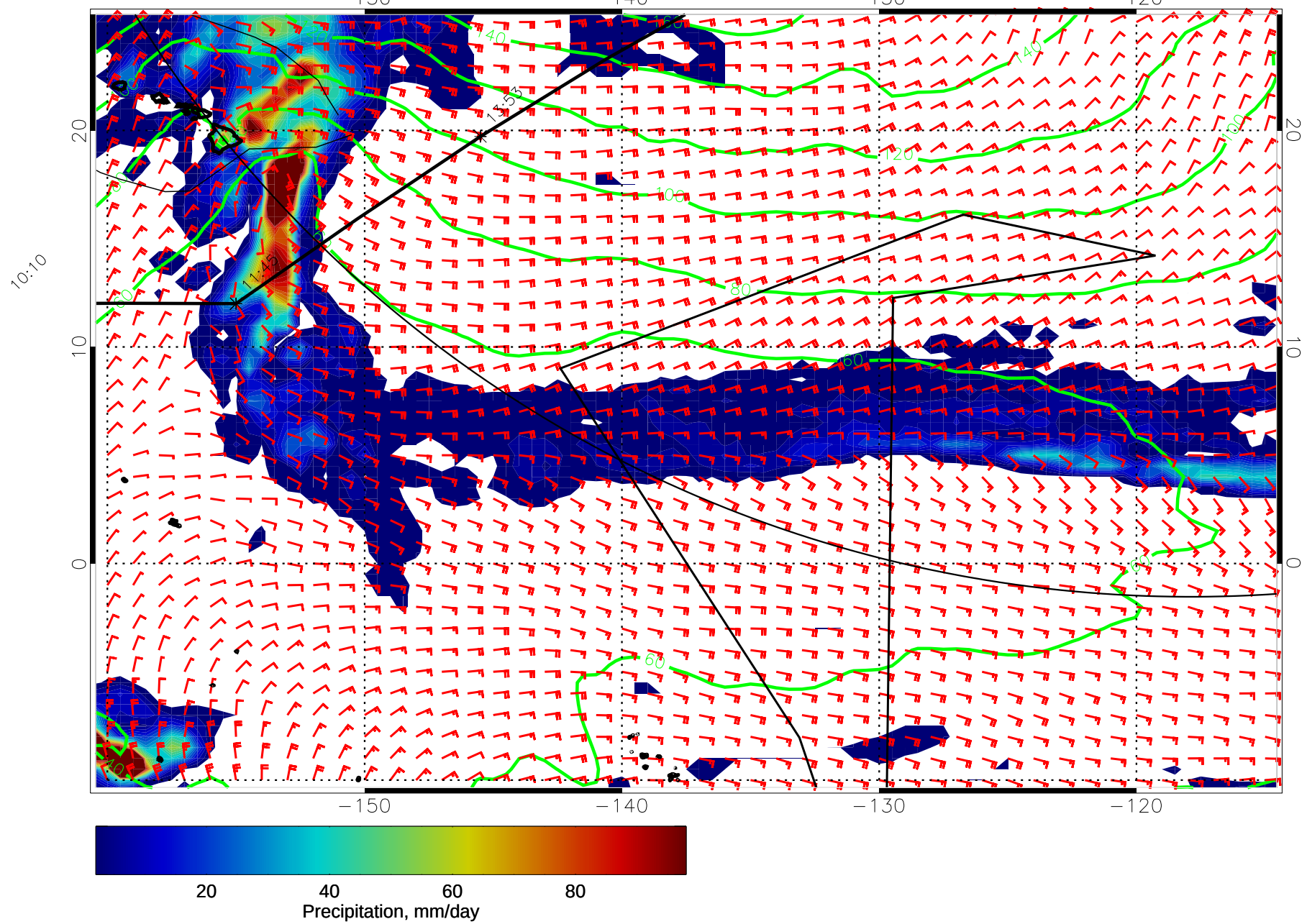
14122412, 36 hour forecast for precip, 1000mb Z, and winds (knots) -- NCEP GFS
