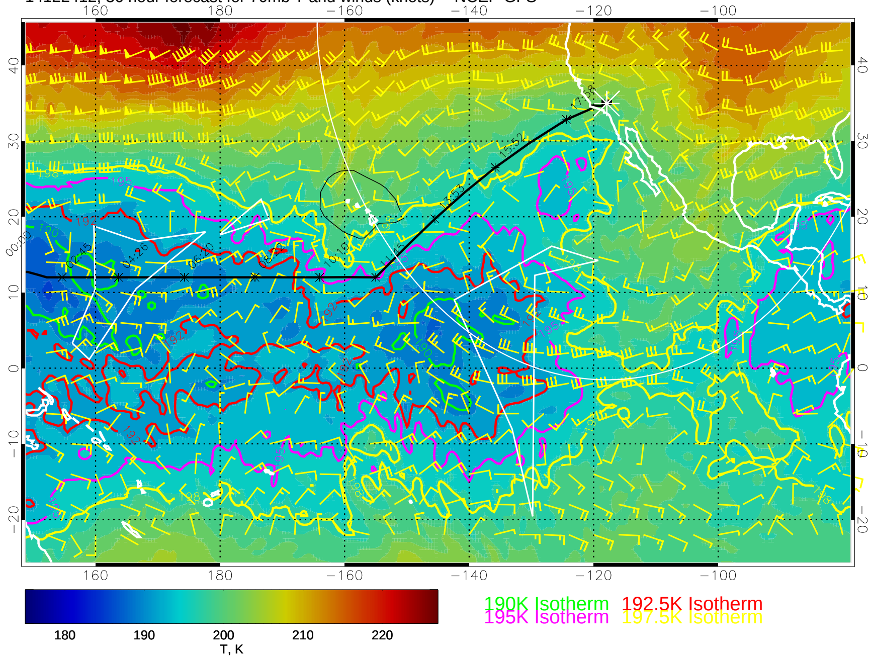
14122412, 36 hour forecast for 70mb T and winds (knots) -- NCEP GFS
