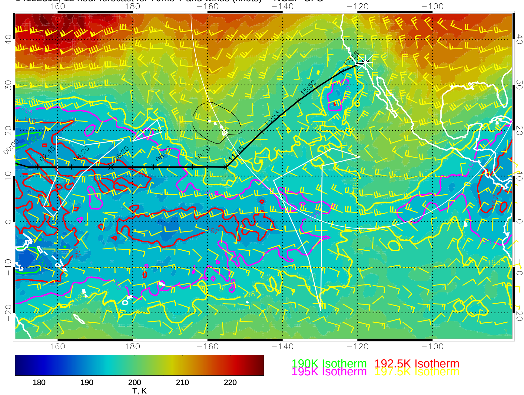
14122312, 12 hour forecast for 70mb T and winds (knots) -- NCEP GFS
