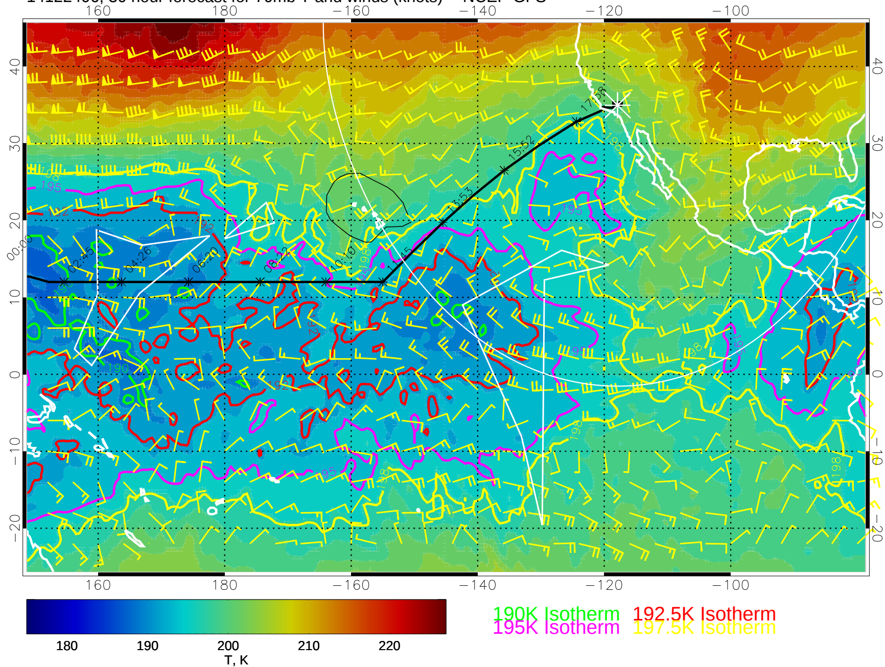
14122406, 30 hour forecast for 70mb T and winds (knots) -- NCEP GFS
