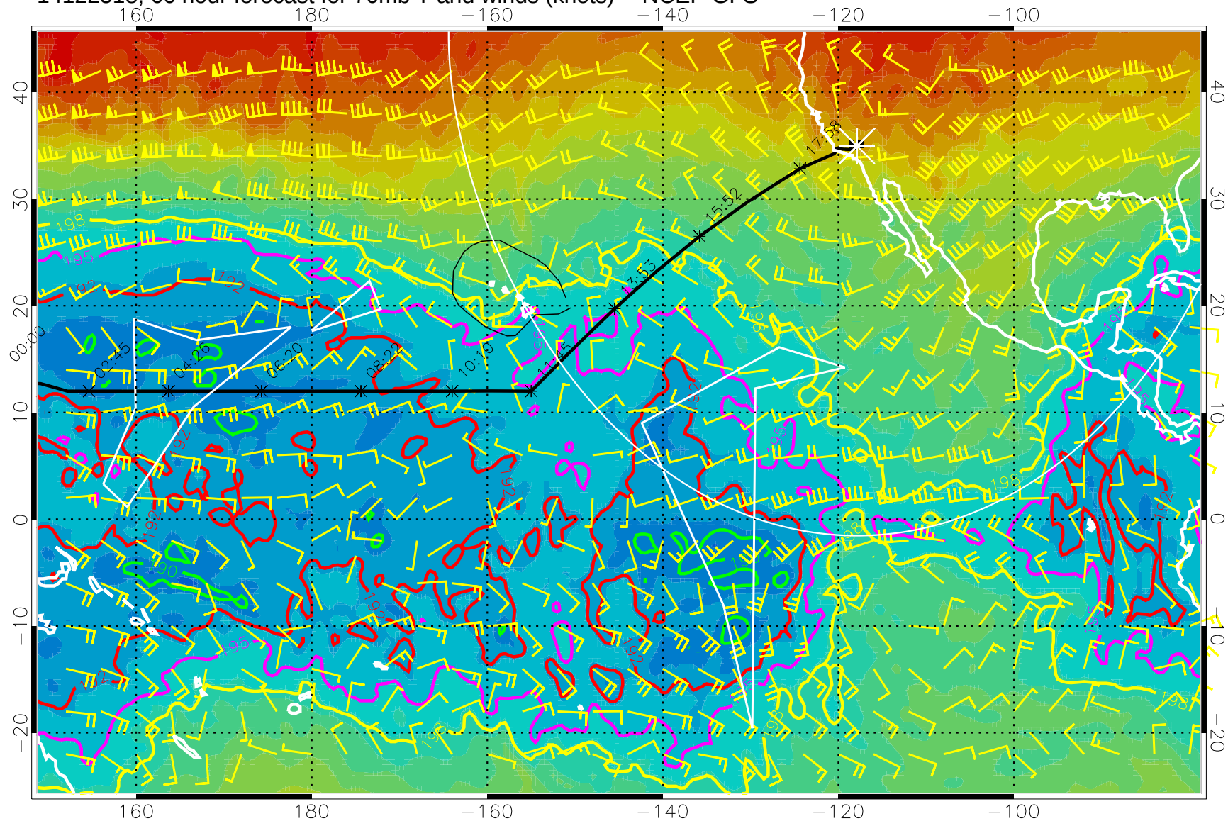
14122518, 66 hour forecast for 70mb T and winds (knots) -- NCEP GFS
