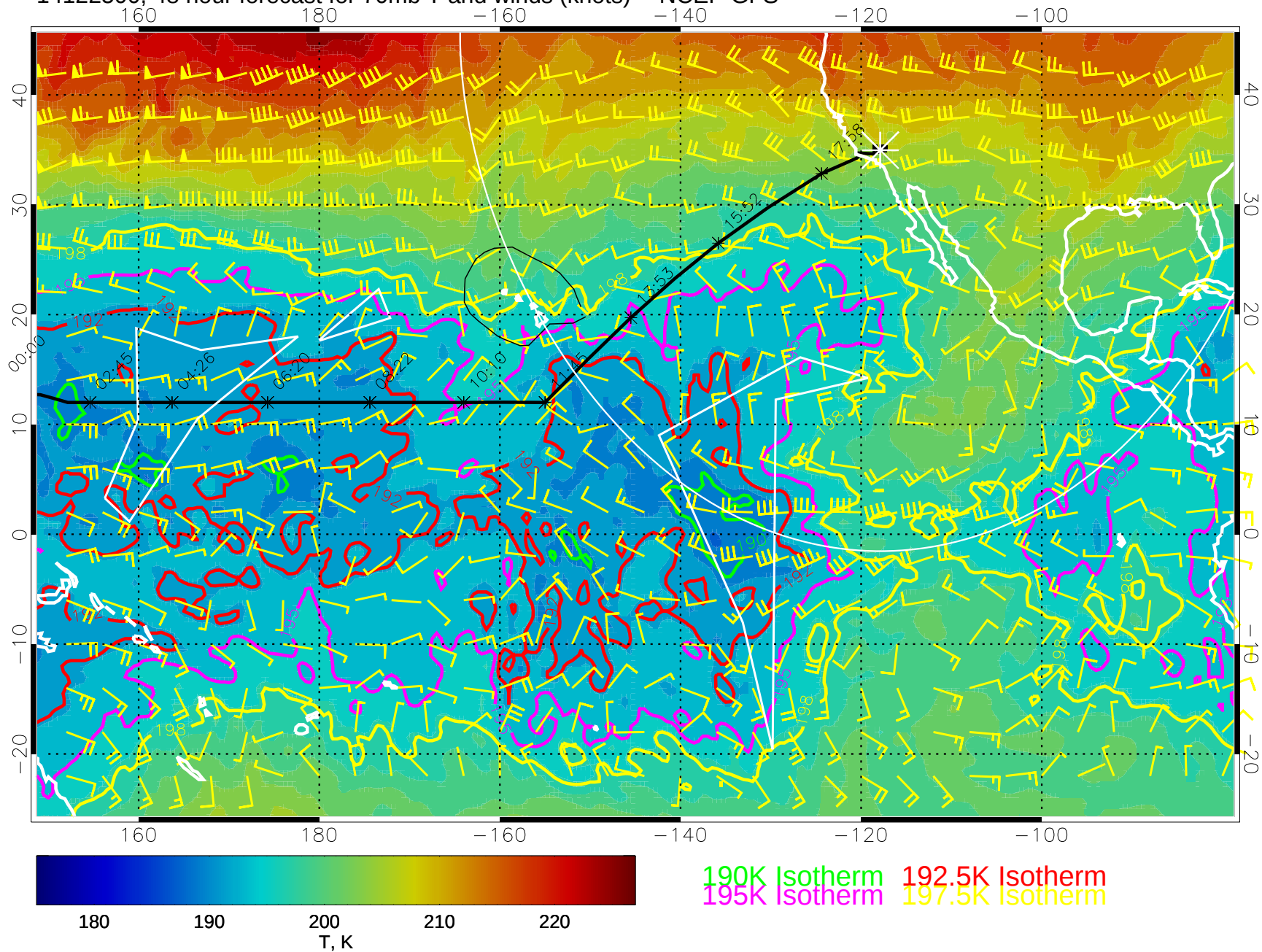
14122500, 48 hour forecast for 70mb T and winds (knots) -- NCEP GFS
