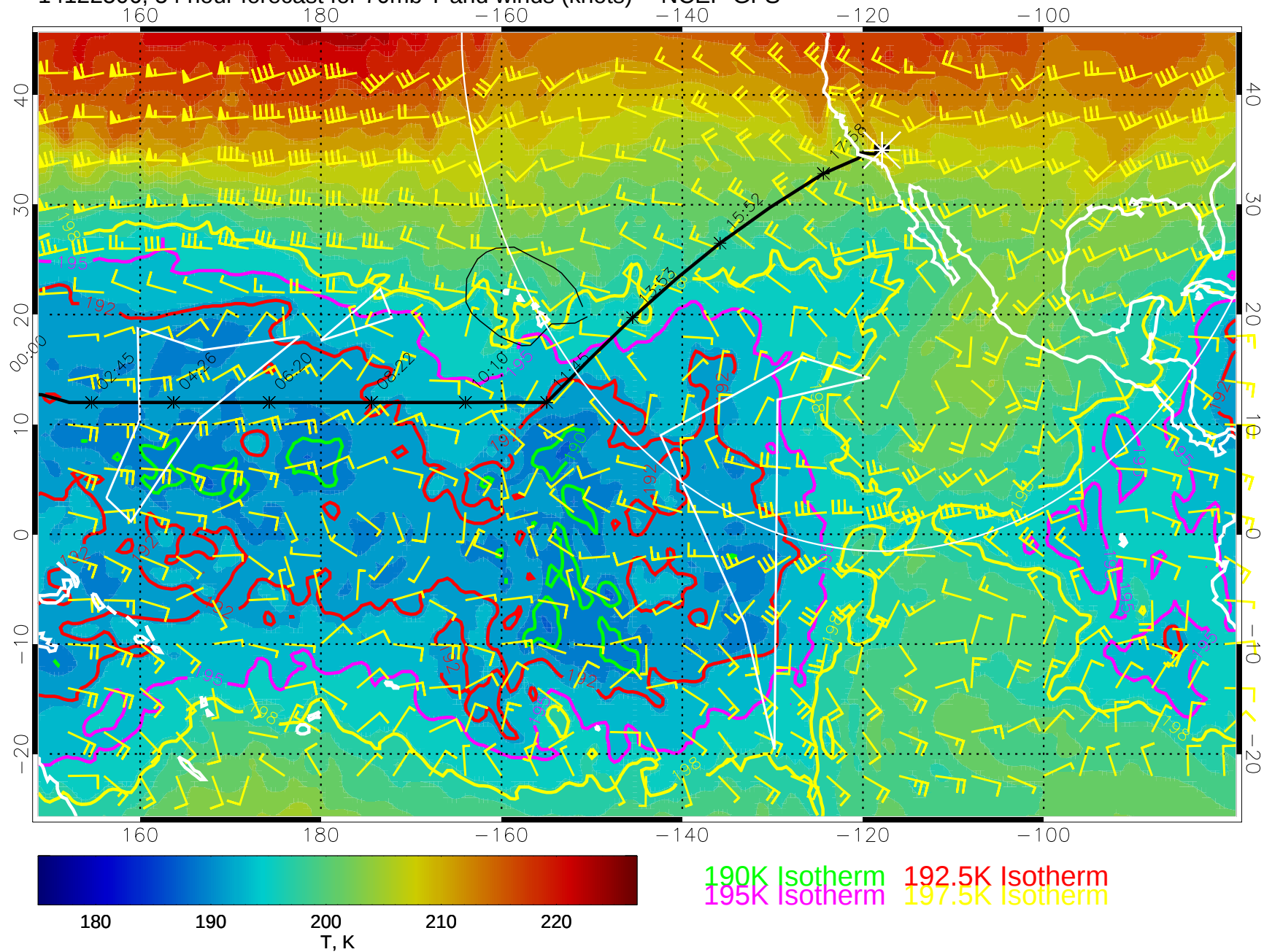
14122506, 54 hour forecast for 70mb T and winds (knots) -- NCEP GFS
