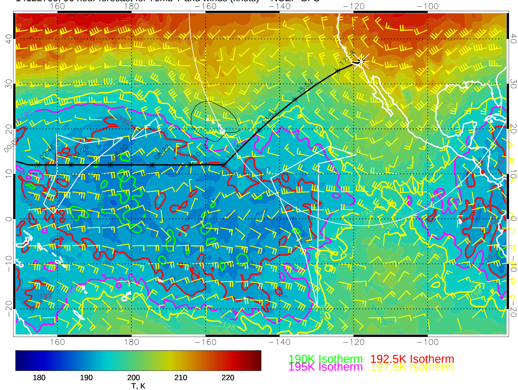
14122700, 96 hour forecast for 70mb T and winds (knots) -- NCEP GFS
