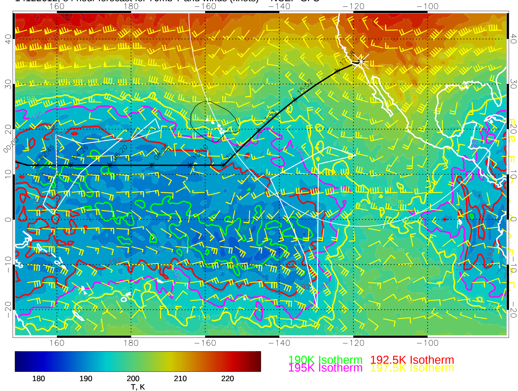
14122612, 84 hour forecast for 70mb T and winds (knots) -- NCEP GFS
