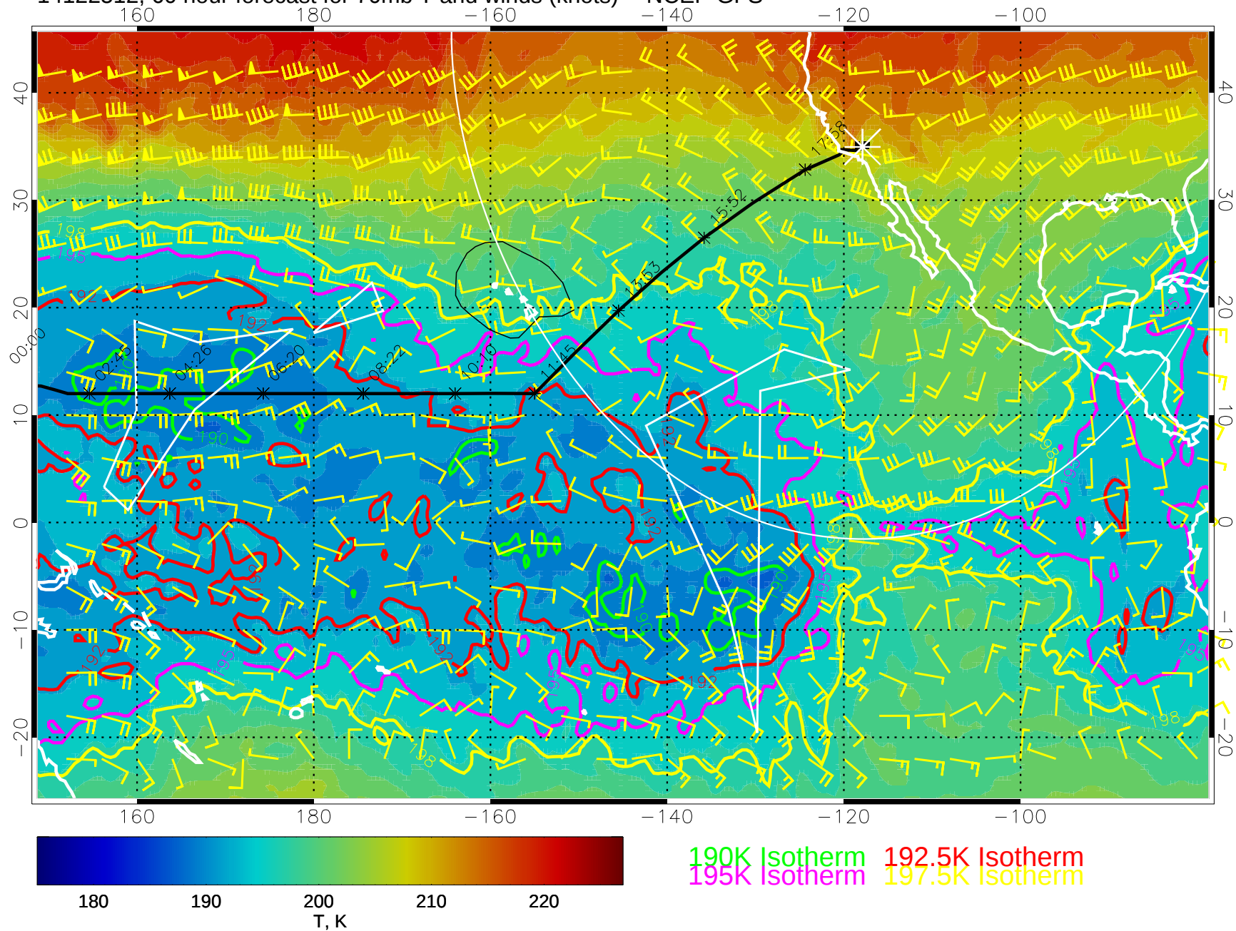
14122512, 60 hour forecast for 70mb T and winds (knots) -- NCEP GFS
