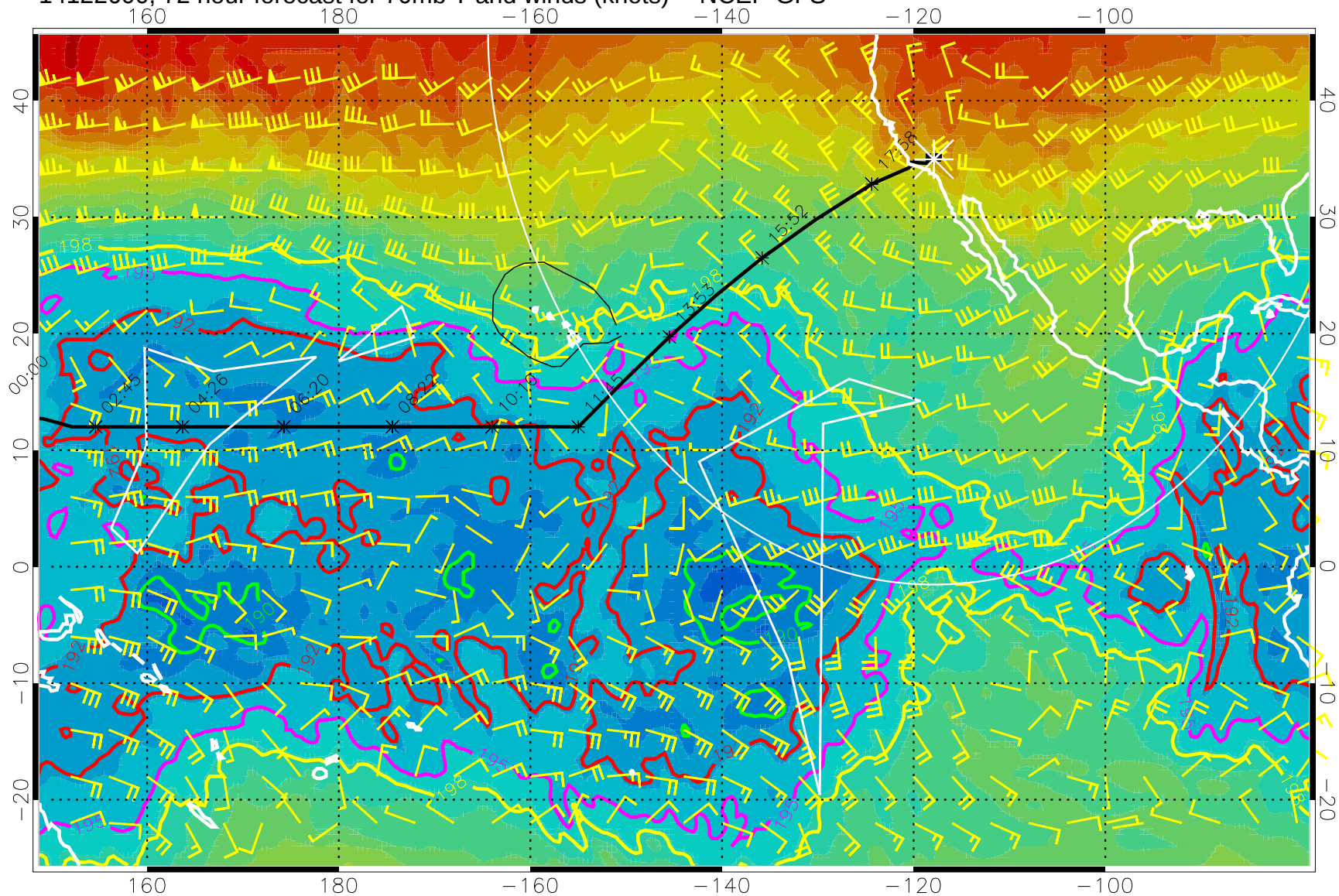
14122600, 72 hour forecast for 70mb T and winds (knots) -- NCEP GFS
