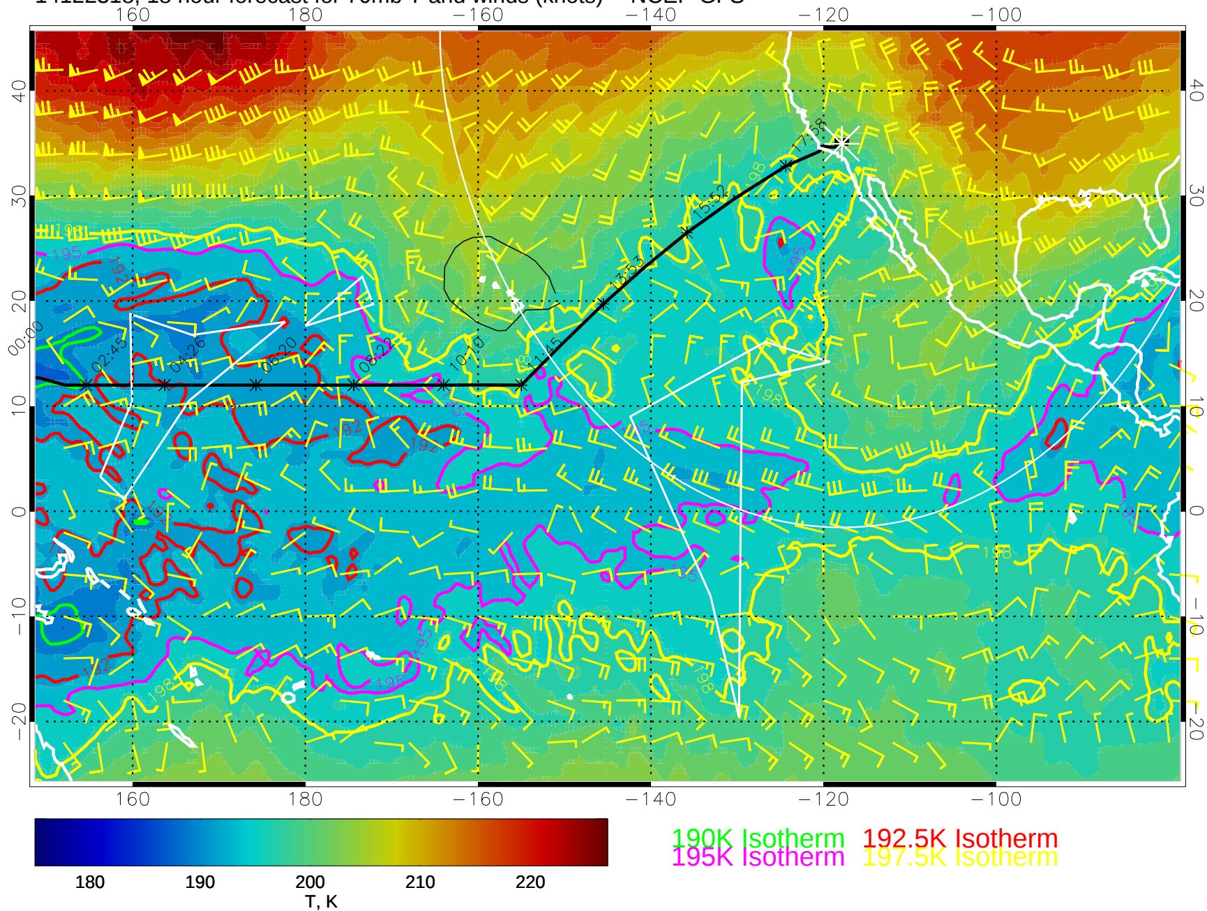
14122318, 18 hour forecast for 70mb T and winds (knots) -- NCEP GFS
