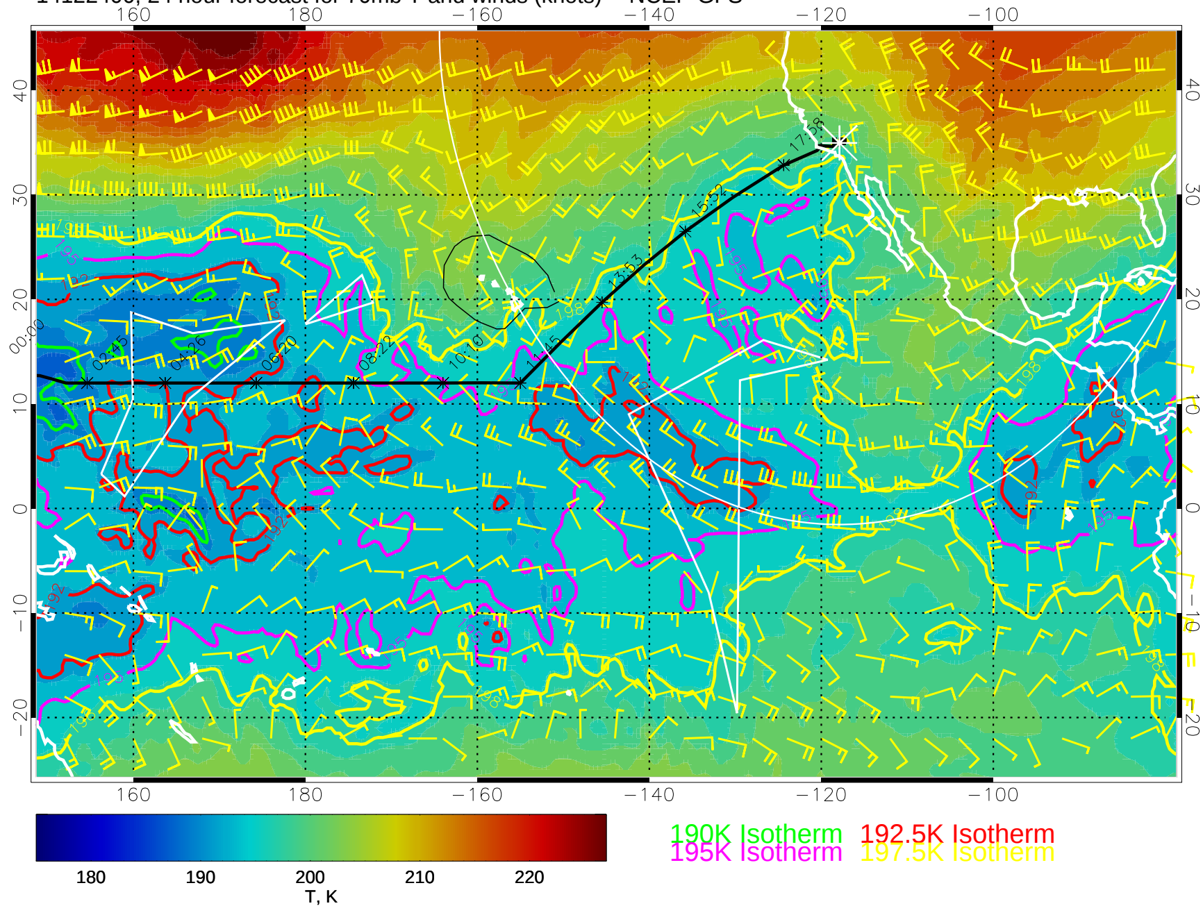
14122400, 24 hour forecast for 70mb T and winds (knots) -- NCEP GFS
