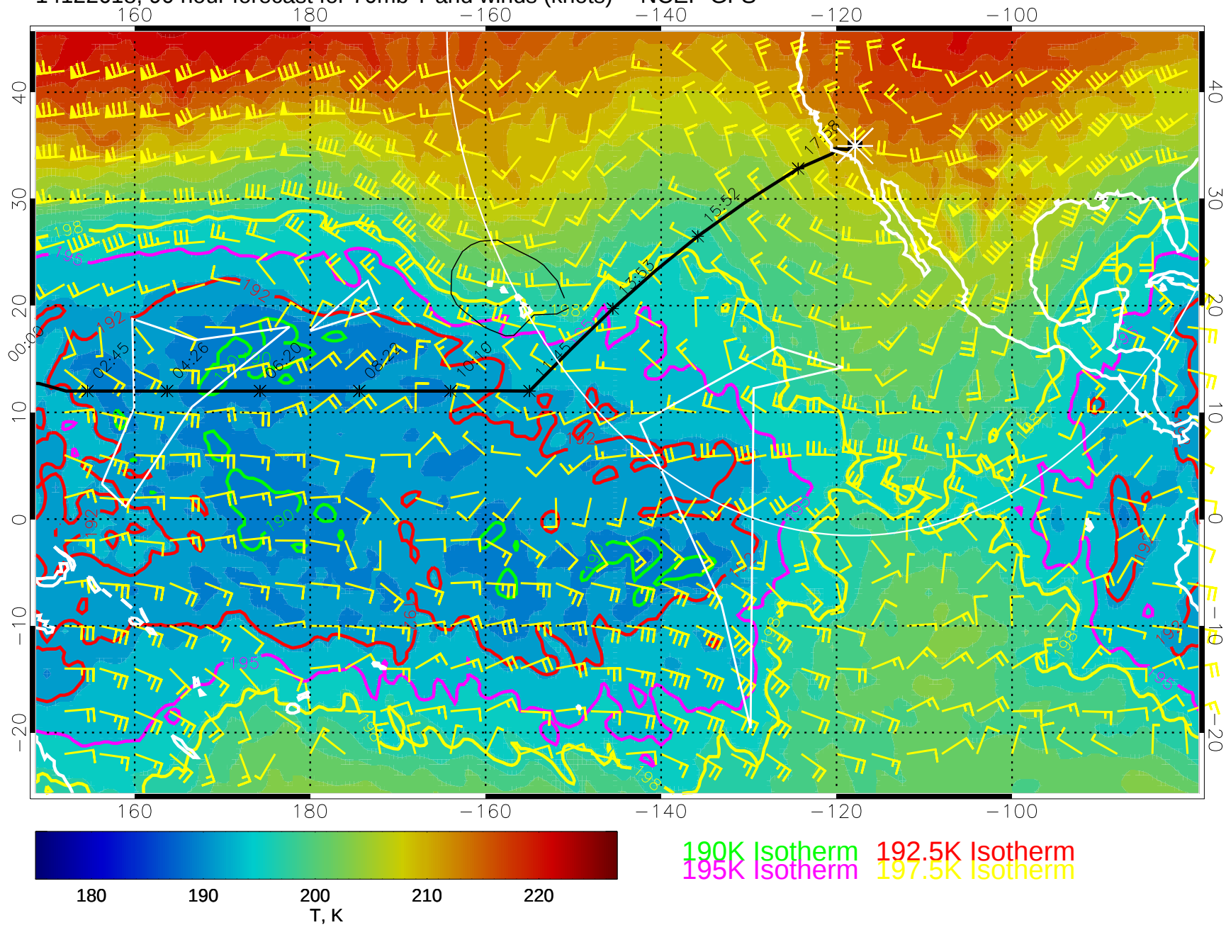
14122618, 90 hour forecast for 70mb T and winds (knots) -- NCEP GFS
