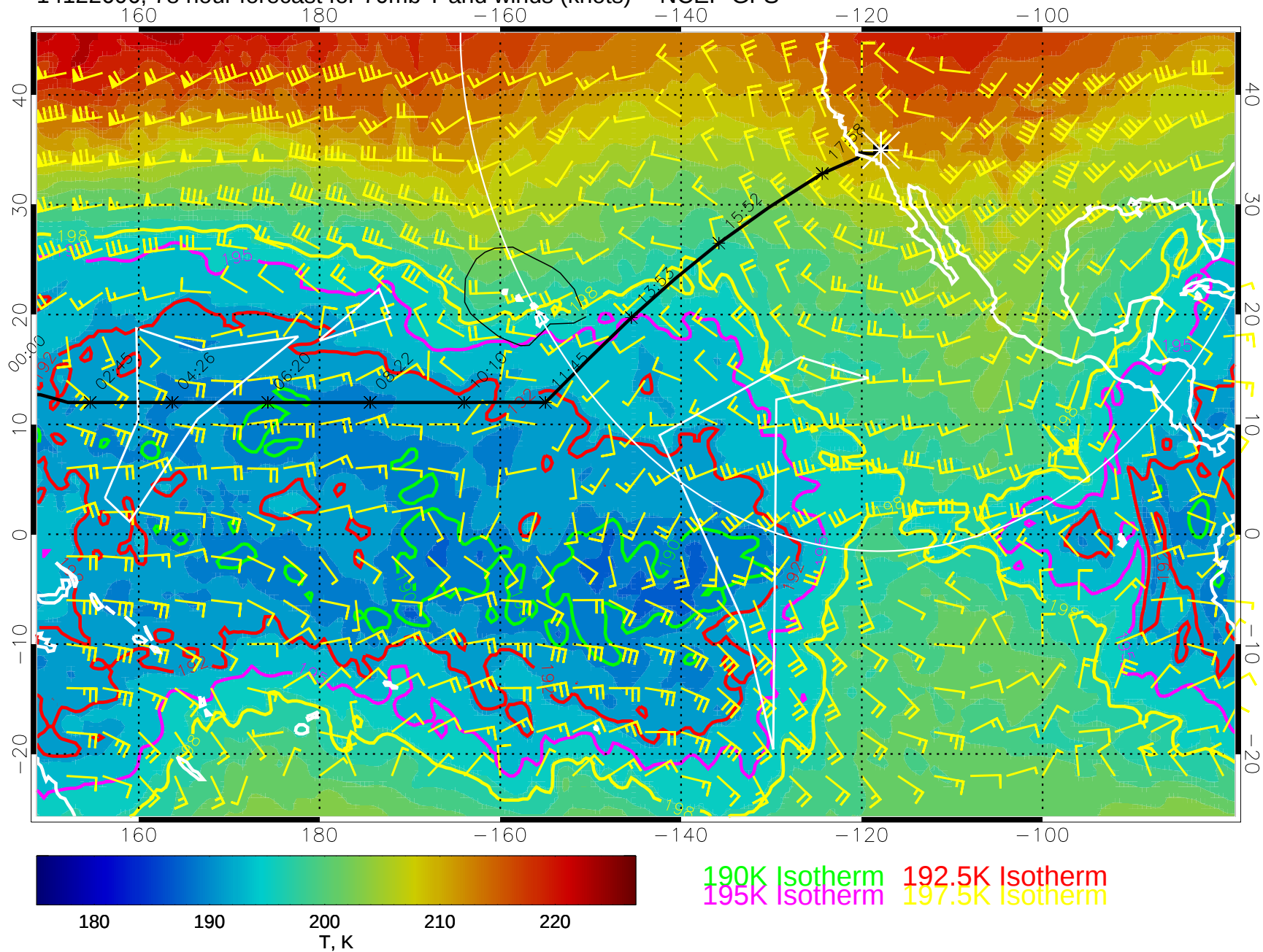
14122606, 78 hour forecast for 70mb T and winds (knots) -- NCEP GFS
