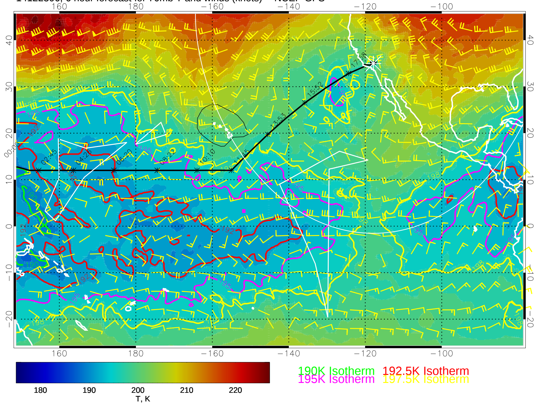
14122306, 6 hour forecast for 70mb T and winds (knots) -- NCEP GFS
