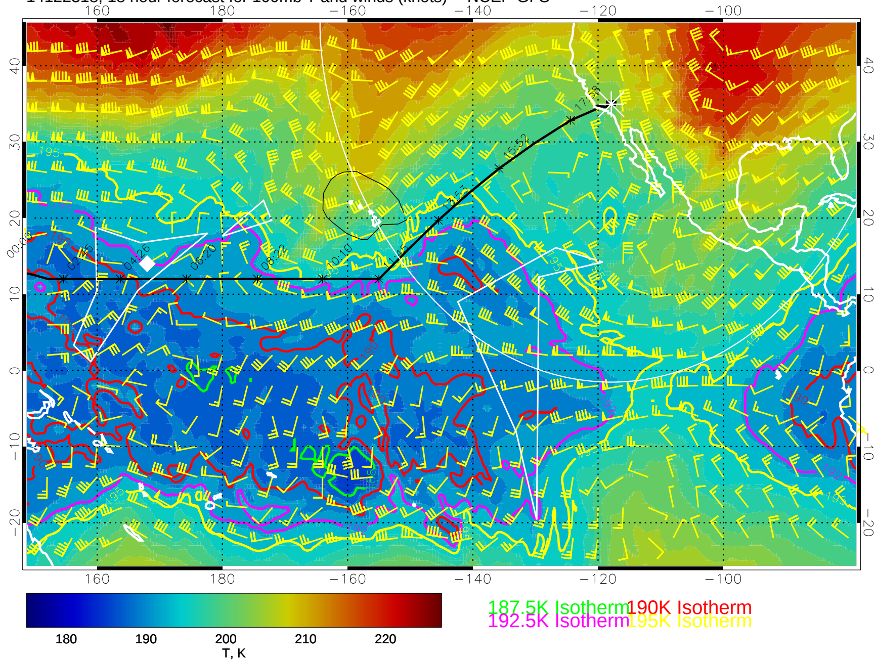
14122318, 18 hour forecast for 100mb T and winds (knots) -- NCEP GFS
