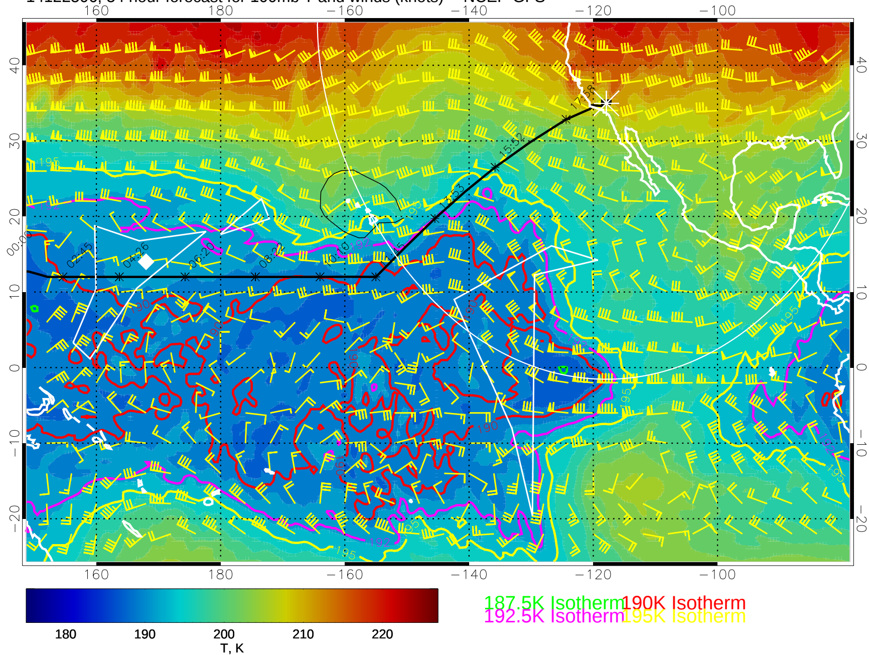
14122506, 54 hour forecast for 100mb T and winds (knots) -- NCEP GFS
