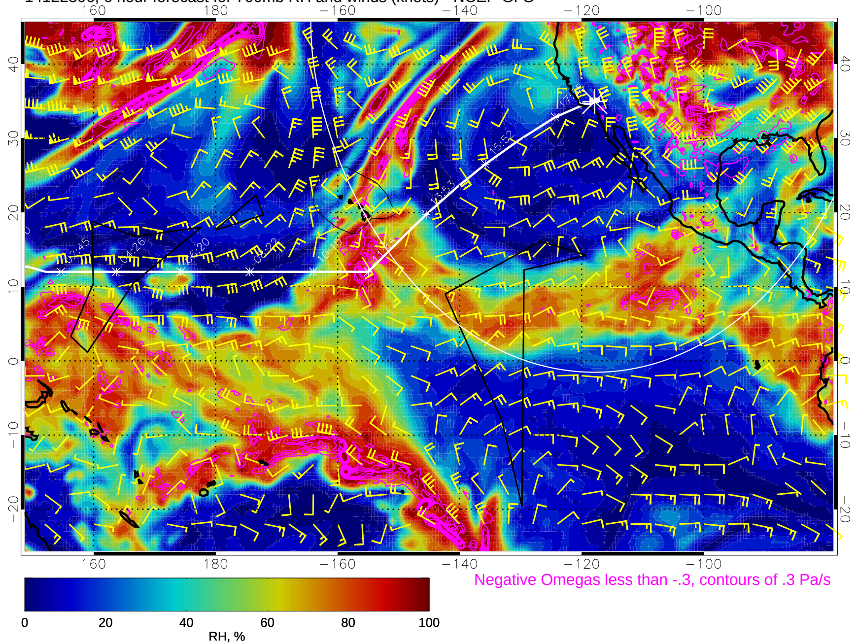
14122306, 6 hour forecast for 700mb RH and winds (knots) - NCEP GFS
