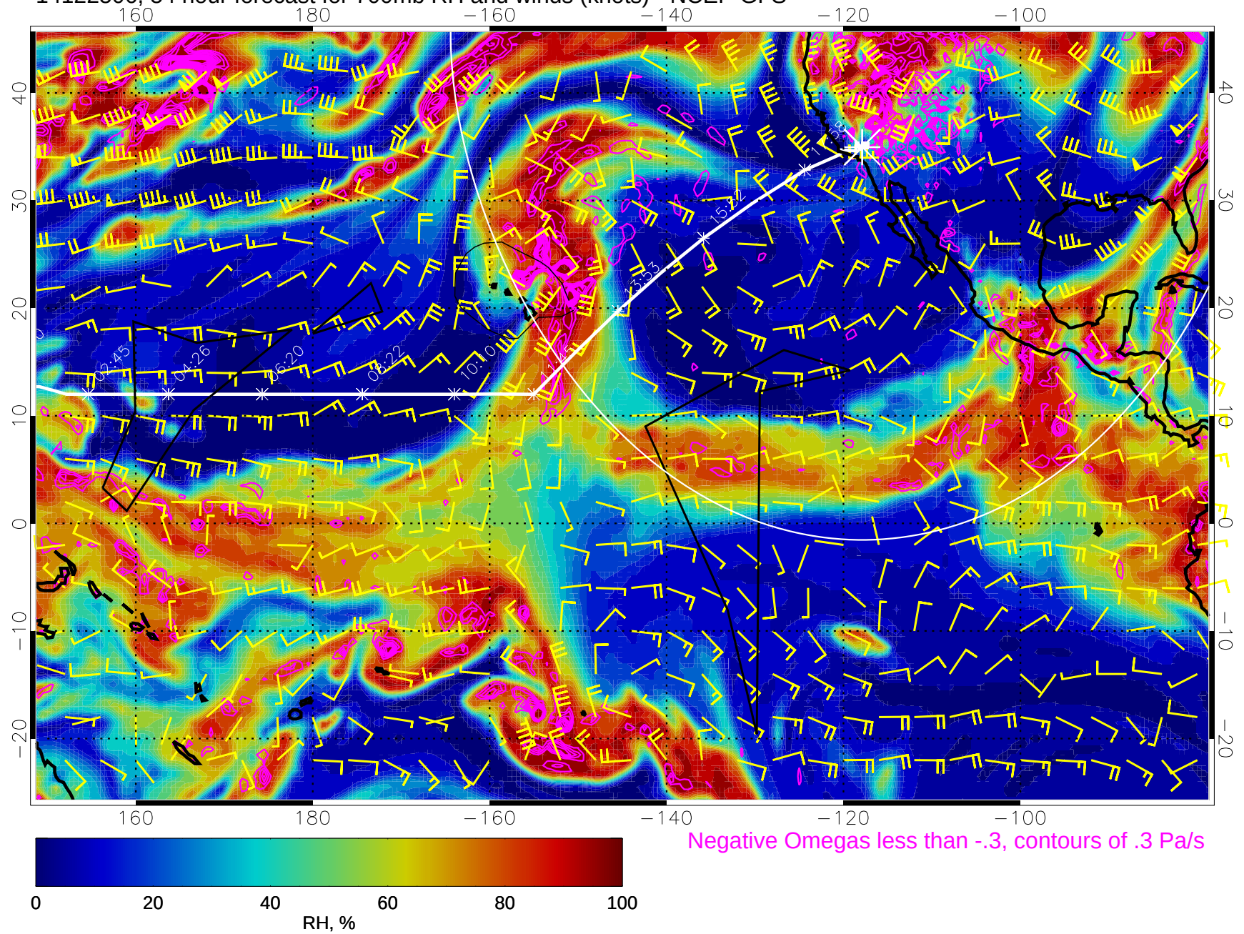
14122506, 54 hour forecast for 700mb RH and winds (knots) - NCEP GFS
