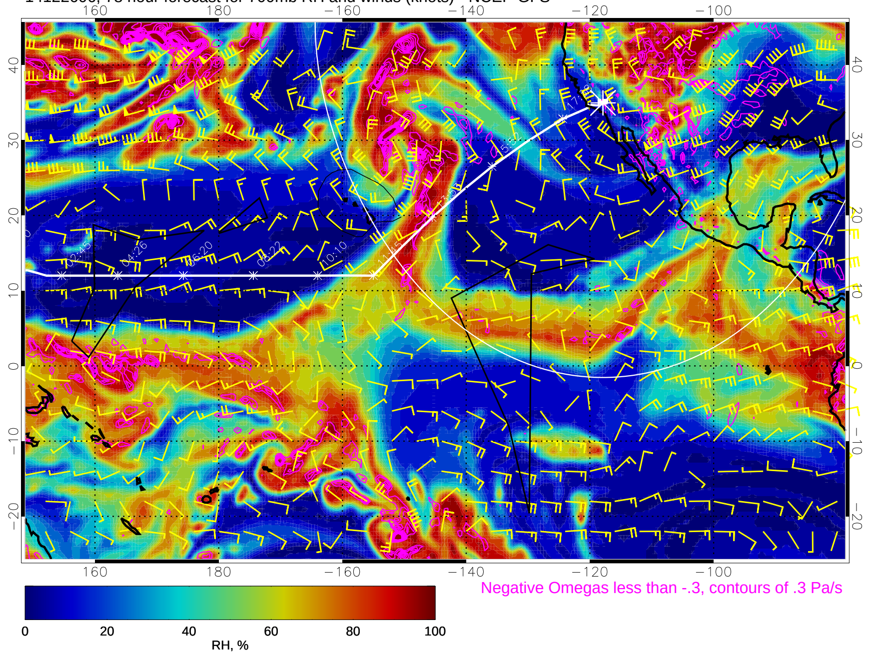
14122606, 78 hour forecast for 700mb RH and winds (knots) - NCEP GFS
