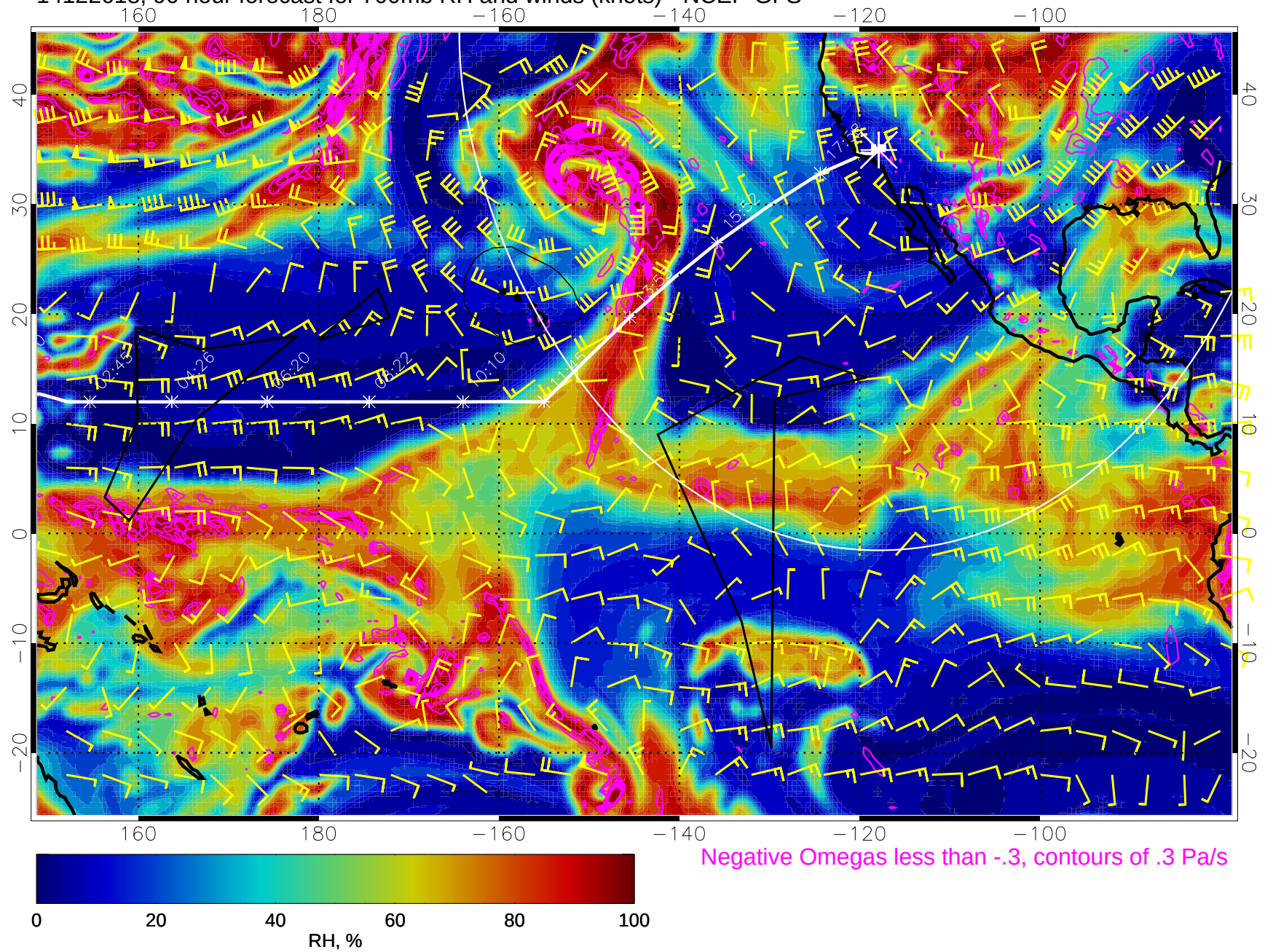
14122618, 90 hour forecast for 700mb RH and winds (knots) - NCEP GFS
