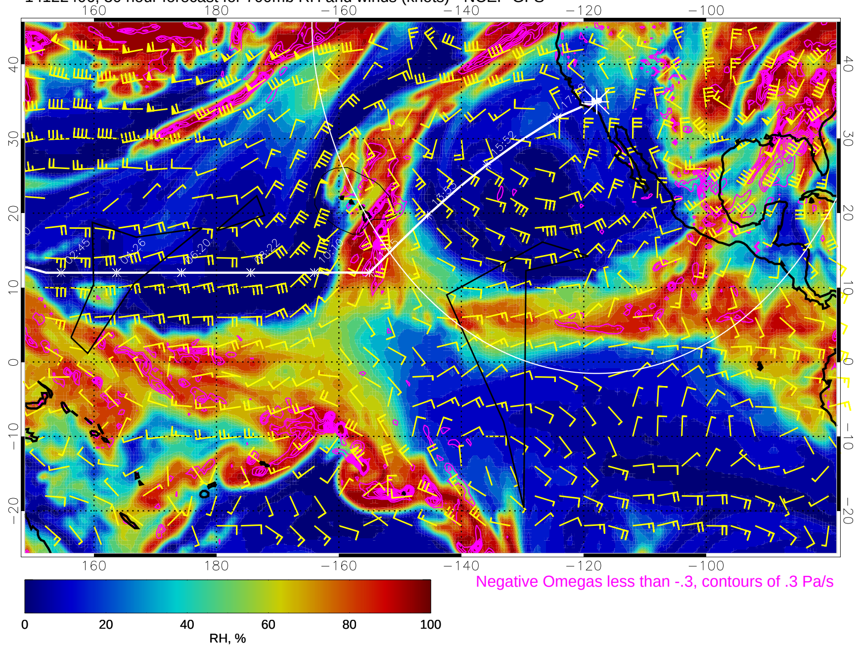
14122406, 30 hour forecast for 700mb RH and winds (knots) - NCEP GFS
