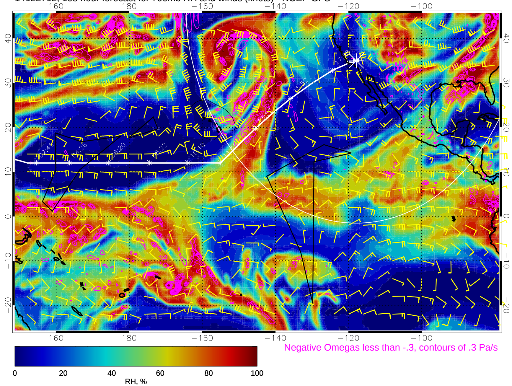
14122712, 108 hour forecast for 700mb RH and winds (knots) - NCEP GFS
