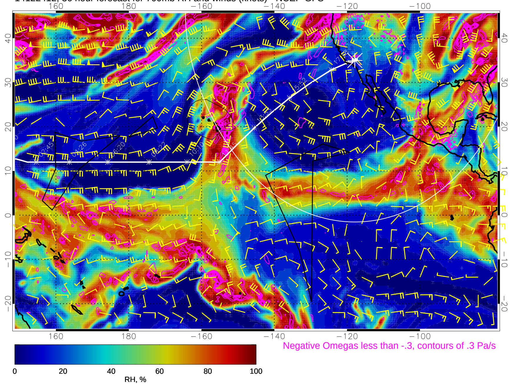
14122412, 36 hour forecast for 700mb RH and winds (knots) - NCEP GFS
