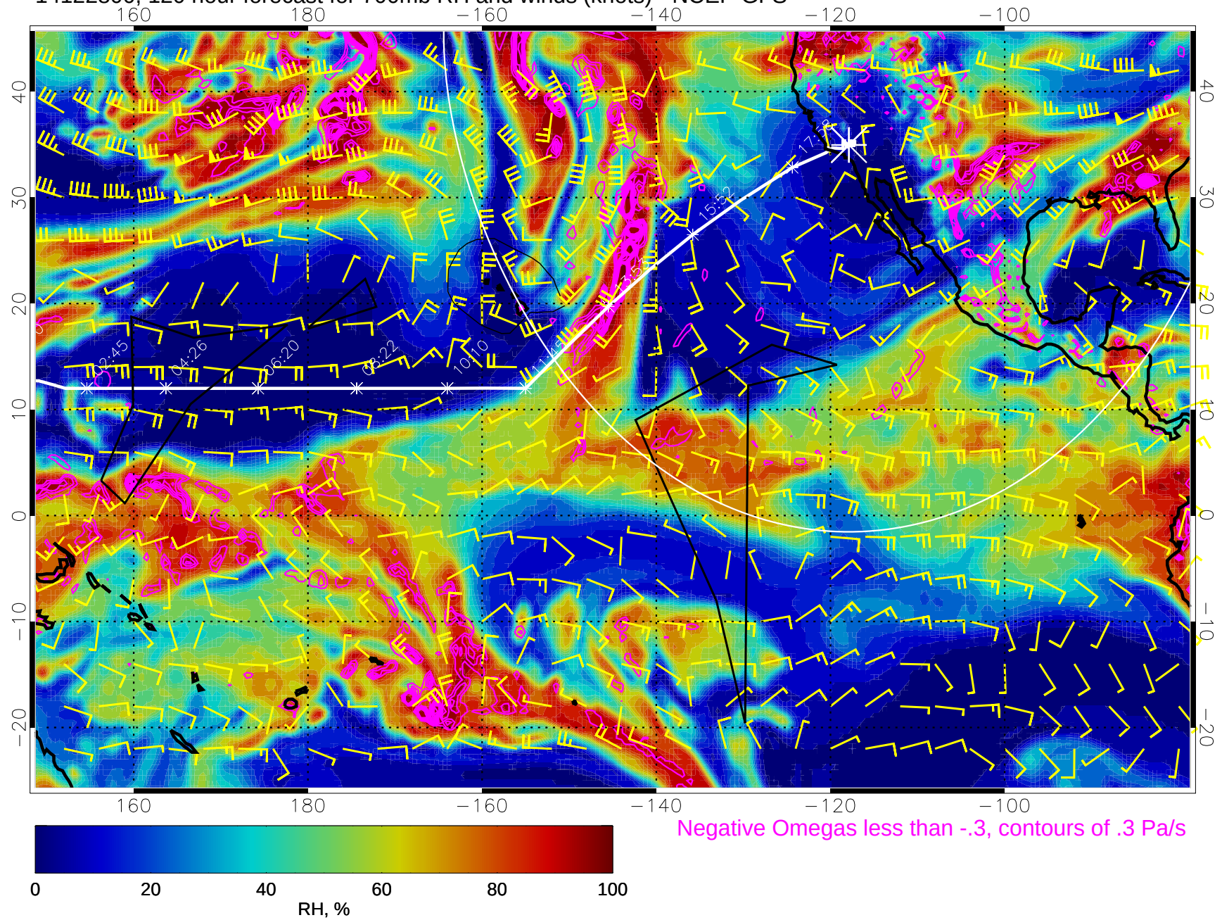
14122800, 120 hour forecast for 700mb RH and winds (knots) - NCEP GFS
