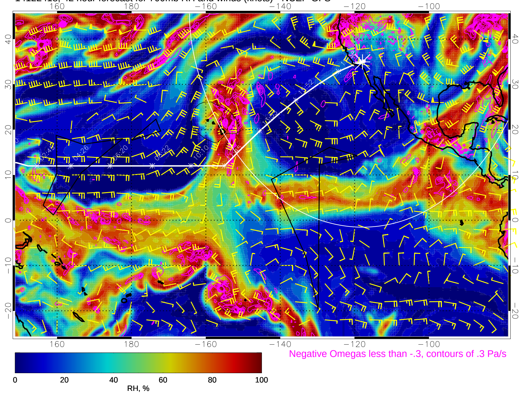
14122418, 42 hour forecast for 700mb RH and winds (knots) - NCEP GFS
