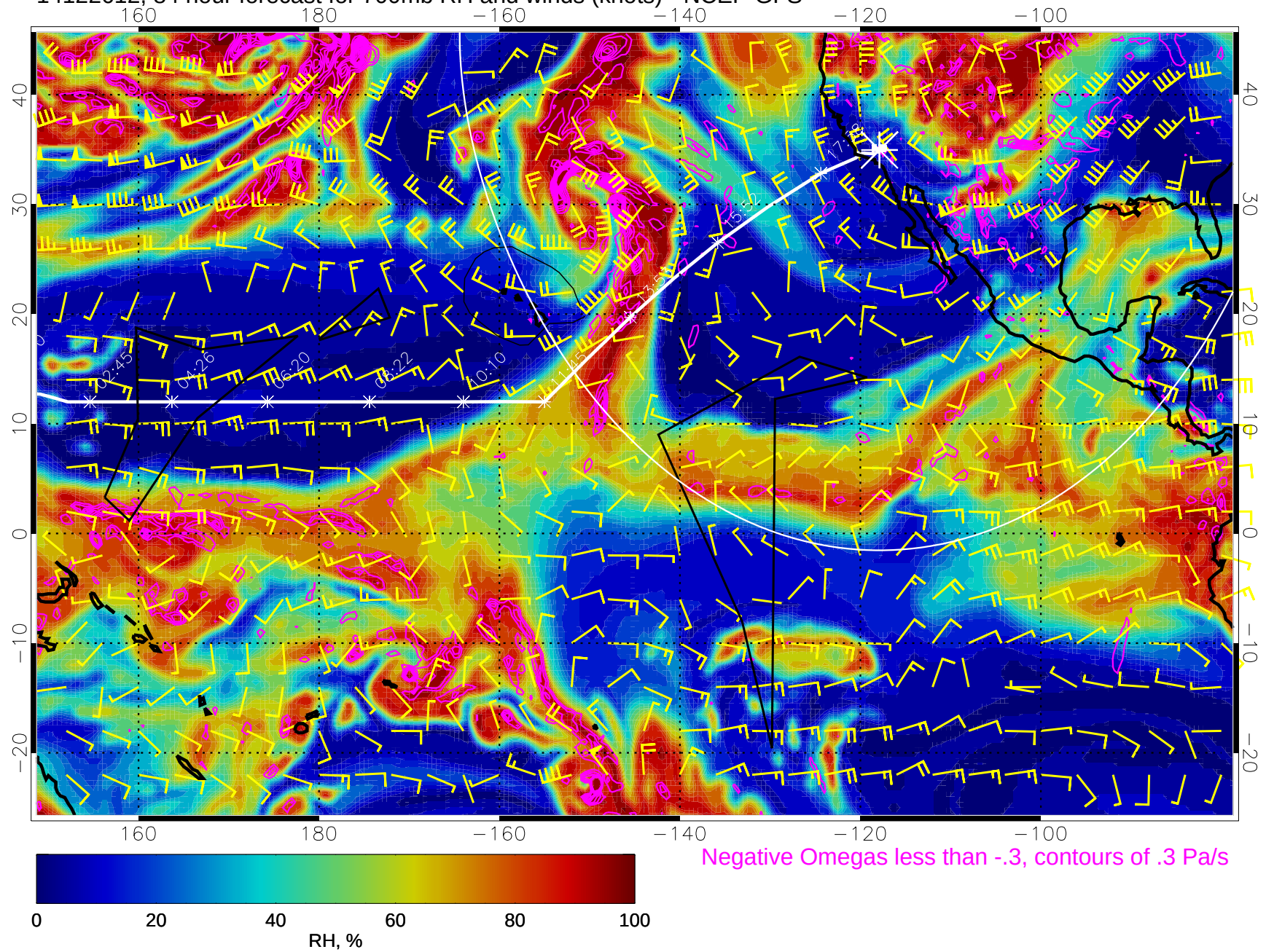
14122612, 84 hour forecast for 700mb RH and winds (knots) - NCEP GFS
