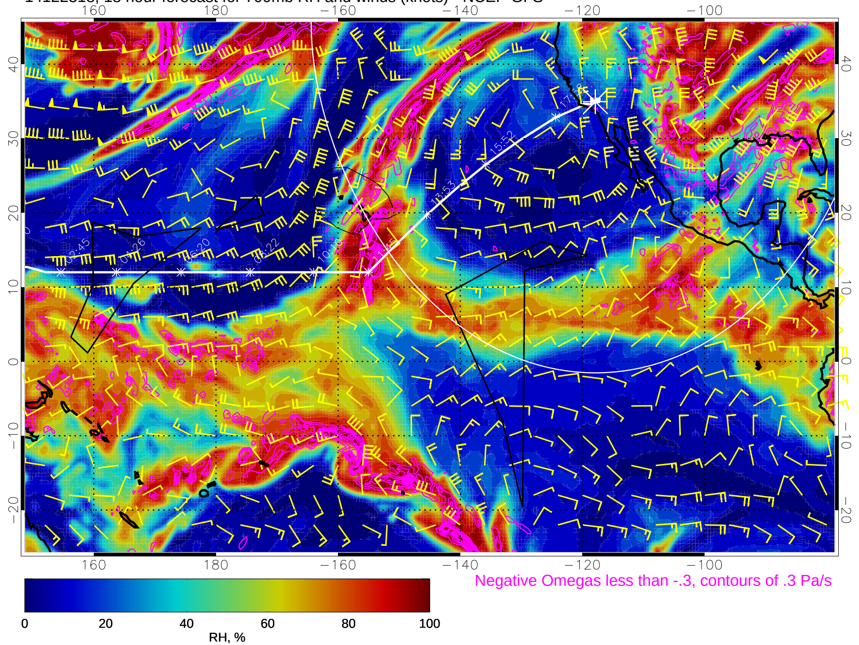
14122318, 18 hour forecast for 700mb RH and winds (knots) - NCEP GFS
