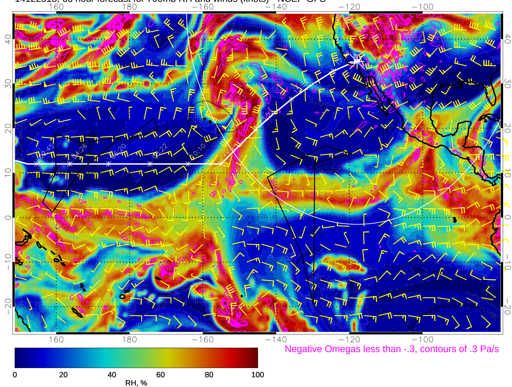
14122518, 66 hour forecast for 700mb RH and winds (knots) - NCEP GFS
