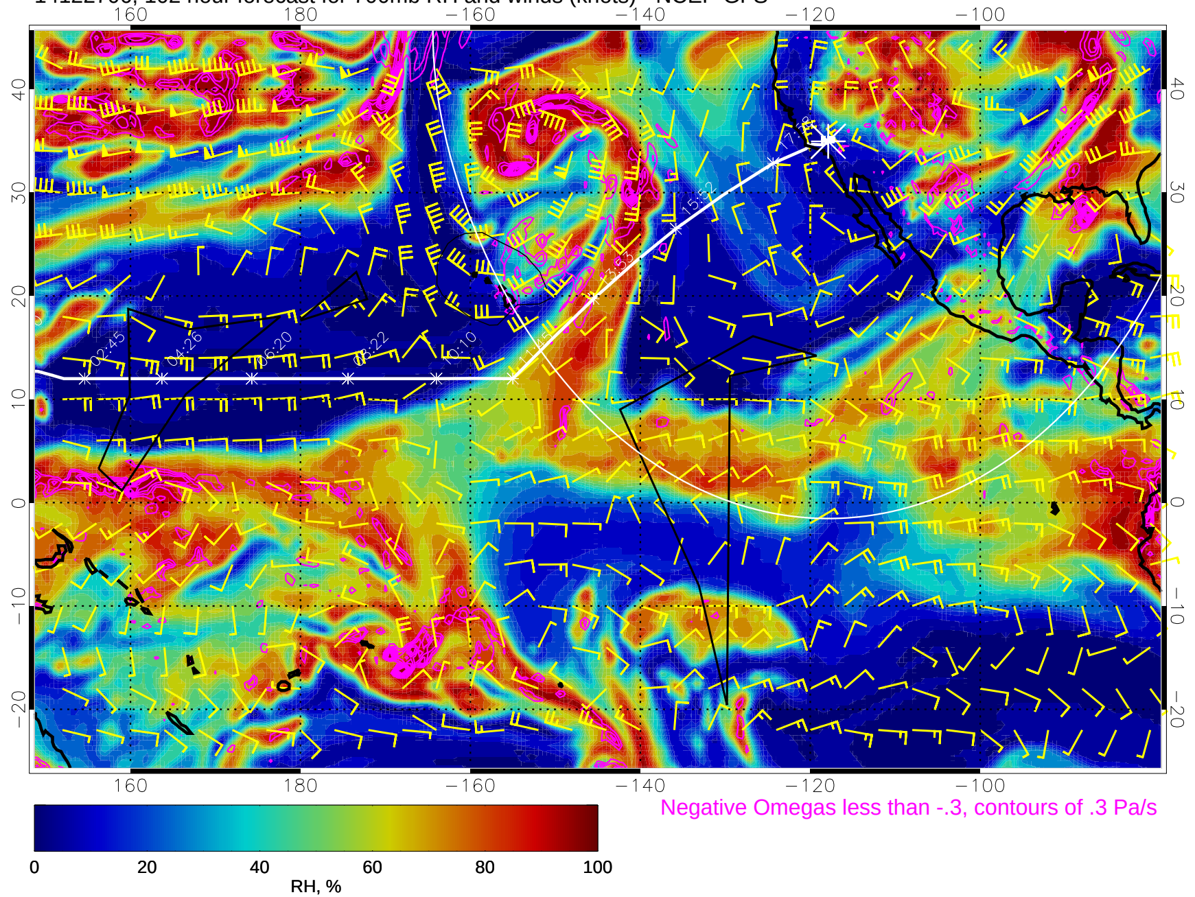
14122706, 102 hour forecast for 700mb RH and winds (knots) - NCEP GFS
