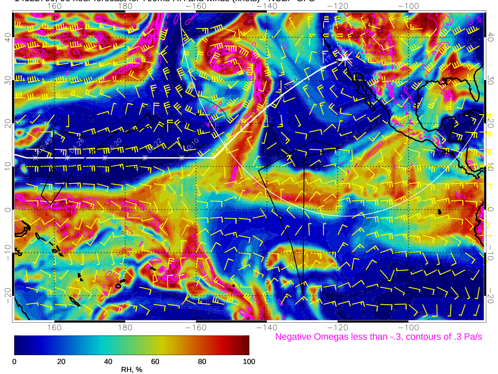
14122700, 96 hour forecast for 700mb RH and winds (knots) - NCEP GFS
