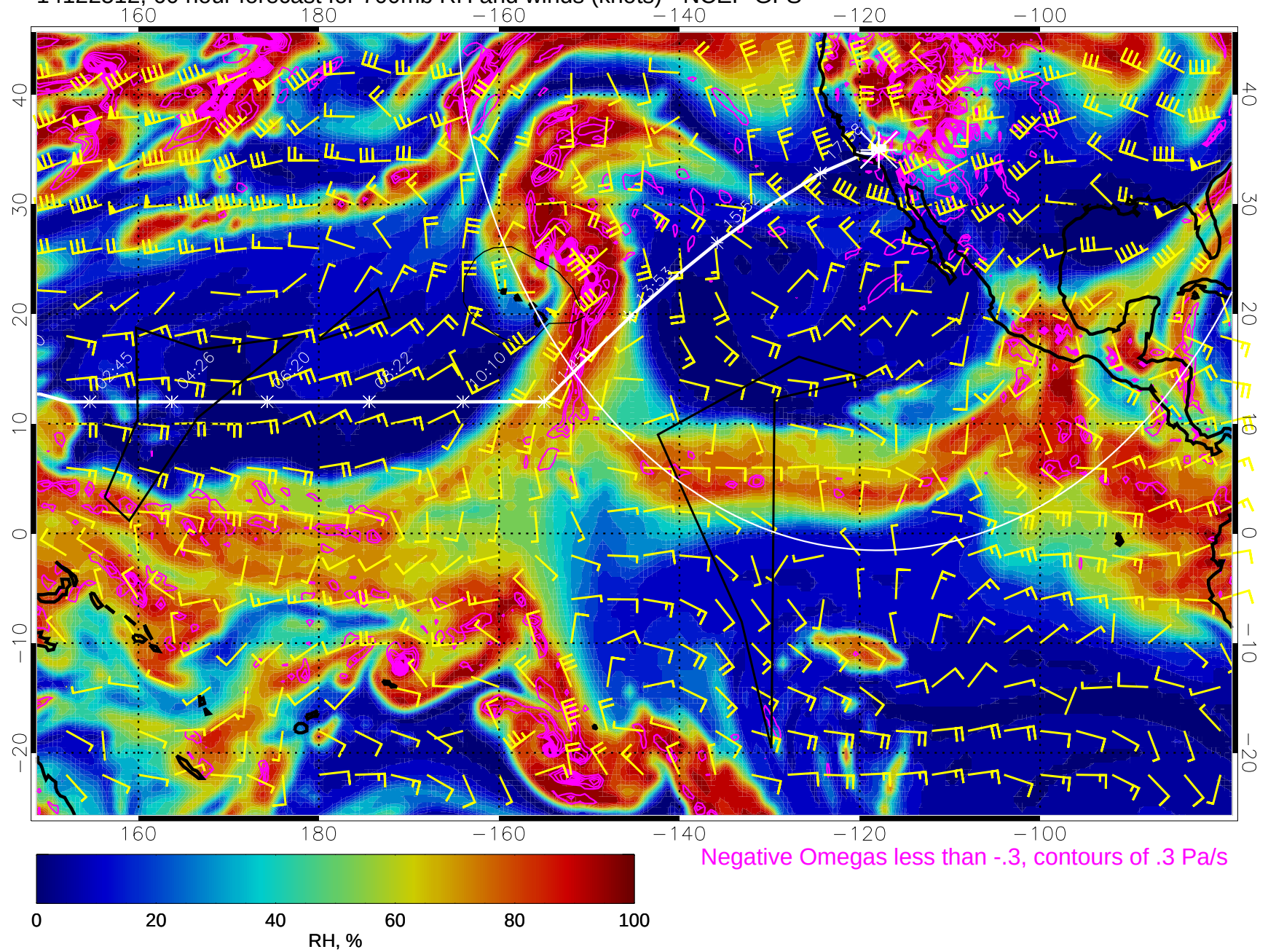
14122512, 60 hour forecast for 700mb RH and winds (knots) - NCEP GFS
