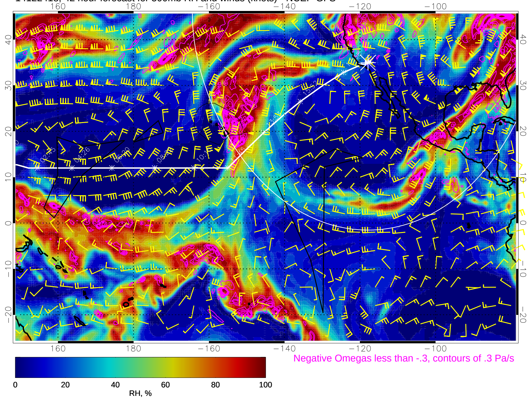
14122418, 42 hour forecast for 500mb RH and winds (knots) - NCEP GFS
