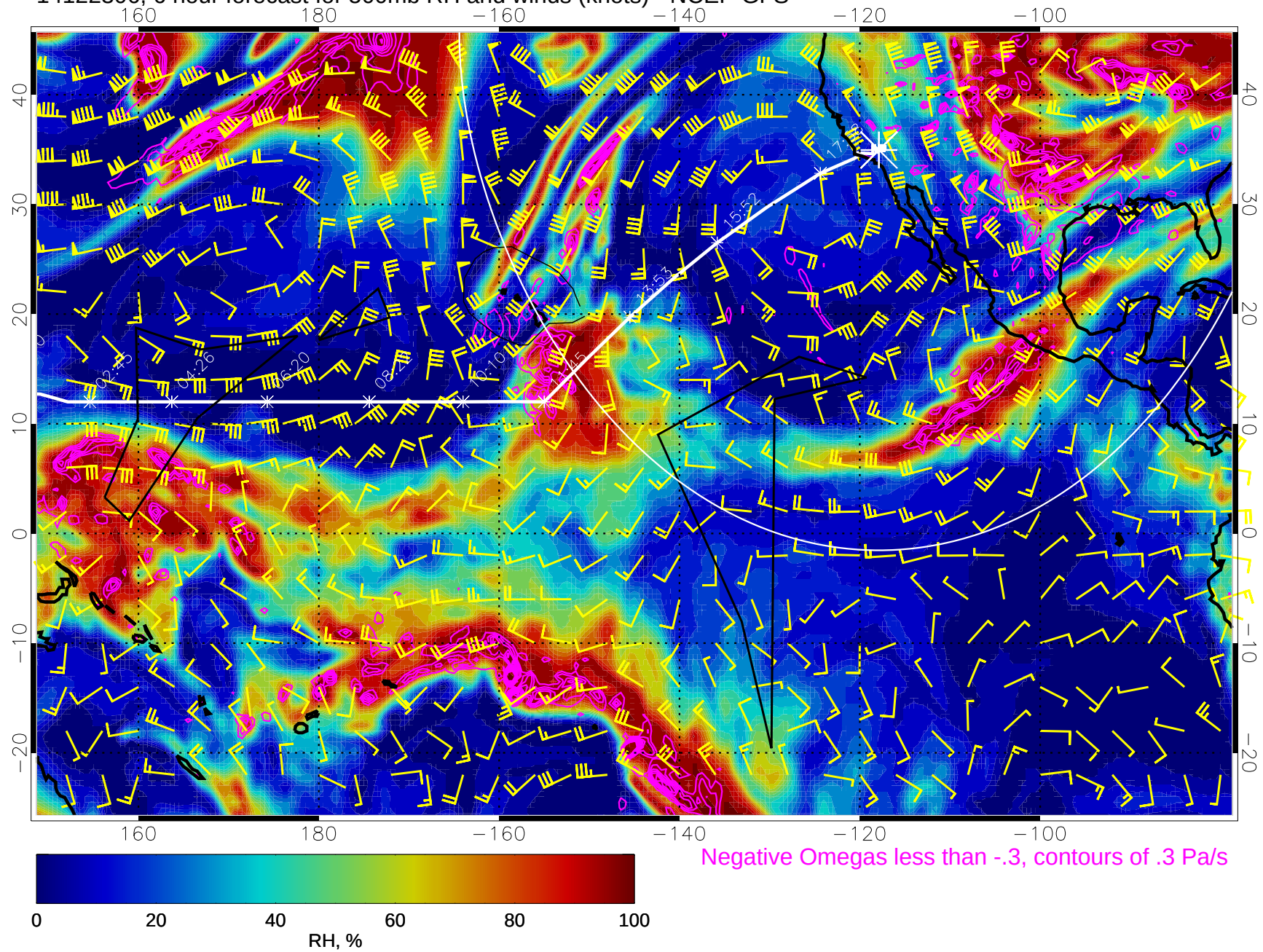
14122306, 6 hour forecast for 500mb RH and winds (knots) - NCEP GFS
