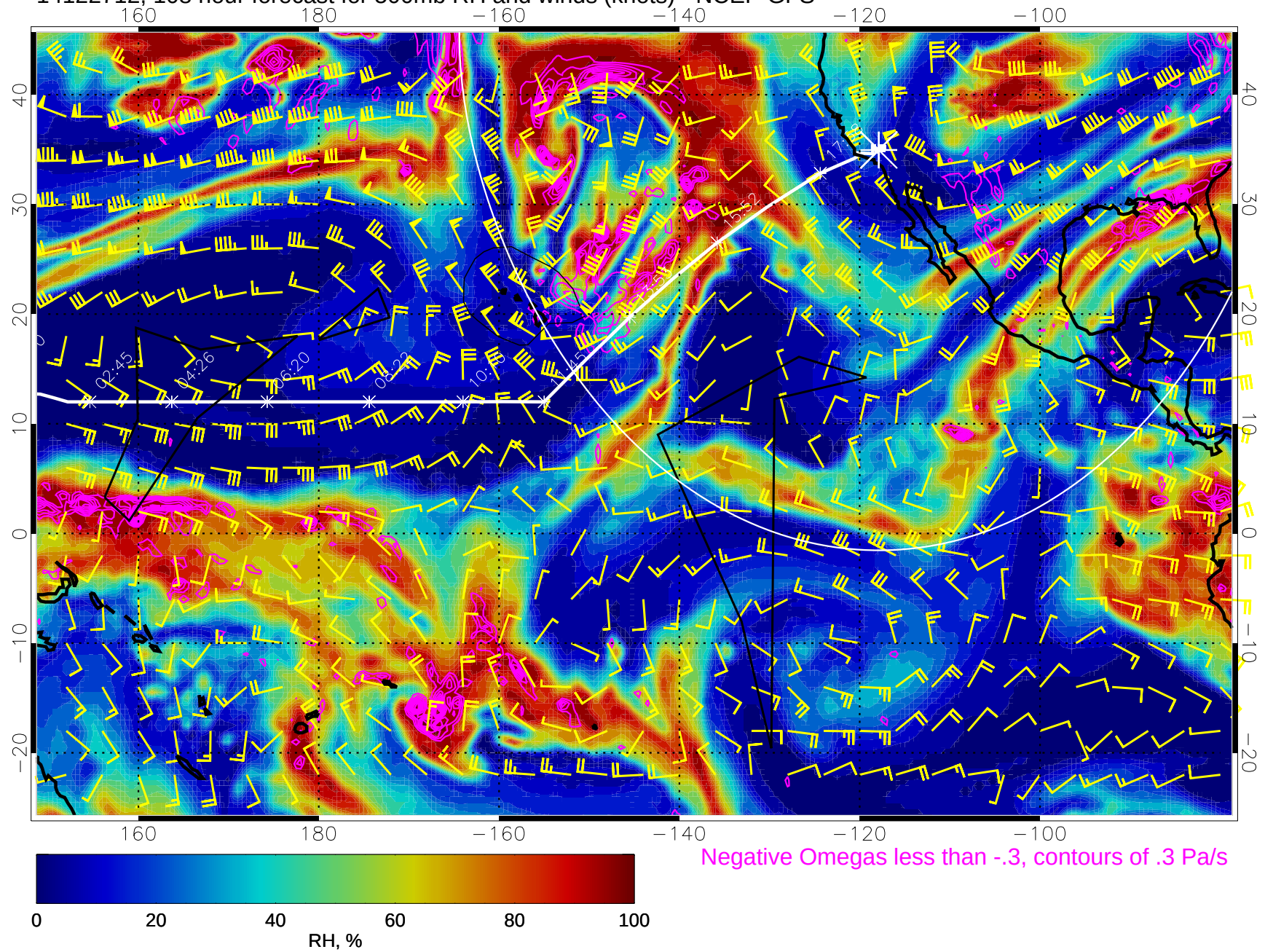
14122712, 108 hour forecast for 500mb RH and winds (knots) - NCEP GFS
