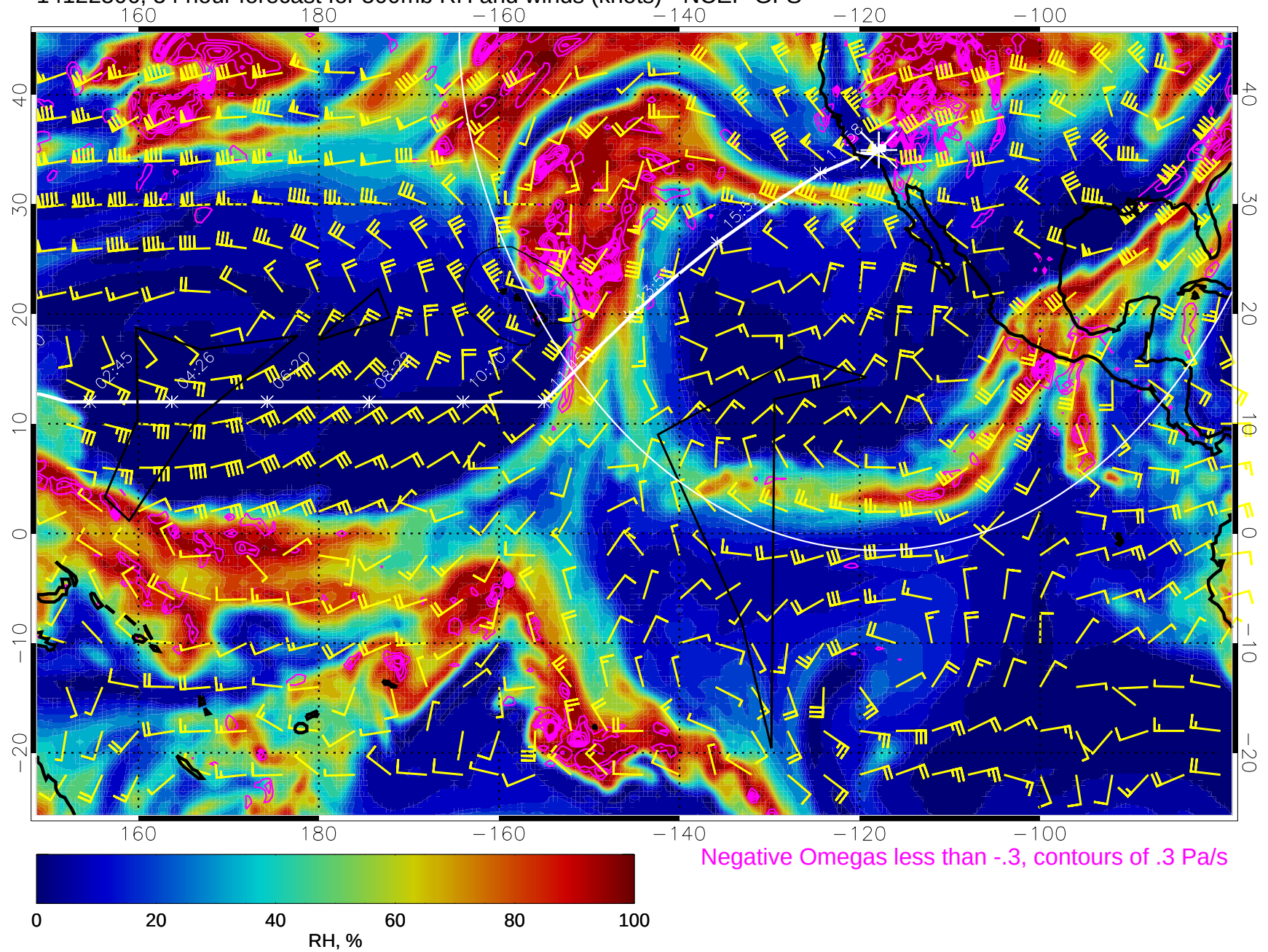
14122506, 54 hour forecast for 500mb RH and winds (knots) - NCEP GFS
