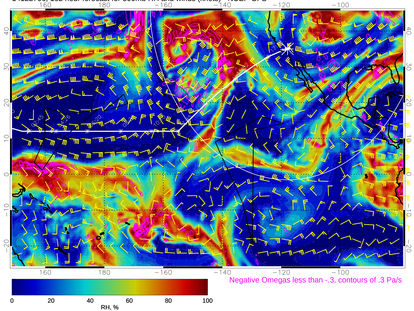
14122706, 102 hour forecast for 500mb RH and winds (knots) - NCEP GFS
