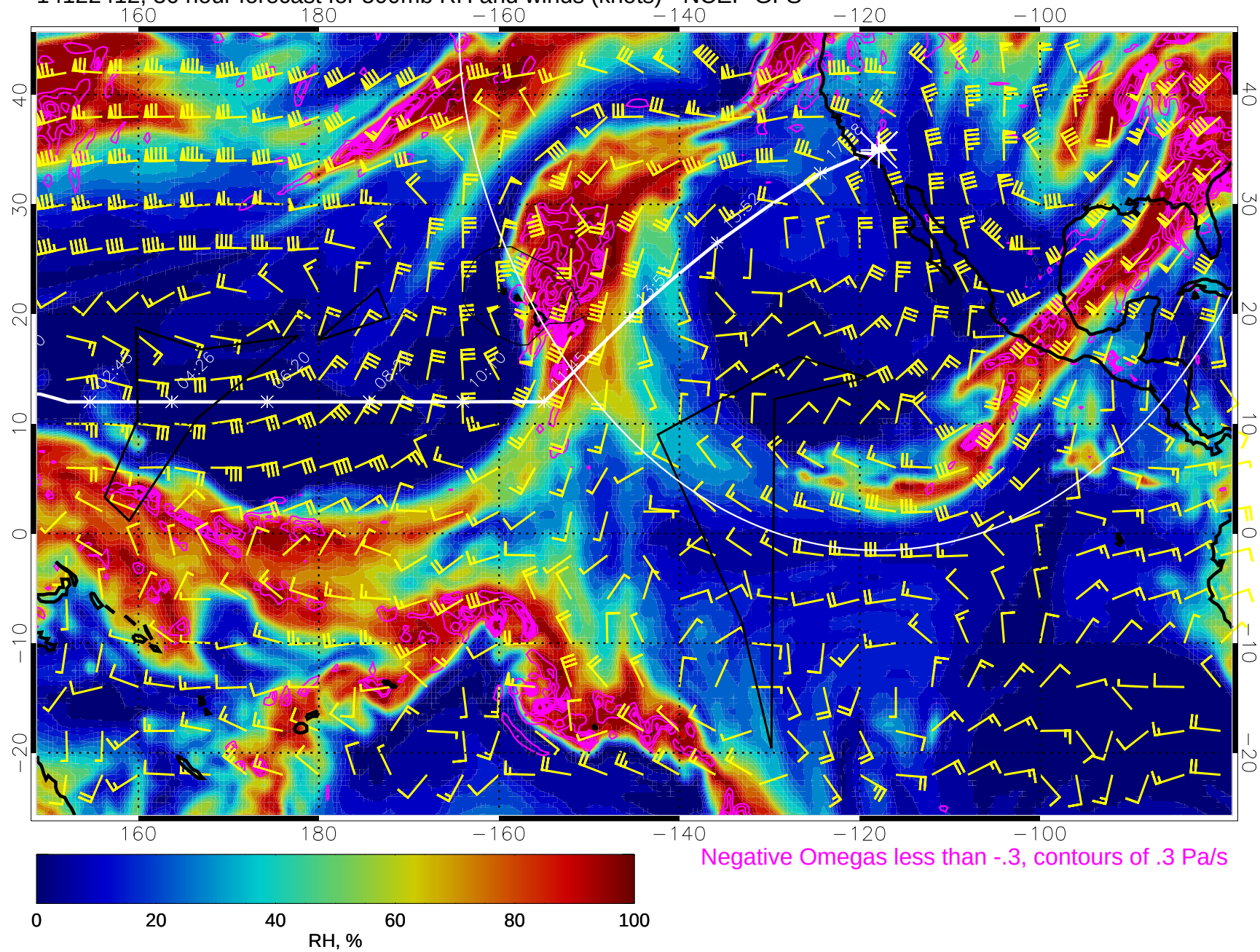
14122412, 36 hour forecast for 500mb RH and winds (knots) - NCEP GFS
