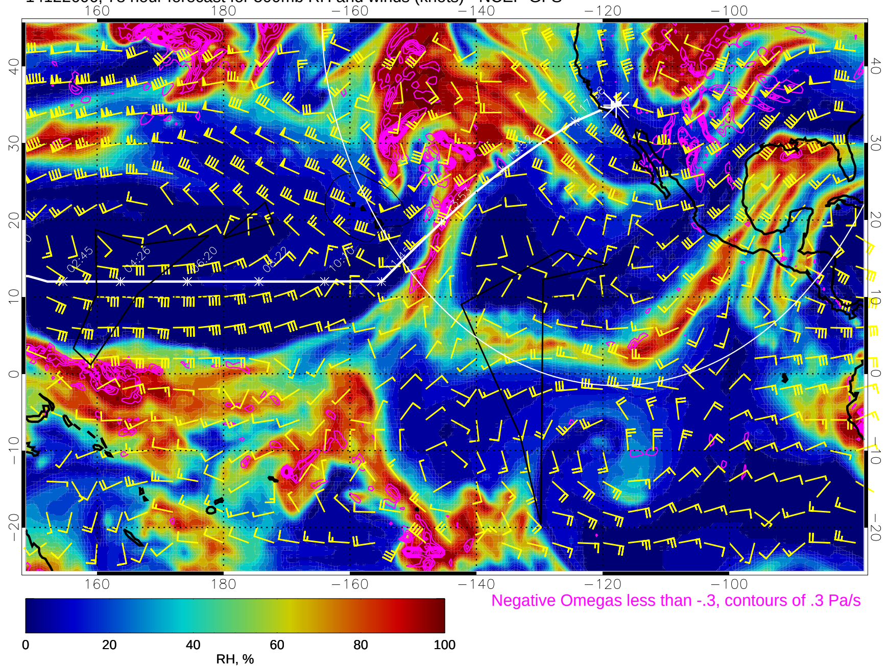
14122606, 78 hour forecast for 500mb RH and winds (knots) - NCEP GFS
