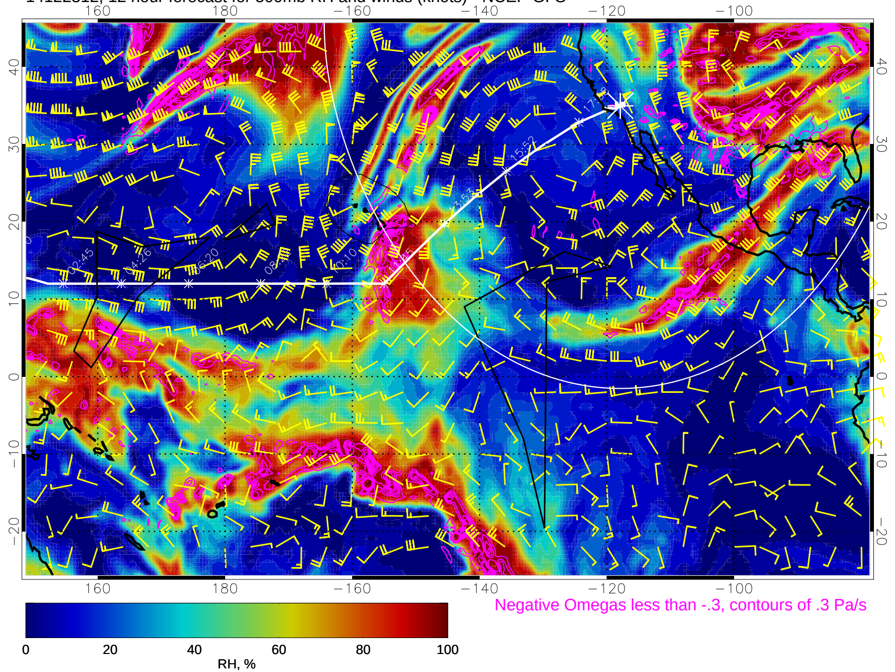
14122312, 12 hour forecast for 500mb RH and winds (knots) - NCEP GFS
