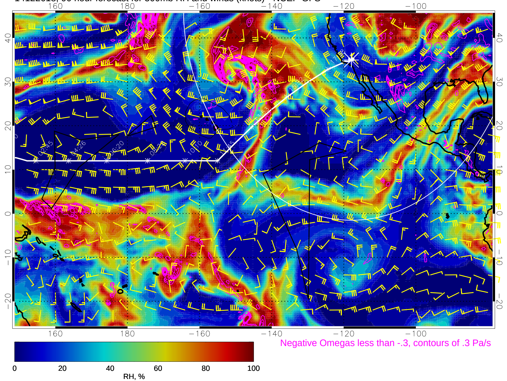
14122618, 90 hour forecast for 500mb RH and winds (knots) - NCEP GFS
