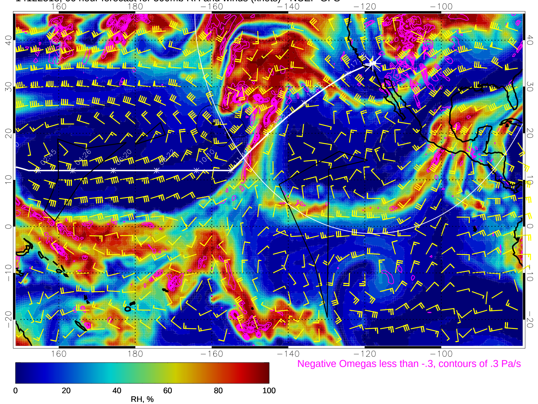
14122518, 66 hour forecast for 500mb RH and winds (knots) - NCEP GFS
