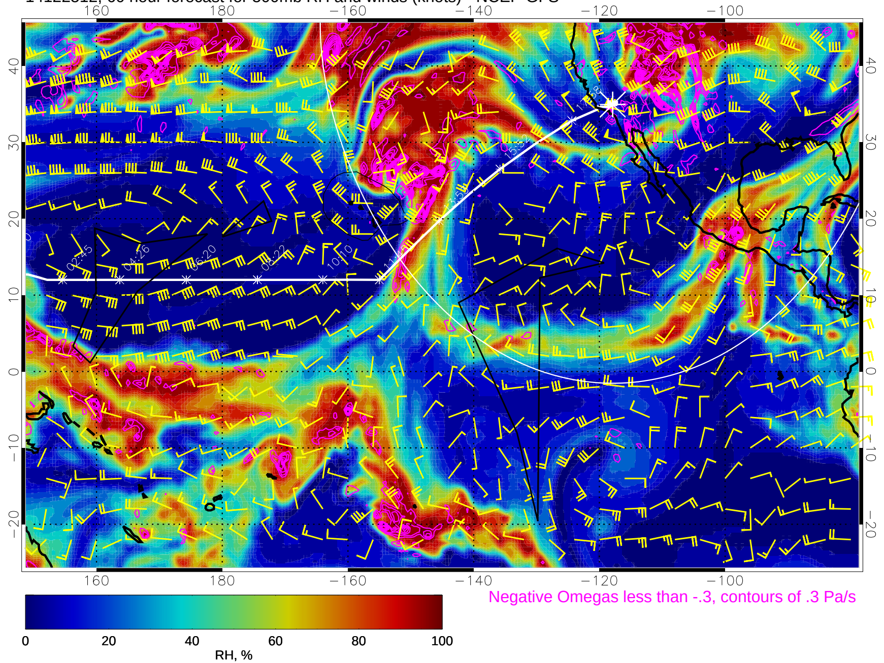
14122512, 60 hour forecast for 500mb RH and winds (knots) - NCEP GFS
