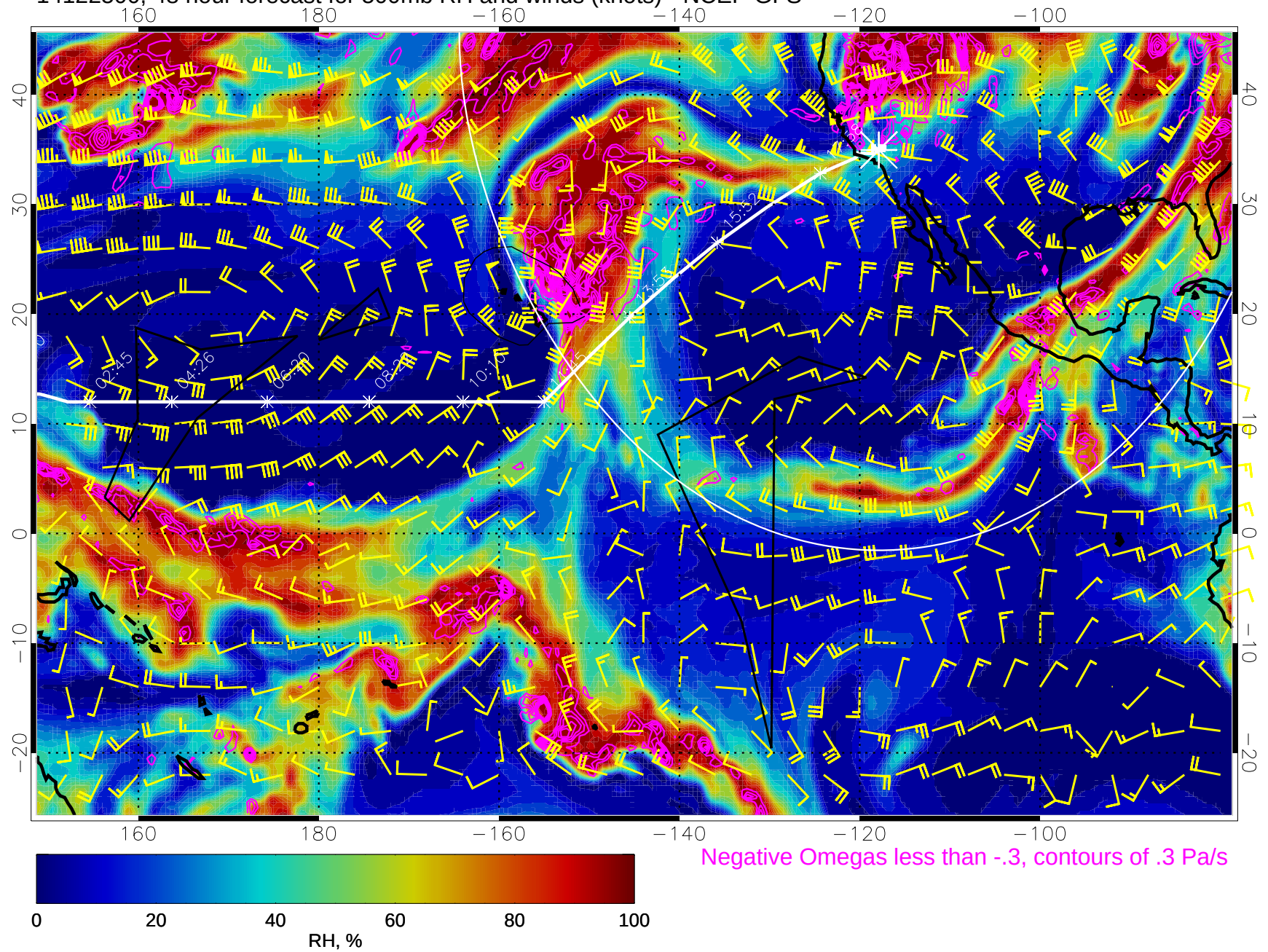
14122500, 48 hour forecast for 500mb RH and winds (knots) - NCEP GFS
