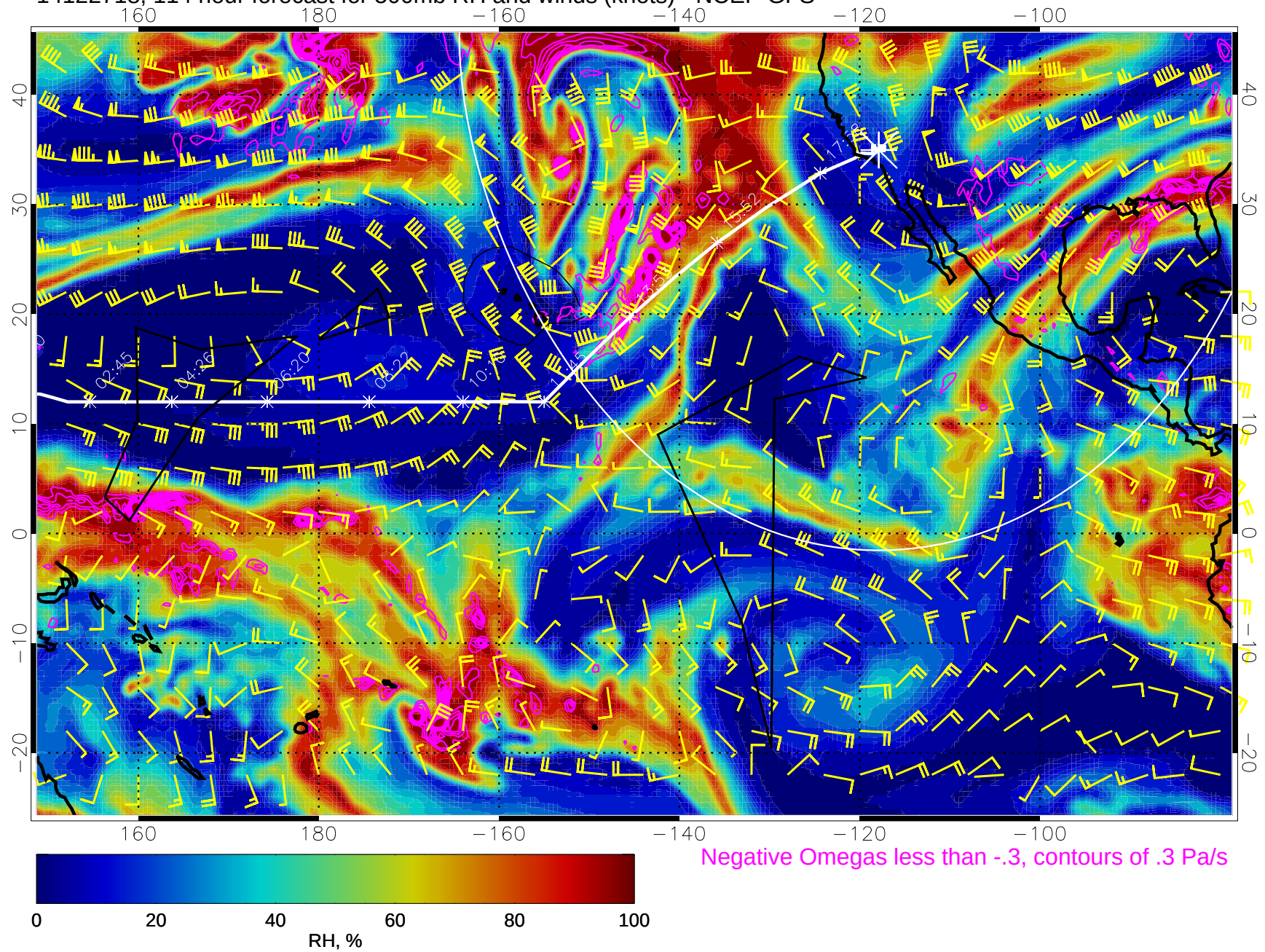
14122718, 114 hour forecast for 500mb RH and winds (knots) - NCEP GFS
