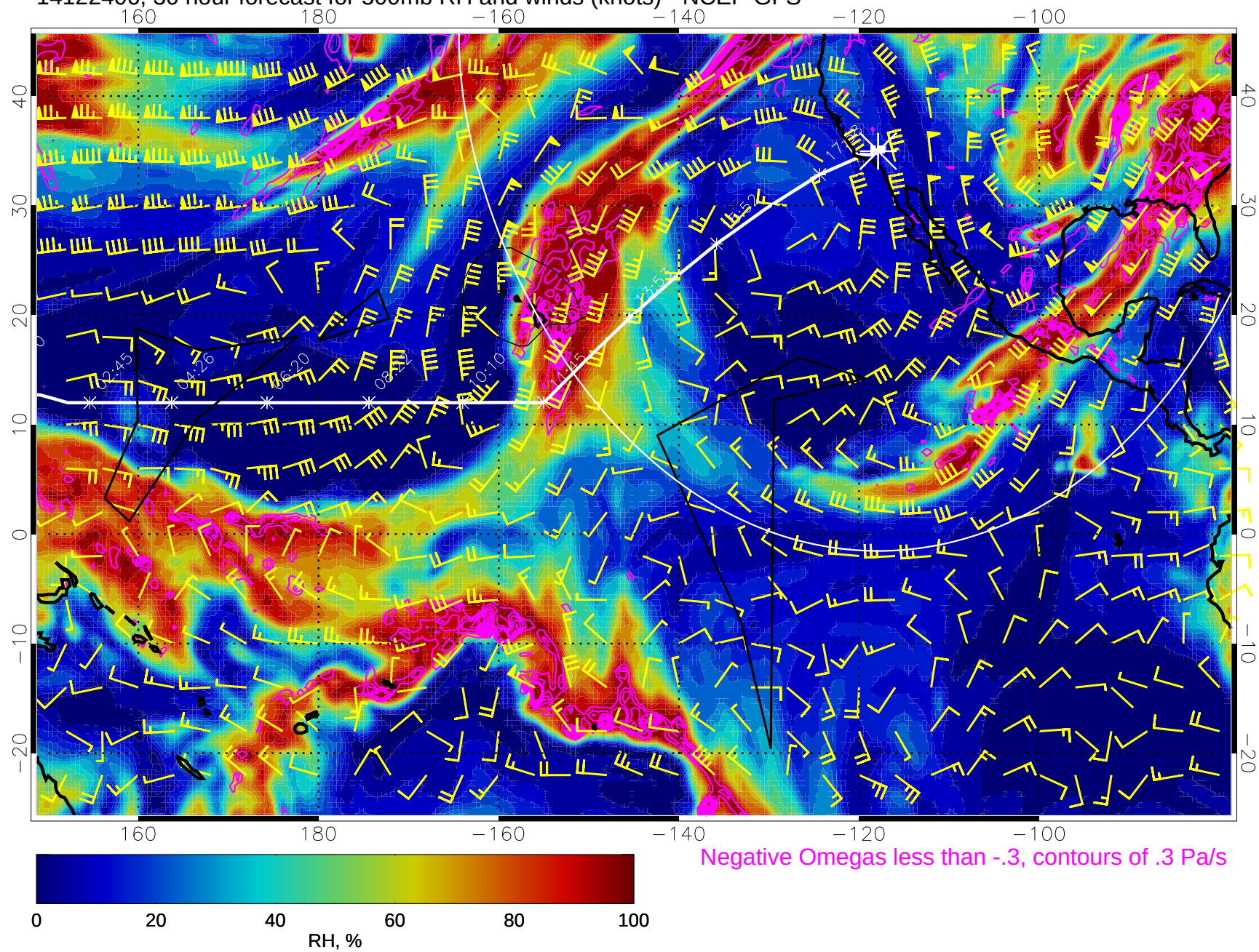
14122406, 30 hour forecast for 500mb RH and winds (knots) - NCEP GFS
