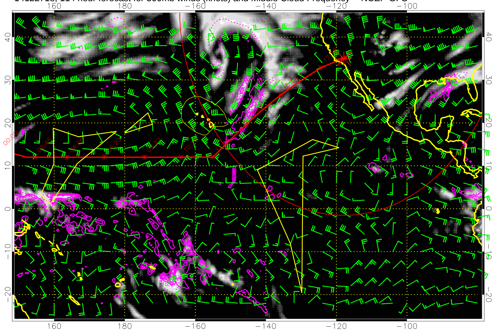
14122718, 114 hour forecast for 500mb winds (knots) and Middle Cloud Frequency -- NCEP GFS
