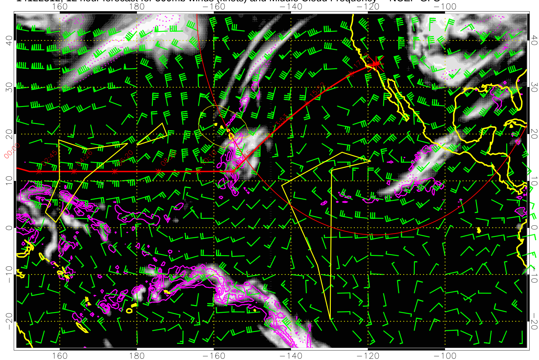
14122312, 12 hour forecast for 500mb winds (knots) and Middle Cloud Frequency -- NCEP GFS
