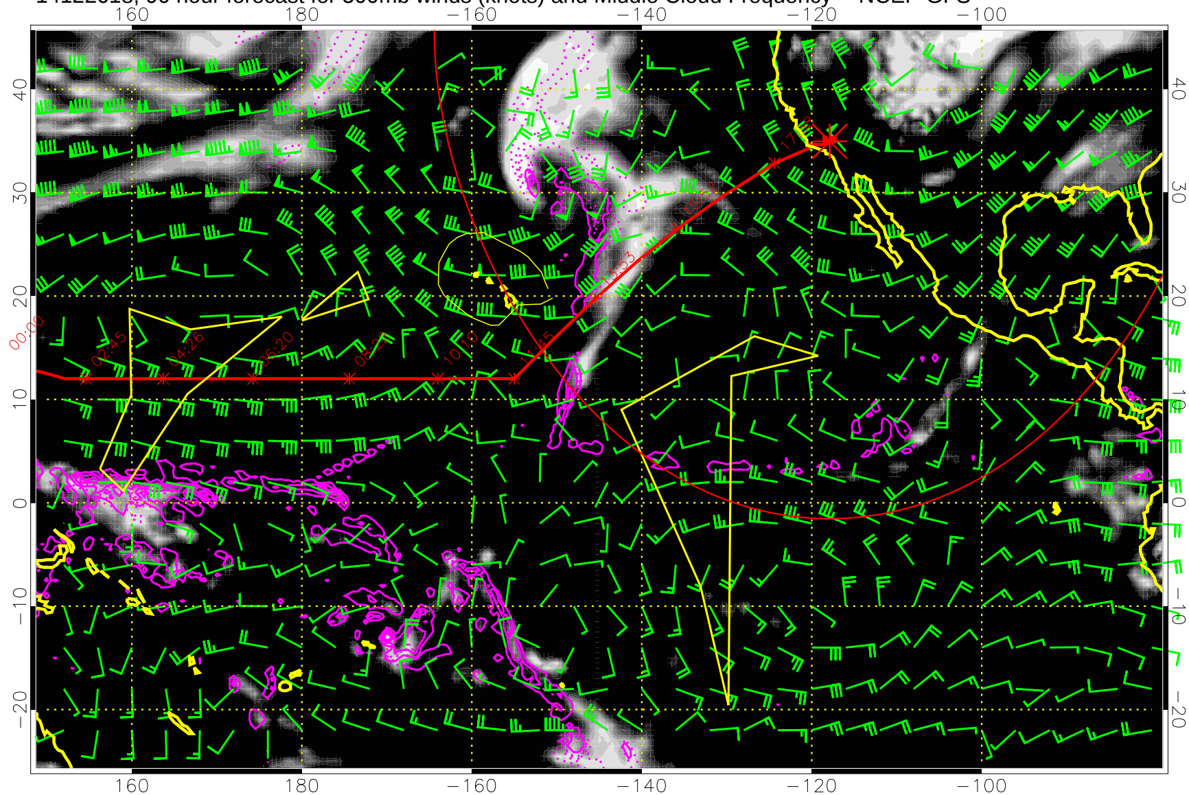
14122618, 90 hour forecast for 500mb winds (knots) and Middle Cloud Frequency -- NCEP GFS
