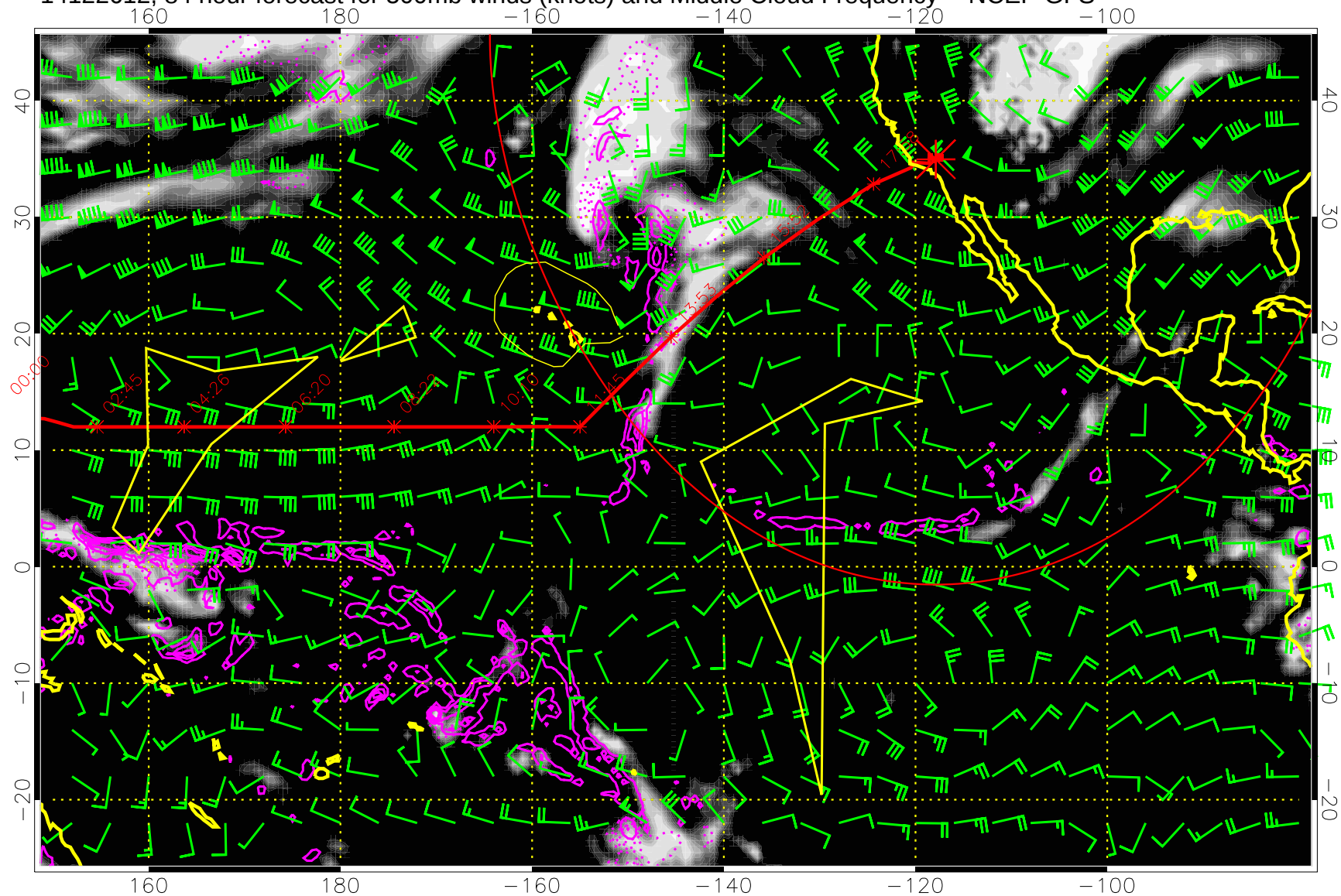
14122612, 84 hour forecast for 500mb winds (knots) and Middle Cloud Frequency -- NCEP GFS
