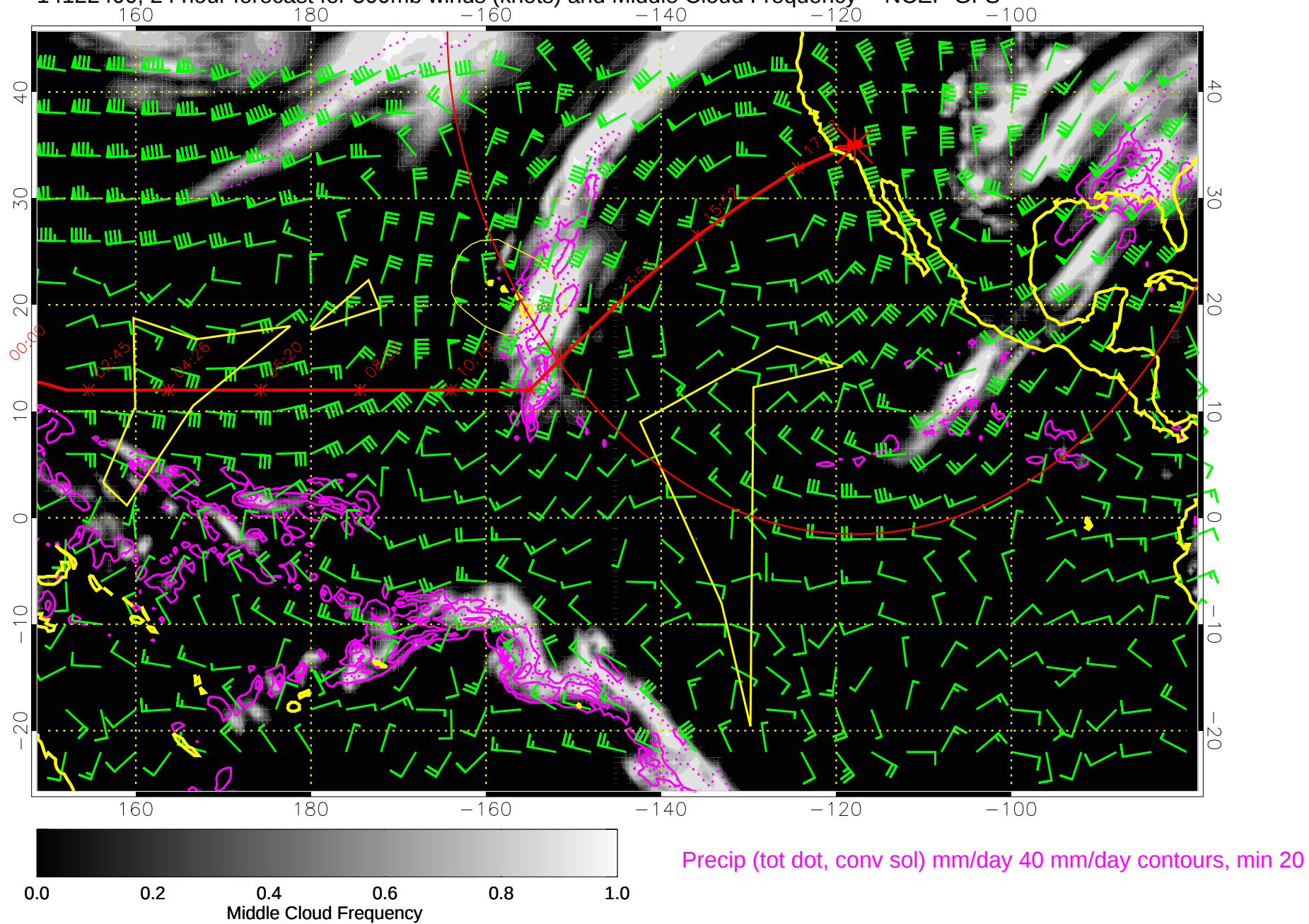
14122400, 24 hour forecast for 500mb winds (knots) and Middle Cloud Frequency -- NCEP GFS
