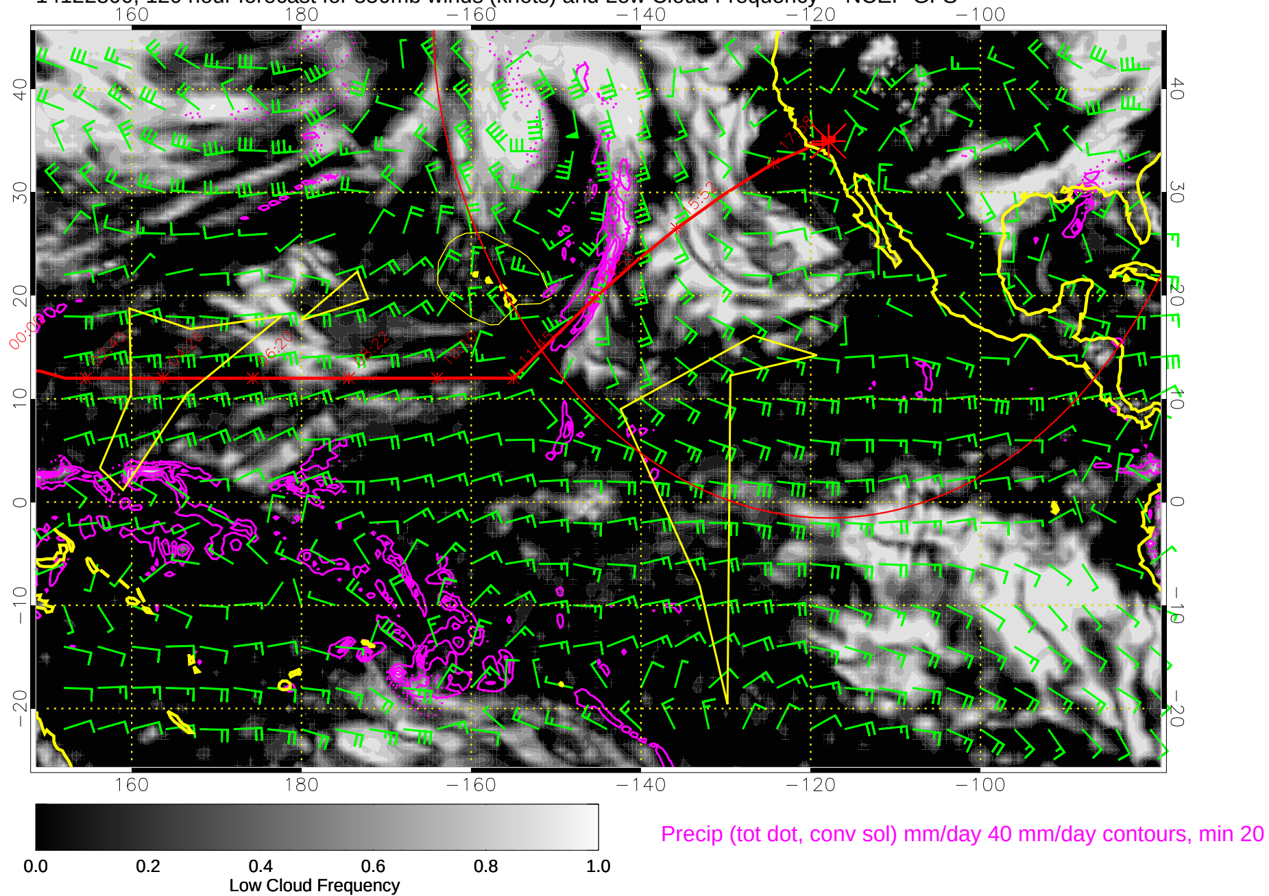
14122800, 120 hour forecast for 850mb winds (knots) and Low Cloud Frequency -- NCEP GFS
