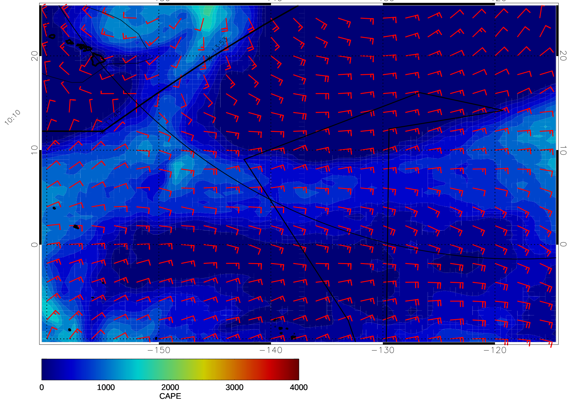
14122706, 102 hour forecast for CAPE and surface winds (knots) -- NCEP GFS
