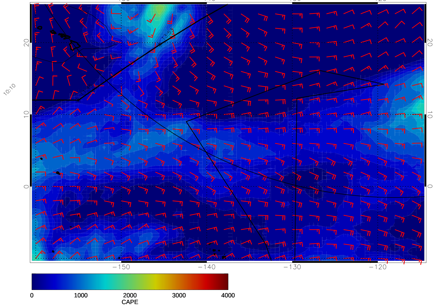
14122718, 114 hour forecast for CAPE and surface winds (knots) -- NCEP GFS
